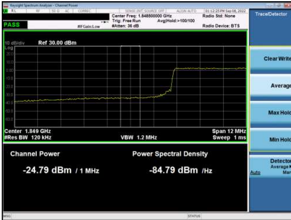
Plot 7-38. Extended Lower Band Edge Plot (LTE Band 2 - 15MHz QPSK – Full RB)
