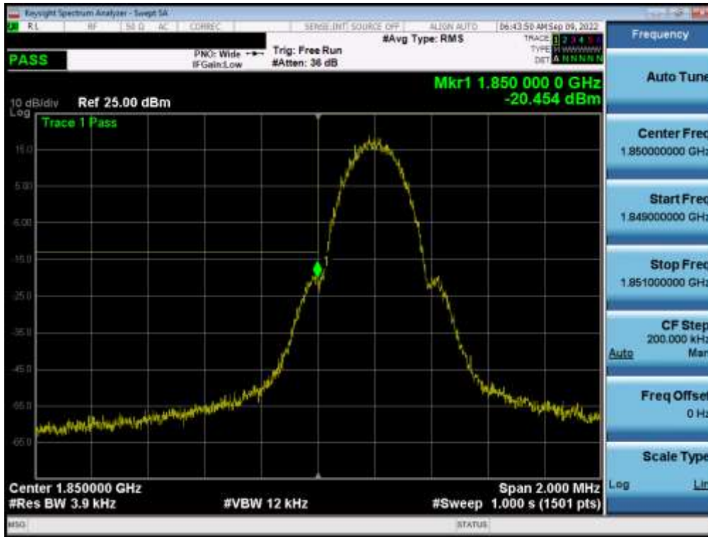
Plot 7-57. Lower Band Edge Plot (GPRS PCS – Ch. 512)
