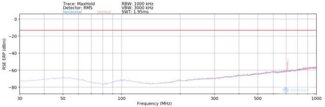
Plot 7-73. Radiated Spurious Plot (LTE Band 2) – Below 1GHz
