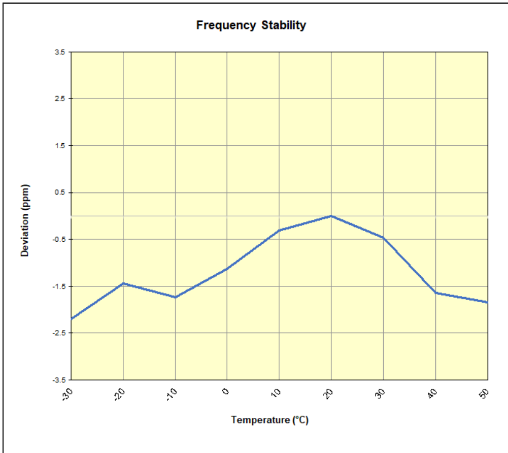
Plot 7-78. GSM/GPRS PCS Frequency Stability Chart
