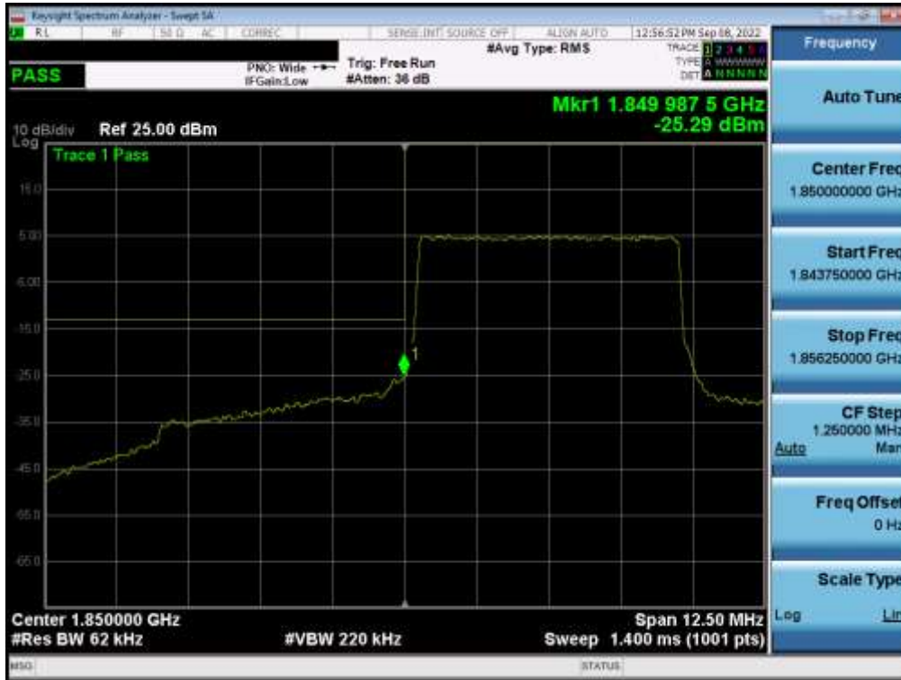
Plot 7-45. Lower Band Edge Plot (LTE Band 2 - 5MHz QPSK – Full RB)
