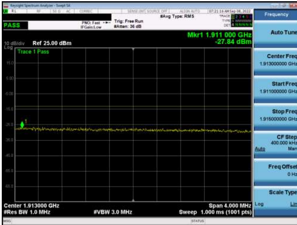
Plot 7-36. Extended Upper Band Edge Plot (LTE Band 2 - 20MHz QPSK – Full RB)
