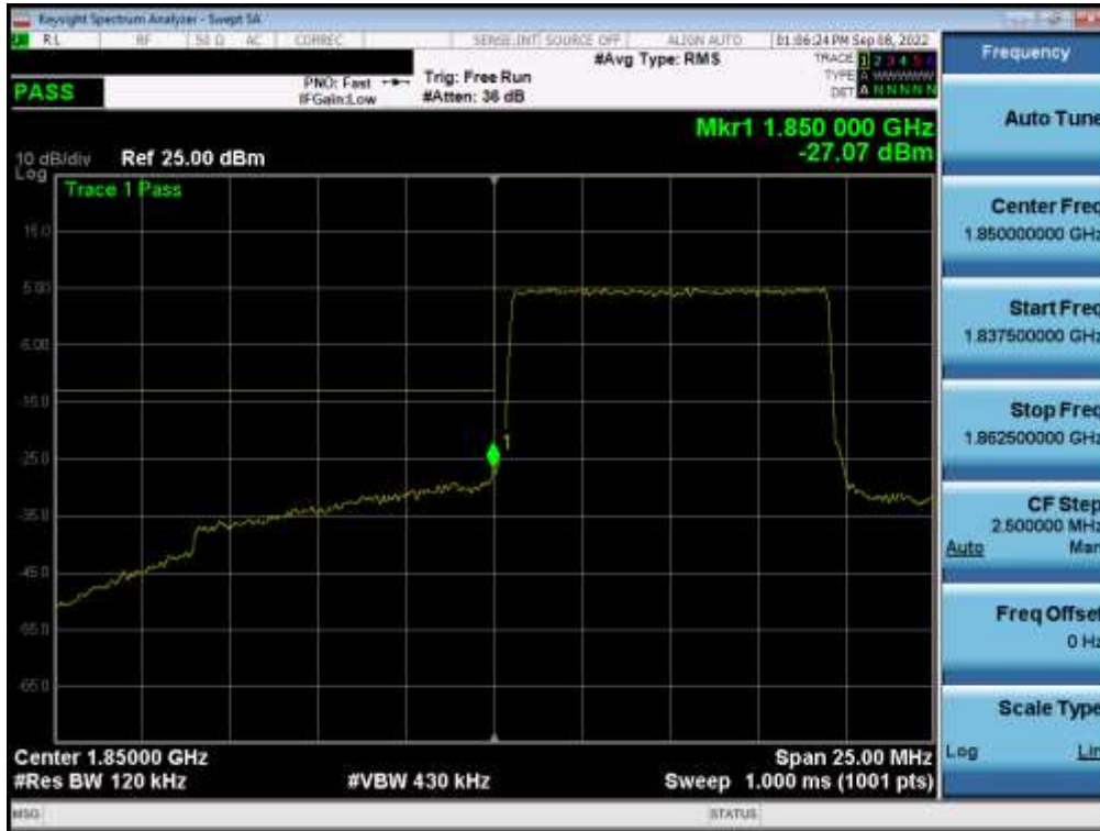
Plot 7-41. Lower Band Edge Plot (LTE Band 2 - 10MHz QPSK – Full RB)
