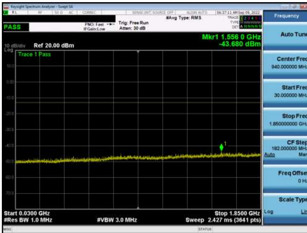
Plot 7-27. Conducted Spurious Plot (GPRS Ch. 661)
