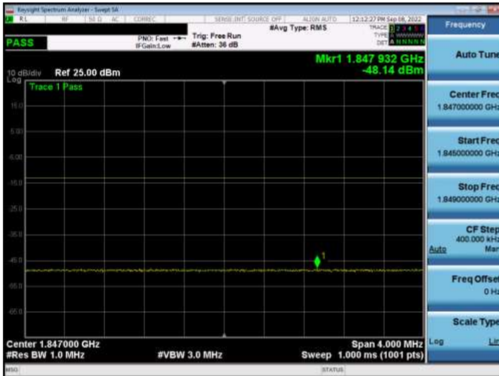
Plot 7-54. Extended Lower Band Edge Plot (LTE Band 2 – 1.4MHz QPSK – Full RB)
