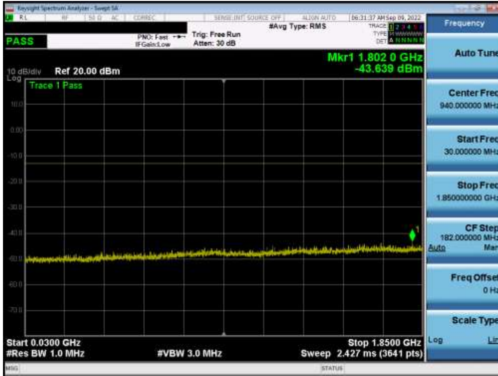
Plot 7-30. Conducted Spurious Plot (GPRS Ch. 810)
