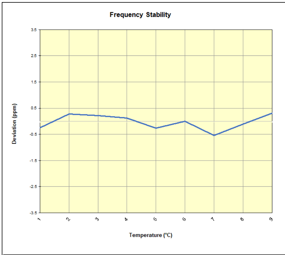
Plot 7-77. LTE Band 2 Frequency Stability Chart
