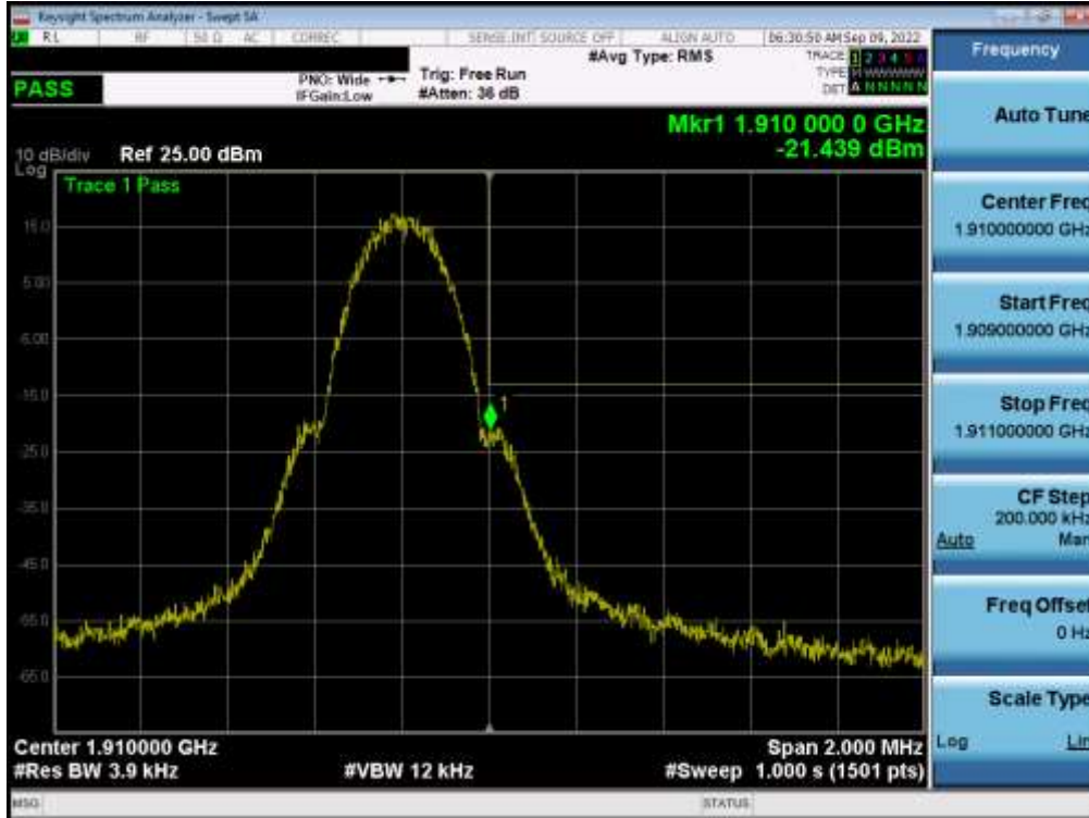
Plot 7-58. Upper Band Edge Plot (GPRS PCS – Ch. 810)
