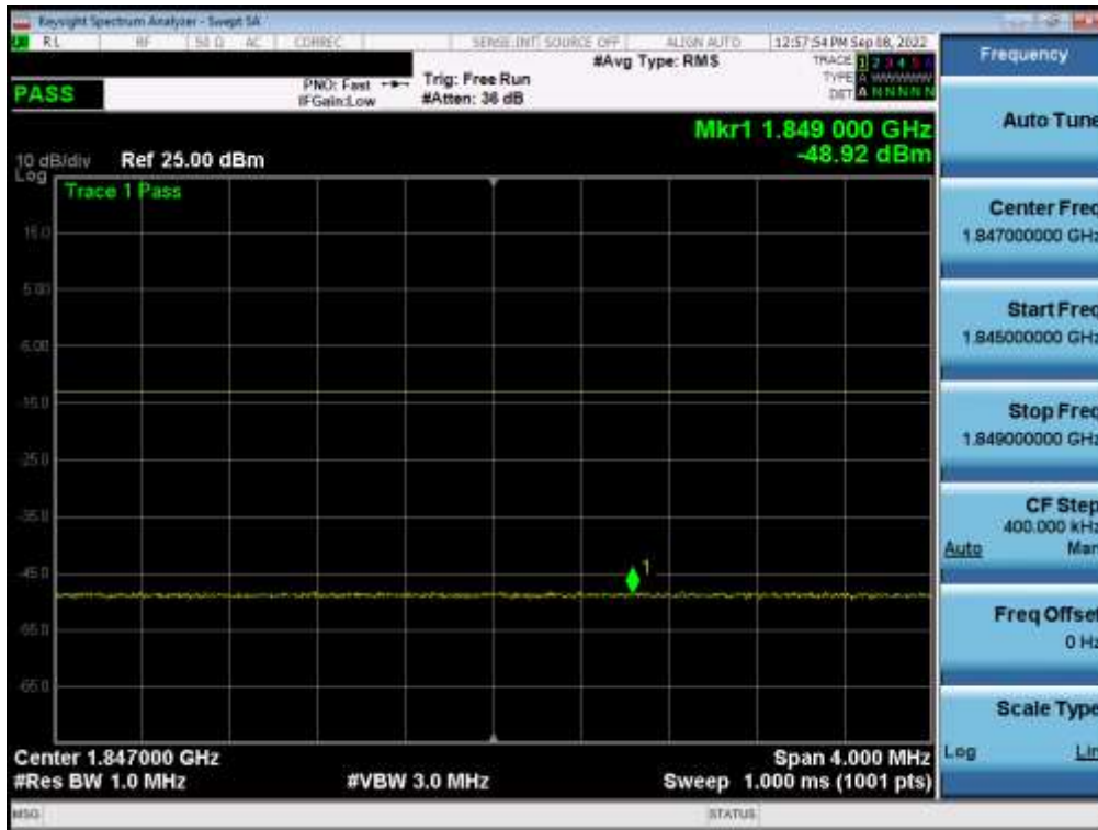
Plot 7-46. Extended Lower Band Edge Plot (LTE Band 2 - 5MHz QPSK – Full RB)
