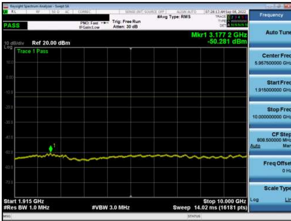
Plot 7-16. Conducted Spurious Plot (LTE Band 2 - 20MHz QPSK - 1RB - Low Channel)
