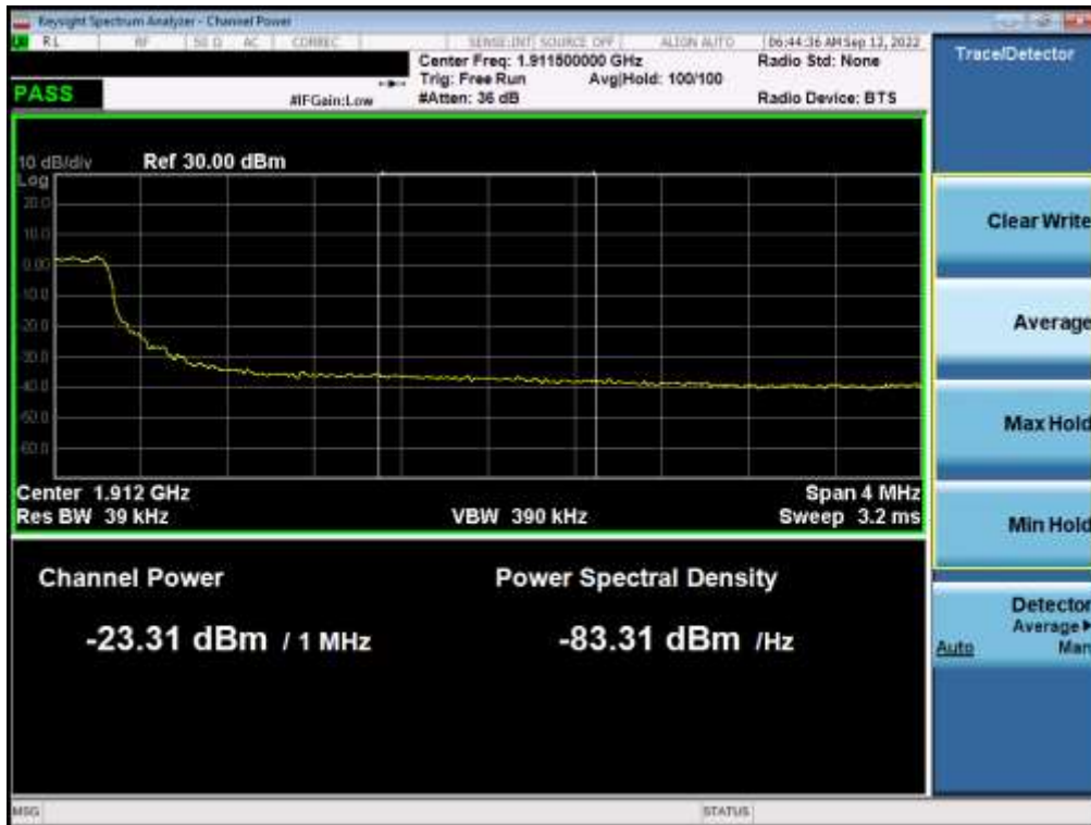
Plot 7-48. Extended Upper Band Edge Plot (LTE Band 2 - 5MHz QPSK – Full RB)
