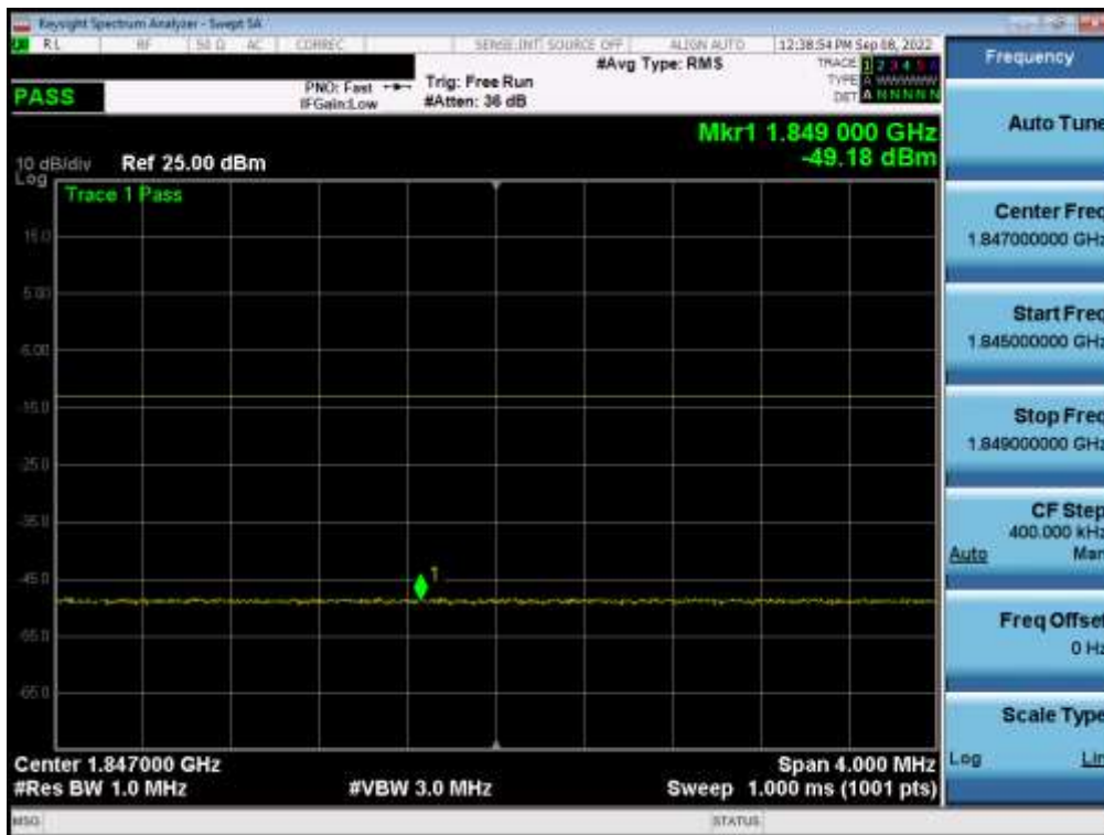
Plot 7-50. Extended Lower Band Edge Plot (LTE Band 2 - 3MHz QPSK – Full RB)
