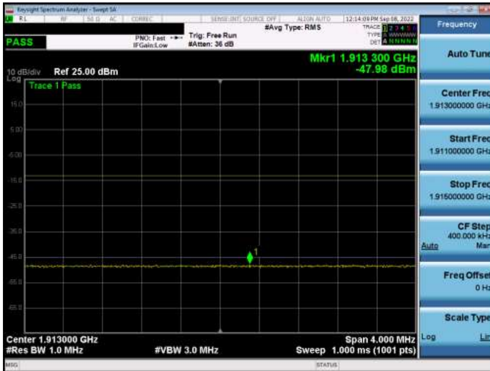
Plot 7-56. Extended Upper Band Edge Plot (LTE Band 2 – 1.4MHz QPSK – Full RB)
