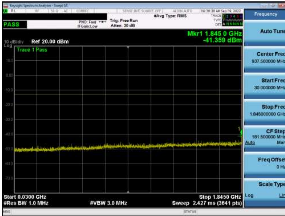
Plot 7-24. Conducted Spurious Plot (GPRS Ch. 512)
