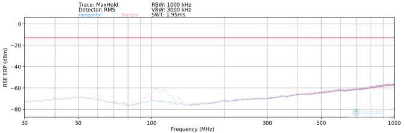
Plot 7-75. Radiated Spurious Plot (GPRS PCS) – Below 1GHz
