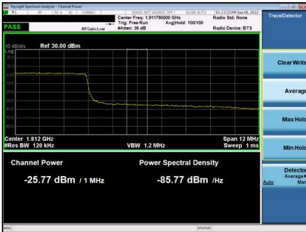
Plot 7-40. Extended Upper Band Edge Plot (LTE Band 2 - 15MHz QPSK – Full RB)
