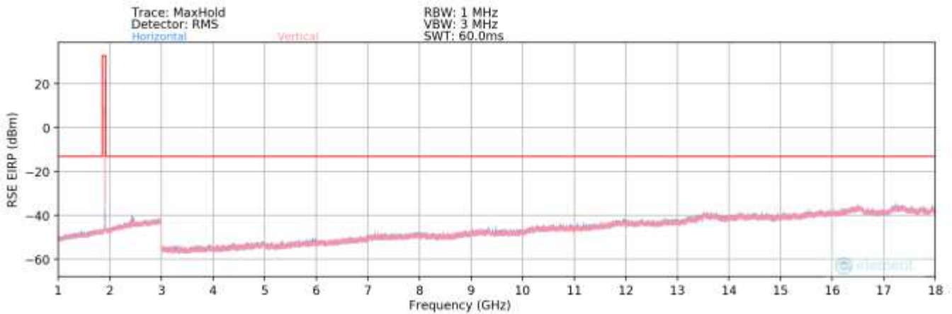
Plot 7-74. Radiated Spurious Plot (LTE Band 2) – Above 1GHz
