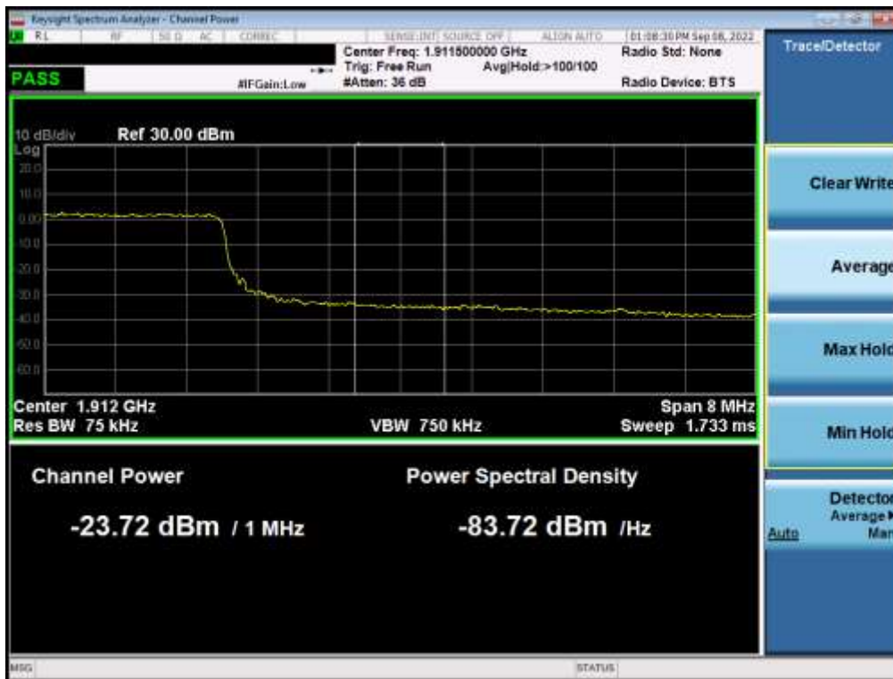
Plot 7-44. Extended Upper Band Edge Plot (LTE Band 2 - 10MHz QPSK – Full RB)
