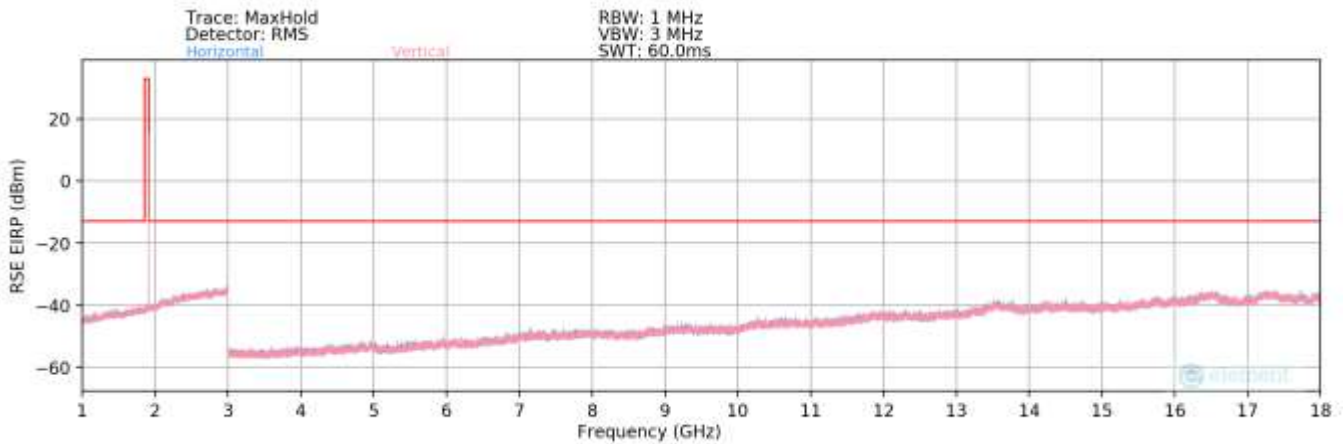
Plot 7-76. Radiated Spurious Plot (GPRS PCS) – Above 1GHz
