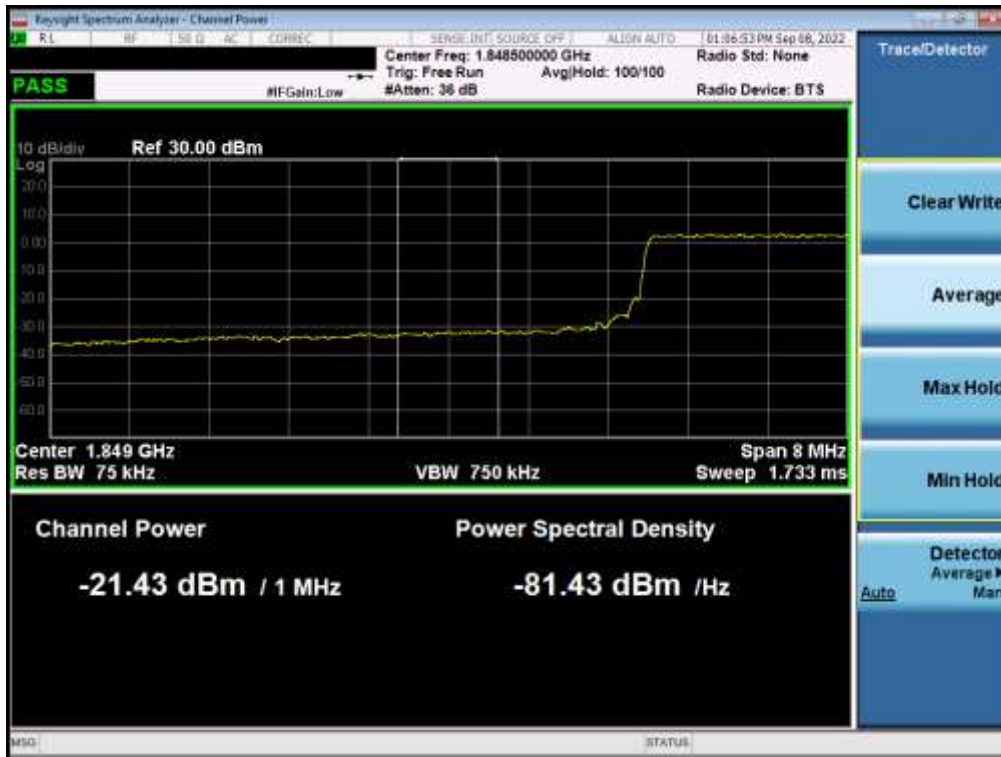
Plot 7-42. Extended Lower Band Edge Plot (LTE Band 2 - 10MHz QPSK – Full RB)
