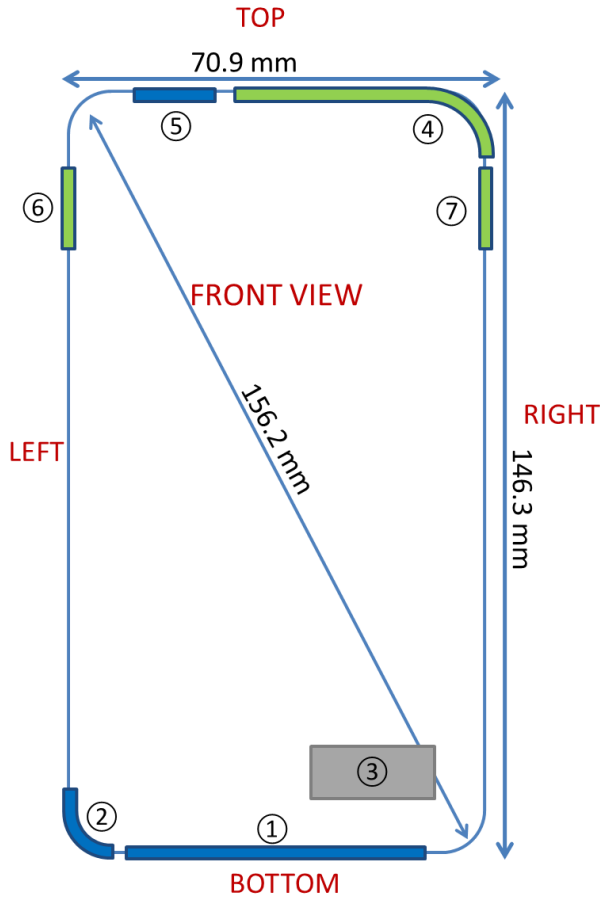
Figure K-1 DUT Antenna Locations
