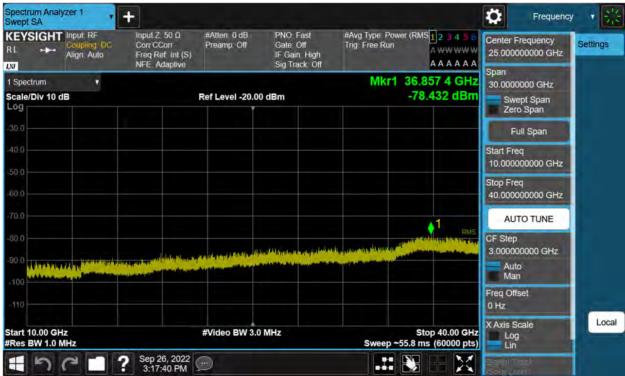
Sub6 n77. Conducted Spurious Plot_2 (634666ch_60 MHz_BPSK)
