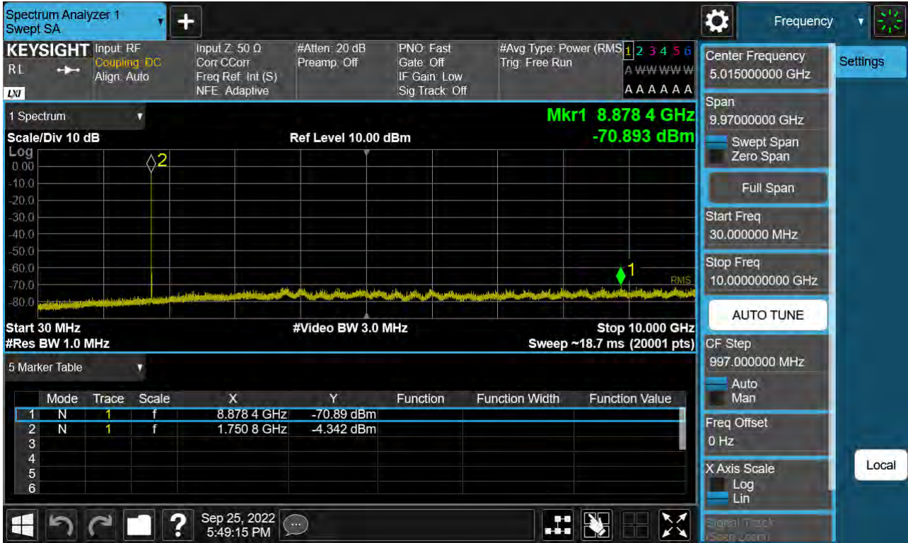
Sub6 n66. Conducted Spurious Plot_1 (353000ch_30 MHz_BPSK_RB 1_1)
