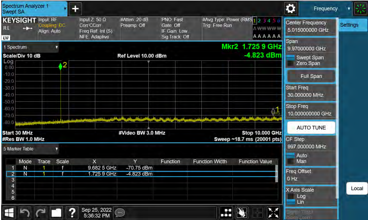
Sub6 n66. Conducted Spurious Plot_1 (349000ch_40 MHz_BPSK_RB 1_1)
