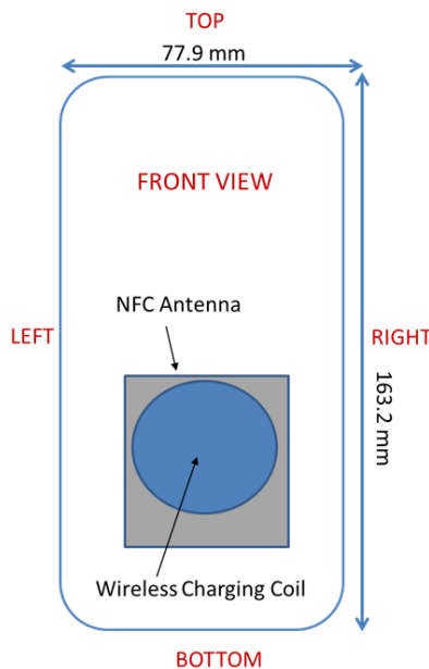
Figure F-2 NFC Antenna Locations
