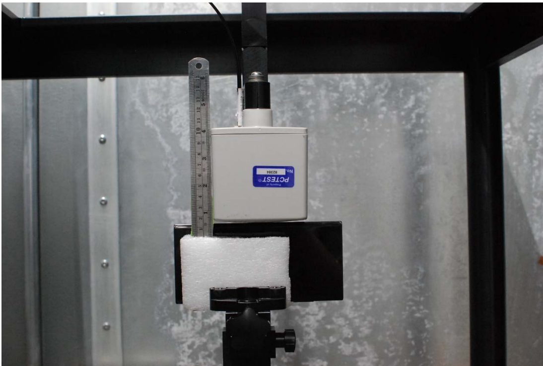
Test Setup Photo 42 H-field, Left edge, 0cm
