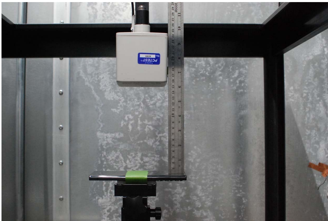
Test Setup Photo 32 H-field, Front side, 15cm
