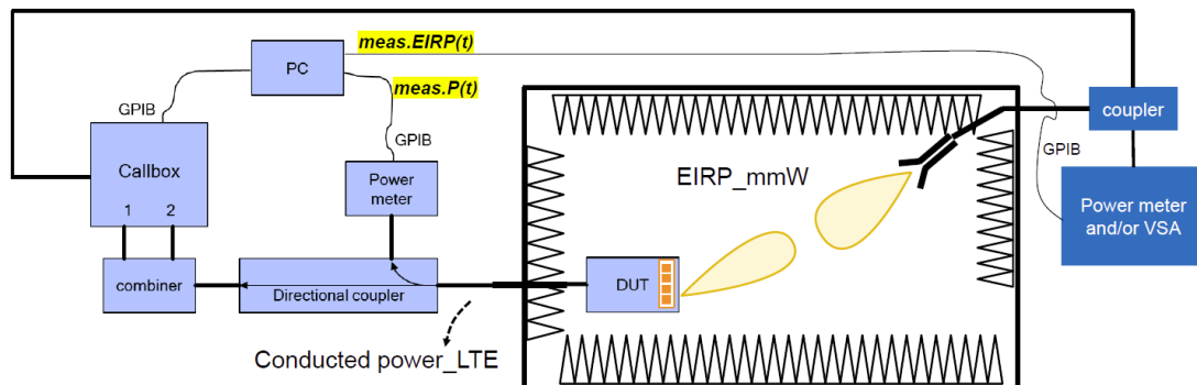
Figure 7-1 mmW NR radiated power measurement setup – Test Setup Photo 13
