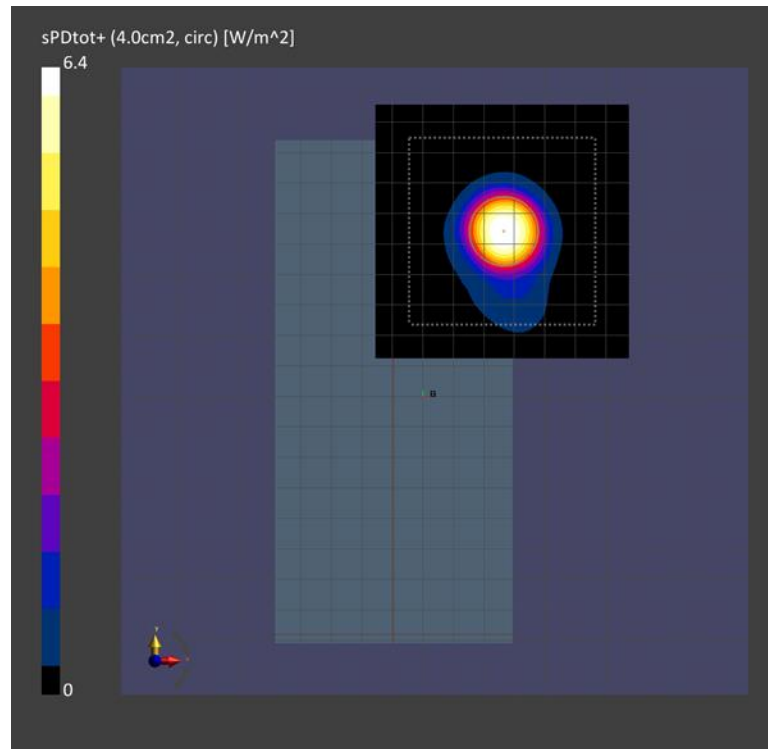
Figure 10-1 4cm 2 psPD distribution measured at input.power.limit of 10.4 dBm on the back side for n261 beam 8
