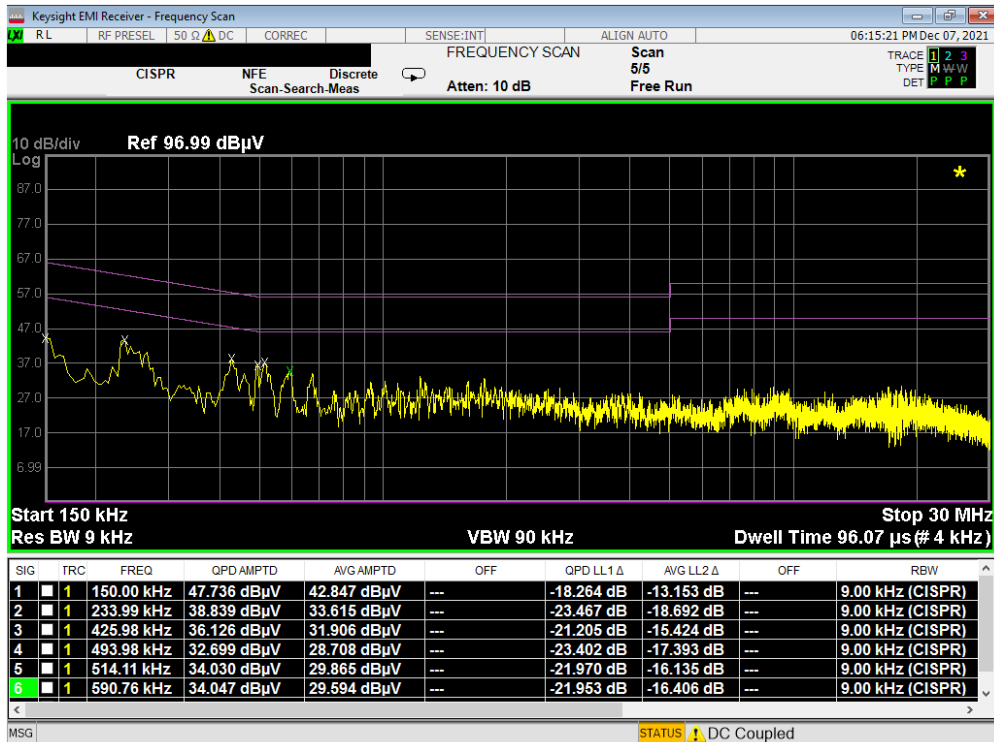
Plot 7-26. Line-Conducted Test Plot (N) - Device to S-Pen
