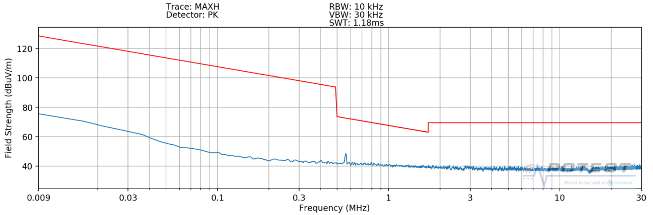
Plot 7-11. Radiated Spurious Plot 9kHz – 30MHz (Pol. Y – Device to S-Pen)
