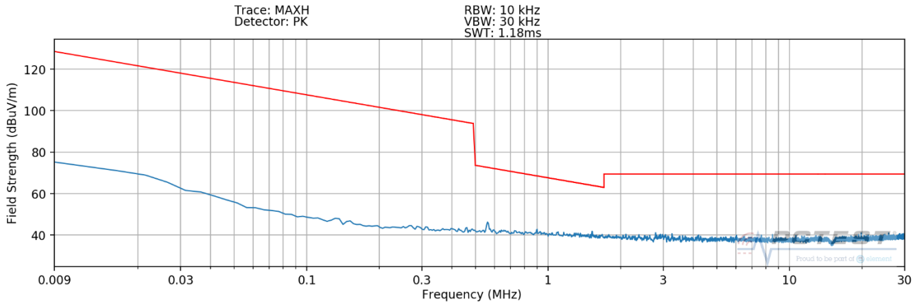
Plot 7-12. Radiated Spurious Plot 9kHz – 30MHz (Pol. Z – Device to S-Pen)
