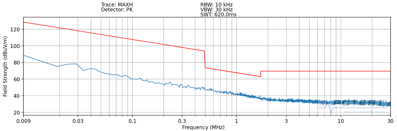
Plot 7-14. Radiated Spurious Plot 9kHz – 30MHz (Pol. Y – WPT – Digitizer Hover)
