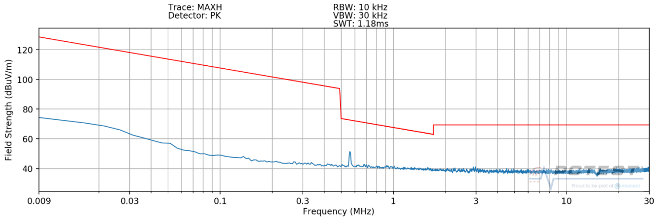
Plot 7-10. Radiated Spurious Plot 9kHz – 30MHz (Pol. X – Device to S-Pen)
