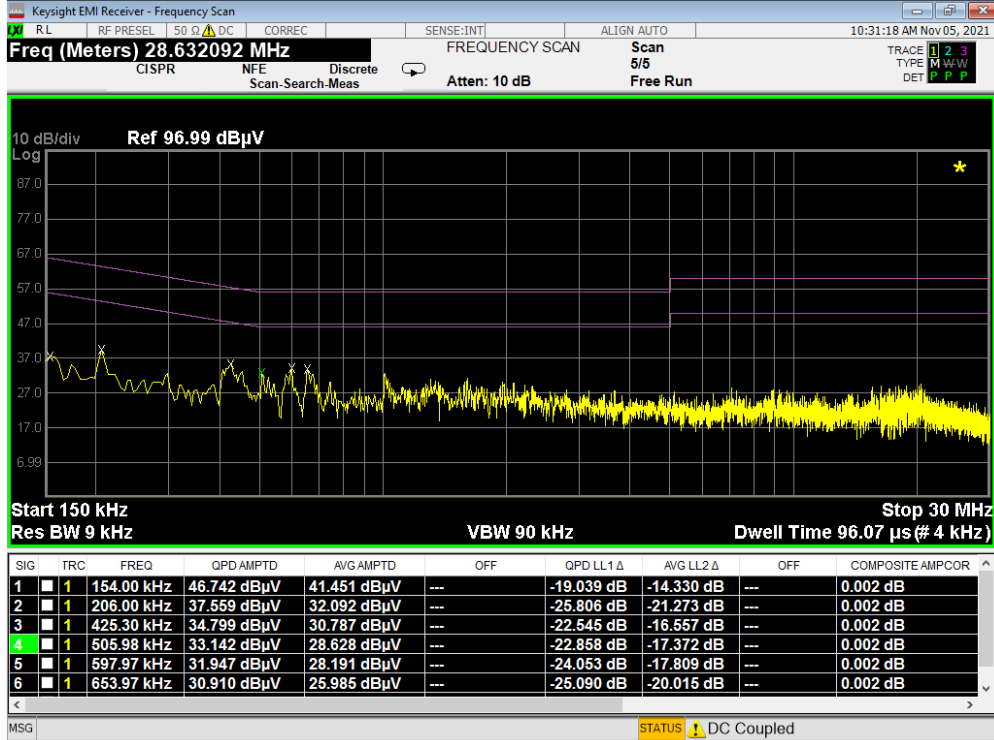
Plot 7-19. Line-Conducted Test Plot (L1) - Device to Device – Config 1
