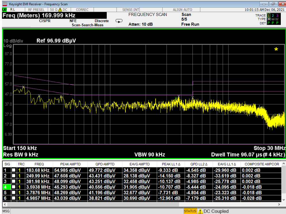
Plot 7-24. Line-Conducted Test Plot (N) - Device to Device – Config 3
