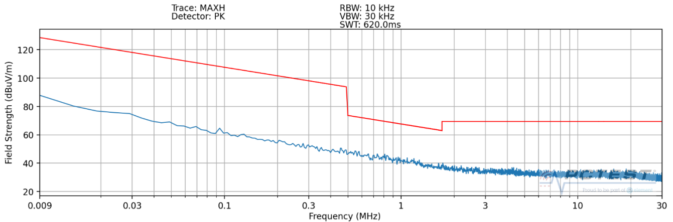
Plot 7-15. Radiated Spurious Plot 9kHz – 30MHz (Pol. Z – WPT – Digitizer Hover)
