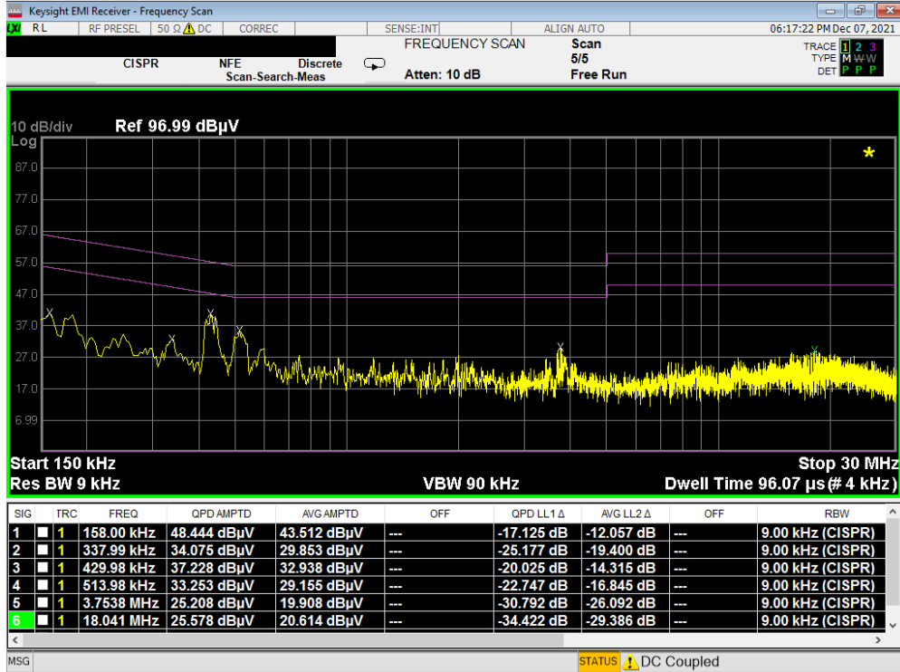
Plot 7-25. Line-Conducted Test Plot (L1) - Device to S-Pen
