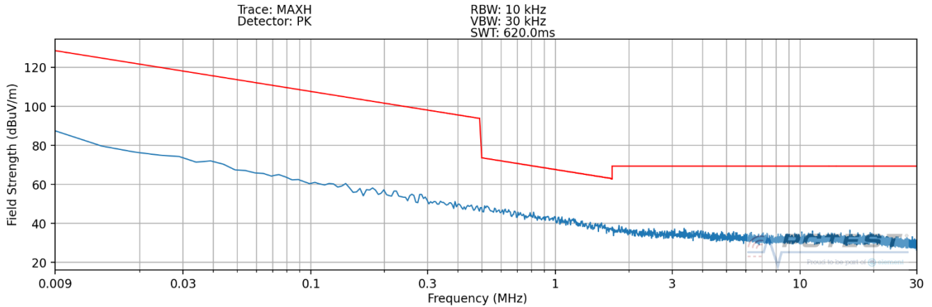
Plot 7-16. Radiated Spurious Plot 9kHz – 30MHz (Pol. X – WPT – Digitizer Click)
