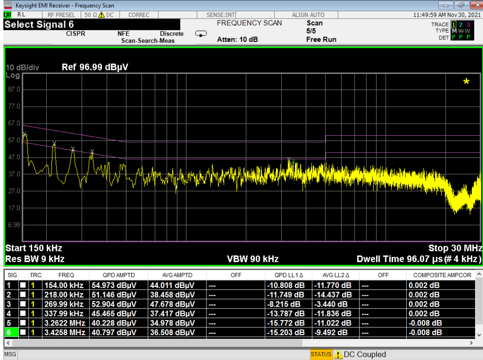
Plot 7-21. Line-Conducted Test Plot (L1) - Device to Device – Config 2
