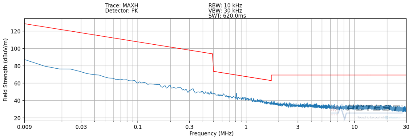
Plot 7-18. Radiated Spurious Plot 9kHz – 30MHz (Pol. Z – WPT – Digitizer Click)
