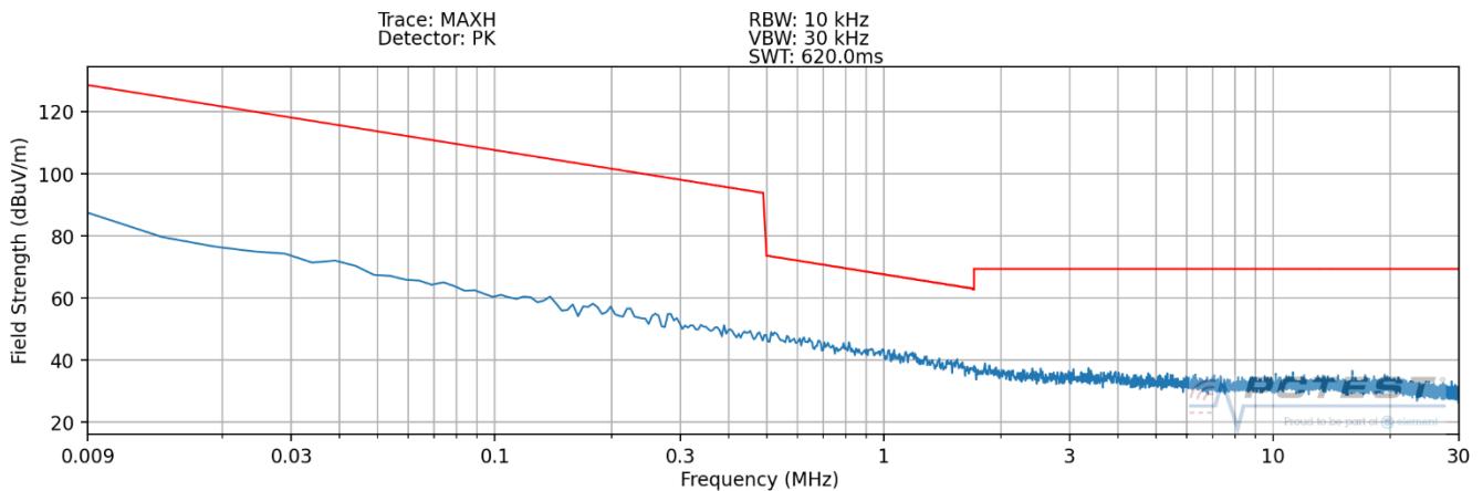
Plot 7-17. Radiated Spurious Plot 9kHz – 30MHz (Pol. Y – WPT – Digitizer Click)
