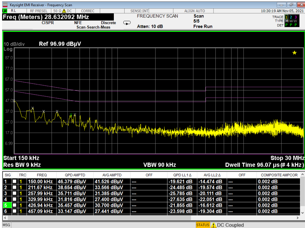
Plot 7-20. Line-Conducted Test Plot (N) - Device to Device – Config 1
