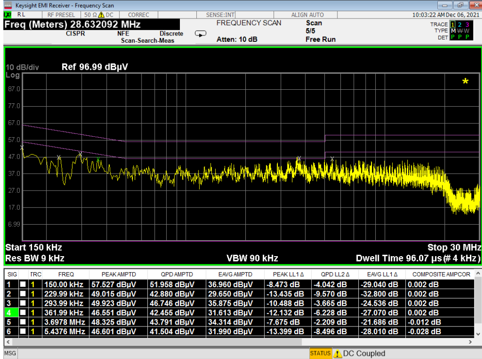
Plot 7-23. Line-Conducted Test Plot (L1) - Device to Device – Config 3
