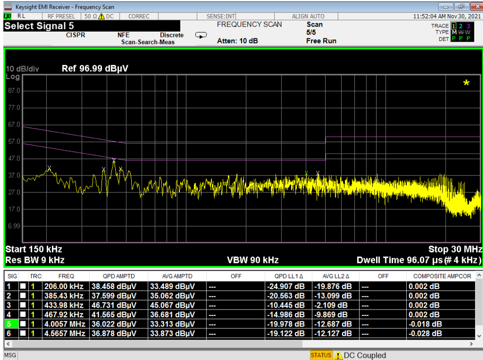
Plot 7-22. Line-Conducted Test Plot (N) - Device to Device – Config 2
