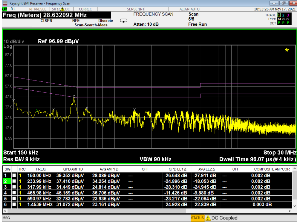
Plot 7-27. Line-Conducted Test Plot (L1) – Digitizer - Hover
