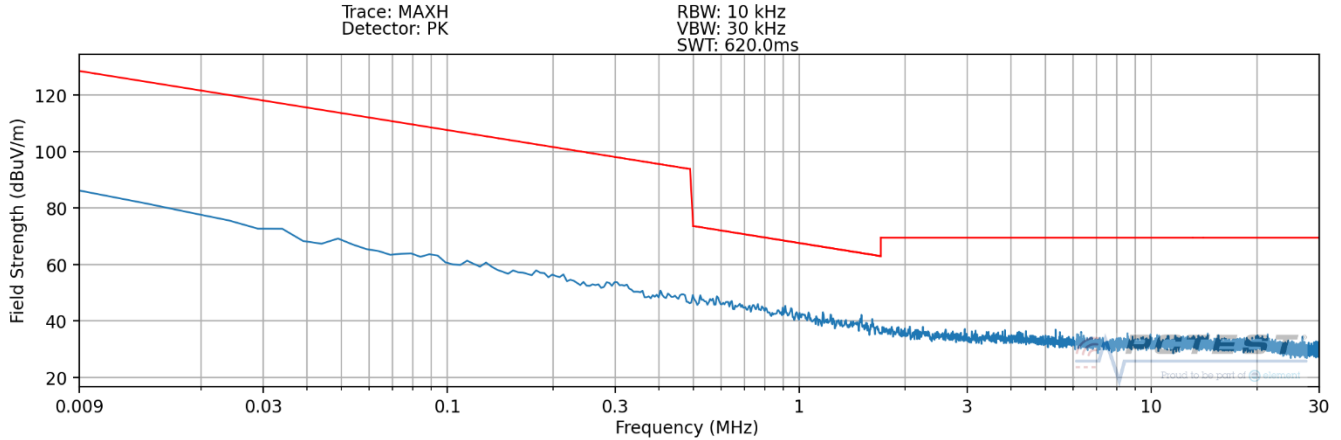
Plot 7-13. Radiated Spurious Plot 9kHz – 30MHz (Pol. X – WPT – Digitizer Hover)
