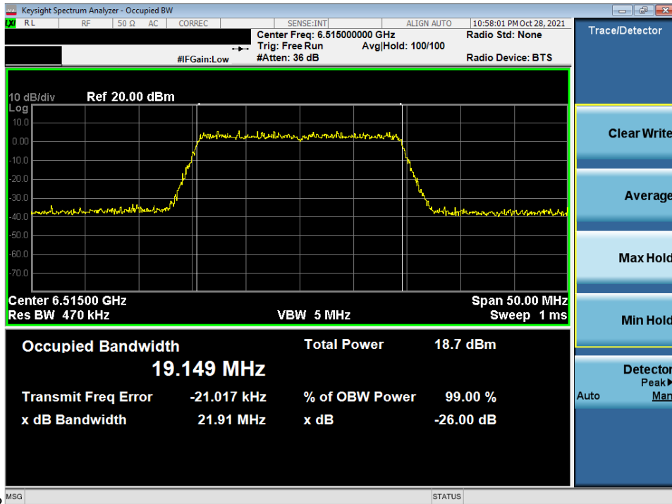
2 Plot 7-21. 26dB Bandwidth Plot MIMO ANT1 (20MHz 802.11ax (UNII Band 6) – Ch. 113)
