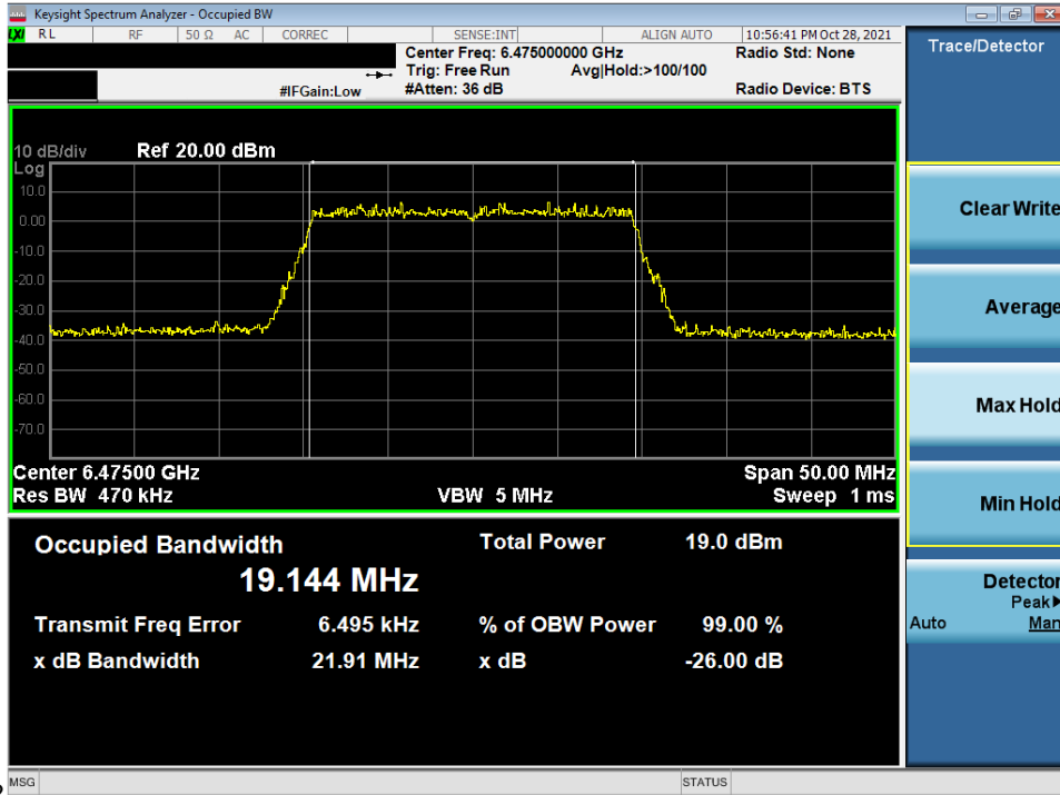
2 Plot 7-20. 26dB Bandwidth Plot MIMO ANT1 (20MHz 802.11ax (UNII Band 6) – Ch. 105)
