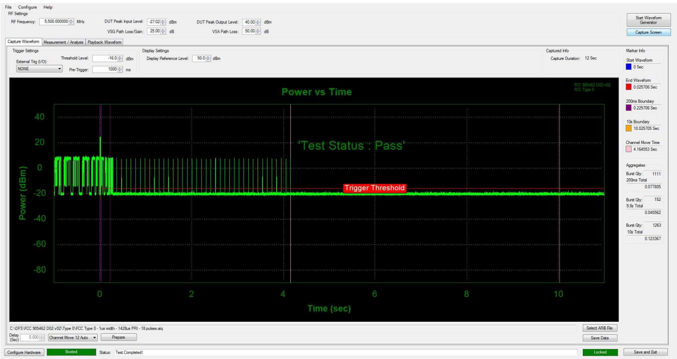
Figure 9-7. 5500MHz - Channel Move/ Closing Transmission Time - (20 MHz)
