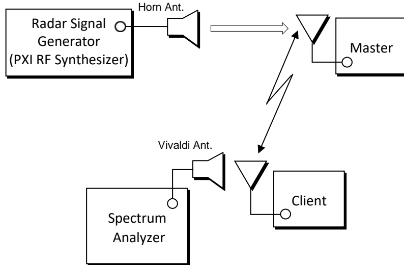
Figure 8-1. Radiated DFS Test Setup
