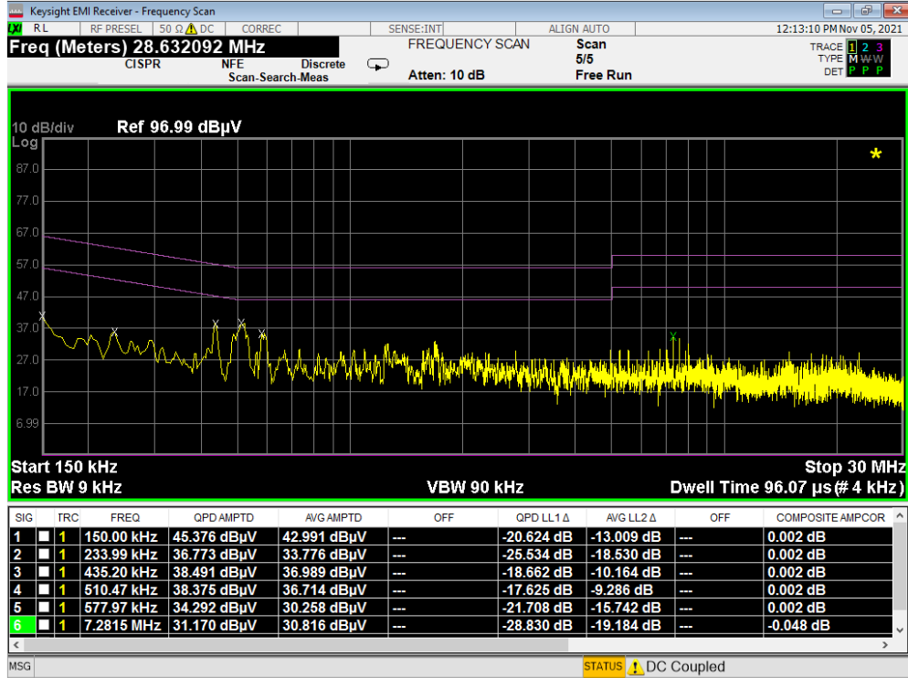
Plot 7-422. Line Conducted Plot with 802.11a UNII Band 3 (L1) – WCP
