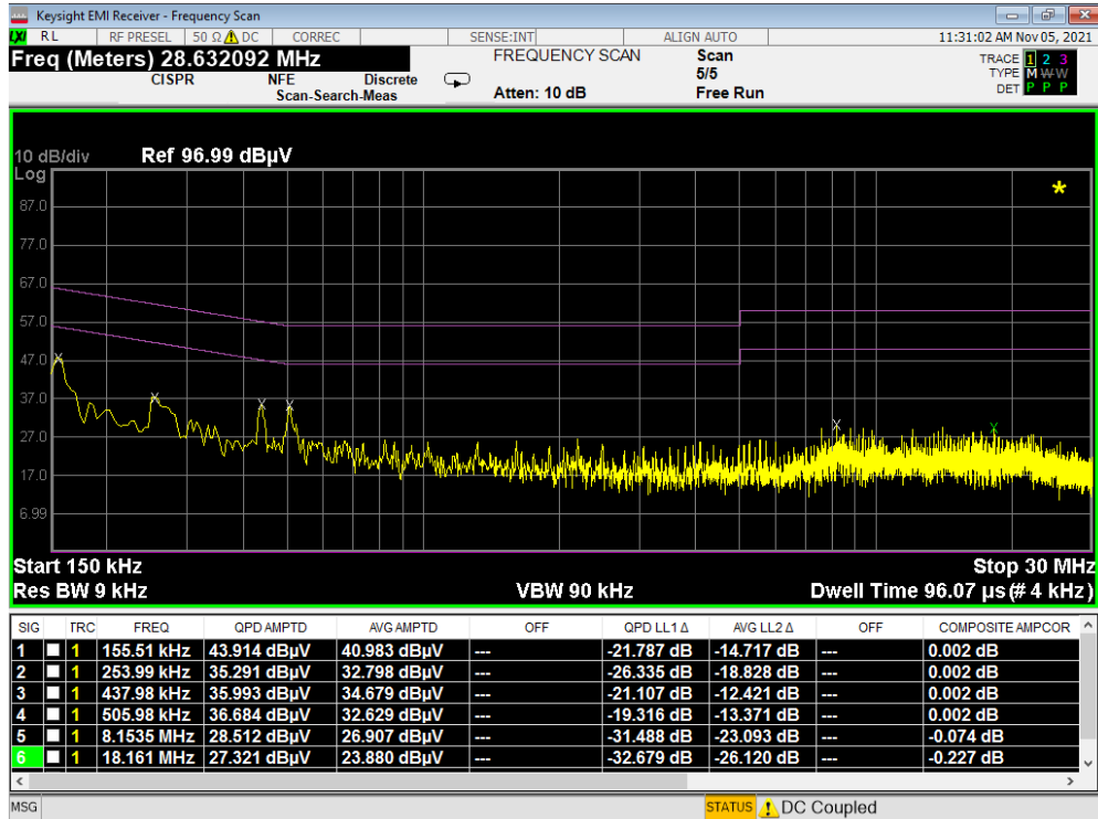
Plot 7-423. Line Conducted Plot with 802.11a UNII Band 3 (N) – WCP
