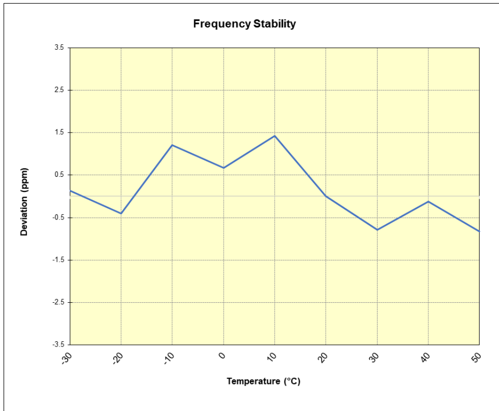
Plot 7-17. GSM/GPRS PCS Frequency Stability Chart
