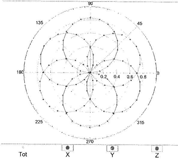
f=600 MHz,TEM
