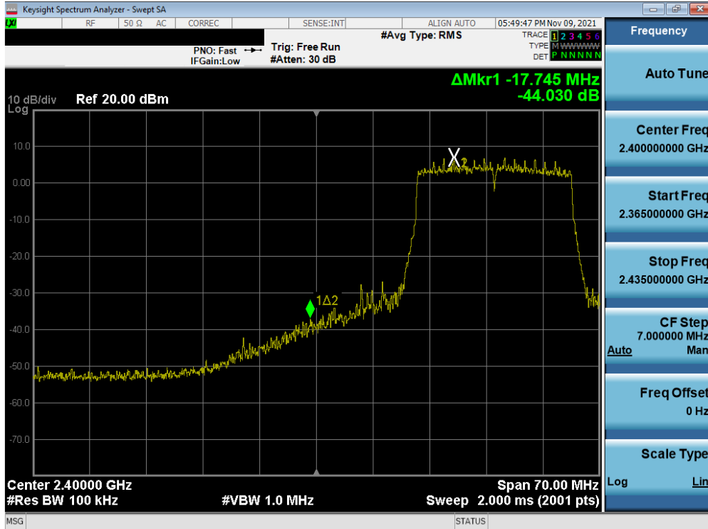
Plot 7-31. Band Edge Plot MIMO ANT1 (802.11ax OFDMA – 242 Tones – Ch. 3)
