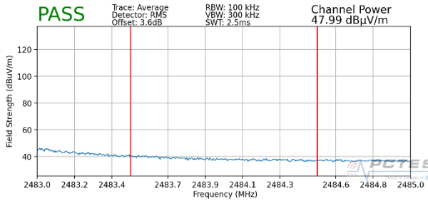
Plot 7-99. Radiated Restricted Upper Band Edge Measurement MIMO (Average – 242 Tones)
