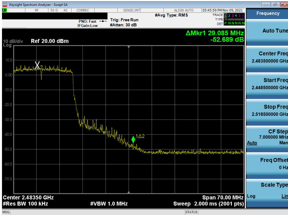
Plot 7-32. Band Edge Plot MIMO ANT1 (802.11ax OFDMA – 242 Tones – Ch. 10)
