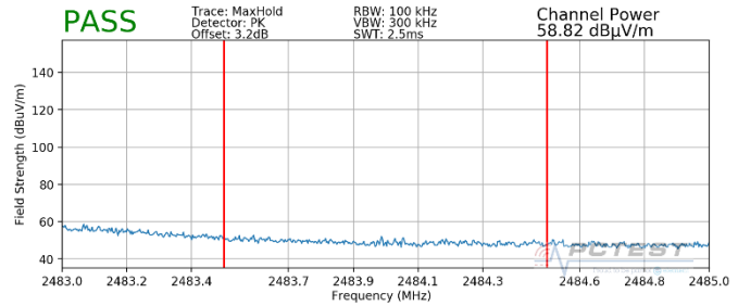
Plot 7-100. Radiated Restricted Upper Band Edge Measurement MIMO (Peak – 242 Tones)
