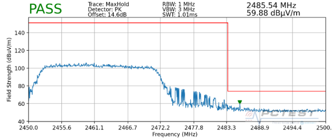
Plot 7-96. Radiated Restricted Upper Band Edge Measurement MIMO (Peak – 242 Tones)
