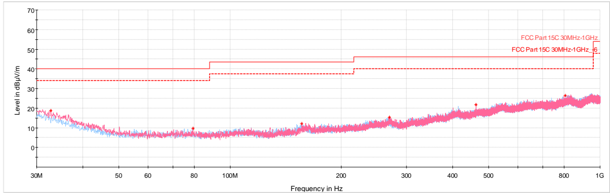
Plot 7-165. Radiated Spurious Emissions Below 1GHz (Antenna 2)
