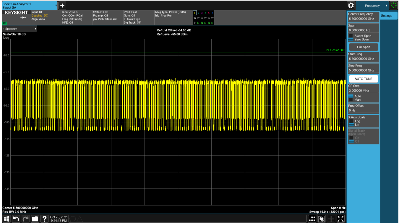
Figure 9-1. 5500MHz - Channel Loading - (20MHz)
