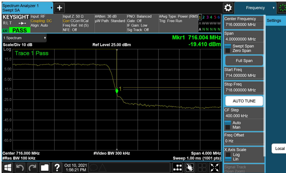
Plot 7-63. Upper Band Edge Plot (LTE Band 12 - 3MHz QPSK – Full RB)
