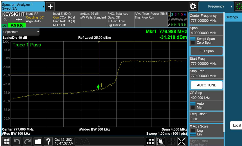
Plot 7-66. Lower Band Edge Plot (LTE Band 13 - 10MHz QPSK – Full RB)
