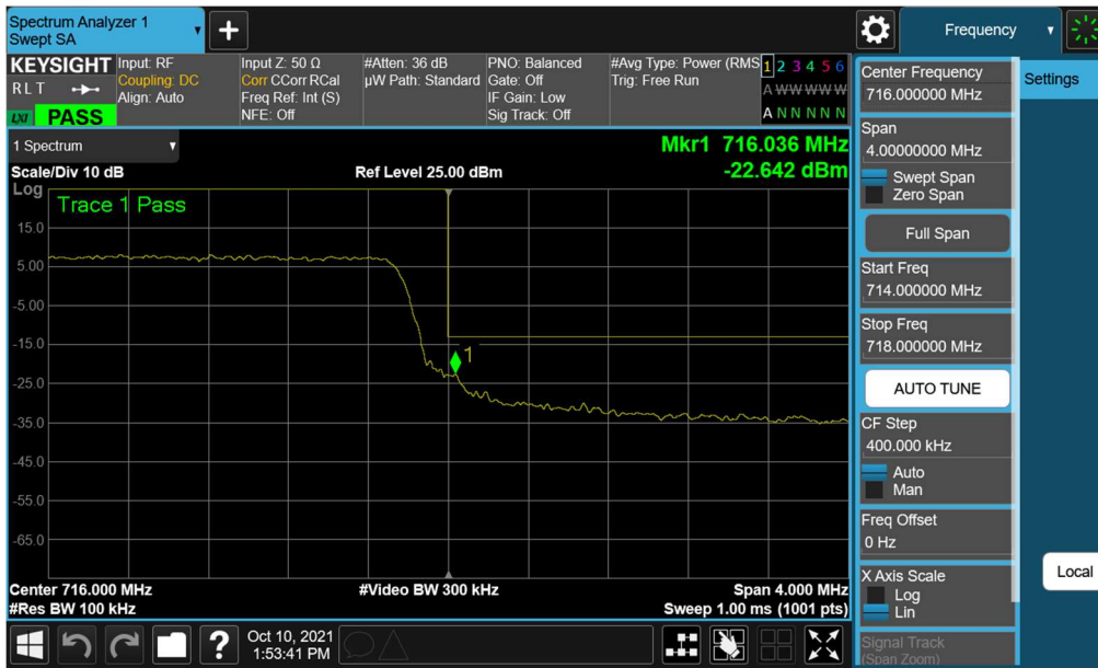
Plot 7-61. Upper Band Edge Plot (LTE Band 12/17 - 5MHz QPSK – Full RB)
