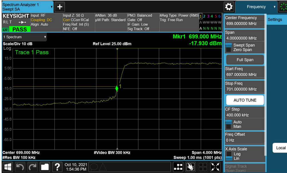
Plot 7-62. Lower Band Edge Plot (LTE Band 12 - 3MHz QPSK – Full RB)
