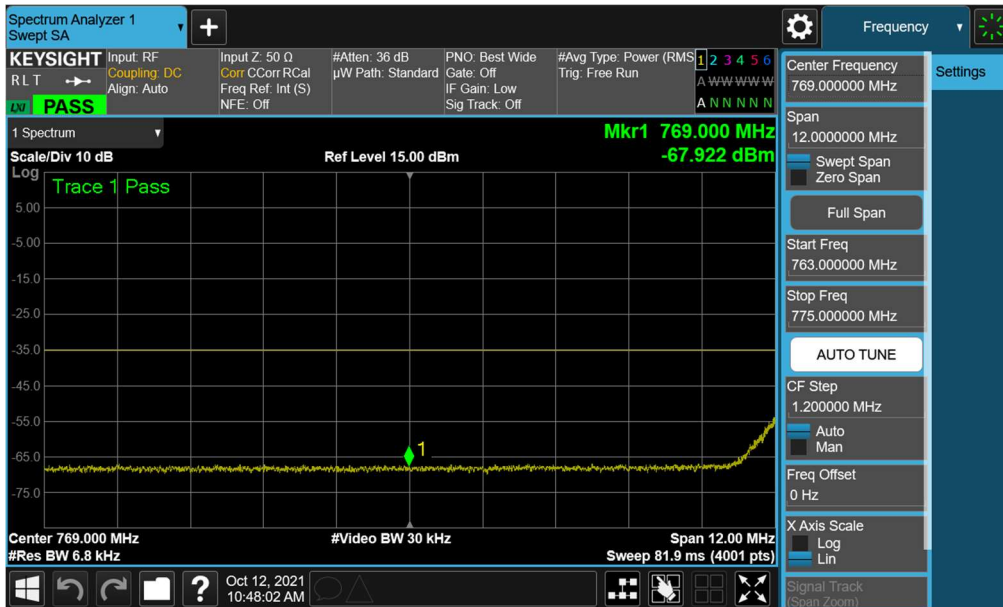
Plot 7-67. Lower Emission Mask Plot (LTE Band 13 - 10MHz QPSK – Full RB)
