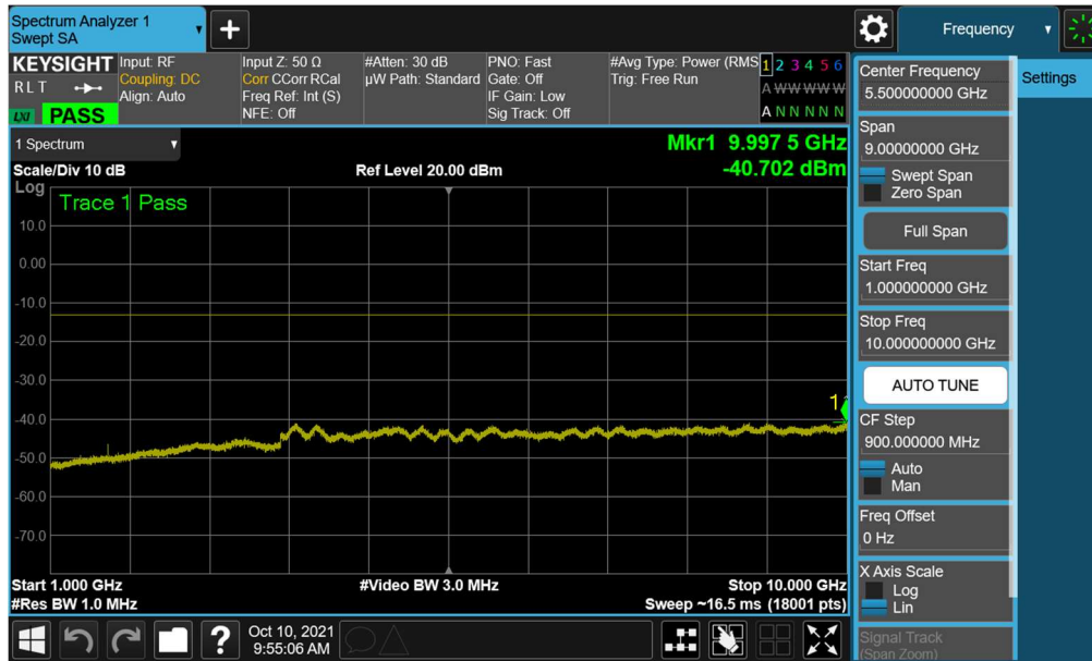
Plot 7-16. Conducted Spurious Plot (LTE Band 26/5 - 10MHz QPSK - 1 RB - Low Channel)
