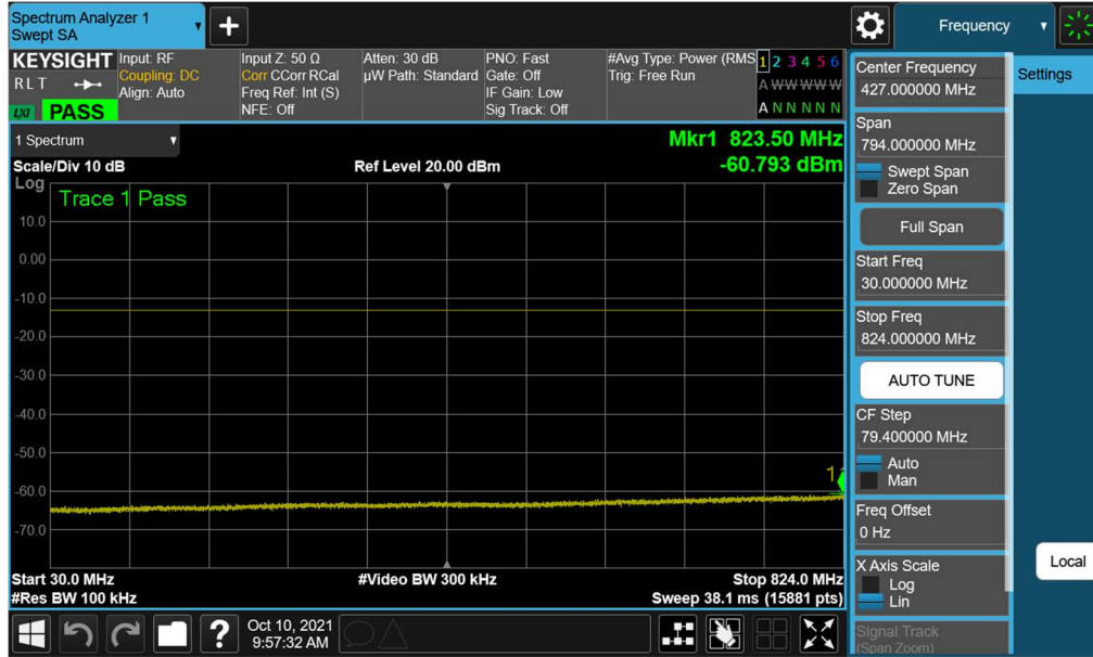
Plot 7-20. Conducted Spurious Plot (LTE Band 26/5 - 10MHz QPSK - 1 RB - High Channel)
