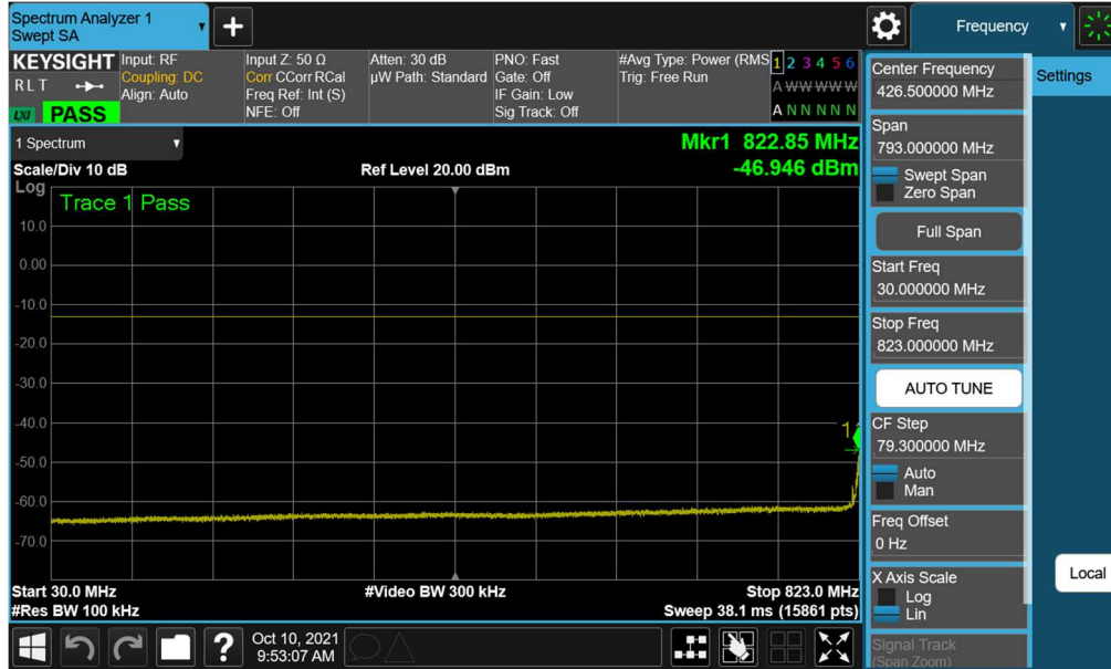
Plot 7-14. Conducted Spurious Plot (LTE Band 26/5 - 10MHz QPSK - 1 RB - Low Channel)
