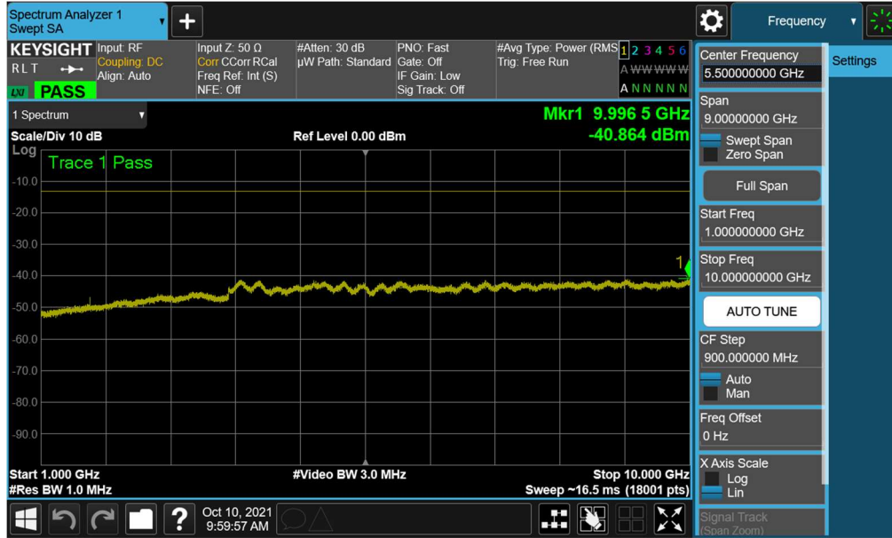
Plot 7-22. Conducted Spurious Plot (LTE Band 26/5 - 10MHz QPSK - 1 RB - High Channel)
