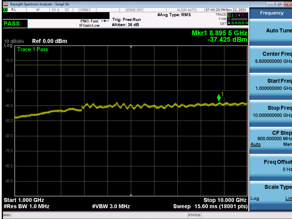
Plot 7-24. Conducted Spurious Plot (NR Band n5 - 20.0MHz - 1 RB - High Channel)
