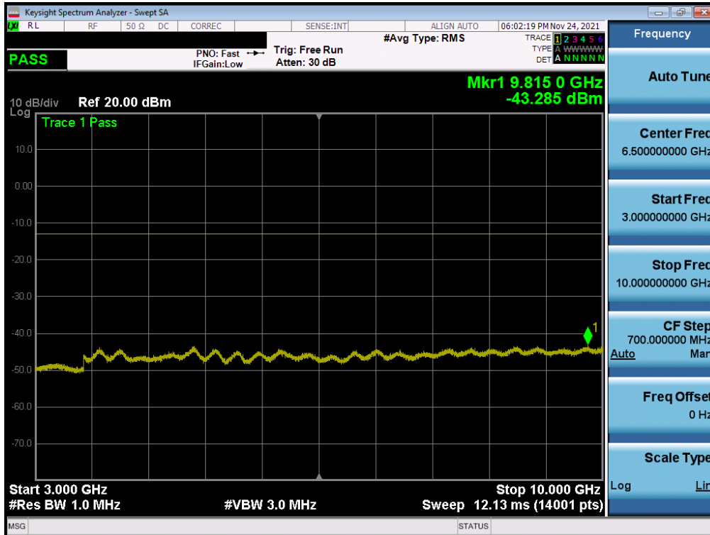
Plot 7-14. Conducted Spurious Plot (LTE ULCA Band 5 - Band 66 - 1 RB - Mid Channel)
