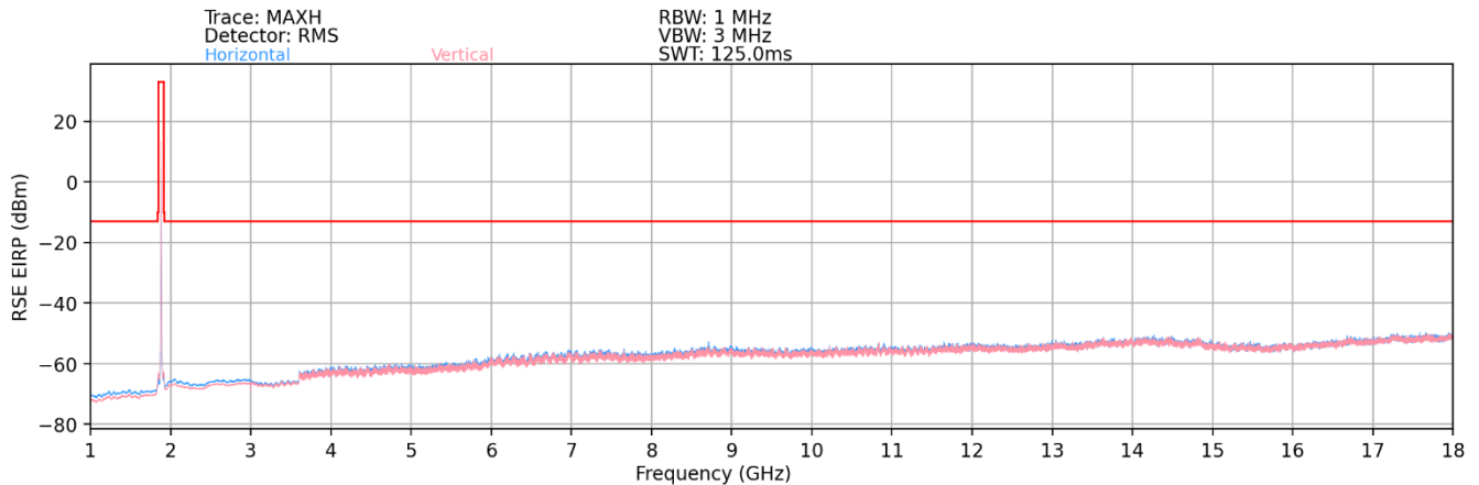
Plot 7-35. Radiated Spurious Plot (NR Band n5 + Band 2)
