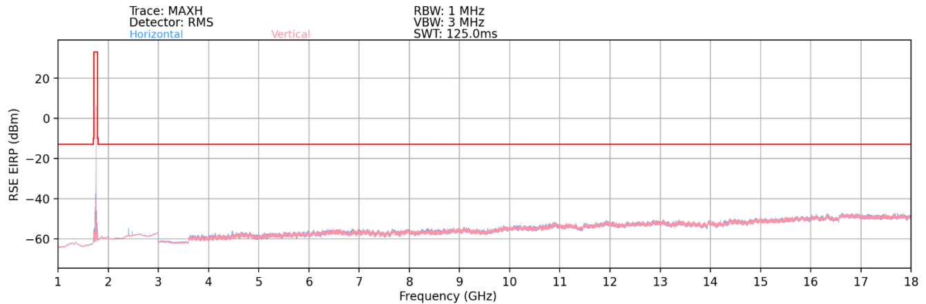
Plot 7-33. Radiated Spurious Plot (LTE ULCA Band 5 - Band 66)
