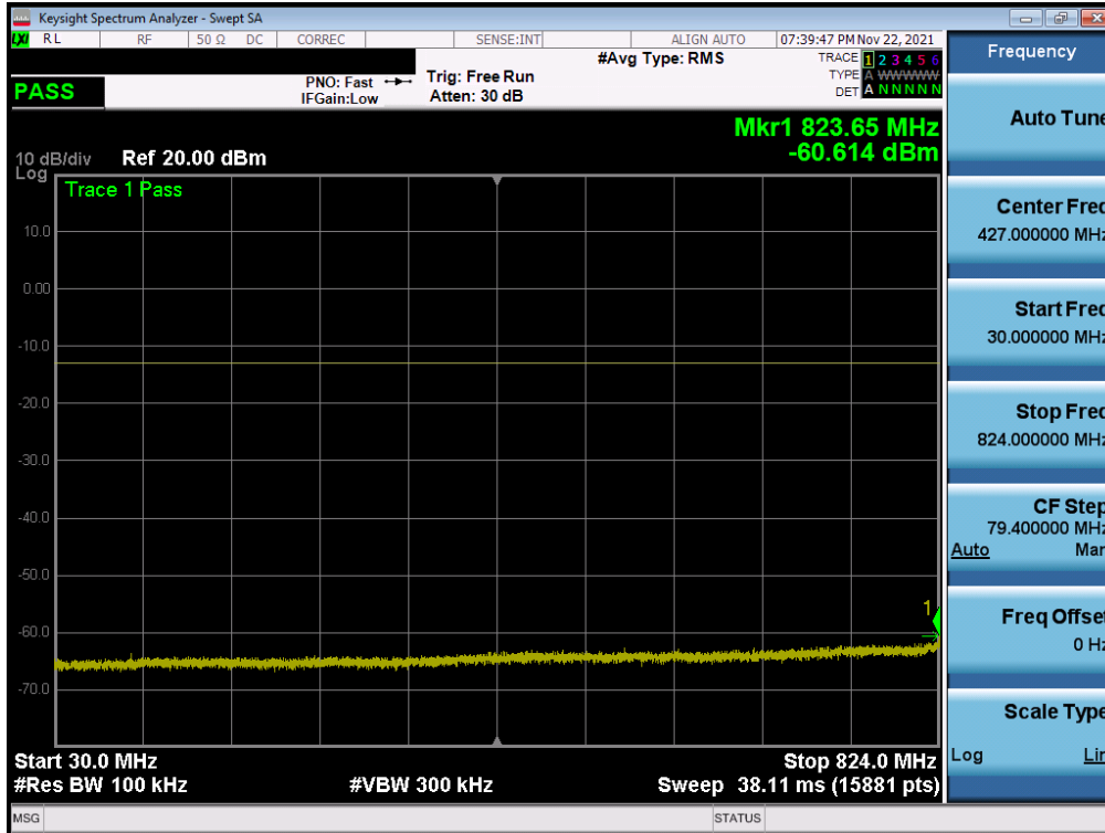
Plot 7-22. Conducted Spurious Plot (NR Band n5 - 20.0MHz - 1 RB - High Channel)
