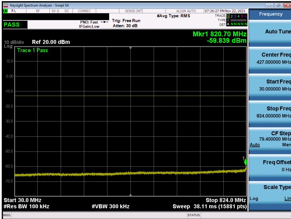
Plot 7-19. Conducted Spurious Plot (NR Band n5 - 20.0MHz - 1 RB - Mid Channel)
