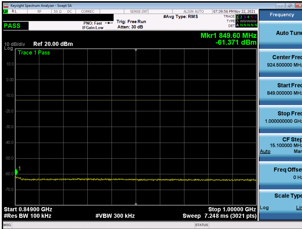
Plot 7-23. Conducted Spurious Plot (NR Band n5 - 20.0MHz - 1 RB - High Channel)
