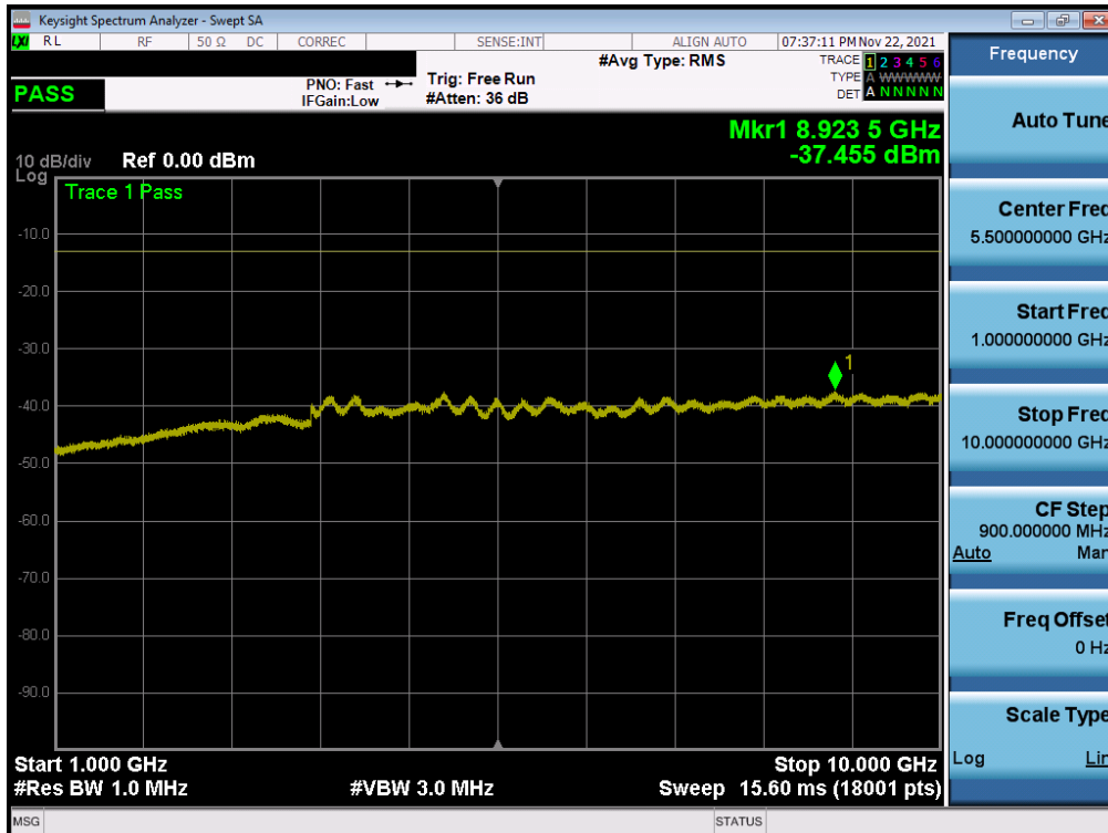
Plot 7-21. Conducted Spurious Plot (NR Band n5 - 20.0MHz - 1 RB - Mid Channel)
