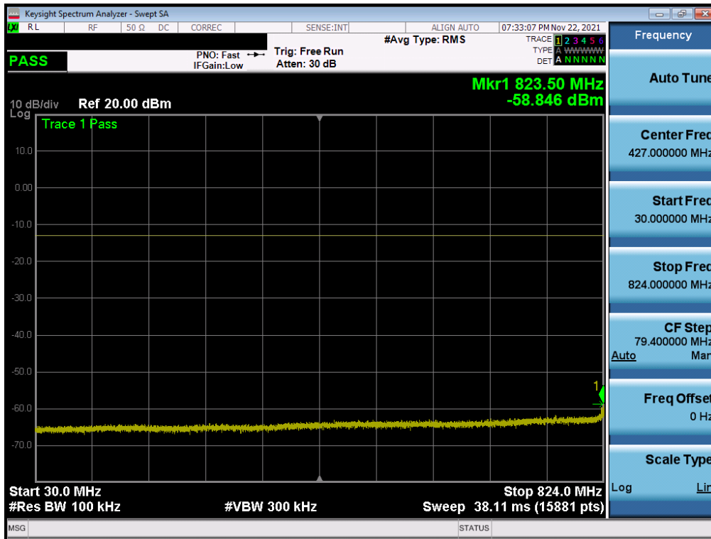
Plot 7-16. Conducted Spurious Plot (NR Band n5 - 20.0MHz - 1 RB - Low Channel)
