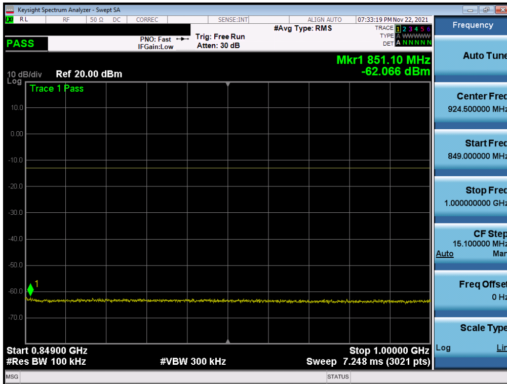
Plot 7-17. Conducted Spurious Plot (NR Band n5 - 20.0MHz - 1 RB - Low Channel)
