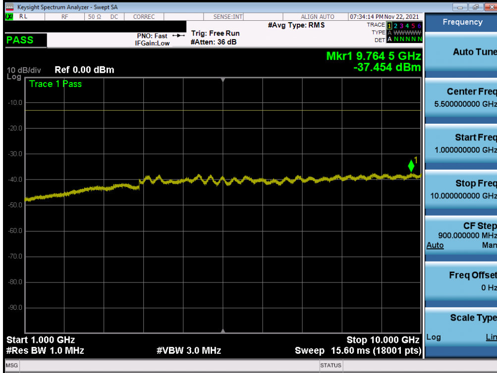
Plot 7-18. Conducted Spurious Plot (NR Band n5 - 20.0MHz - 1 RB - Low Channel)
