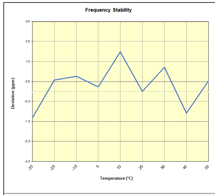
Plot 7-36. NR Band n5 Frequency Stability Chart
