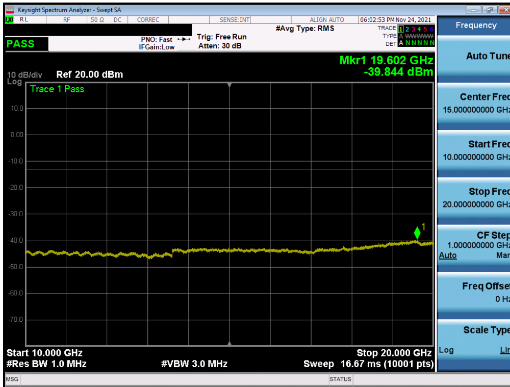
Plot 7-15. Conducted Spurious Plot (LTE ULCA Band 5 - Band 66 - 1 RB - Mid Channel)
