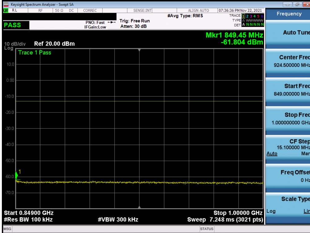
Plot 7-20. Conducted Spurious Plot (NR Band n5 - 20.0MHz - 1 RB - Mid Channel)
