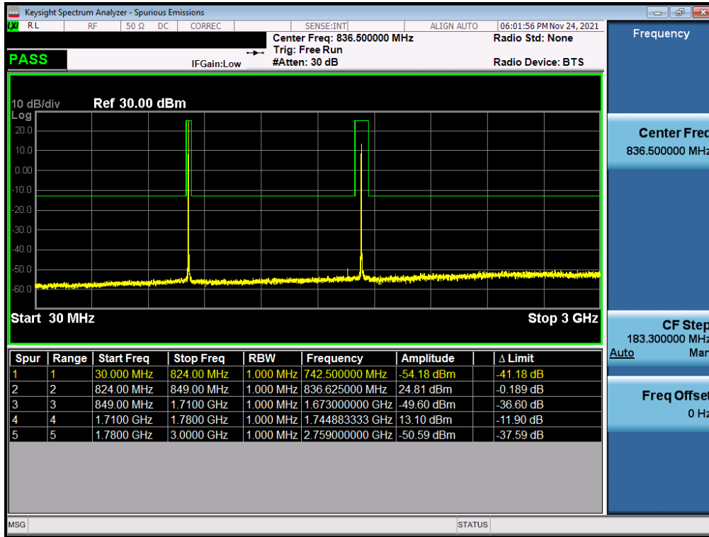
Plot 7-13. Conducted Spurious Plot (LTE ULCA Band 5 - Band 66 - 1 RB - Mid Channel)
