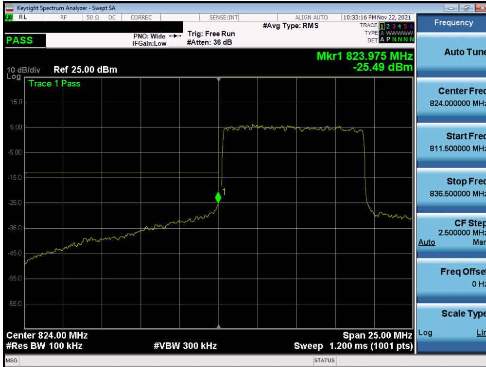
Plot 7-29. Lower Band Edge Plot (NR Band n5 – 10.0MHz - Full RB)
