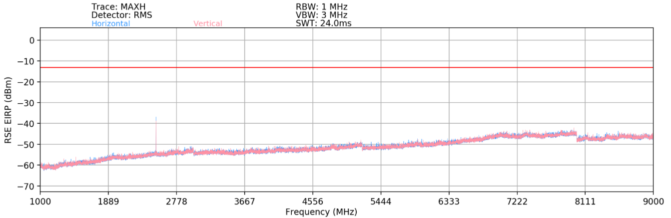
Plot 7-34. Radiated Spurious Plot (NR Band n5)
