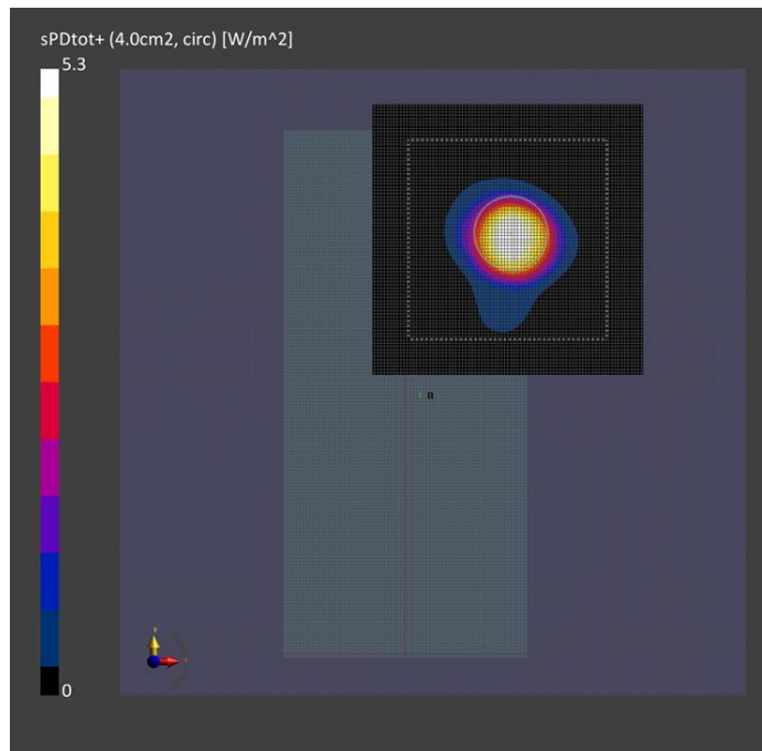
Figure 10-1 4cm 2 psPD distribution measured at input.power.limit of 10.9 dBm on the back side for n261 beam 2
