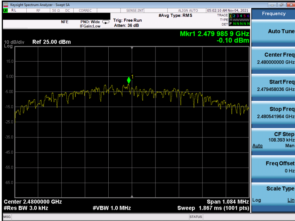
Plot 7-93. Power Spectral Density Plot (Bluetooth (LE), 1Mbps, ePA – Ch. 39) Antenna 2
