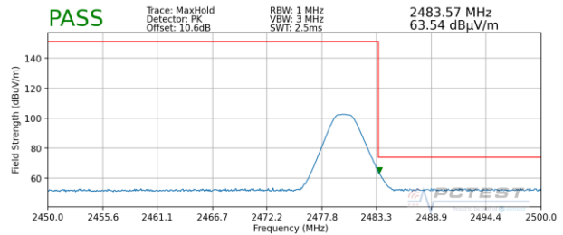
Plot 7-142. Radiated Restricted Upper Band Edge Measurement (Peak) – Dual
