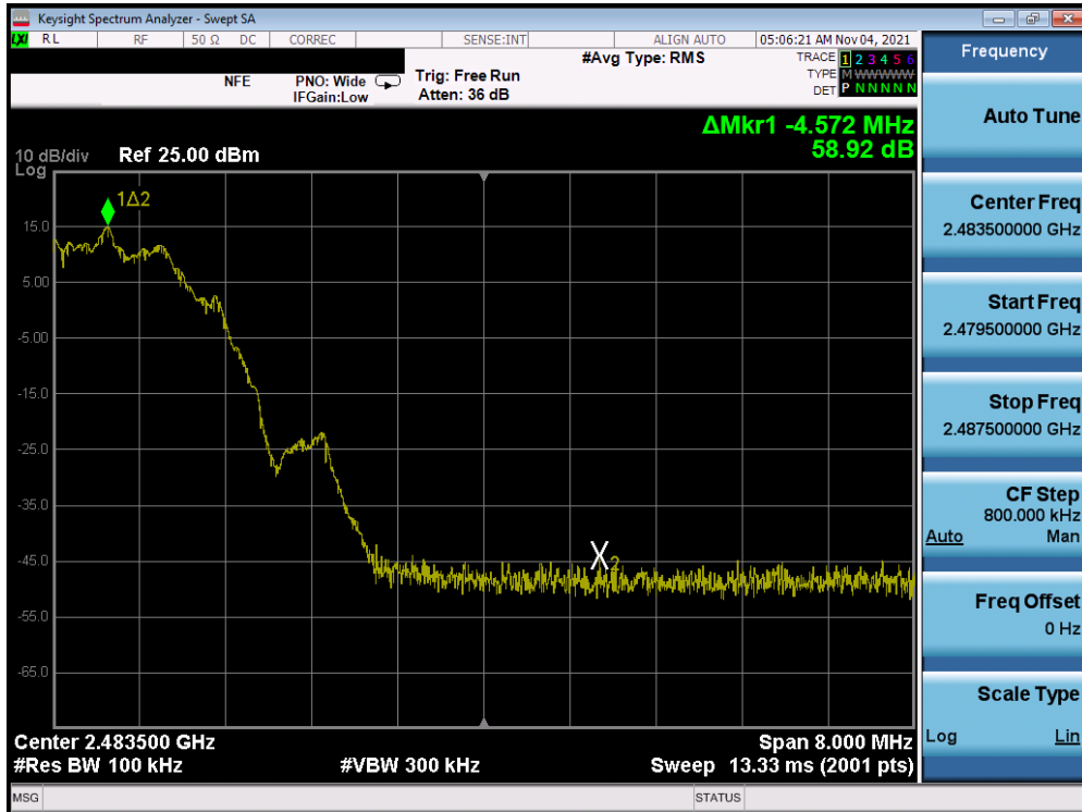
Plot 7-124. Band Edge Plot (Bluetooth (LE), 2Mbps, – Ch. 39) Antenna 2
