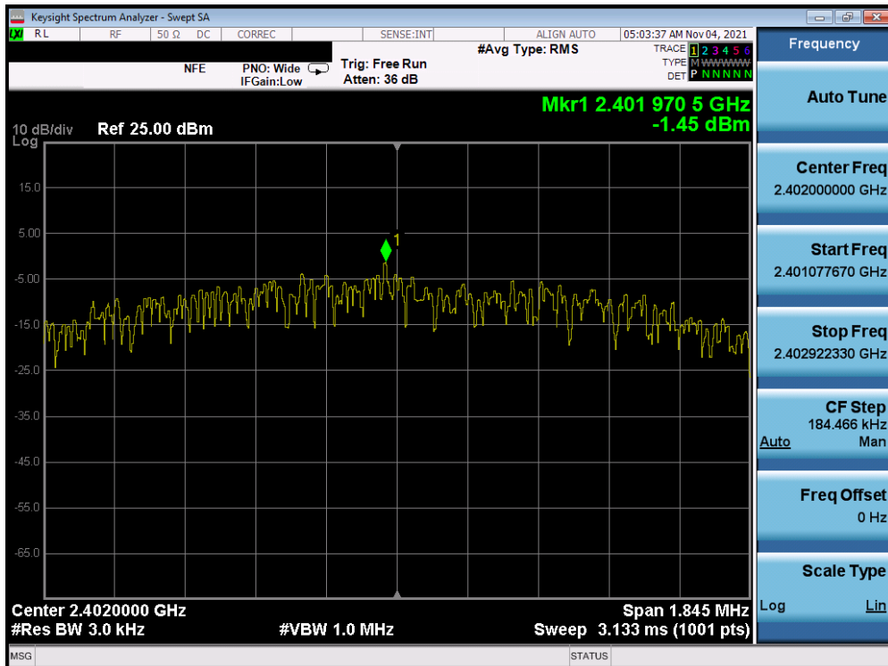
Plot 7-94. Power Spectral Density Plot (Bluetooth (LE), 2Mbps, ePA – Ch. 0) Antenna 2
