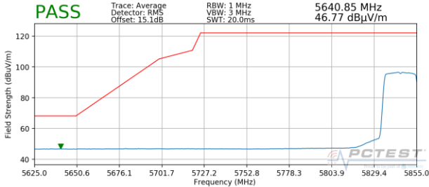
Plot 7-375. Radiated Lower Band Edge Plot MIMO (Average - UNII Band 4)
