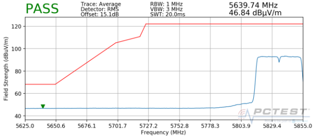
Plot 7-384. Radiated Lower Band Edge Plot MIMO (Average - UNII Band 4)
