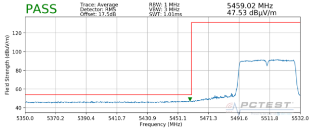
Plot 7-381. Radiated Lower Band Edge Plot MIMO (Average – UNII Band 2C)
