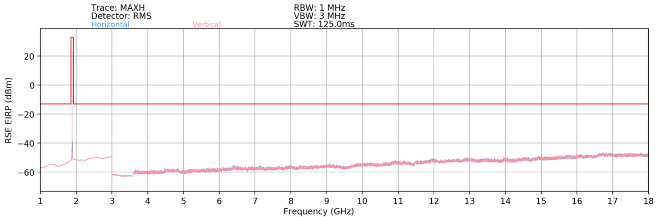
Plot 7-59. Radiated Spurious Plot (NR Band n25/2 –1-18GHz)
