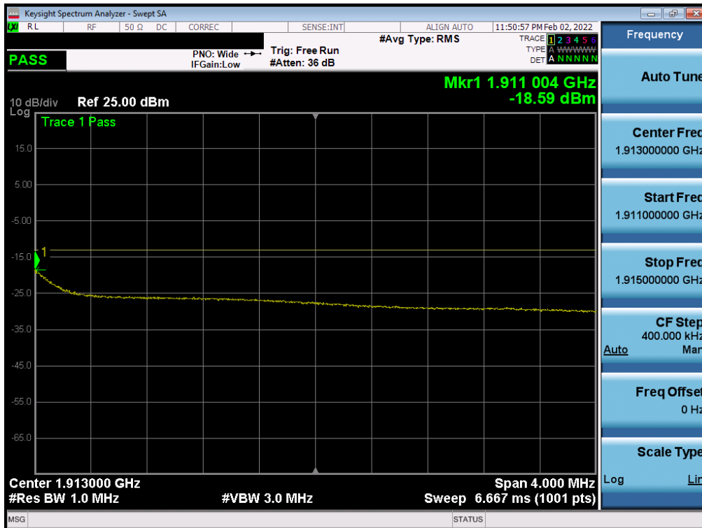
Plot 7-37. Extended Upper Band Edge Plot (NR Band n2 - 10MHz QPSK – Full RB)
