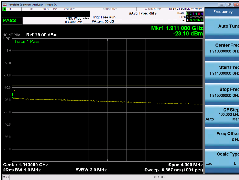
Plot 7-25. Extended Upper Band Edge Plot (NR Band n2 - 20MHz QPSK – Full RB)
