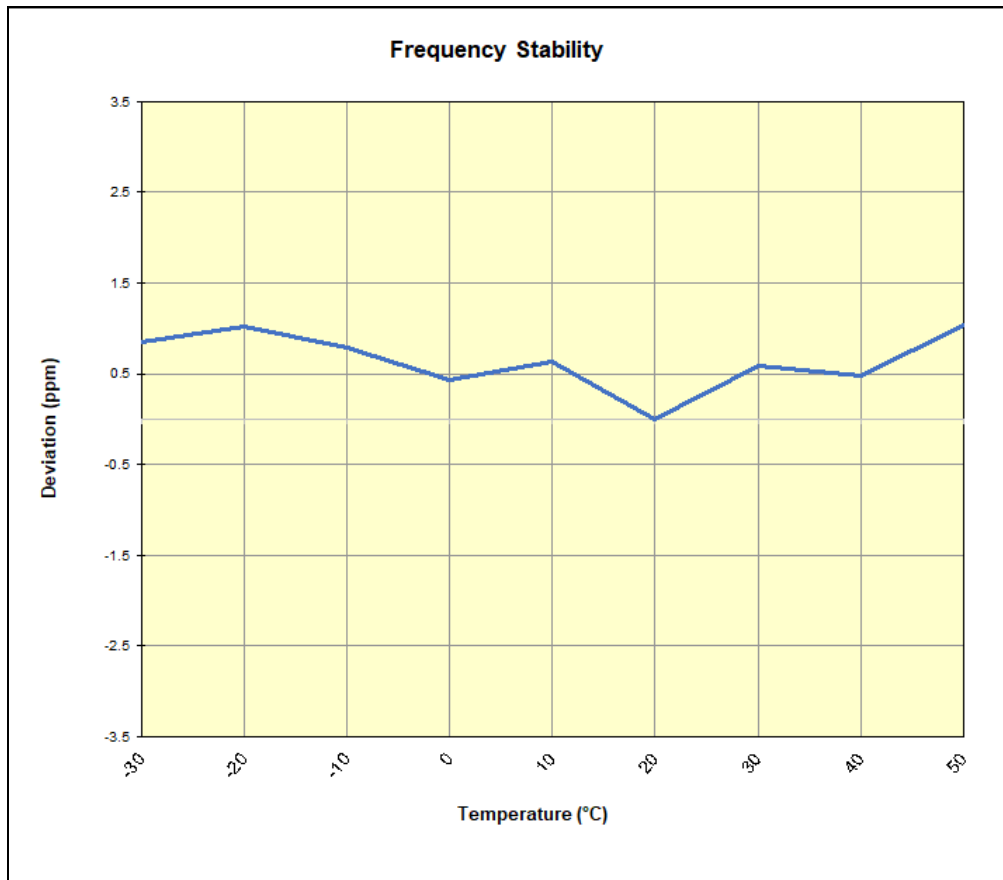
Plot 7-62. NR Band n25/2 Frequency Stability Chart
