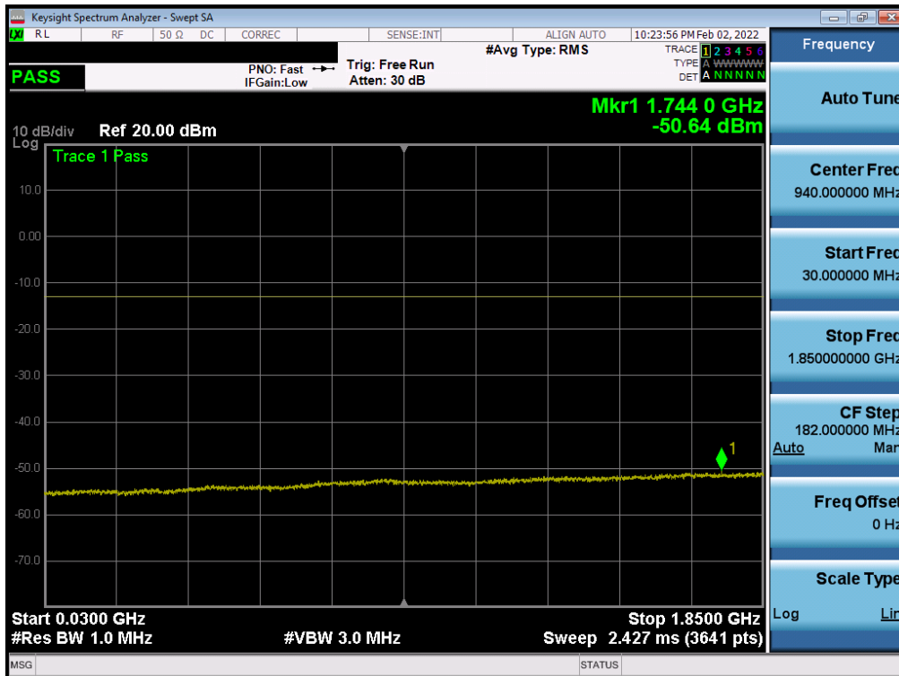
Plot 7-16. Conducted Spurious Plot (NR Band n25/2 - 20.0MHz - 1RB - Mid Channel)
