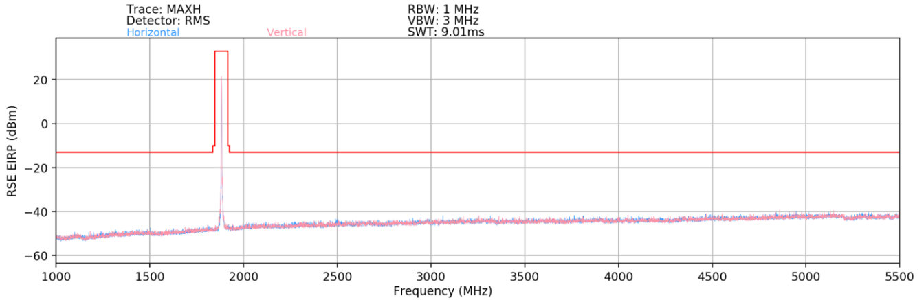
Plot 7-60. Radiated Spurious Plot (EN-DC: n25/2 – Band 12 – 1-5.5GHz)
