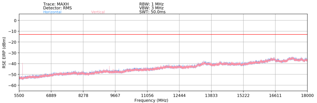
Plot 7-61. Radiated Spurious Plot (EN-DC: n25/2 – Band 12 – 5.5-18GHz)
