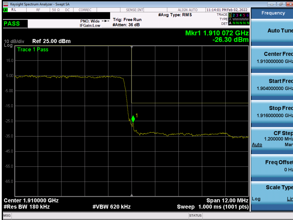
Plot 7-30. Upper Band Edge Plot (NR Band n2 - 15MHz QPSK – Full RB)
