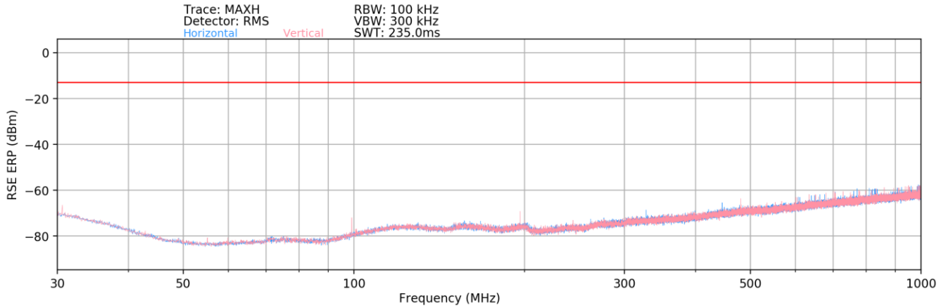
Plot 7-58. Radiated Spurious Plot (NR Band n25/2 – 30MHz-1GHz)
