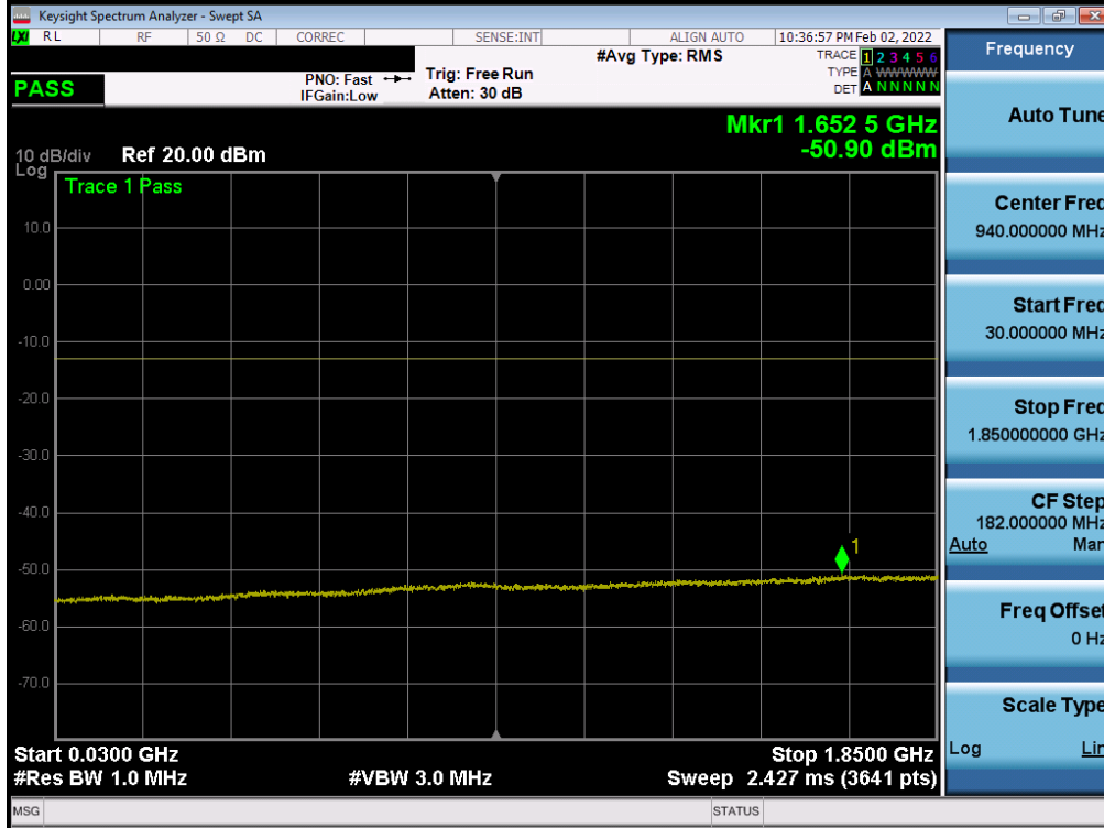
Plot 7-19. Conducted Spurious Plot (NR Band n25/2 - 20.0MHz - 1RB - High Channel)
