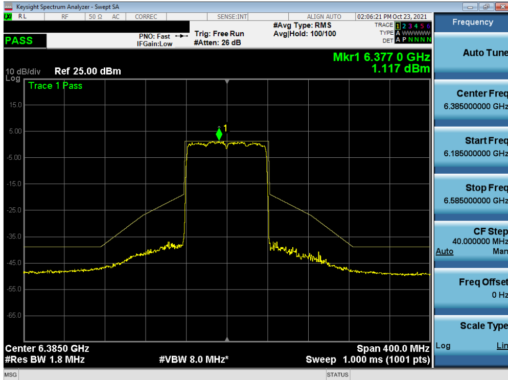
Plot 7-362. In-Band Emission Plot MIMO ANT1 (80MHz BW 802.11ax (Full Tones) (UNII Band 5) – Ch. 87)
