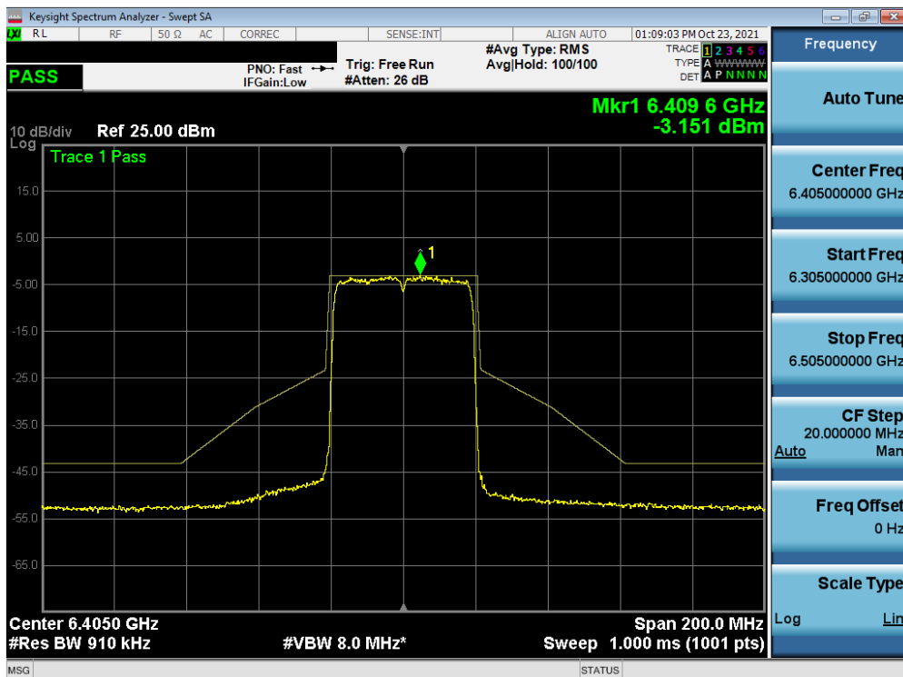
Plot 7-359. In-Band Emission Plot MIMO ANT1 (40MHz BW 802.11ax (Full Tones) (UNII Band 5) – Ch. 91)
