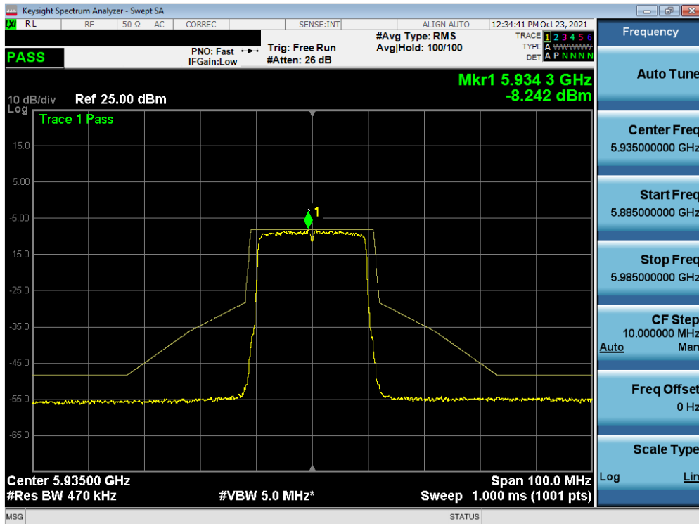
Plot 7-354. In-Band Emission Plot MIMO ANT1 (20MHz BW 802.11ax (Full Tones) UNII Band 5) – Ch. 2)
