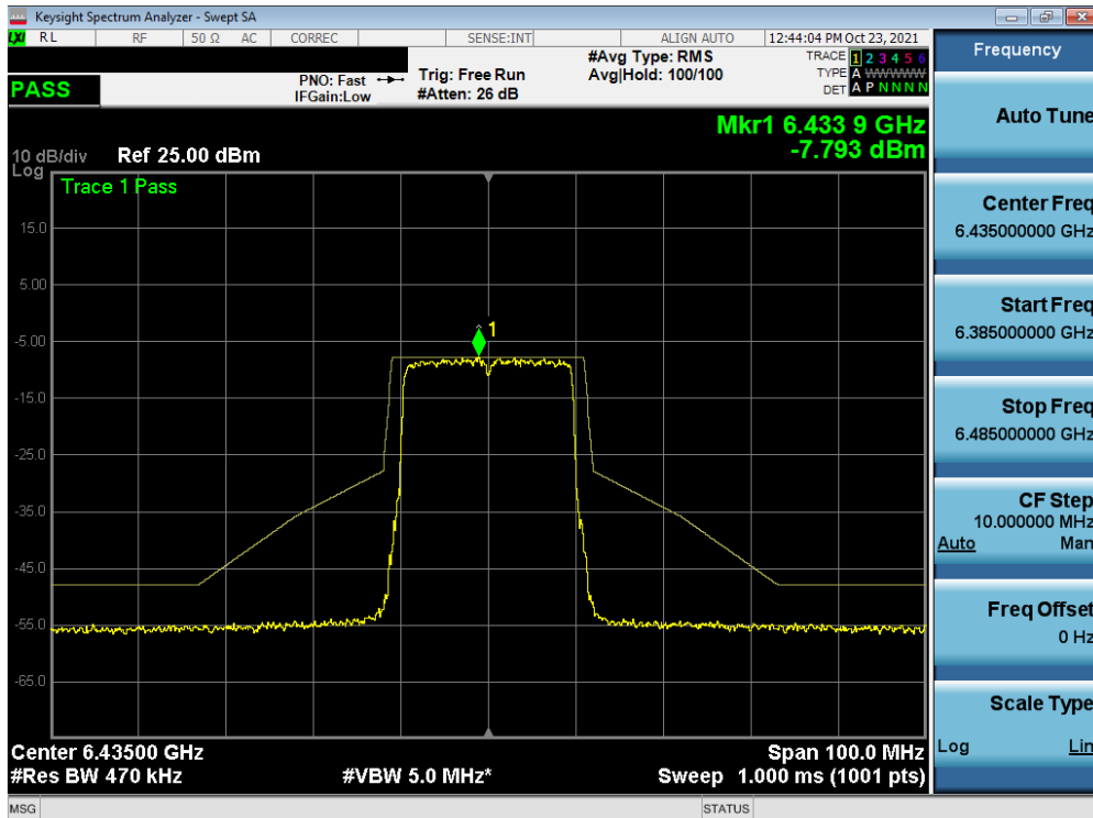
Plot 7-363. In-Band Emission Plot MIMO ANT1 (20MHz BW 802.11ax (Full Tones) (UNII Band 6) – Ch. 97)
