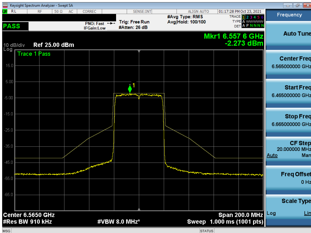
Plot 7-373. In-Band Emission Plot MIMO ANT1 (40MHz BW 802.11ax (Full Tones) (UNII Band 7) – Ch. 123)
