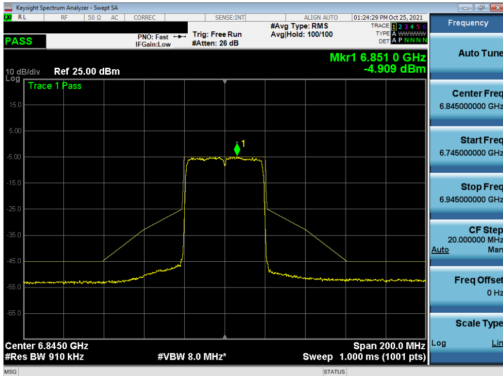
Plot 7-375. In-Band Emission Plot MIMO ANT1 (40MHz BW 802.11ax (Full Tones) (UNII Band 7) – Ch. 179)
