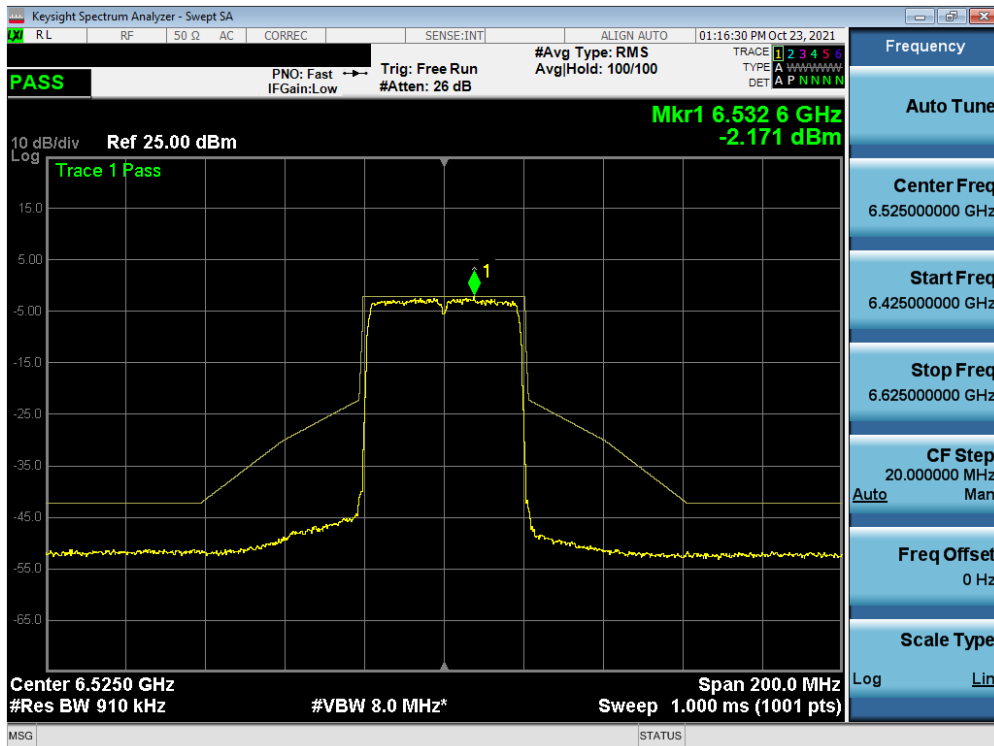
Plot 7-368. In-Band Emission Plot MIMO ANT1 (40MHz BW 802.11ax (Full Tones) (UNII Band 6) – Ch. 115)
