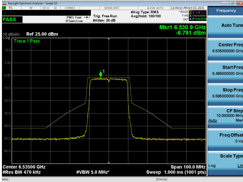
Plot 7-370. In-Band Emission Plot MIMO ANT1 (20MHz BW 802.11ax (Full Tones) (UNII Band 7) – Ch. 117)
