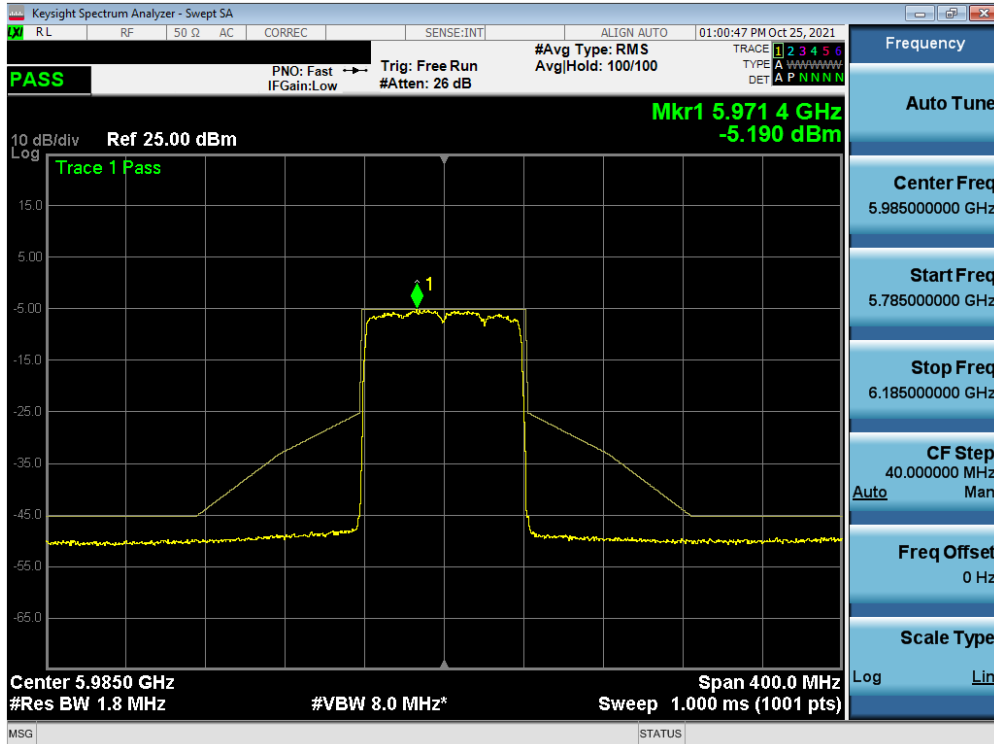
Plot 7-360. In-Band Emission Plot MIMO ANT1 (80MHz BW 802.11ax (Full Tones) (UNII Band 5) – Ch. 7)
