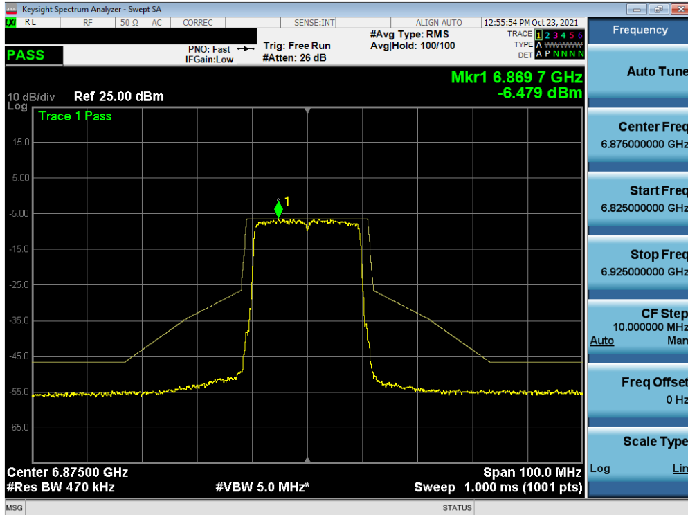
Plot 7-372. In-Band Emission Plot MIMO ANT1 (20MHz BW 802.11ax (Full Tones) (UNII Band 7) – Ch. 185)
