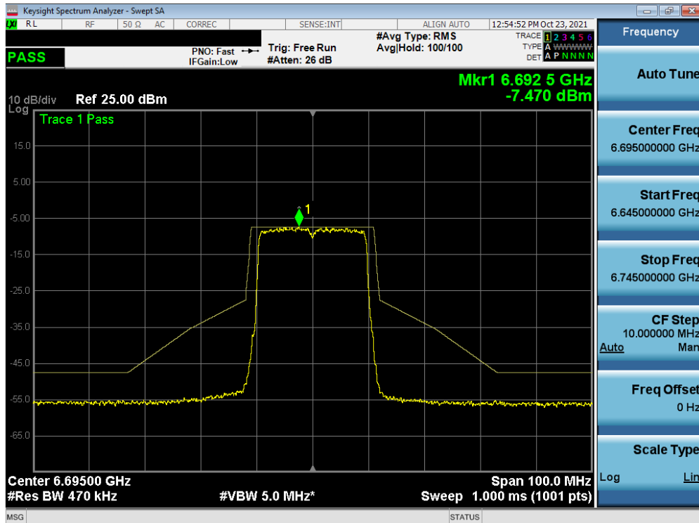
Plot 7-371. In-Band Emission Plot MIMO ANT1 (20MHz BW 802.11ax (Full Tones) (UNII Band 7) – Ch. 149)
