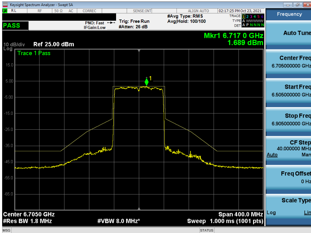
Plot 7-377. In-Band Emission Plot MIMO ANT1 (80MHz BW 802.11ax (Full Tones) (UNII Band 7) – Ch. 151)
