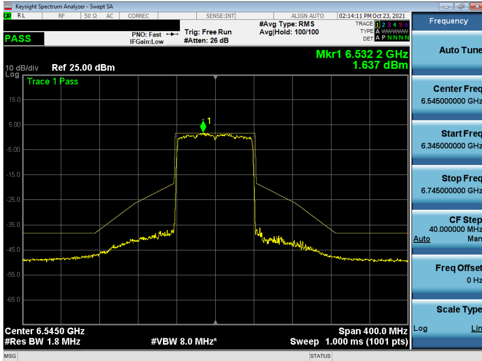
Plot 7-376. In-Band Emission Plot MIMO ANT1 (80MHz BW 802.11ax (Full Tones) (UNII Band 7) – Ch. 119)
