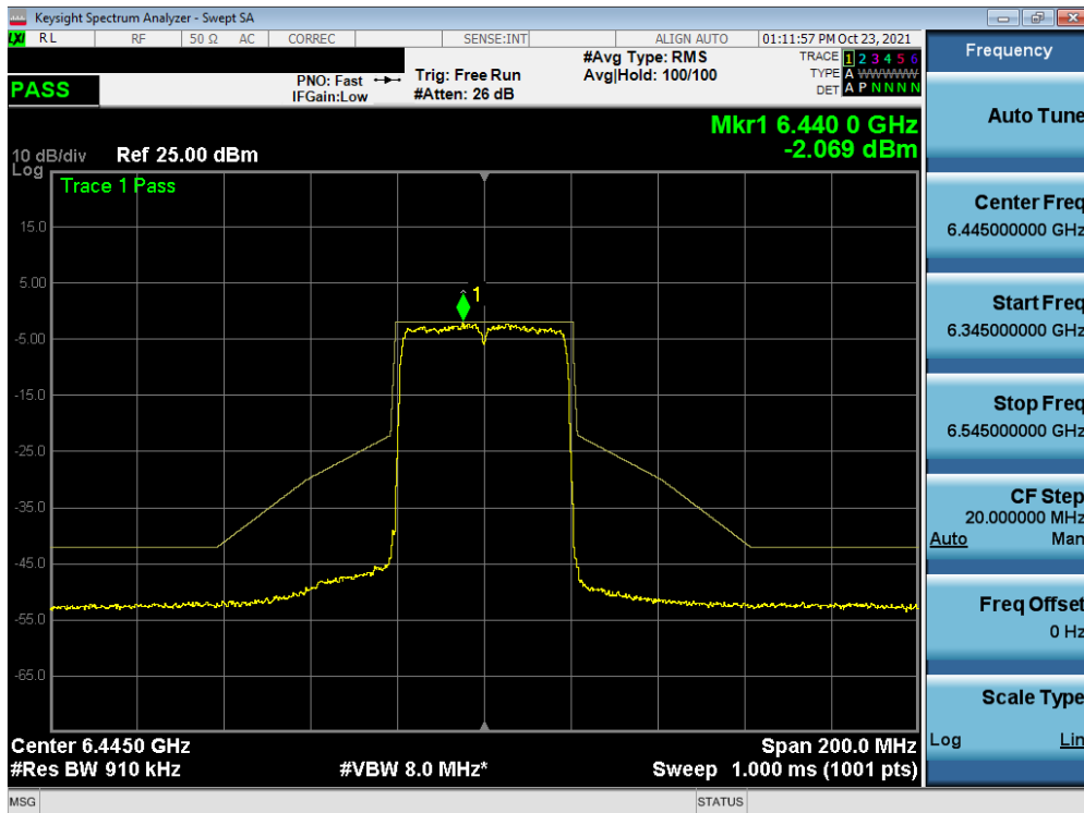
Plot 7-366. In-Band Emission Plot MIMO ANT1 (40MHz BW 802.11ax (Full Tones) (UNII Band 6) – Ch. 99)
