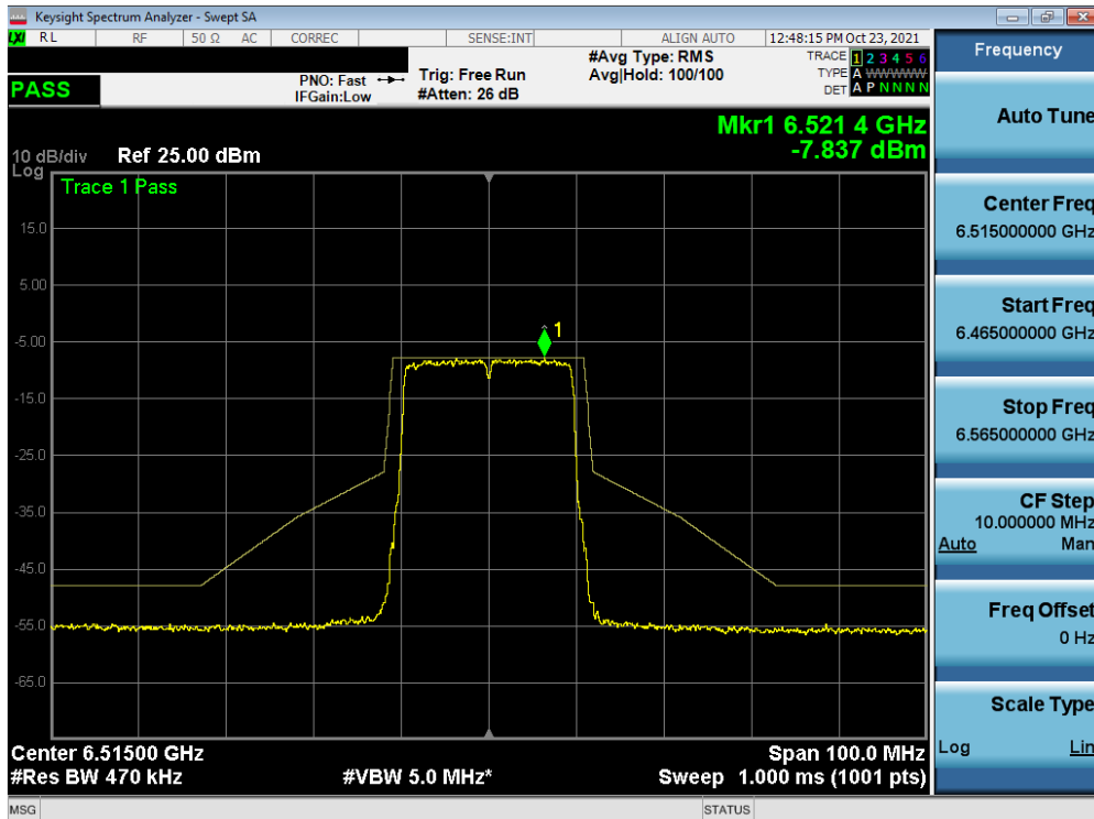
Plot 7-365. In-Band Emission Plot MIMO ANT1 (20MHz BW 802.11ax (Full Tones) (UNII Band 6) – Ch. 113)
