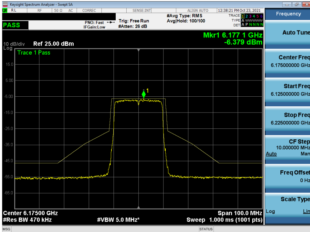
Plot 7-355. In-Band Emission Plot MIMO ANT1 (20MHz BW 802.11ax (Full Tones) UNII Band 5) – Ch. 45)
