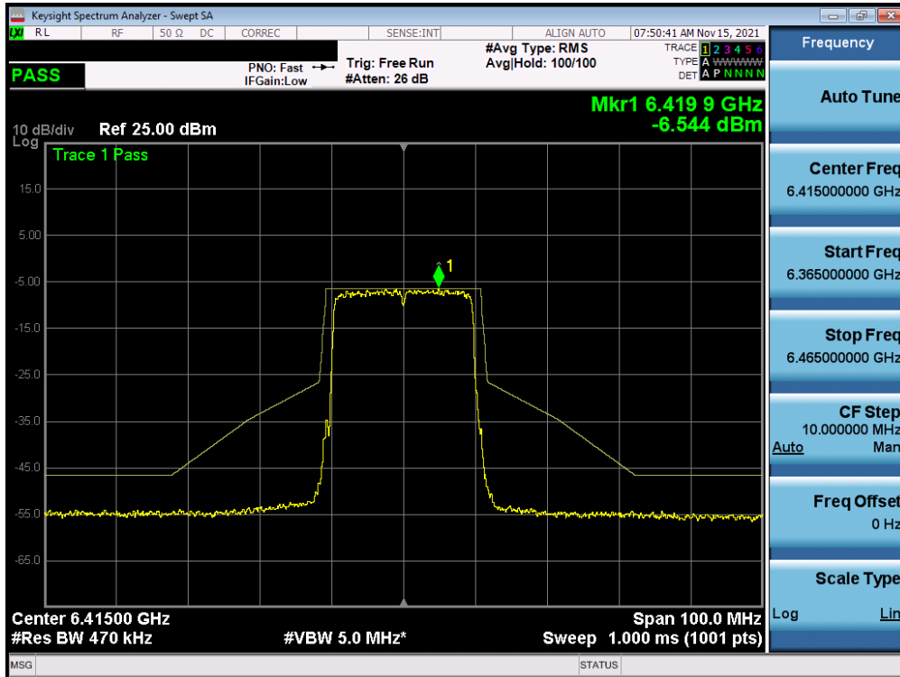
Plot 7-356. In-Band Emission Plot MIMO ANT1 (20MHz BW 802.11ax (Full Tones) UNII Band 5) – Ch. 93)
