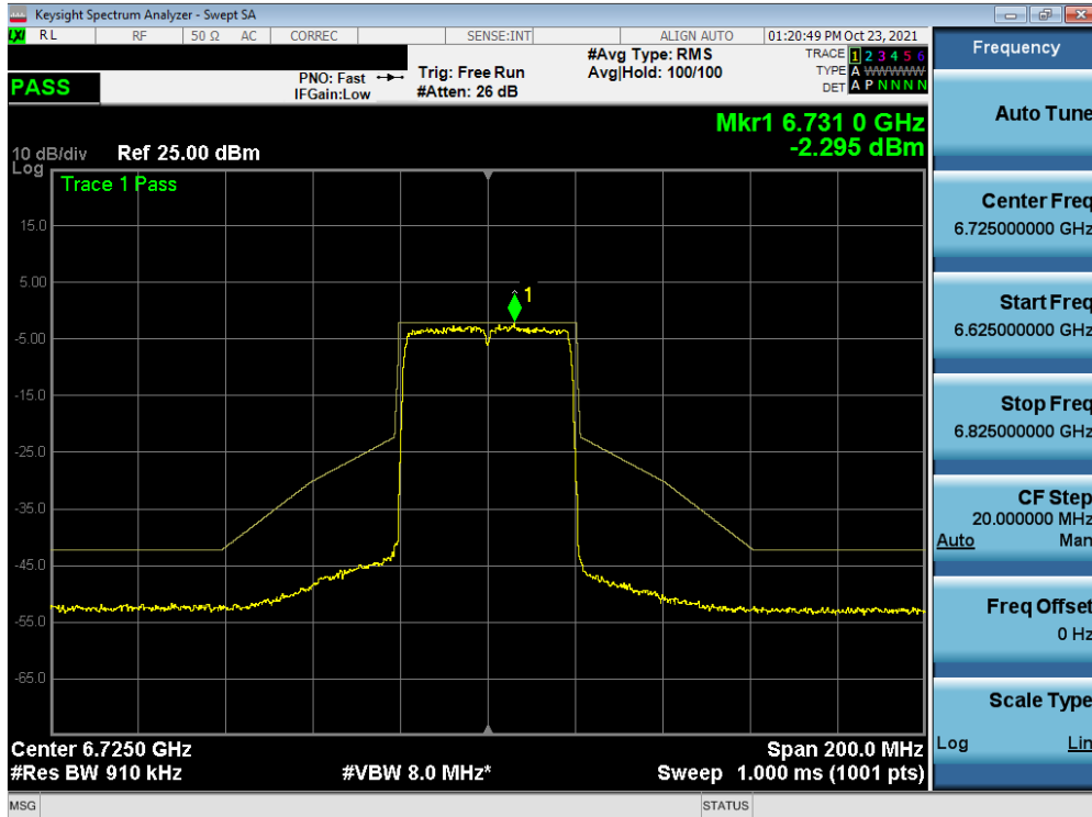
Plot 7-374. In-Band Emission Plot MIMO ANT1 (40MHz BW 802.11ax (Full Tones) (UNII Band 7) – Ch. 155)
