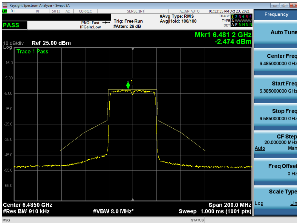
Plot 7-367. In-Band Emission Plot MIMO ANT1 (40MHz BW 802.11ax (Full Tones) (UNII Band 6) – Ch. 107)
