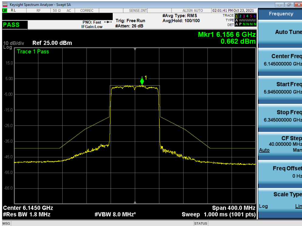
Plot 7-361. In-Band Emission Plot MIMO ANT1 (80MHz BW 802.11ax (Full Tones) (UNII Band 5) – Ch. 39)
