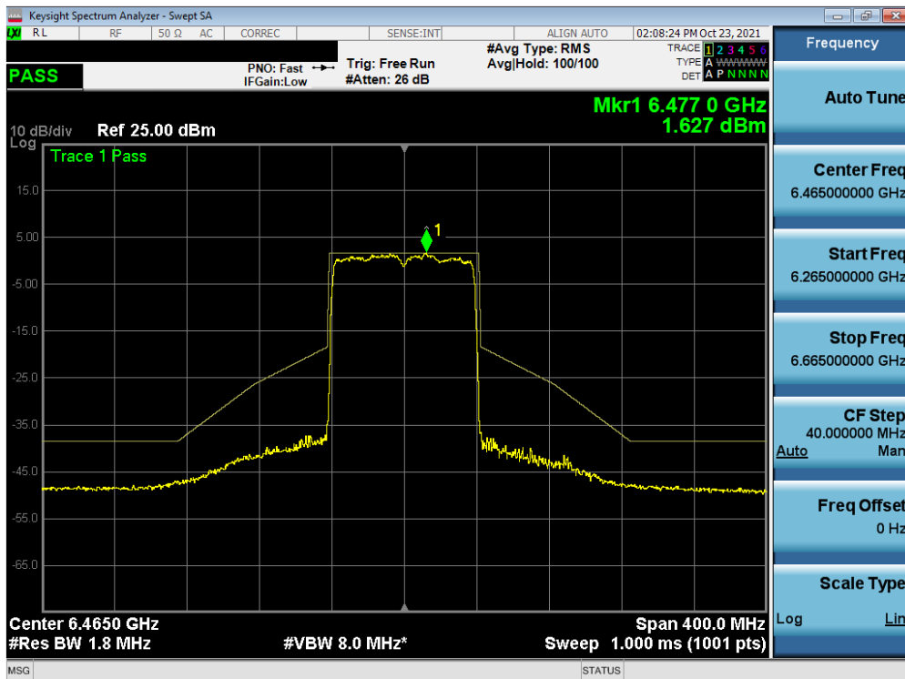
Plot 7-369. In-Band Emission Plot MIMO ANT1 (80MHz BW 802.11ax (Full Tones) (UNII Band 6) – Ch. 103)
