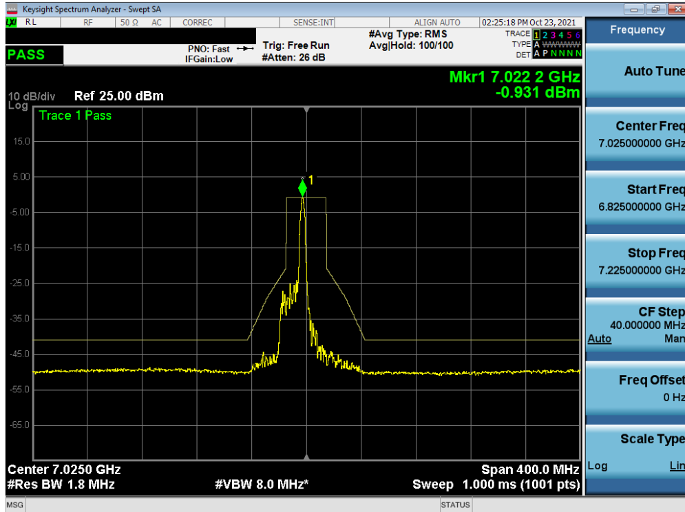
Plot 7-353. In-Band Emission Plot MIMO ANT1 (80MHz BW 802.11ax (26 Tones) (UNII Band 8) – Ch. 215)
