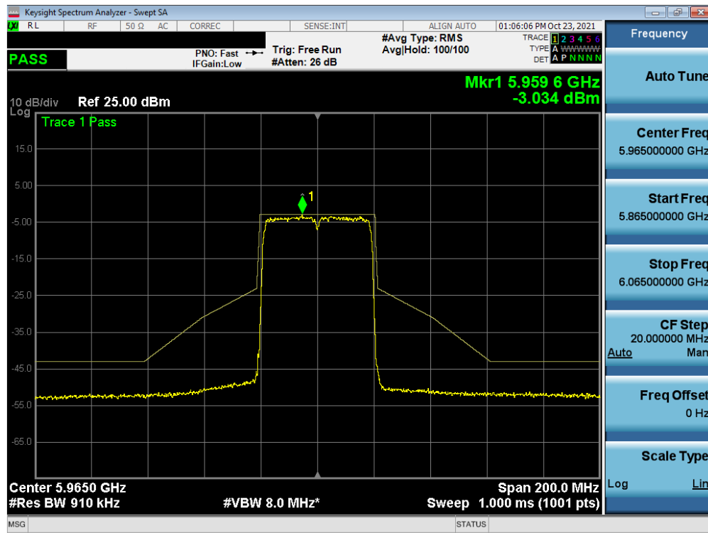
Plot 7-357. In-Band Emission Plot MIMO ANT1 (40MHz BW 802.11ax (Full Tones) (UNII Band 5) – Ch. 3)
