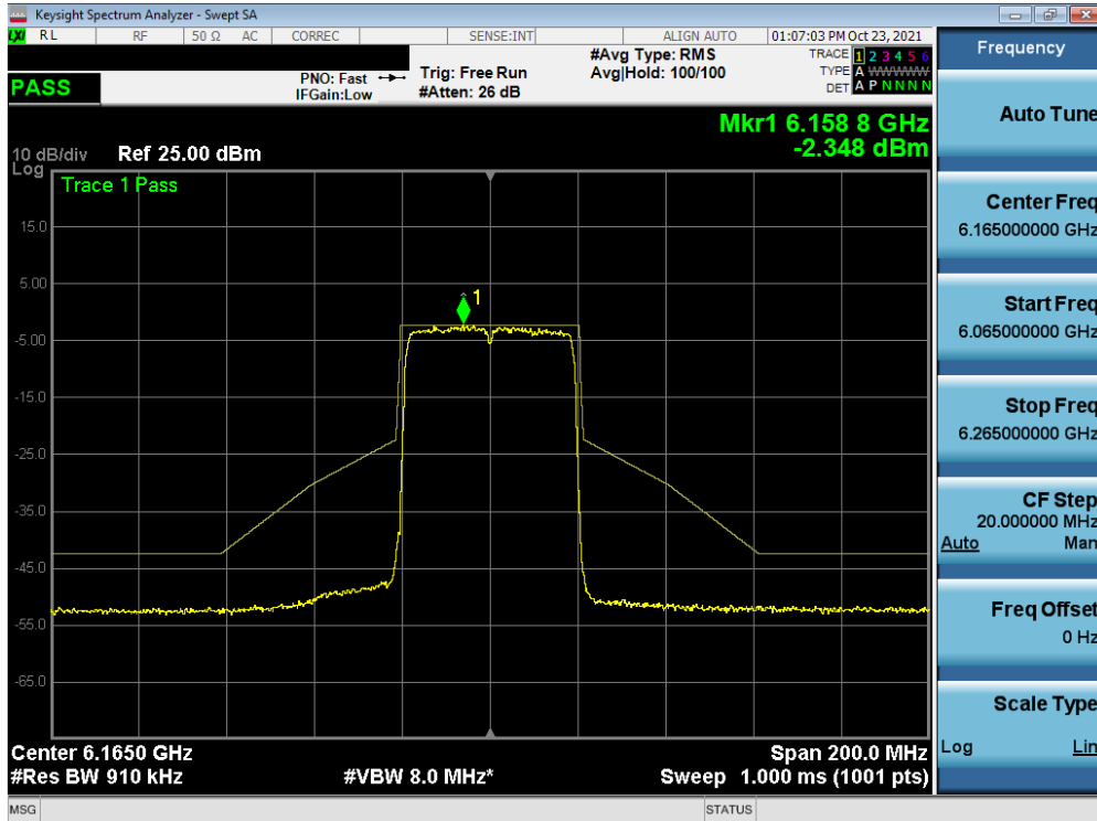
Plot 7-358. In-Band Emission Plot MIMO ANT1 (40MHz BW 802.11ax (Full Tones) (UNII Band 5) – Ch. 43)
