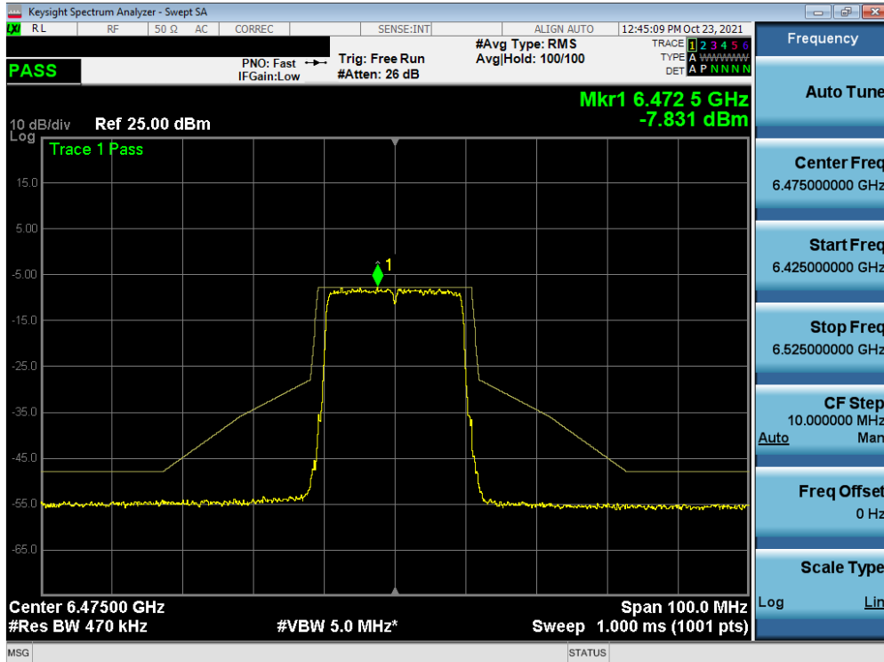
Plot 7-364. In-Band Emission Plot MIMO ANT1 (20MHz BW 802.11ax (Full Tones) (UNII Band 6) – Ch. 105)
