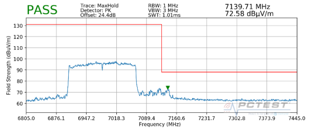
Plot 7-330. Radiated Upper Band Edge Plot MIMO (Peak – UNII Band 8)
