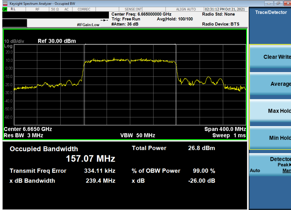
Plot 7-91. 26dB Bandwidth Plot MIMO ANT2 (160MHz 802.11ax (UNII Band 7) – Ch. 143)
