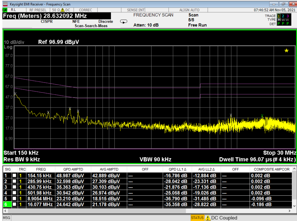
Plot 7-400. Line Conducted Plot with 802.11a UNII Band 2C (N)
