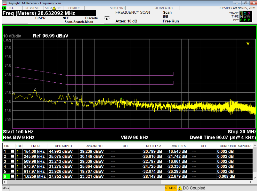
Plot 7-403. Line Conducted Plot with 802.11a UNII Band 4 (L1)
