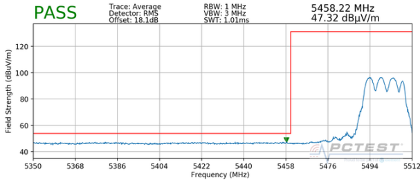
Plot 7-372. Radiated Lower Band Edge Plot CDD (Average – UNII Band 2C)
