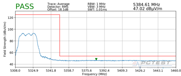
Plot 7-370. Radiated Upper Band Edge Plot CDD (Average – UNII Band 2A)
