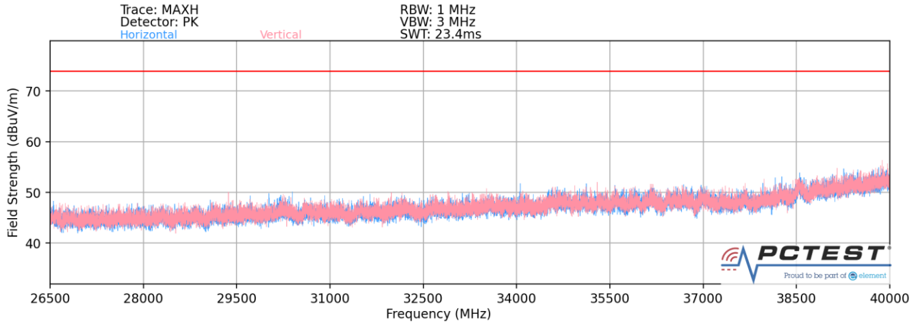
Plot 7-367. Radiated Spurious Plot above 26.5GHz (Dual Band Simult. Tx)
