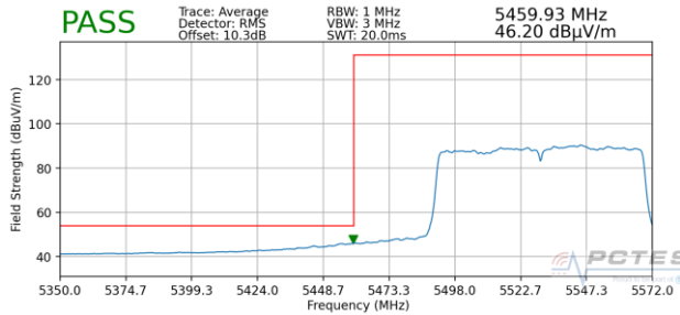
Plot 7-390. Radiated Lower Band Edge Plot MIMO (Average – UNII Band 2C)
