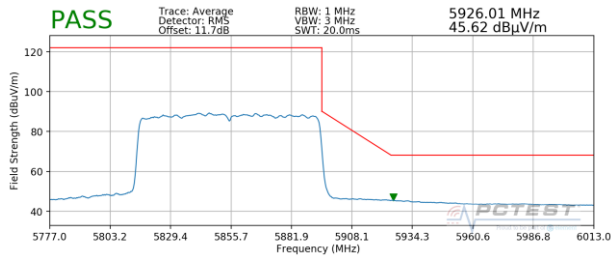
Plot 7-394. Radiated Upper Band Edge Plot MIMO (Average - UNII Band 4)
