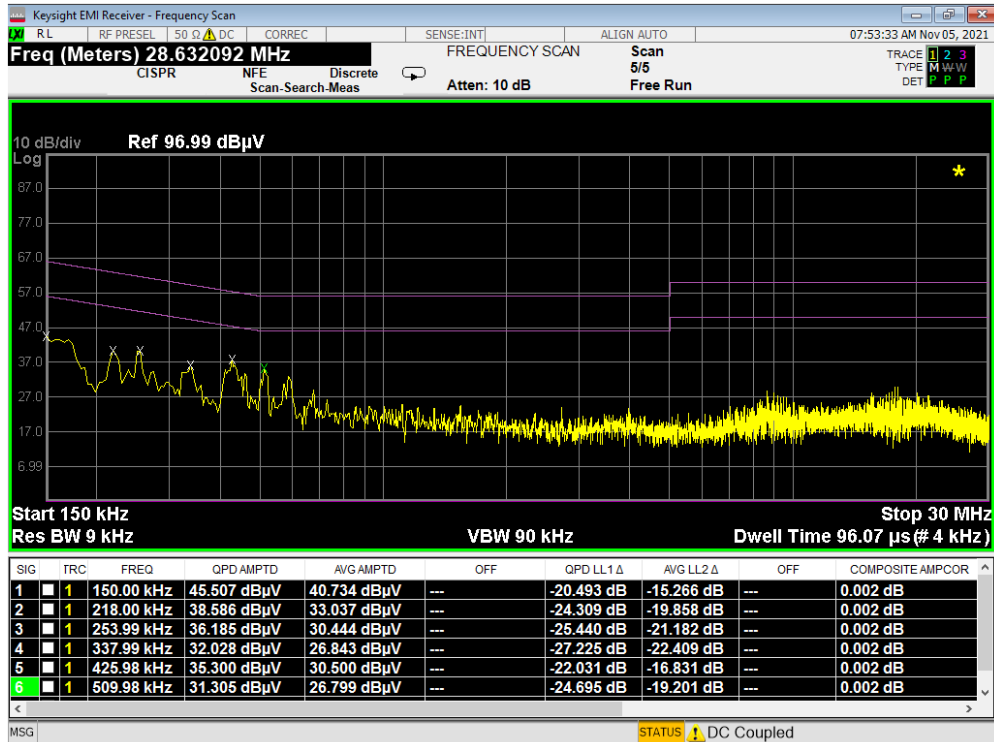
Plot 7-402. Line Conducted Plot with 802.11a UNII Band 3 (N)
