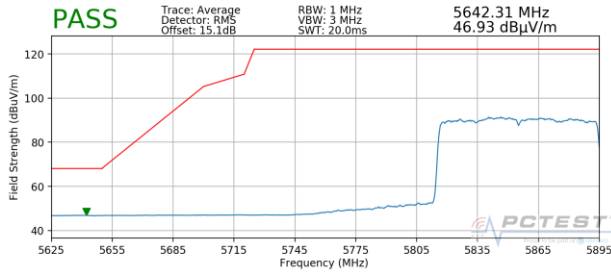
Plot 7-393. Radiated Lower Band Edge Plot MIMO (Average - UNII Band 4)
