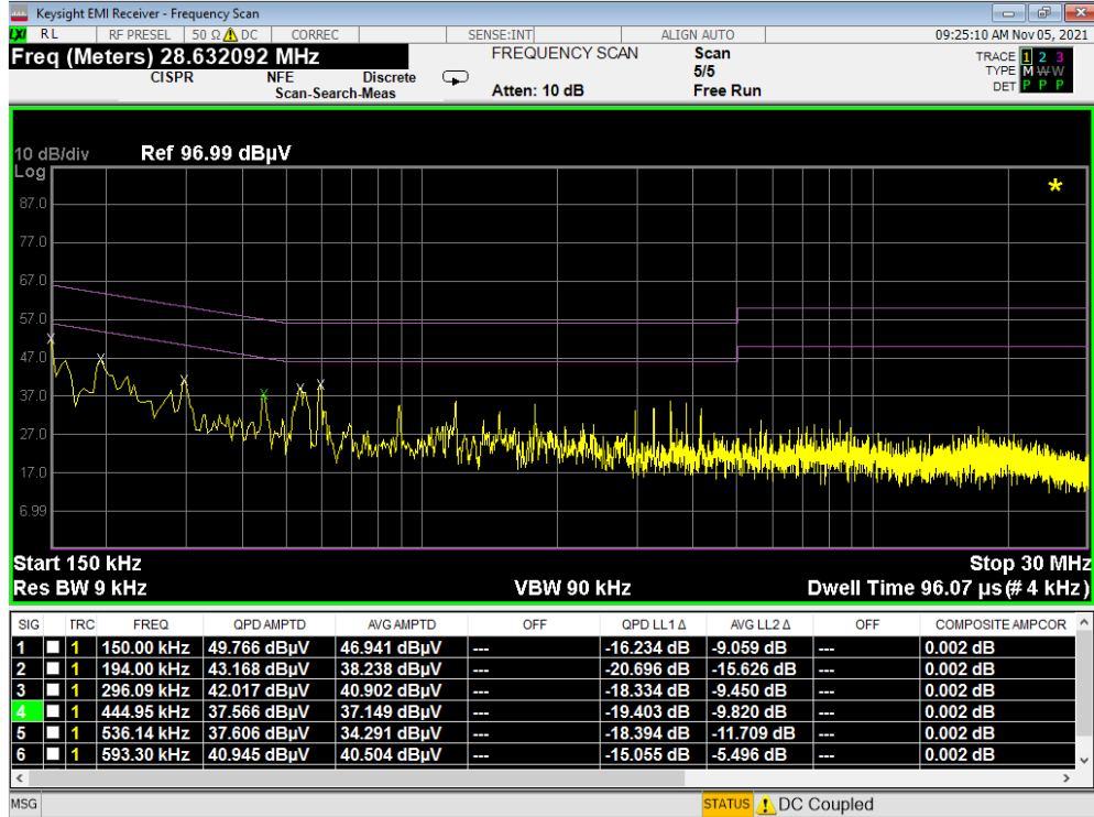
Plot 7-405. Line Conducted Plot with 802.11a UNII Band 1 (L1) WCP
