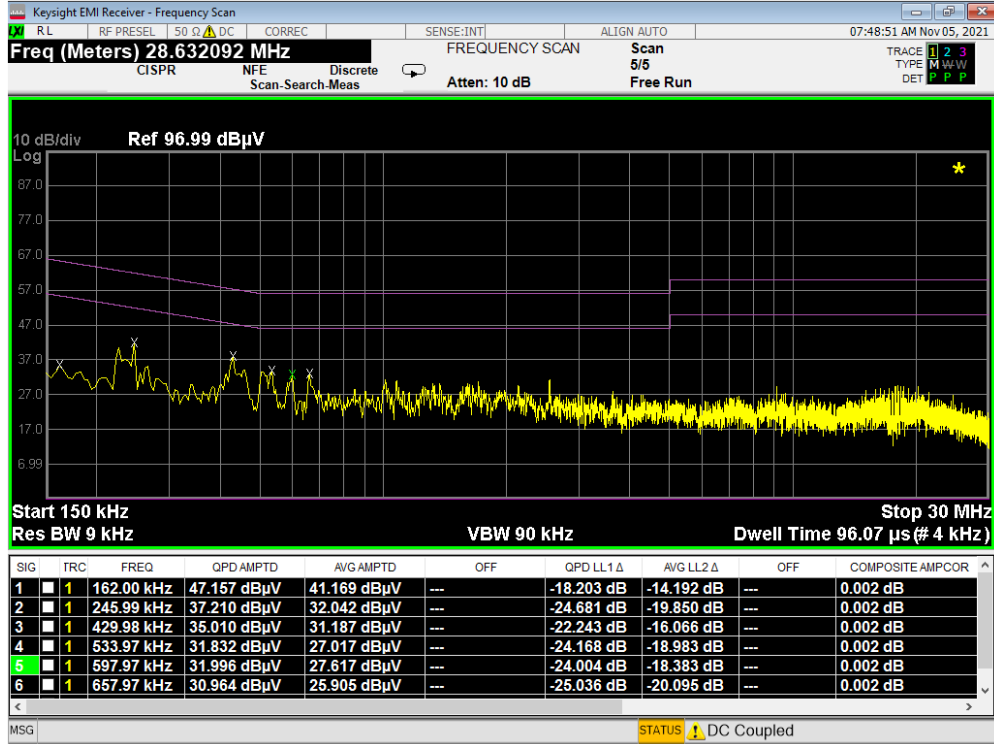
Plot 7-397. Line Conducted Plot with 802.11a UNII Band 2A (L1)
