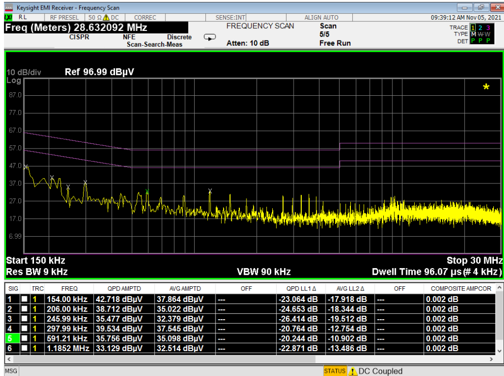
Plot 7-414. Line Conducted Plot with 802.11a UNII Band 4 (N) WCP
