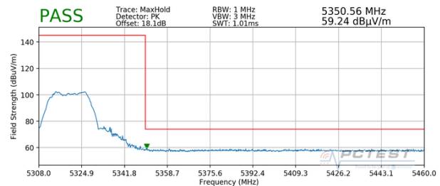
Plot 7-371. Radiated Upper Band Edge Plot CDD (Peak – UNII Band 2A)
