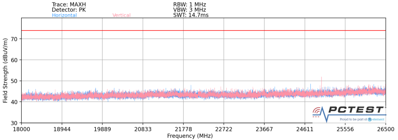
Plot 7-366. Radiated Spurious Plot 18GHz – 26.5GHz (Dual Band Simult. Tx)
