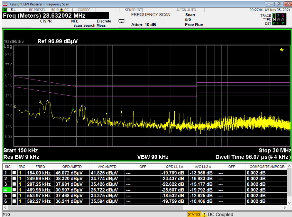
Plot 7-406. Line Conducted Plot with 802.11a UNII Band 1 (N) WCP
