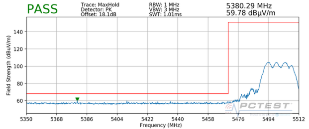
Plot 7-373. Radiated Lower Band Edge Plot CDD (Peak – UNII Band 2C)
