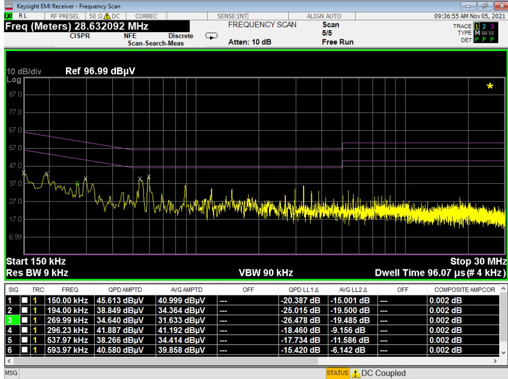
Plot 7-411. Line Conducted Plot with 802.11a UNII Band 3 (L1) WCP
