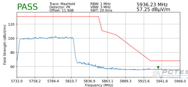
Plot 7-392. Radiated Upper Band Edge Plot MIMO (Peak – UNII Band 3)
