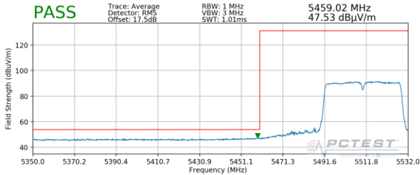
Plot 7-381. Radiated Lower Band Edge Plot MIMO (Average – UNII Band 2C)
