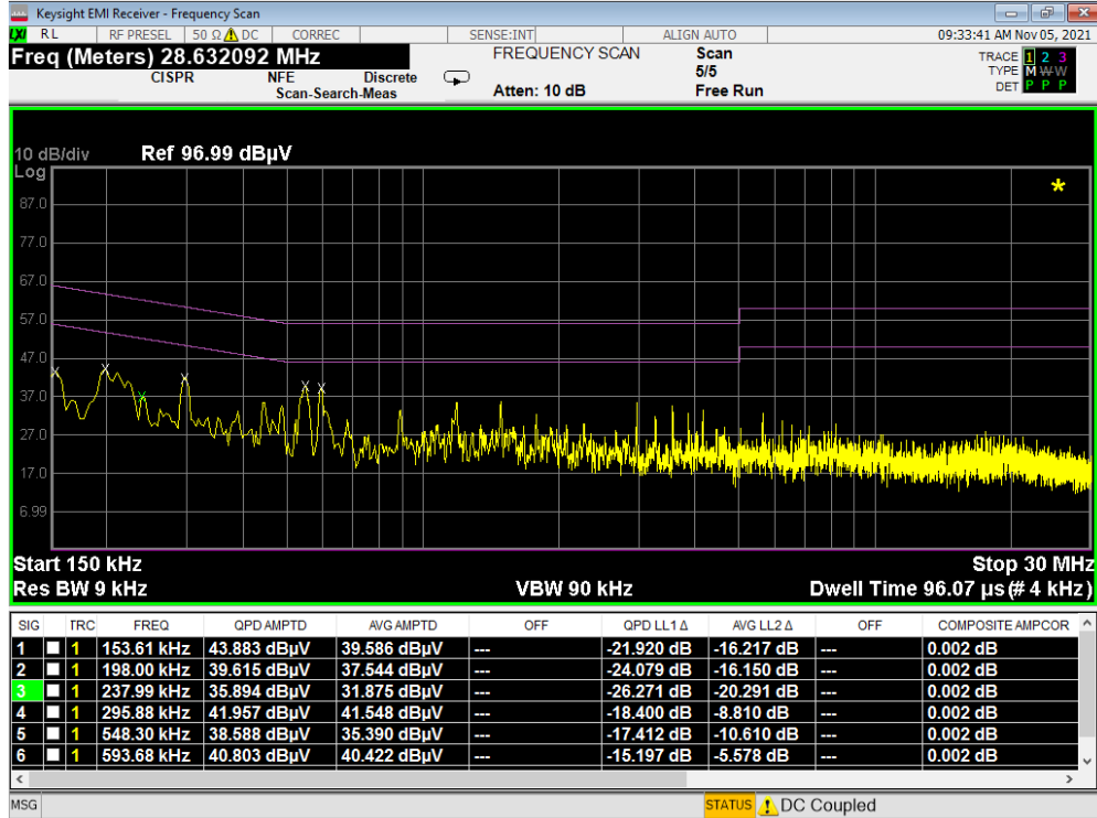
Plot 7-409. Line Conducted Plot with 802.11a UNII Band 2C (L1) WCP
