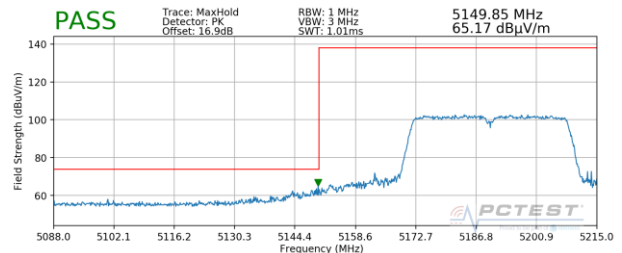
Plot 7-378. Radiated Lower Band Edge Plot MIMO (Peak – UNII Band 1)
