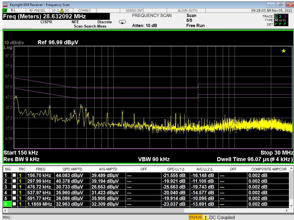
Plot 7-408. Line Conducted Plot with 802.11a UNII Band 2A (N) WCP
