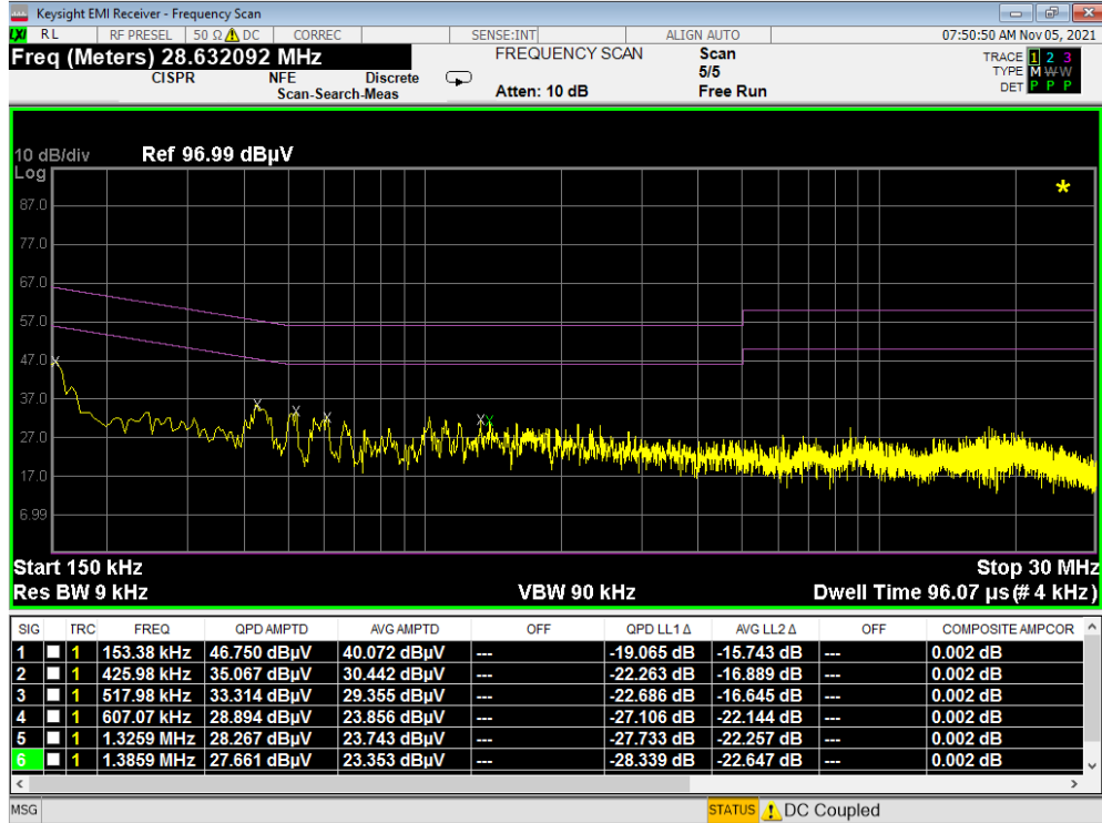
Plot 7-401. Line Conducted Plot with 802.11a UNII Band 3 (L1)
