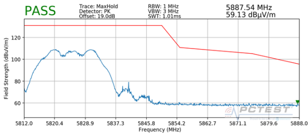
Plot 7-374. Radiated Upper Band Edge Plot CDD (Peak – UNII Band 3)
