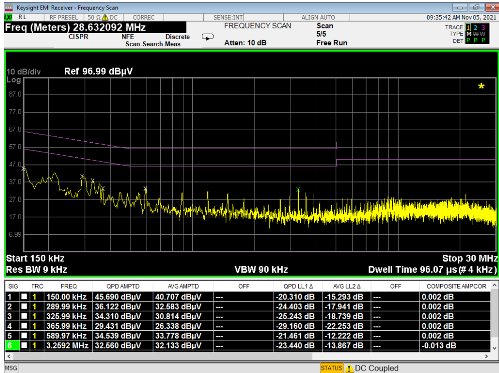
Plot 7-412. Line Conducted Plot with 802.11a UNII Band 3 (N) WCP
