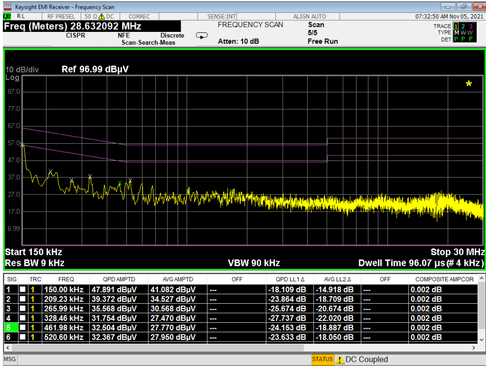
Plot 7-395. Line Conducted Plot with 802.11a UNII Band 1 (L1)
