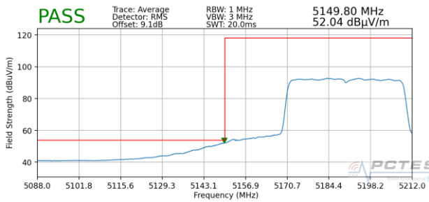
Plot 7-377. Radiated Lower Band Edge Plot MIMO (Average – UNII Band 1)
