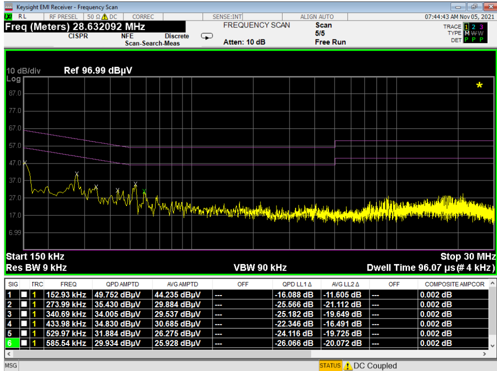
Plot 7-398. Line Conducted Plot with 802.11a UNII Band 2A (N)
