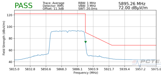
Plot 7-385. Radiated Upper Band Edge Plot MIMO (Average - UNII Band 4)
