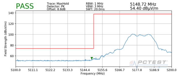
Plot 7-369. Radiated Lower Band Edge Plot MIMO (Peak – UNII Band 1)
