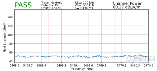
Plot 7-382. Radiated Lower Band Edge Plot MIMO (Peak – UNII Band 2C)
