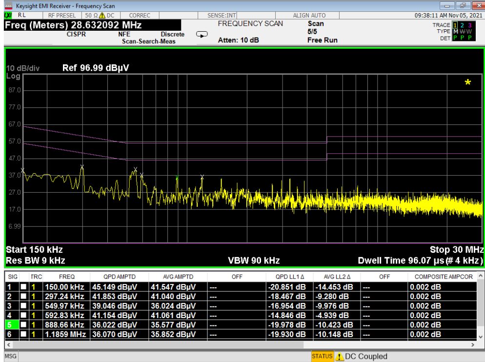
Plot 7-413. Line Conducted Plot with 802.11a UNII Band 4 (L1) WCP
