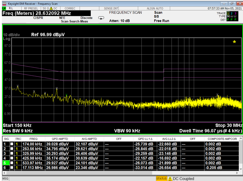
Plot 7-404. Line Conducted Plot with 802.11a UNII Band 4 (N)
