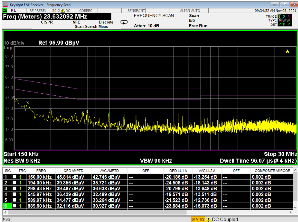
Plot 7-410. Line Conducted Plot with 802.11a UNII Band 2C (N) WCP
