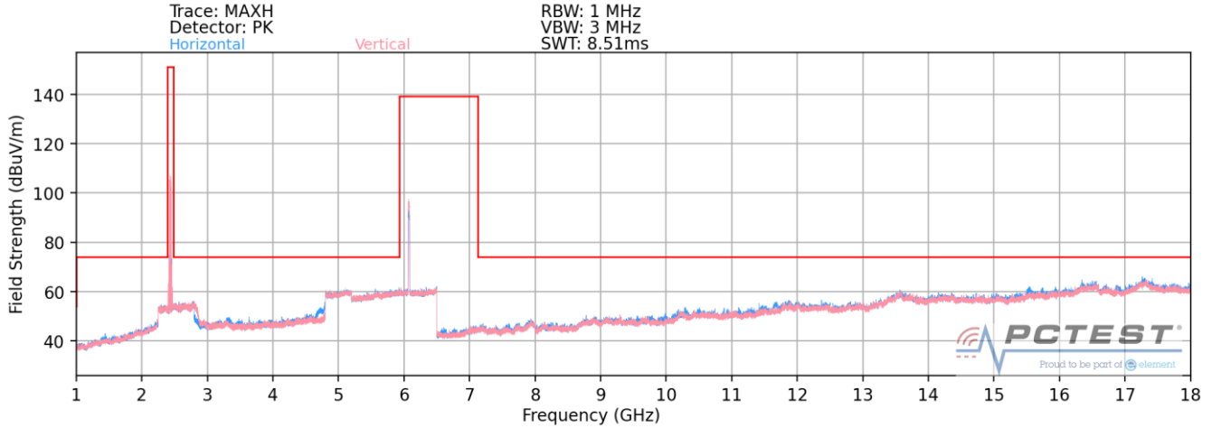
Plot 7-365. Radiated Spurious Plot above 1GHz (Dual Band Simult. Tx)
