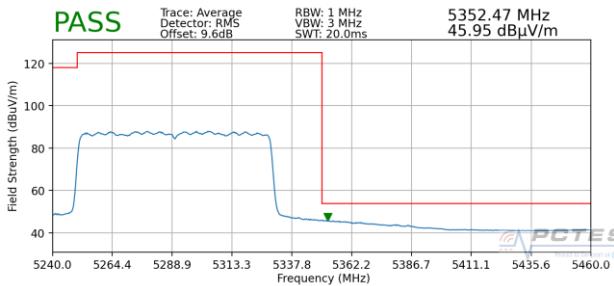
Plot 7-388. Radiated Upper Band Edge Plot MIMO (Average – UNII Band 2A)
