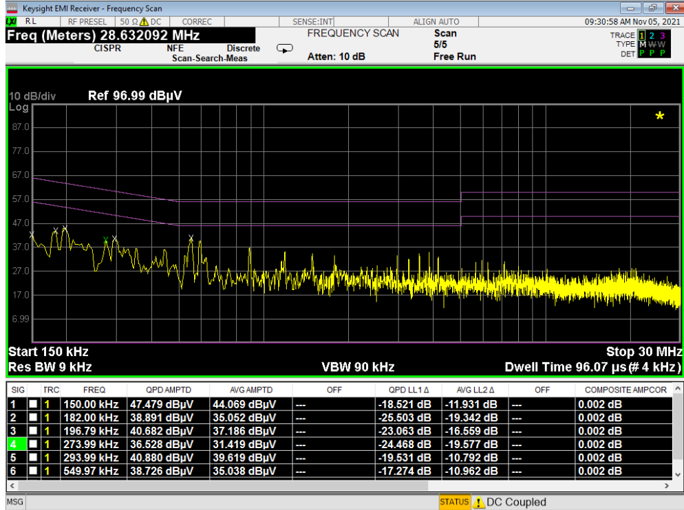
Plot 7-407. Line Conducted Plot with 802.11a UNII Band 2A (L1) WCP
