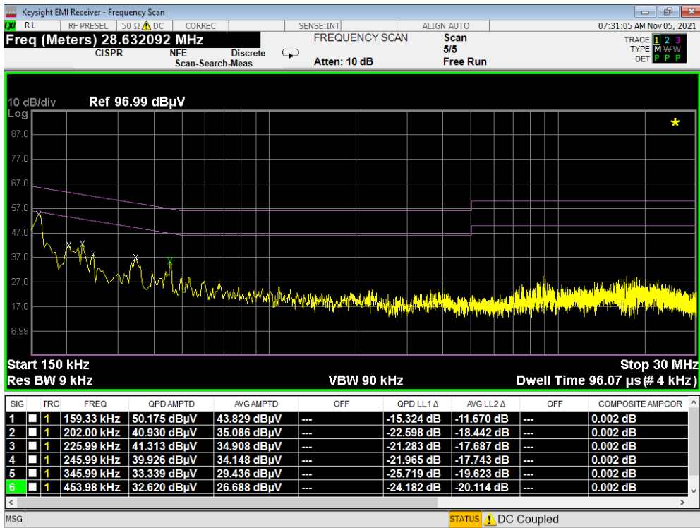
Plot 7-396. Line Conducted Plot with 802.11a UNII Band 1 (N)
