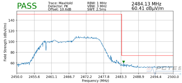
Plot 7-80. Radiated Restricted Upper Band Edge Measurement MIMO (Peak – 106 Tones)
