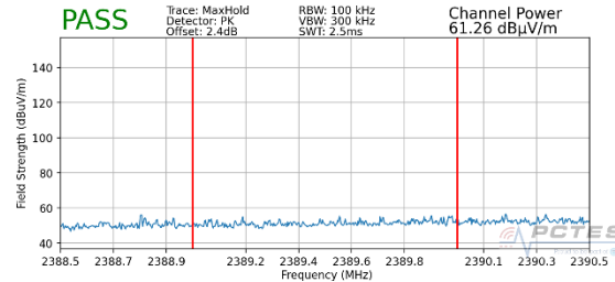
Plot 7-84. Radiated Restricted Lower Band Edge Measurement MIMO (Peak – 242 Tones)
