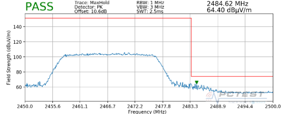
Plot 7-90. Radiated Restricted Upper Band Edge Measurement MIMO (Peak – 242 Tones)
