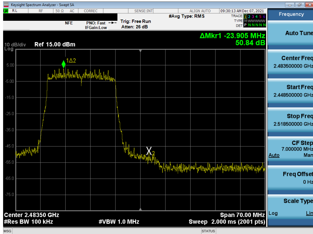
Plot 7-41. Band Edge Plot MIMO ANT2 (802.11ax OFDMA – 242 Tones – Ch. 12)
