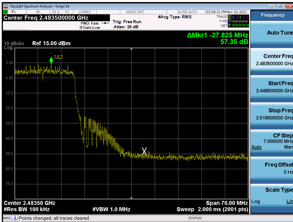
Plot 7-39. Band Edge Plot MIMO ANT2 (802.11ax OFDMA – 242 Tones – Ch. 10)
