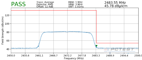
Plot 7-91. Radiated Restricted Upper Band Edge Measurement MIMO (Average – 242 Tones)
