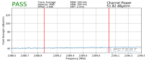
Plot 7-83. Radiated Restricted Lower Band Edge Measurement MIMO (Average – 242 Tones)
