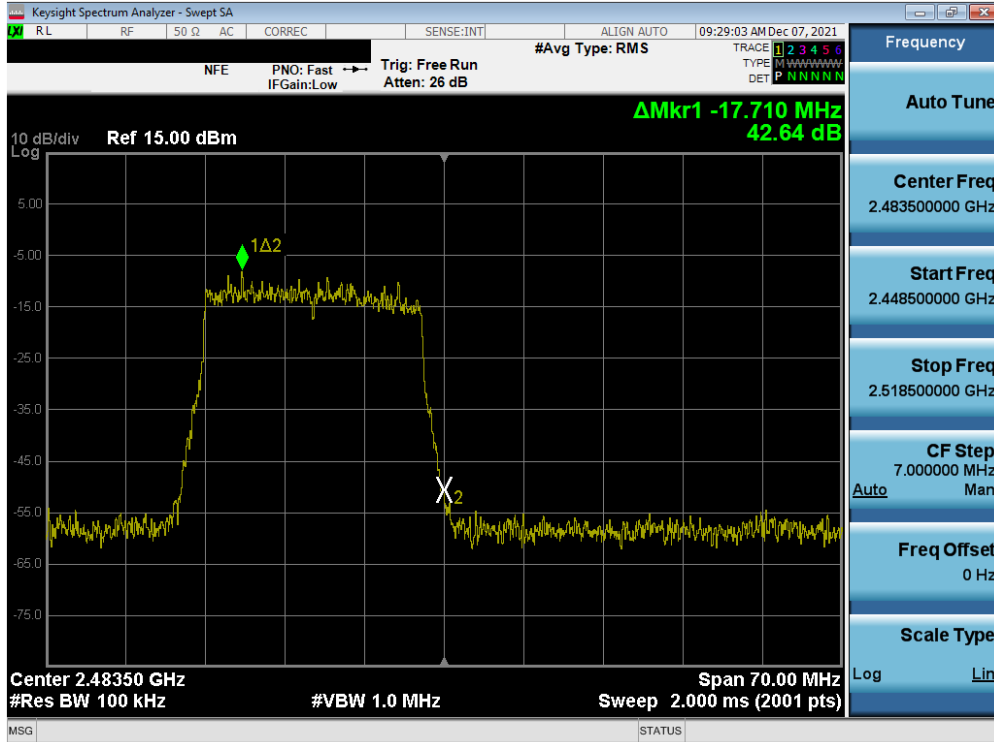
Plot 7-33. Band Edge Plot MIMO ANT1 (802.11ax OFDMA – 242 Tones – Ch. 13)
