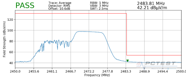
Plot 7-79. Radiated Restricted Upper Band Edge Measurement MIMO (Average – 106 Tones)
