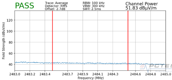
Plot 7-87. Radiated Restricted Upper Band Edge Measurement MIMO (Average – 242 Tones)
