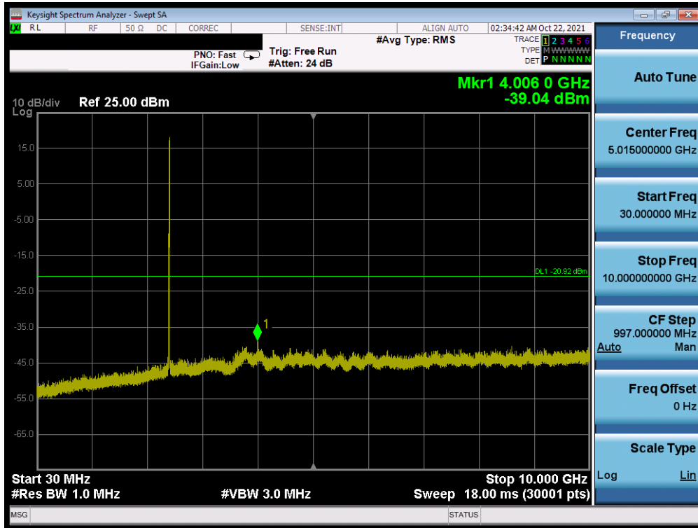
Plot 7-55. Conducted Spurious Plot MIMO ANT2 (802.11ax OFDMA – 26 Tones – Ch. 1)
