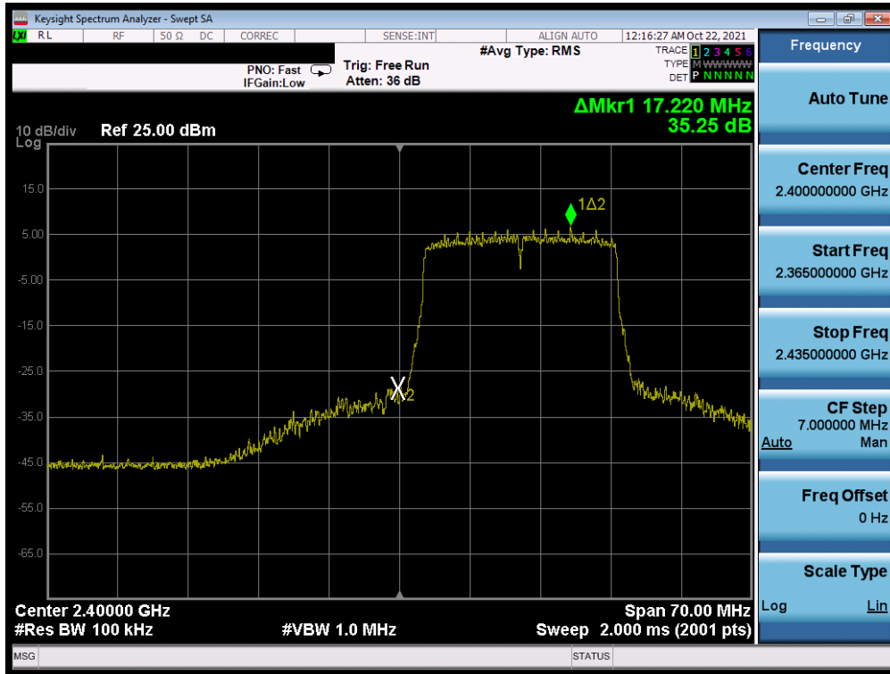
Plot 7-38. Band Edge Plot MIMO ANT2 (802.11ax OFDMA – 242 Tones – Ch. 1)
