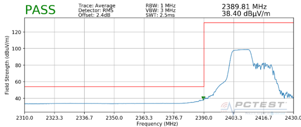
Plot 7-75. Radiated Restricted Lower Band Edge Measurement MIMO (Average – 106 Tones)
