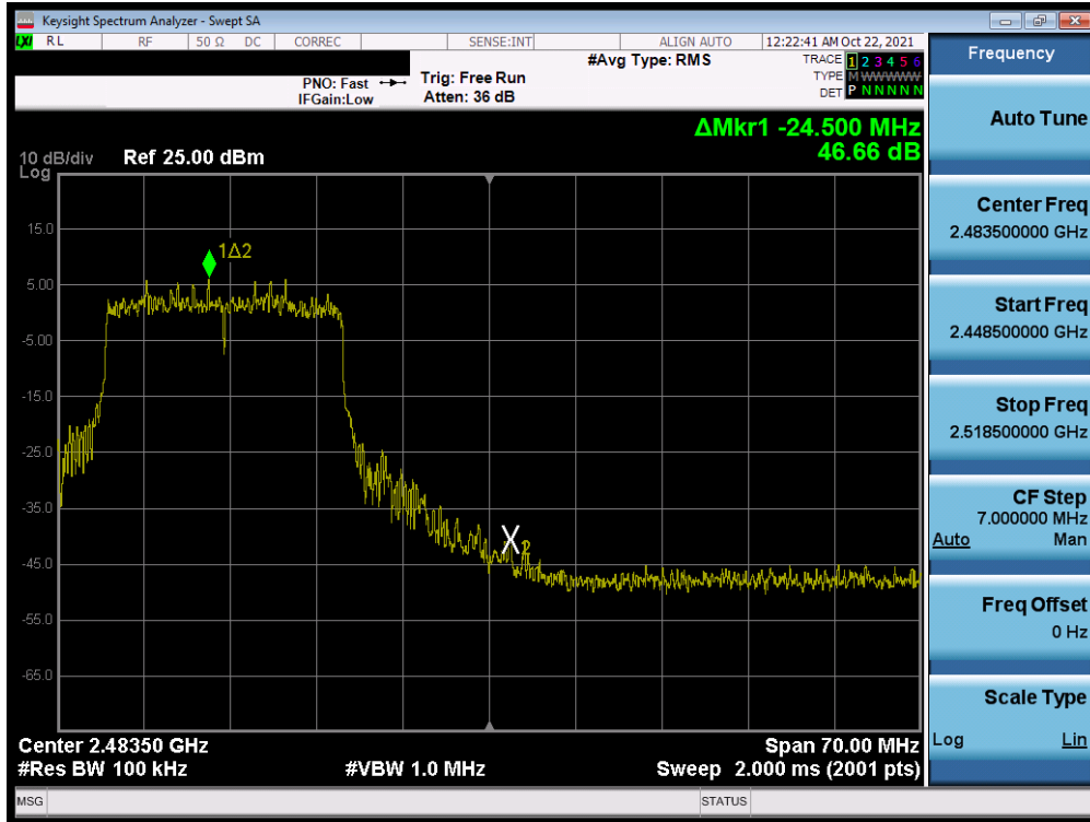
Plot 7-40. Band Edge Plot MIMO ANT2 (802.11ax OFDMA – 242 Tones – Ch. 11)
