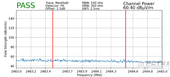
Plot 7-88. Radiated Restricted Upper Band Edge Measurement MIMO (Peak – 242 Tones)
