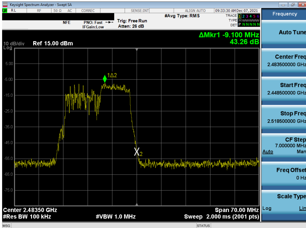
Plot 7-37. Band Edge Plot MIMO ANT2 (802.11ax OFDMA – 106 Tones – Ch. 13)
