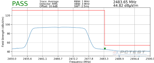
Plot 7-89. Radiated Restricted Upper Band Edge Measurement MIMO (Average – 242 Tones)
