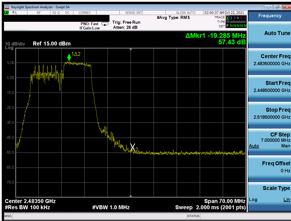
Plot 7-35. Band Edge Plot MIMO ANT2 (802.11ax OFDMA – 106 Tones – Ch. 11)
