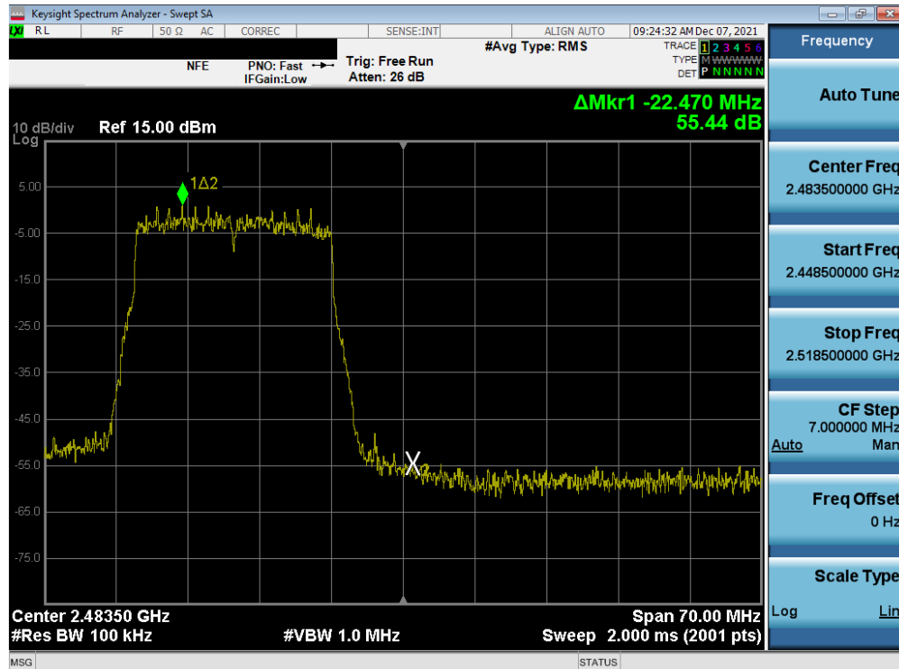
Plot 7-32. Band Edge Plot MIMO ANT1 (802.11ax OFDMA – 242 Tones – Ch. 12)
