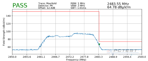
Plot 7-82. Radiated Restricted Upper Band Edge Measurement MIMO (Peak – 106 Tones)
