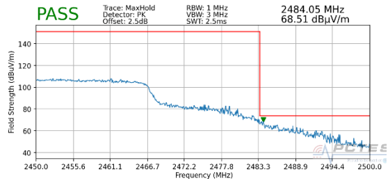
Plot 7-86. Radiated Restricted Upper Band Edge Measurement MIMO (Peak – 242 Tones)
