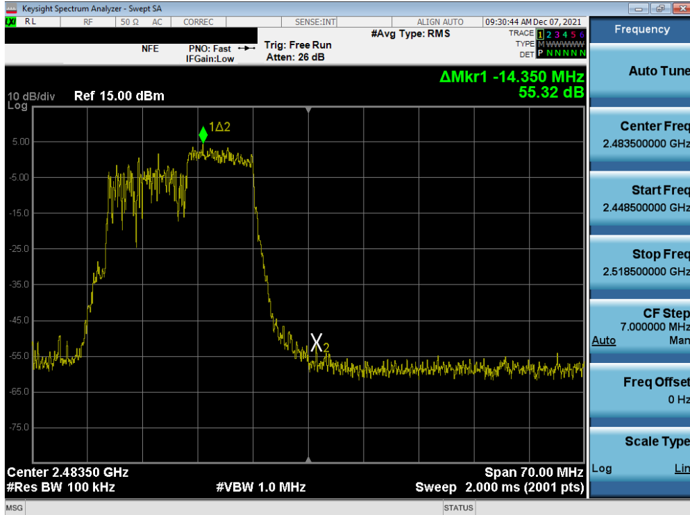
Plot 7-36. Band Edge Plot MIMO ANT2 (802.11ax OFDMA – 106 Tones – Ch. 12)
