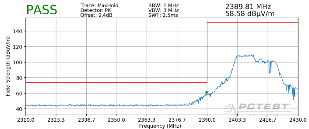
Plot 7-76. Radiated Restricted Lower Band Edge Measurement MIMO (Peak – 106 Tones)
