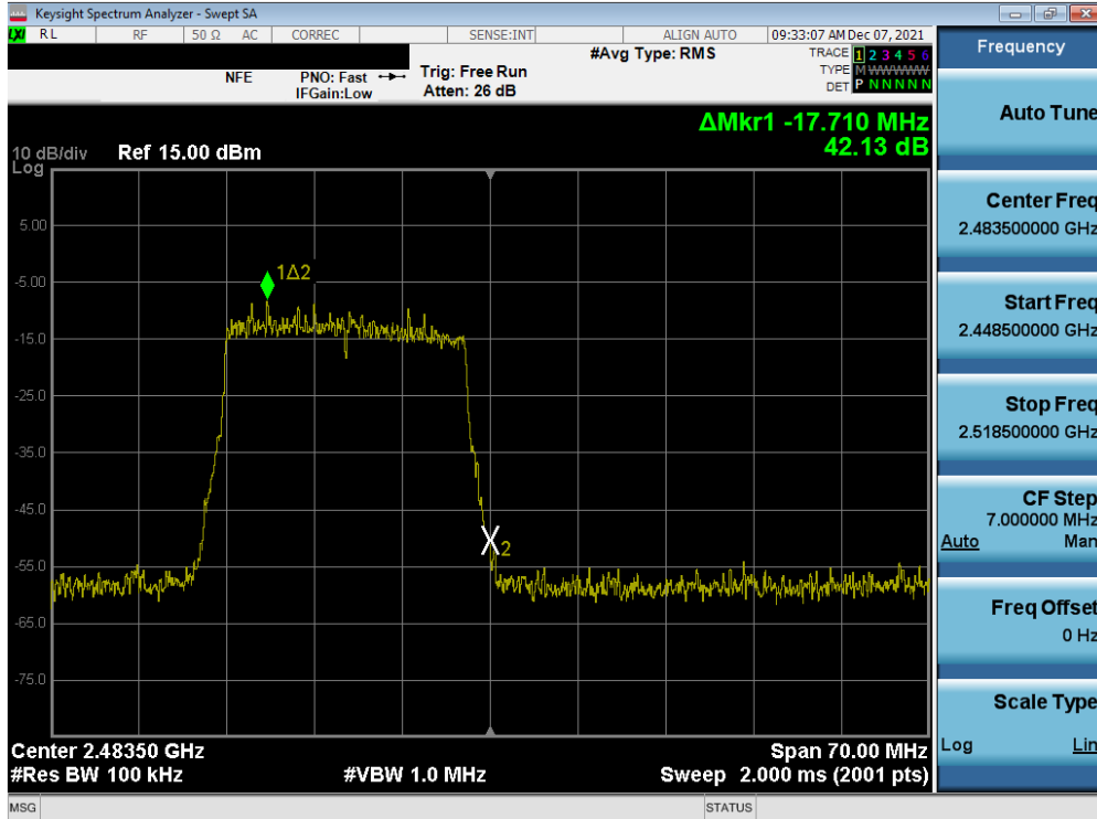
Plot 7-42. Band Edge Plot MIMO ANT2 (802.11ax OFDMA – 242 Tones – Ch. 13)
