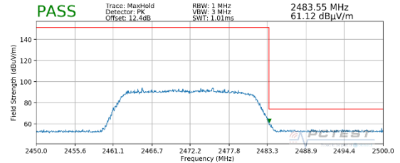
Plot 7-92. Radiated Restricted Upper Band Edge Measurement MIMO (Peak – 242 Tones)
