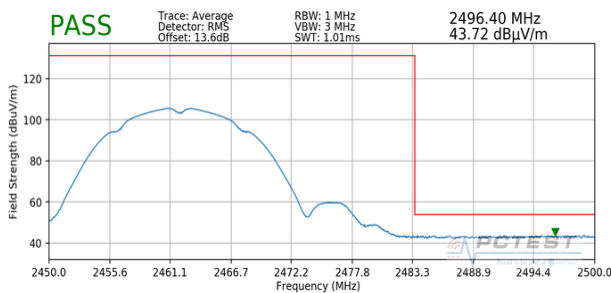
Plot 7-125. Radiated Restricted Upper Band Edge Measurement SISO ANT2 (Average)
