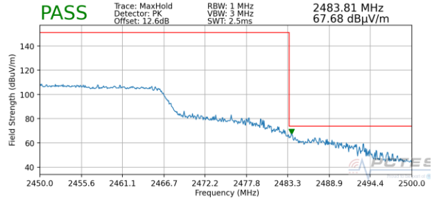
Plot 7-136. Radiated Restricted Upper Band Edge Measurement MIMO (Peak)
