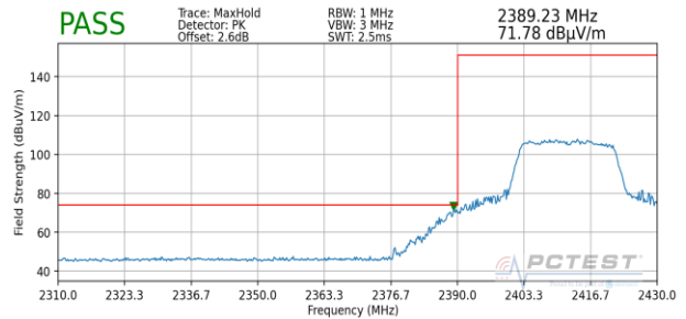
Plot 7-132. Radiated Restricted Lower Band Edge Measurement MIMO (Peak)
