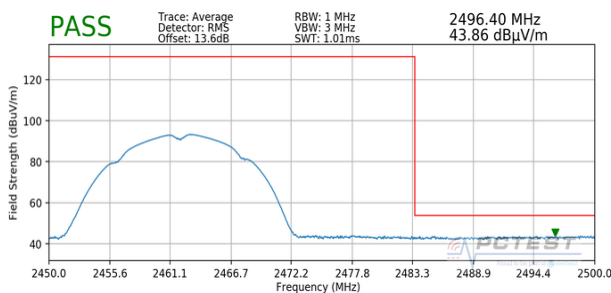
Plot 7-117. Radiated Restricted Upper Band Edge Measurement SISO ANT1 (Average)
