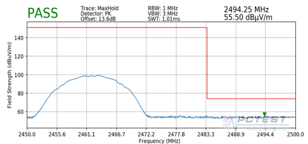
Plot 7-118. Radiated Restricted Upper Band Edge Measurement SISO ANT1 (Peak)
