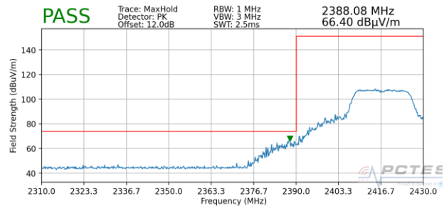
Plot 7-134. Radiated Restricted Lower Band Edge Measurement MIMO (Peak)
