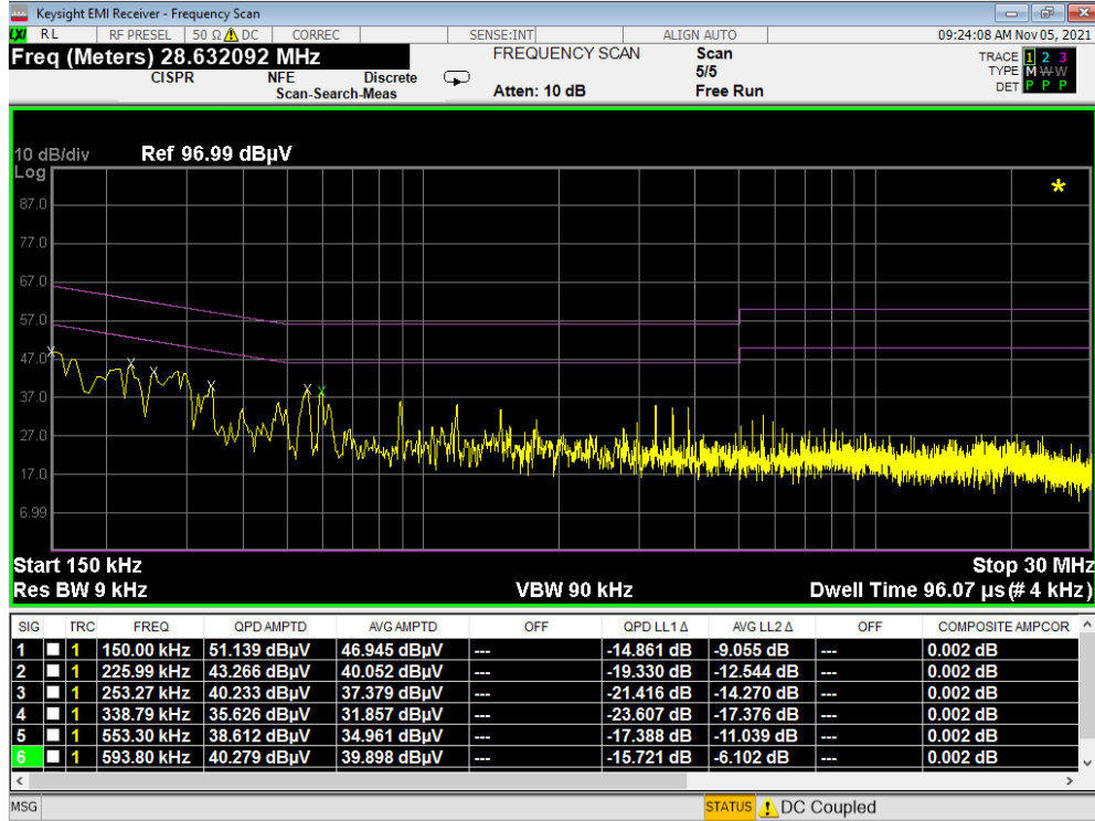
Plot 7-146. Line Conducted Plot with 802.11b (L1) WCP
