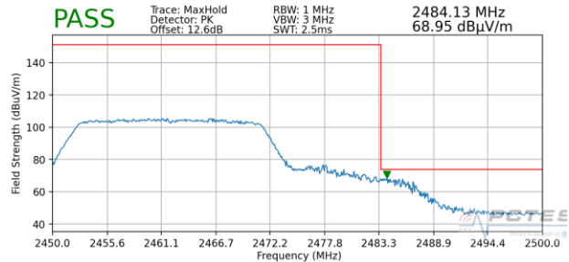
Plot 7-138. Radiated Restricted Upper Band Edge Measurement MIMO (Peak)
