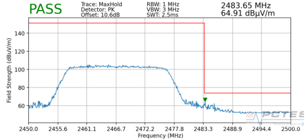
Plot 7-140. Radiated Restricted Upper Band Edge Measurement MIMO (Peak)
