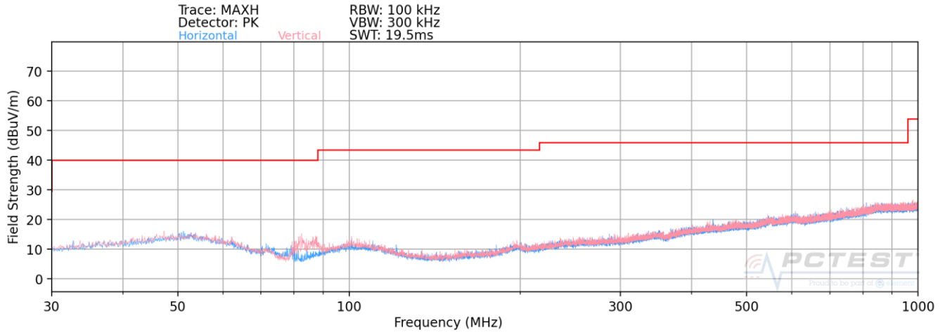
Plot 7-143. Radiated Spurious Plot below 1GHz MIMO
