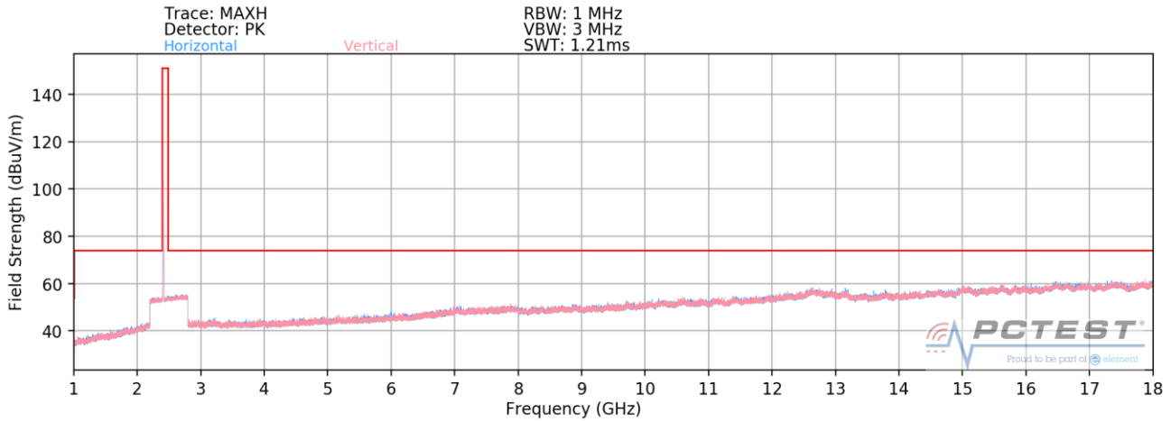
Plot 7-107. Radiated Spurious Plot above 1GHz SISO ANT2 (802.11b – Ch. 1)
