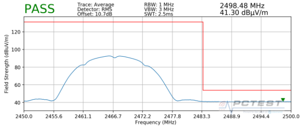
Plot 7-119. Radiated Restricted Upper Band Edge Measurement SISO ANT1 (Average)
