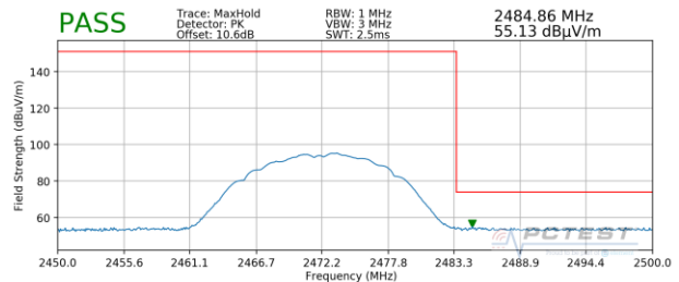
Plot 7-122. Radiated Restricted Upper Band Edge Measurement SISO ANT1 (Peak)
