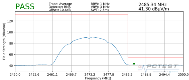
Plot 7-121. Radiated Restricted Upper Band Edge Measurement SISO ANT1 (Average)
