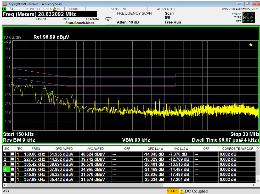
Plot 7-147. Line Conducted Plot with 802.11b (N) WCP
