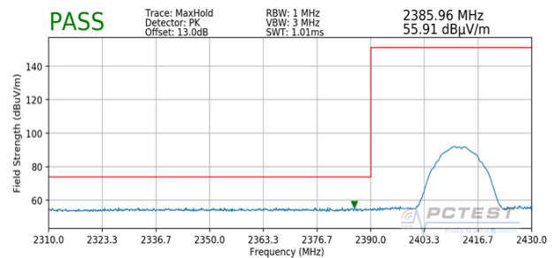
Plot 7-116. Radiated Restricted Lower Band Edge Measurement SISO ANT1 (Peak)
