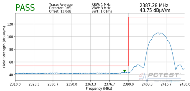
Plot 7-123. Radiated Restricted Lower Band Edge Measurement SISO ANT2 (Average)
