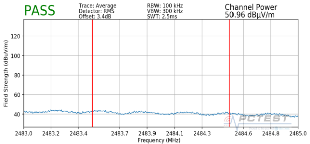
Plot 7-137. Radiated Restricted Upper Band Edge Measurement MIMO (Average)
