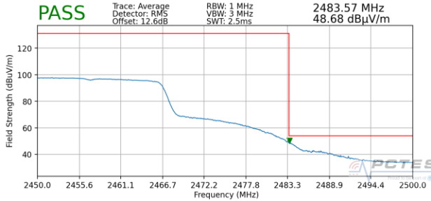
Plot 7-135. Radiated Restricted Upper Band Edge Measurement MIMO (Average)
