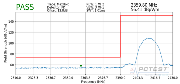
Plot 7-124. Radiated Restricted Lower Band Edge Measurement SISO ANT2 (Peak)
