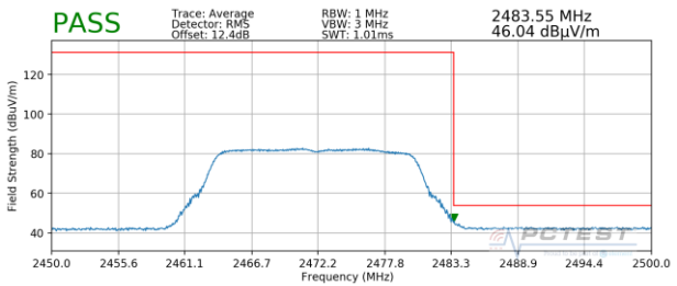
Plot 7-141. Radiated Restricted Upper Band Edge Measurement MIMO (Average)
