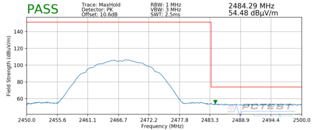
Plot 7-128. Radiated Restricted Upper Band Edge Measurement SISO ANT2 (Peak)
