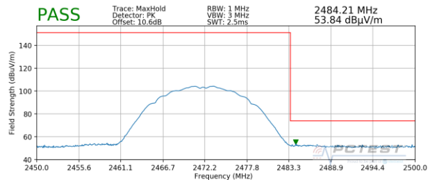
Plot 7-130. Radiated Restricted Upper Band Edge Measurement SISO ANT2 (Peak)
