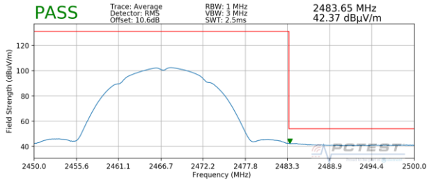
Plot 7-127. Radiated Restricted Upper Band Edge Measurement SISO ANT2 (Average)
