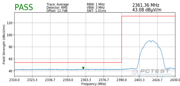
Plot 7-115. Radiated Restricted Lower Band Edge Measurement SISO ANT1 (Average)
