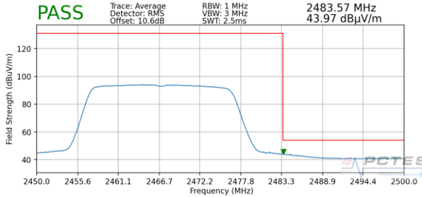
Plot 7-139. Radiated Restricted Upper Band Edge Measurement MIMO (Average)
