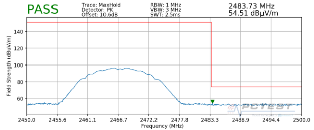
Plot 7-120. Radiated Restricted Upper Band Edge Measurement SISO ANT1 (Peak)
