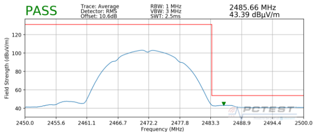
Plot 7-129. Radiated Restricted Upper Band Edge Measurement SISO ANT2 (Average)
