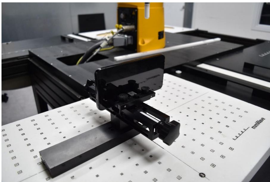
Left View of the DUT
