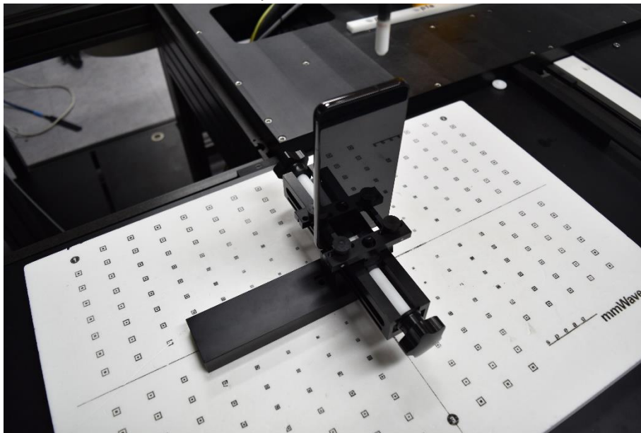
Top View of the DUT
