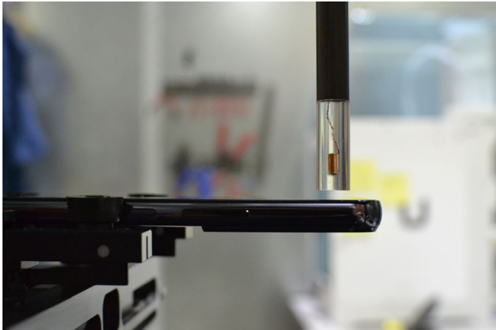
Figure 14-2 Test Setup for Wireless Device
