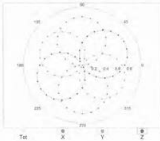
f=600 MHz,TEM
