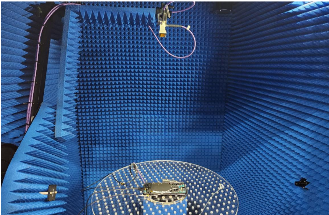
Test Setup Photo 16 – sub6 NR + mmW Power Measurement Setup (Figure 7-2)
