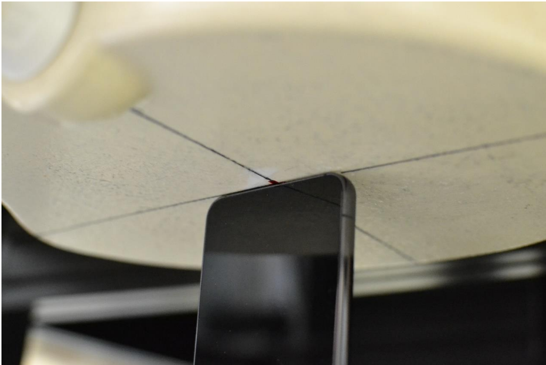
Test Setup Photo 15 – Body, Bottom Edge at 0 mm
