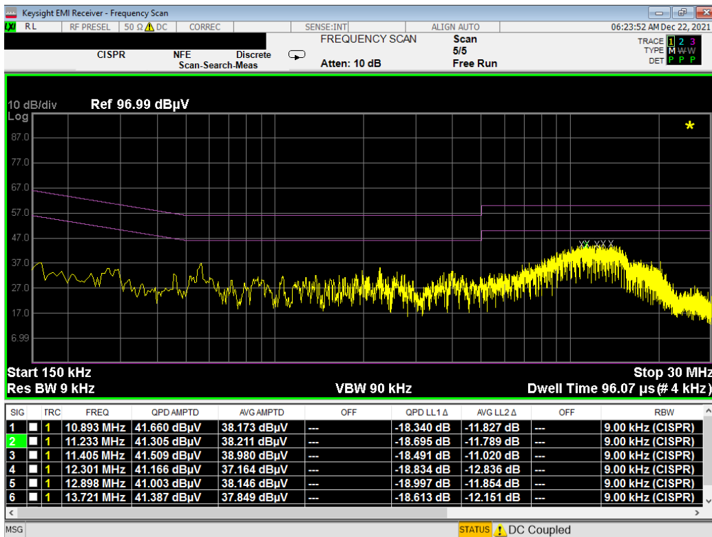
Plot 7-8. Line-Conducted Test Plot (N) - Device to Device WPT- Config 1
