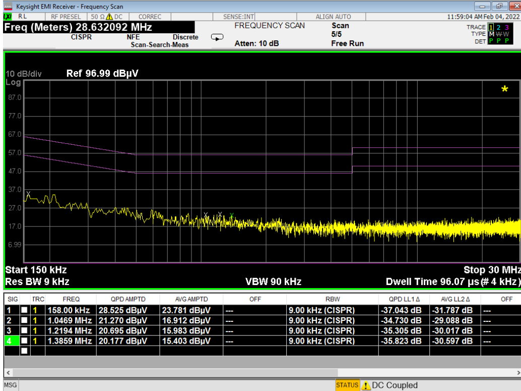
Plot 7-9. Line-Conducted Test Plot (L1) - Device to Device WPT- Config 2
