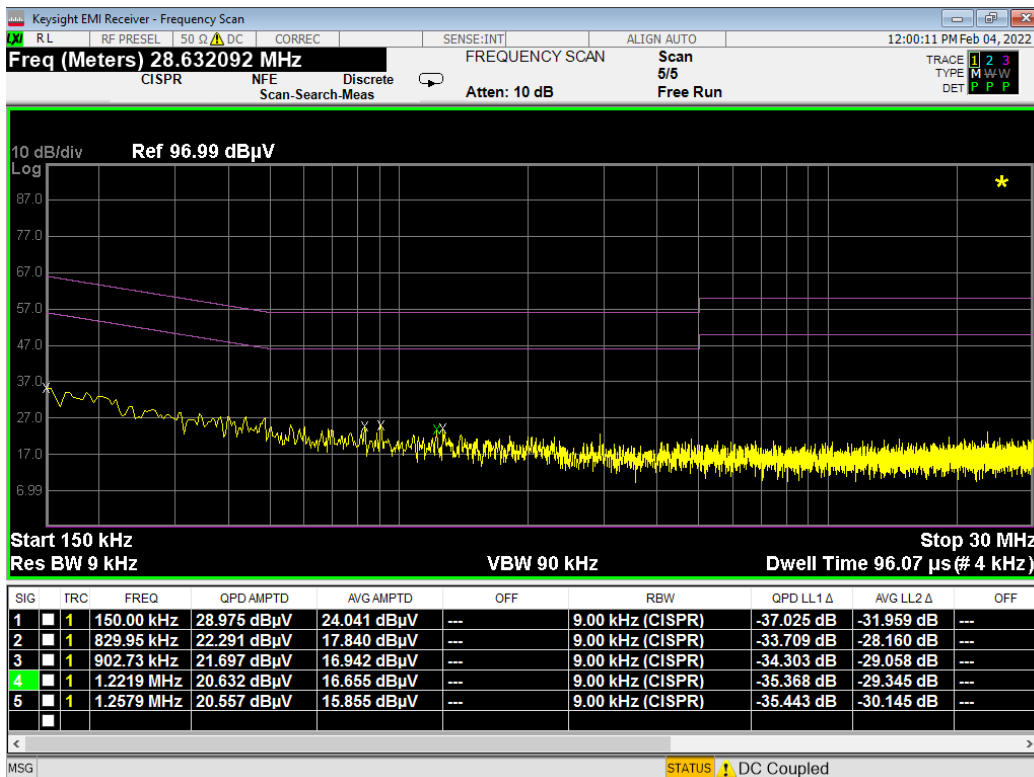
Plot 7-10. Line-Conducted Test Plot (N) - Device to Device WPT- Config 2
