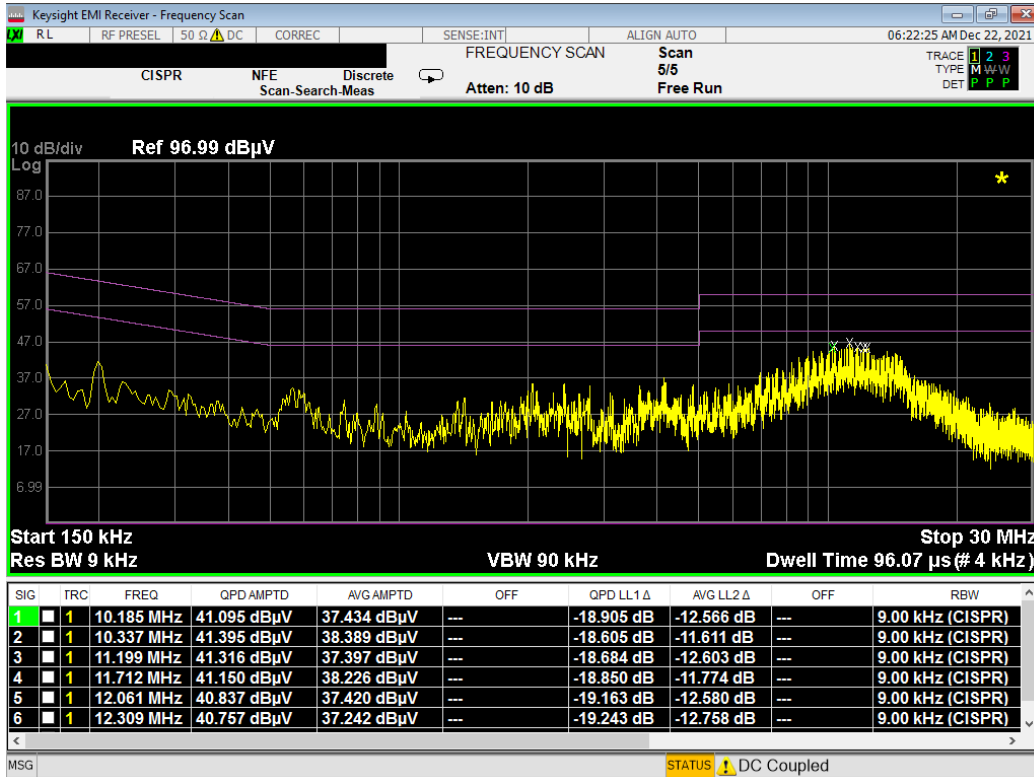
Plot 7-7. Line-Conducted Test Plot (L1) - Device to Device WPT- Config 1
