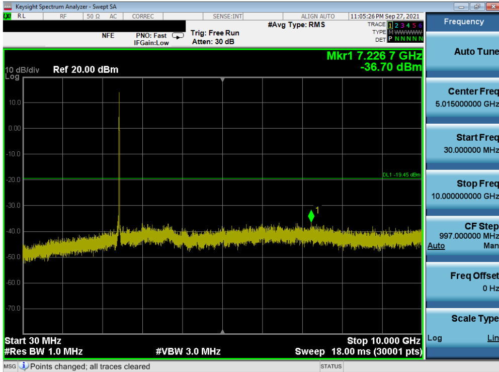
Plot 7-111. Conducted Spurious Plot SISO ANT1 (802.11b – Ch. 6)
