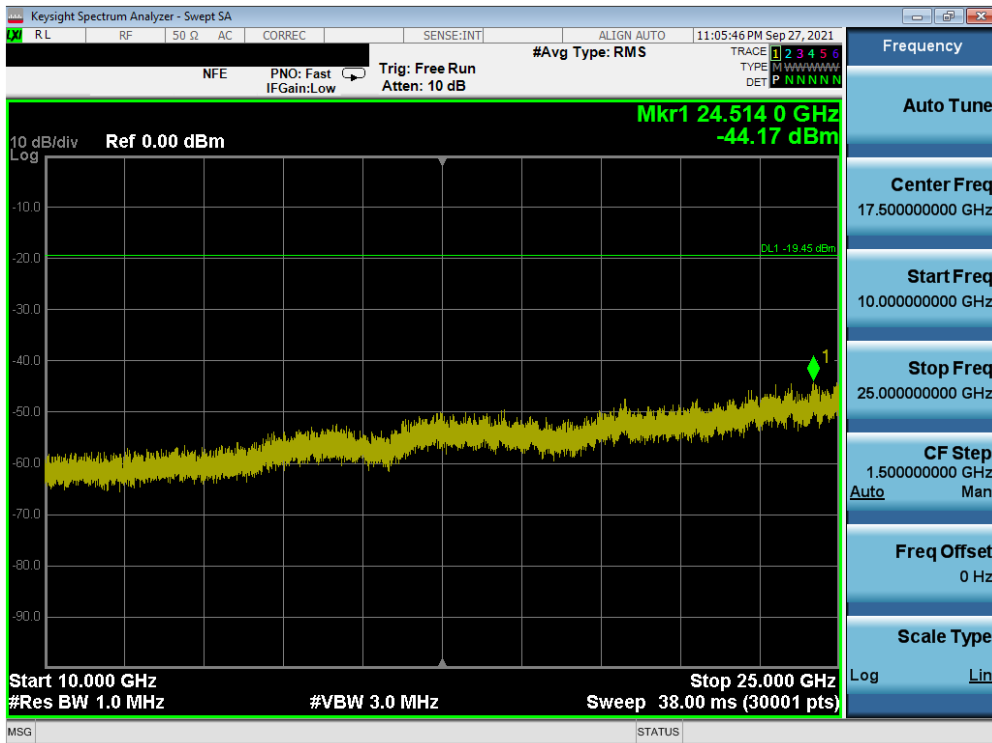
Plot 7-112. Conducted Spurious Plot SISO ANT1 (802.11b – Ch. 6)
