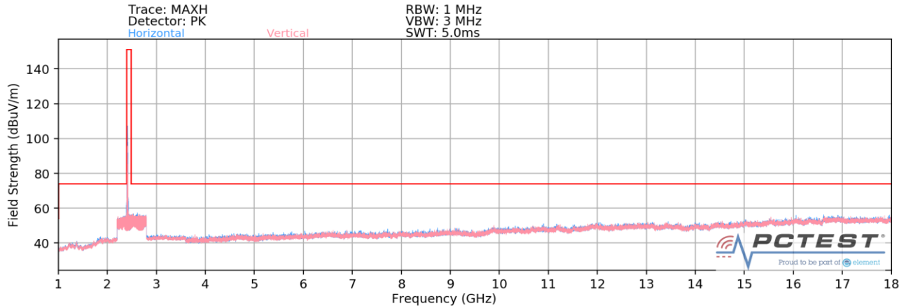
Plot 7-121. Radiated Spurious Plot above 1GHz SISO ANT1 (802.11b – Ch. 1)
