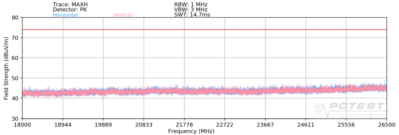
Plot 7-124. Radiated Spurious Plot above 18GHz SISO ANT1
