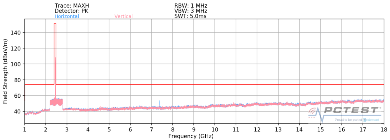
Plot 7-131. Radiated Spurious Plot above 1GHz MIMO/CDD (802.11g – Ch. 11)
