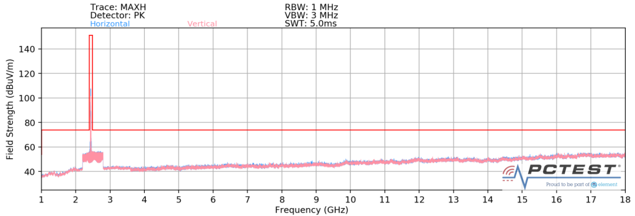
Plot 7-122. Radiated Spurious Plot above 1GHz SISO ANT1 (802.11b – Ch. 6)
