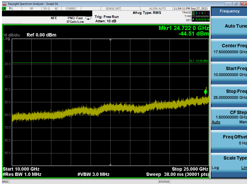
Plot 7-110. Conducted Spurious Plot SISO ANT1 (802.11b – Ch. 1)
