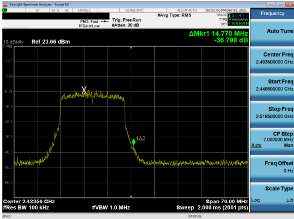
Plot 7-108. Band Edge Plot SISO ANT2 (802.11ax (2.4GHz) – Ch. 13)
