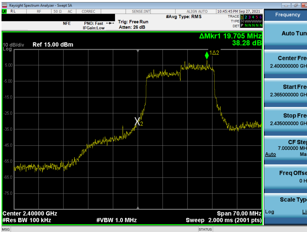
Plot 7-86. Band Edge Plot SISO ANT1 (802.11ax (2.4GHz) – Ch. 1)
