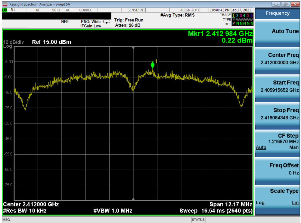
Plot 7-49. Power Spectral Density Plot MIMO ANT1 (802.11b (2.4GHz) – Ch. 1)
