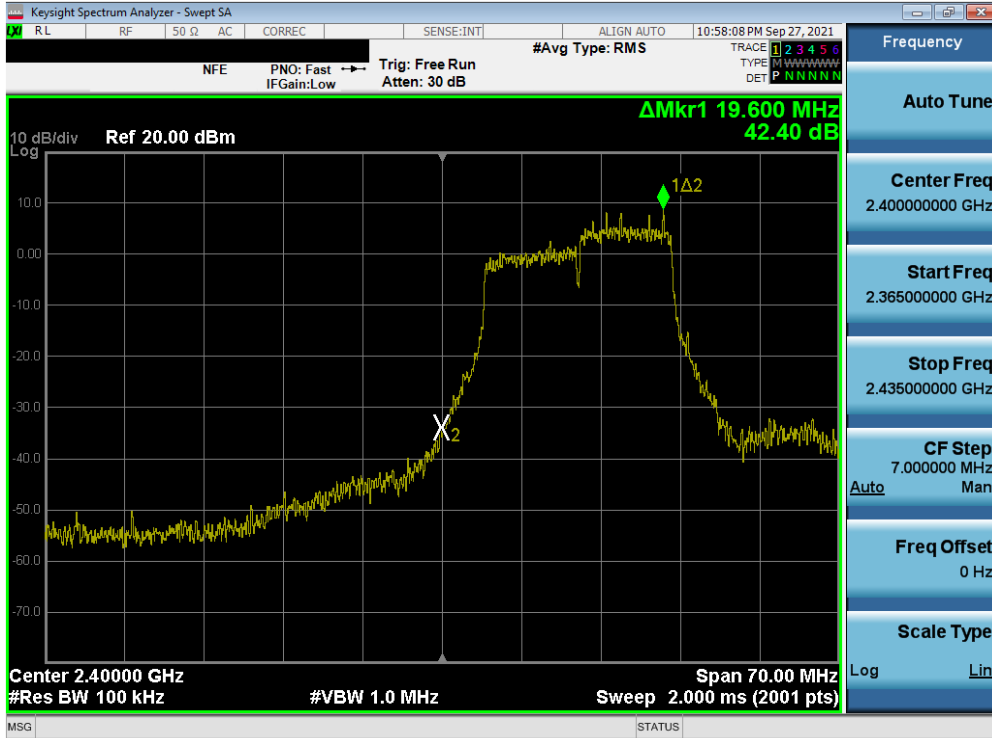
Plot 7-77. Band Edge Plot SISO ANT1 (802.11g- Ch. 1)
