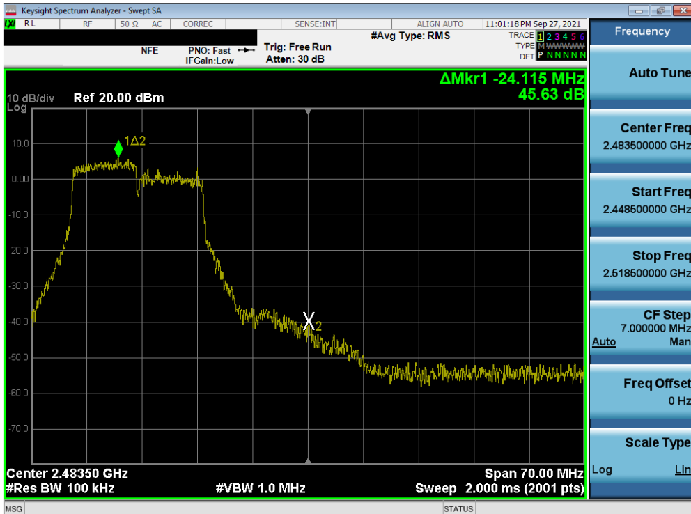
Plot 7-78. Band Edge Plot SISO ANT1 (802.11g - Ch. 11)
