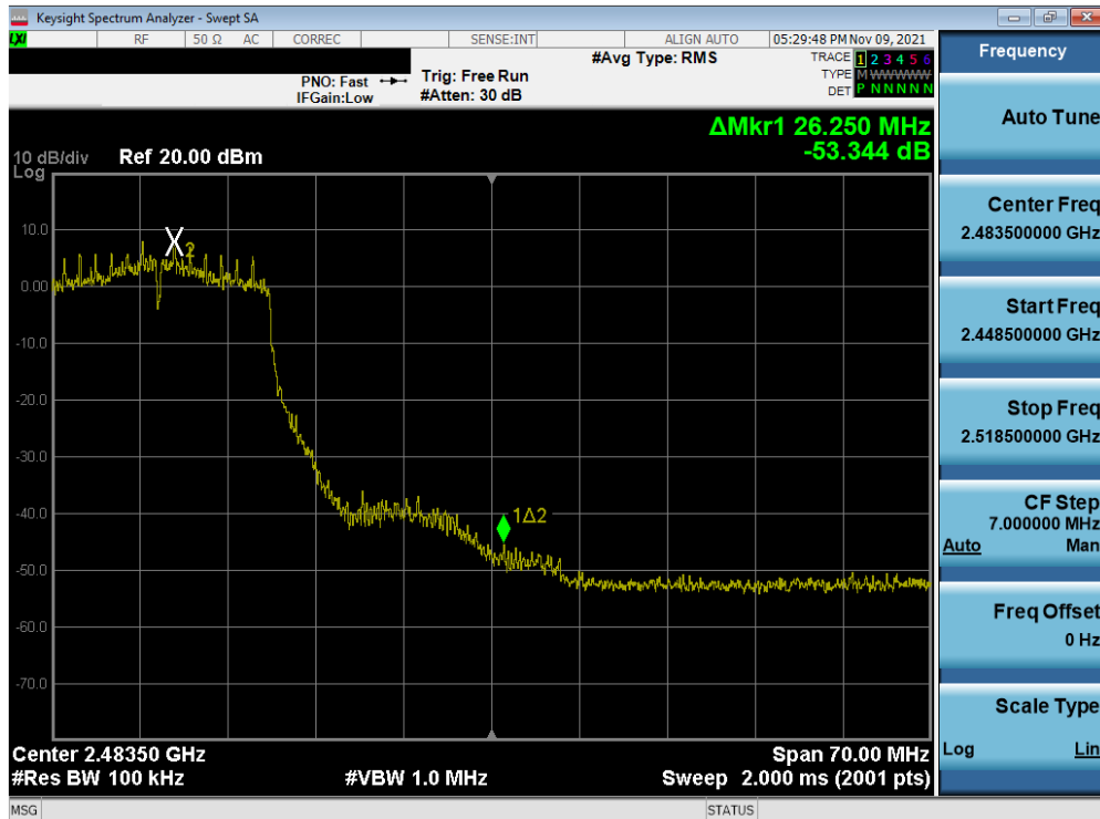
Plot 7-82. Band Edge Plot SISO ANT1 (802.11n (2.4GHz) – Ch. 10)
