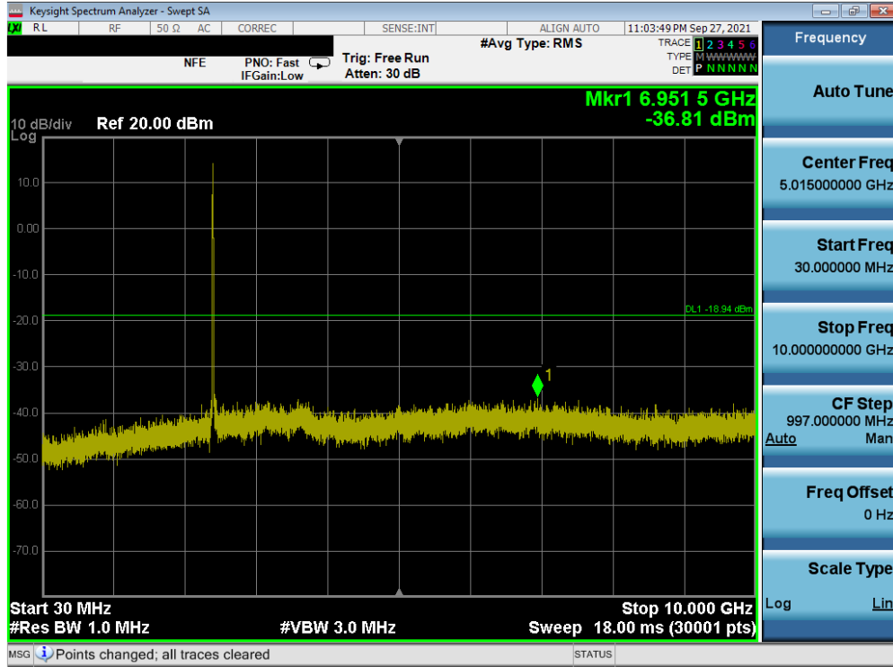
Plot 7-109. Conducted Spurious Plot SISO ANT1 (802.11b – Ch. 1)
