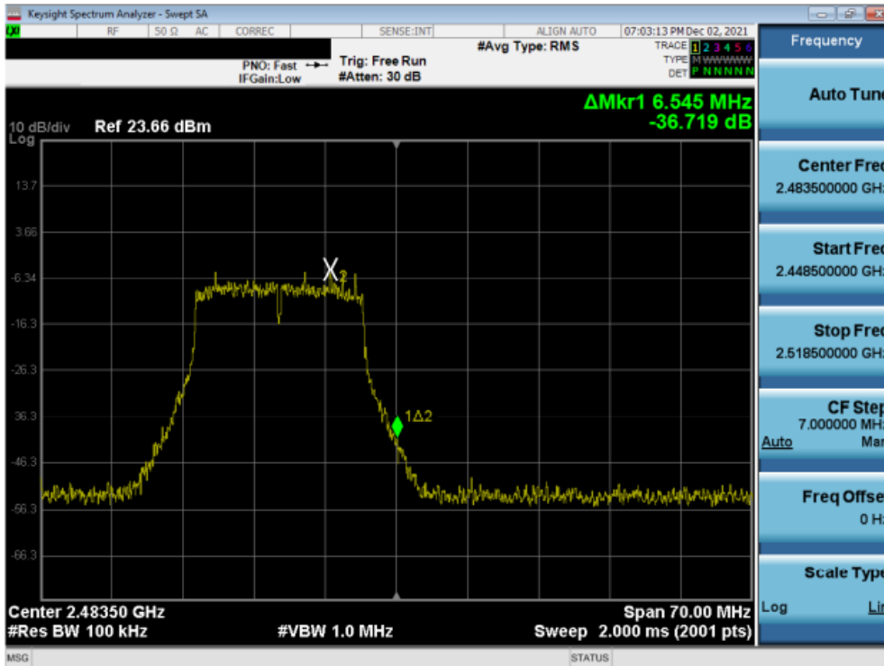
Plot 7-98. Band Edge Plot SISO ANT2 (802.11g – Ch. 13)
