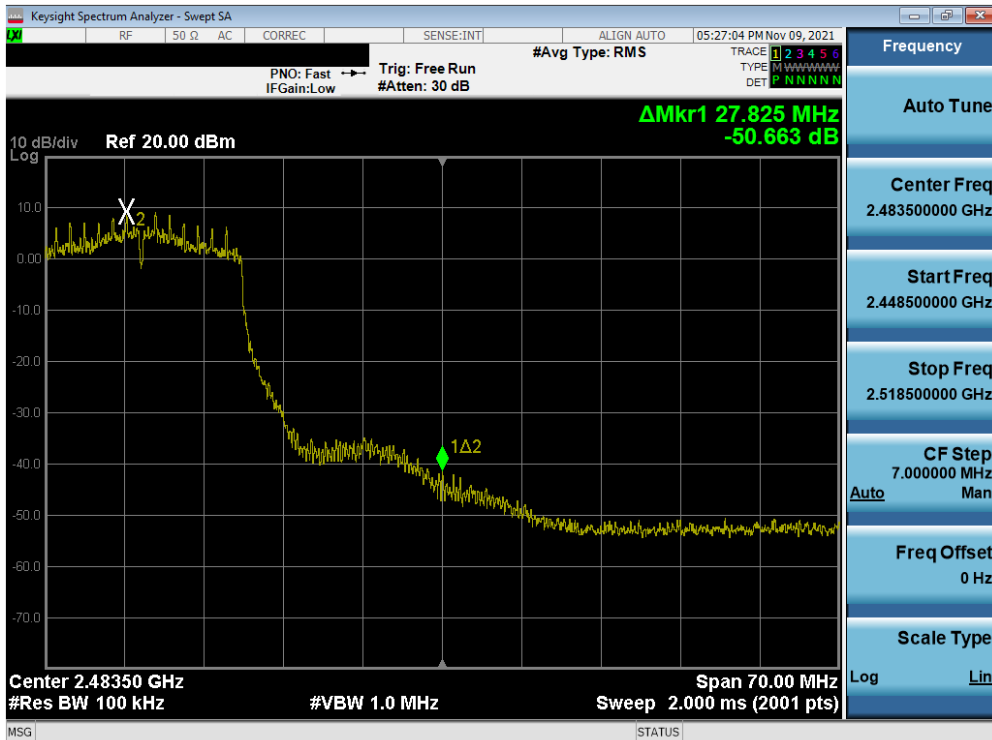
Plot 7-100. Band Edge Plot SISO ANT2 (802.11n (2.4GHz) – Ch. 10)
