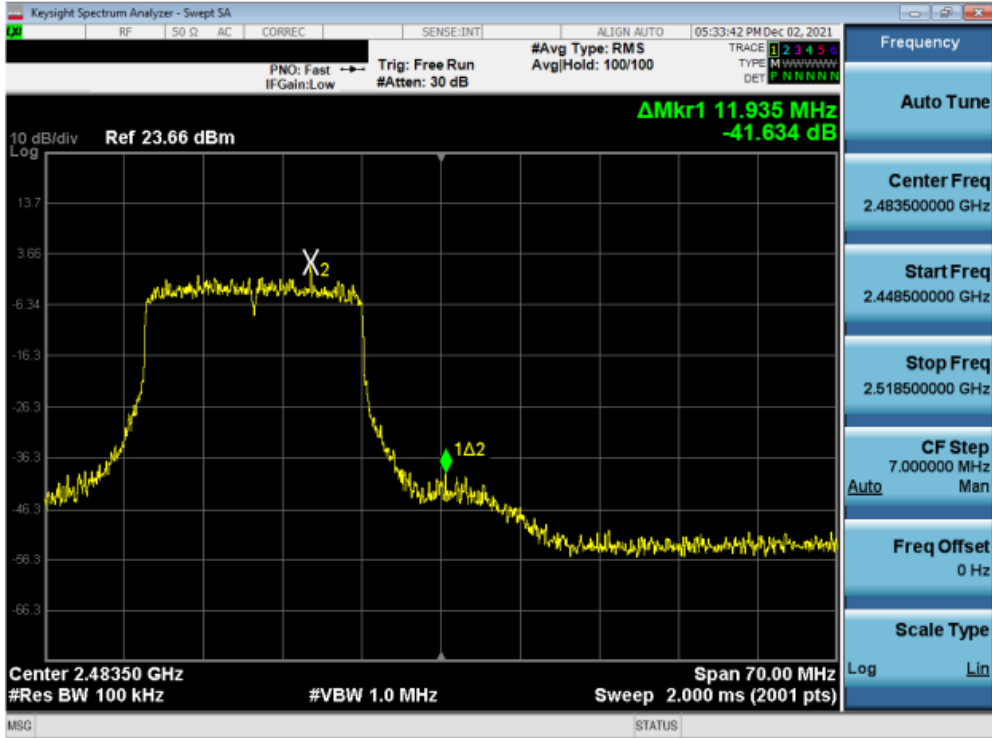
Plot 7-107. Band Edge Plot SISO ANT2 (802.11ax (2.4GHz) – Ch. 12)
