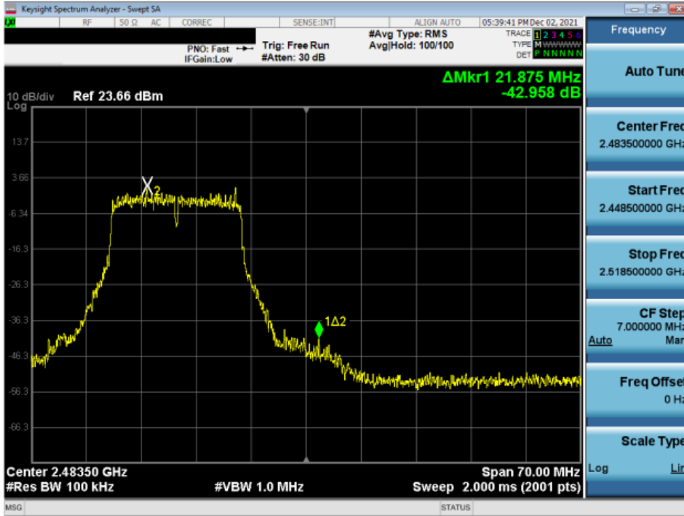
Plot 7-97. Band Edge Plot SISO ANT2 (802.11g – Ch. 12)
