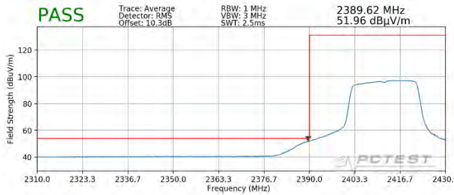
Plot 7-99. Radiated Restricted Lower Band Edge Measurement SISO ANT1 (Average – 242 Tones)
