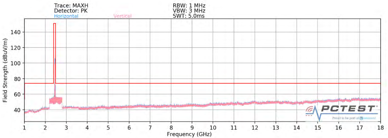
Plot 7-72. Radiated Spurious Plot above 1GHz SISO ANT1 (802.11ax OFDMA – 242 Tones – Ch. 11)
