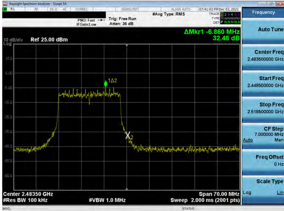
Plot 7-33. Band Edge Plot SISO ANT1 (802.11ax OFDMA – 242 Tones – Ch. 13)
