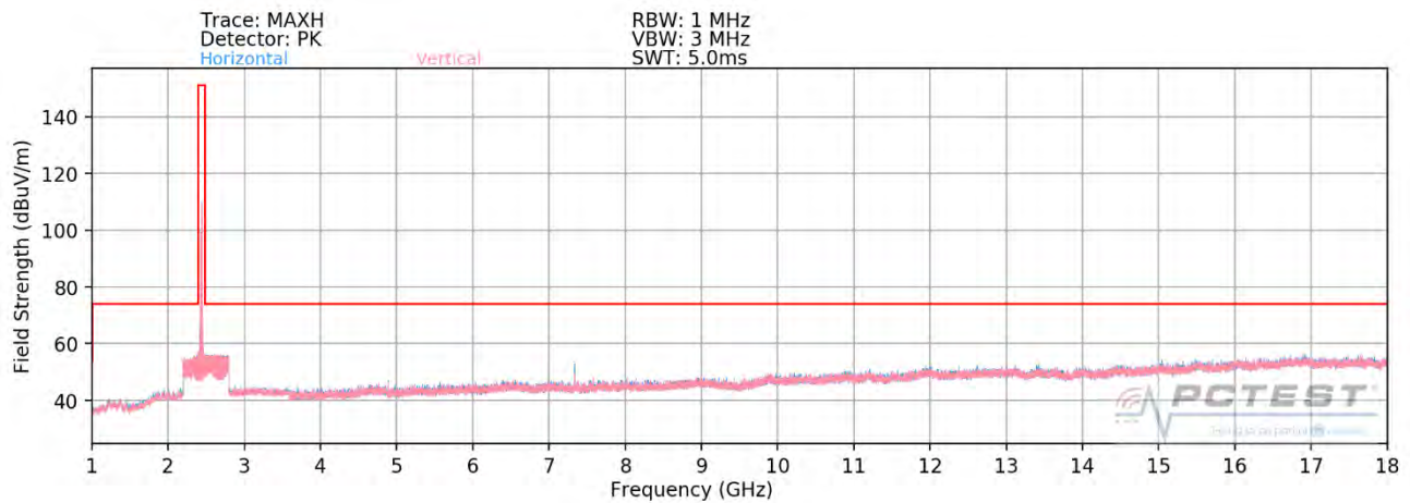
Plot 7-76. Radiated Spurious Plot above 1GHz SISO ANT2 (802.11ax OFDMA – 106 Tones – Ch. 6)
