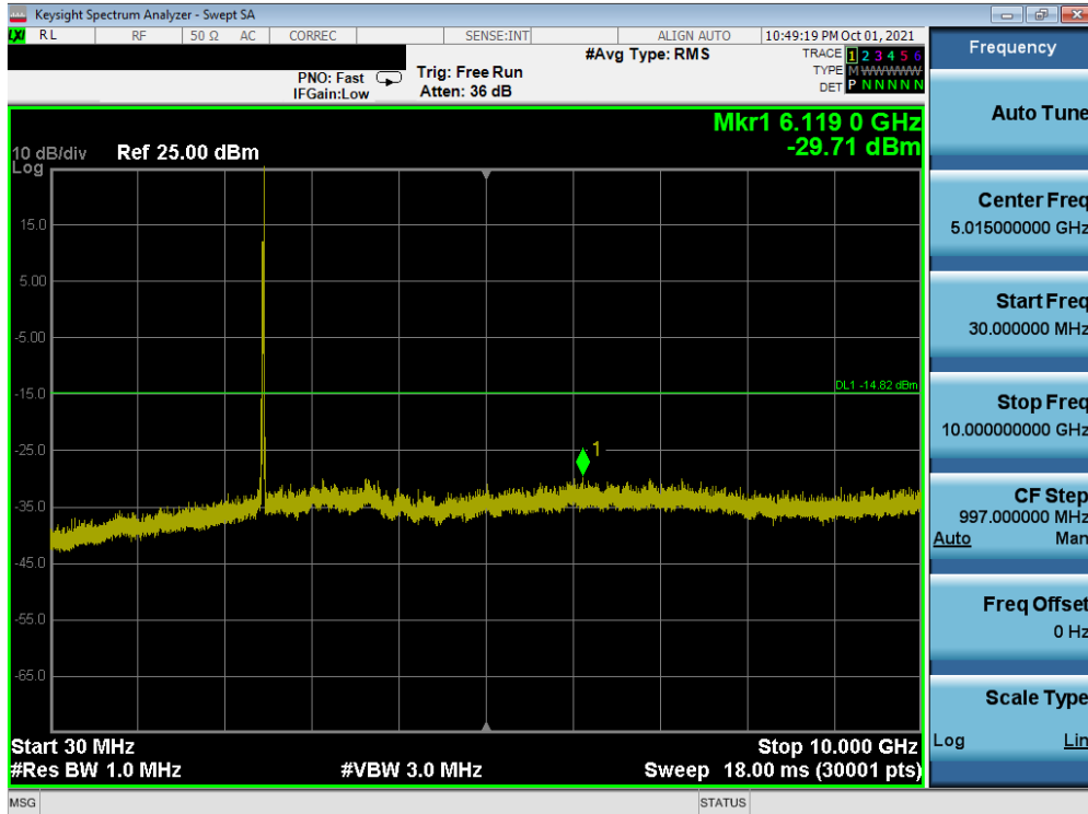
Plot 7-47. Conducted Spurious Plot SISO ANT1 (802.11ax OFDMA – 26 Tones – Ch. 11)
