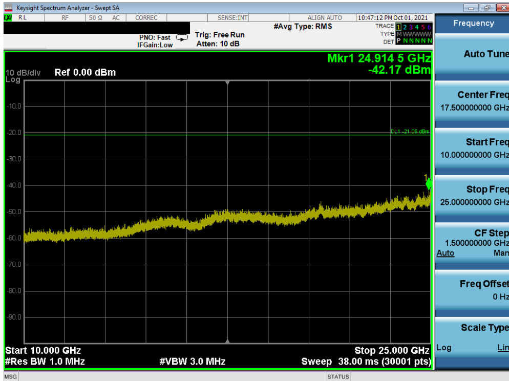
Plot 7-52. Conducted Spurious Plot SISO ANT1 (802.11ax OFDMA – 242 Tones – Ch. 6)
