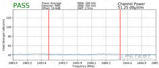
Plot 7-121. Radiated Restricted Upper Band Edge Measurement SISO ANT2 (Average – 242 Tones)
