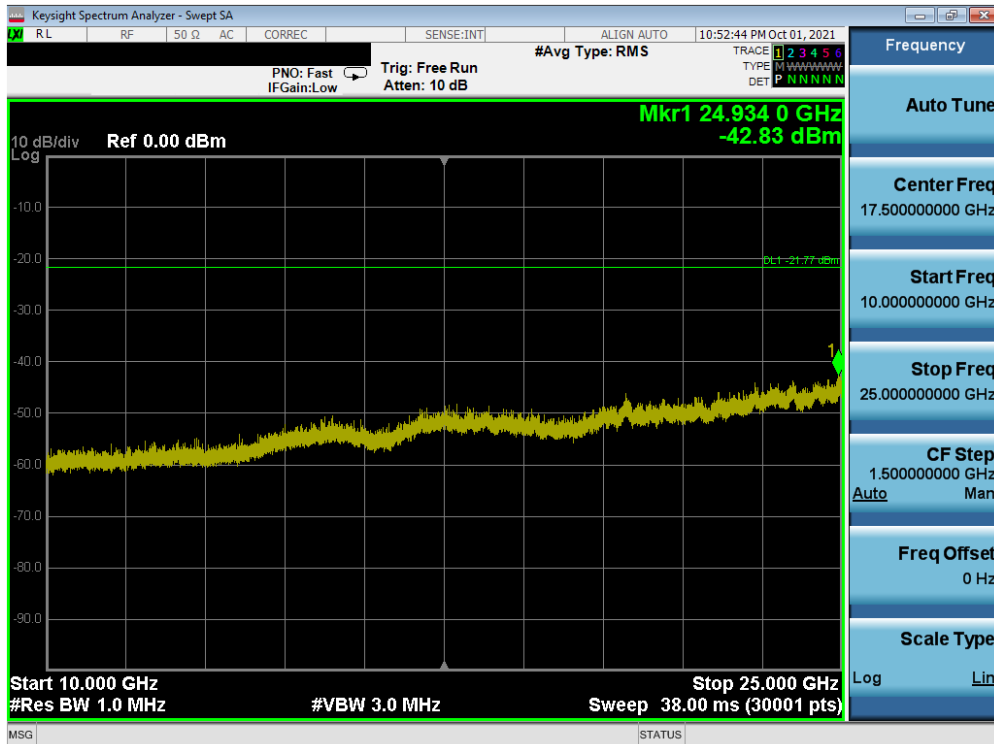
Plot 7-54. Conducted Spurious Plot SISO ANT1 (802.11ax OFDMA – 242 Tones – Ch. 11)
