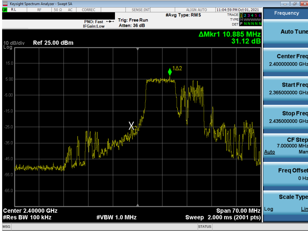
Plot 7-34. Band Edge Plot SISO ANT2 (802.11ax OFDMA – 106 Tones – Ch. 1)
