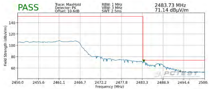
Plot 7-138. Radiated Restricted Upper Band Edge Measurement MIMO (Peak – 242 Tones)
