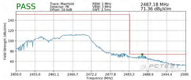
Plot 7-130. Radiated Restricted Upper Band Edge Measurement MIMO (Peak – 106 Tones)
