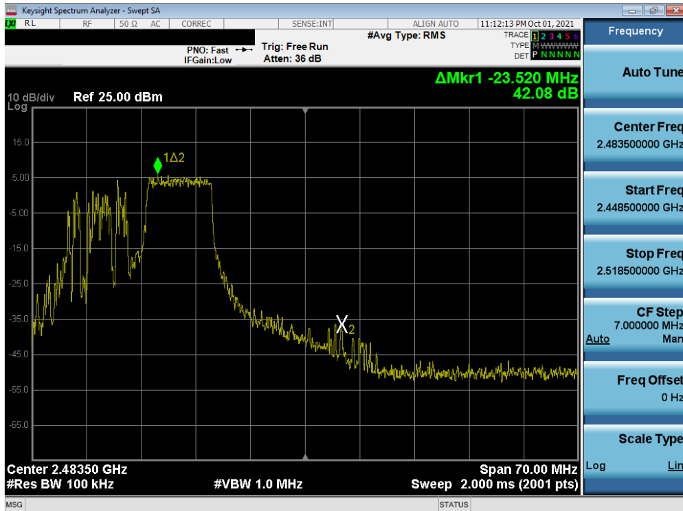
Plot 7-35. Band Edge Plot SISO ANT2 (802.11ax OFDMA – 106 Tones – Ch. 11)
