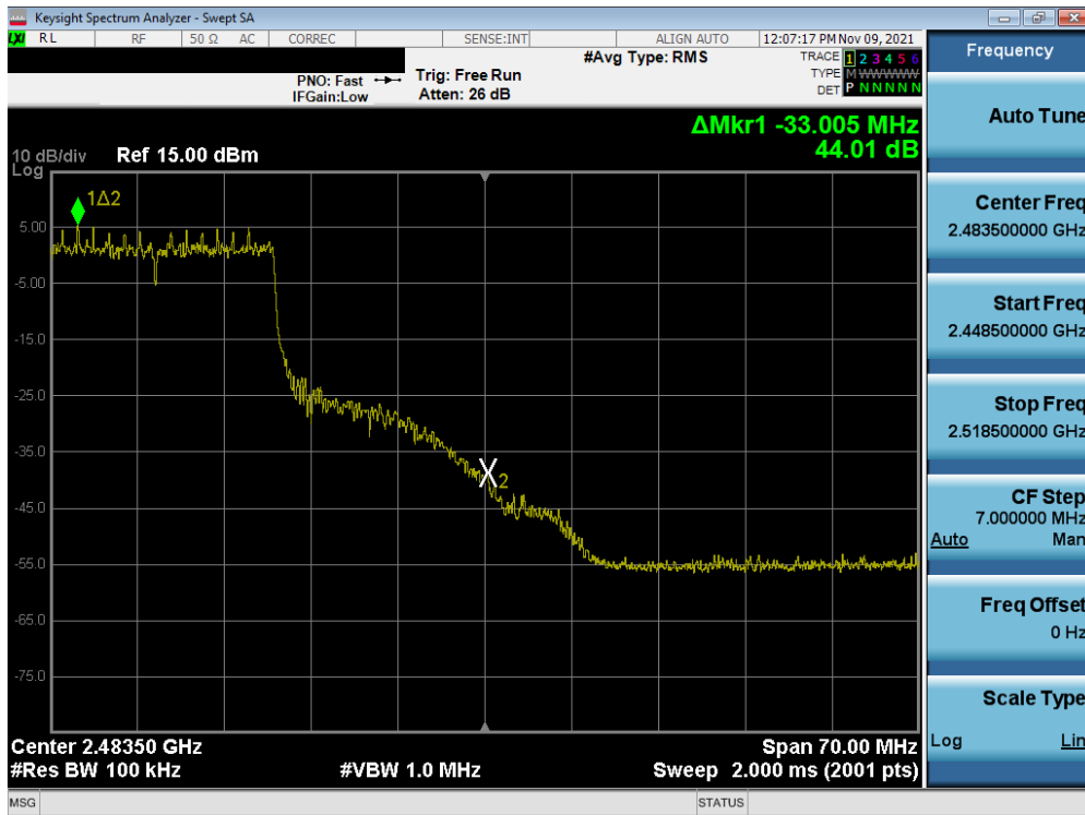
Plot 7-30. Band Edge Plot SISO ANT1 (802.11ax OFDMA – 242 Tones – Ch. 10)
