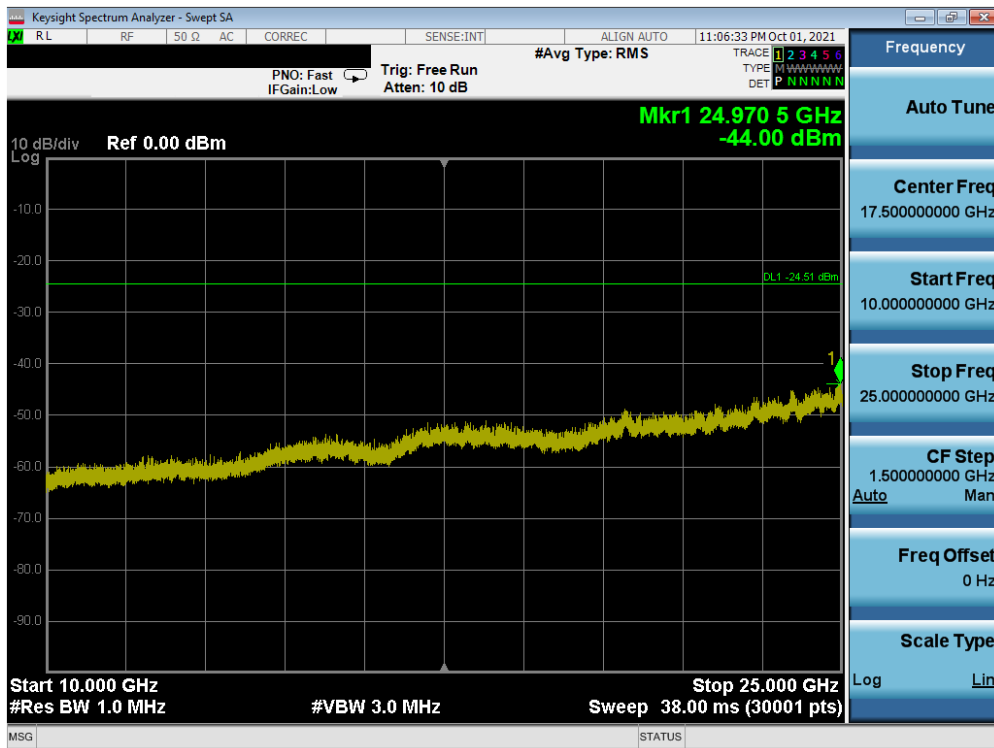
Plot 7-62. Conducted Spurious Plot SISO ANT2 (802.11ax OFDMA – 242 Tones – Ch. 1)
