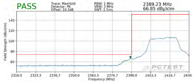
Plot 7-100. Radiated Restricted Lower Band Edge Measurement SISO ANT1 (Peak – 242 Tones)
