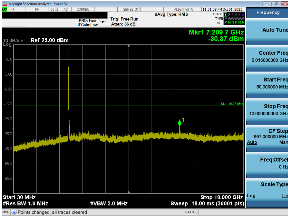
Plot 7-55. Conducted Spurious Plot SISO ANT2 (802.11ax OFDMA – 26 Tones – Ch. 1)
