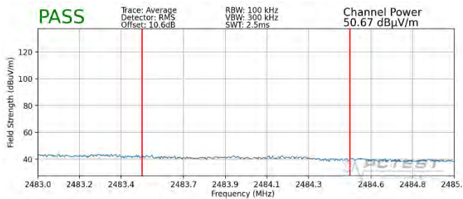
Plot 7-137. Radiated Restricted Upper Band Edge Measurement MIMO (Average – 242 Tones)
