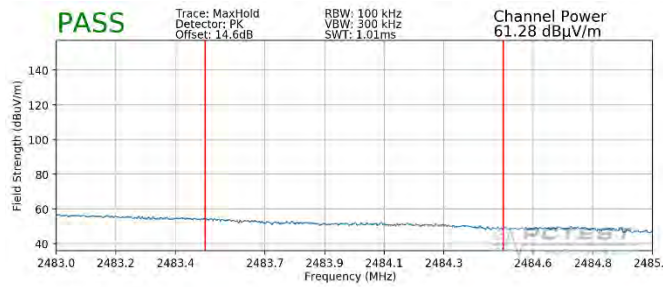
Plot 7-144. Radiated Restricted Upper Band Edge Measurement MIMO (Peak – 242 Tones)
