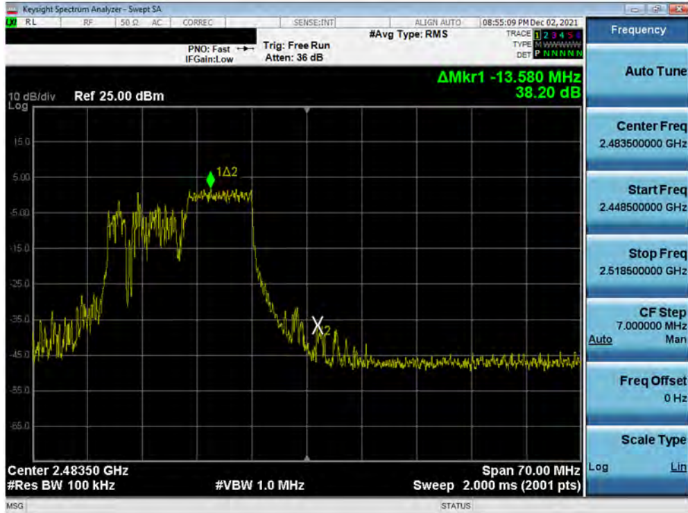
Plot 7-36. Band Edge Plot SISO ANT2 (802.11ax OFDMA – 106 Tones – Ch. 12)
