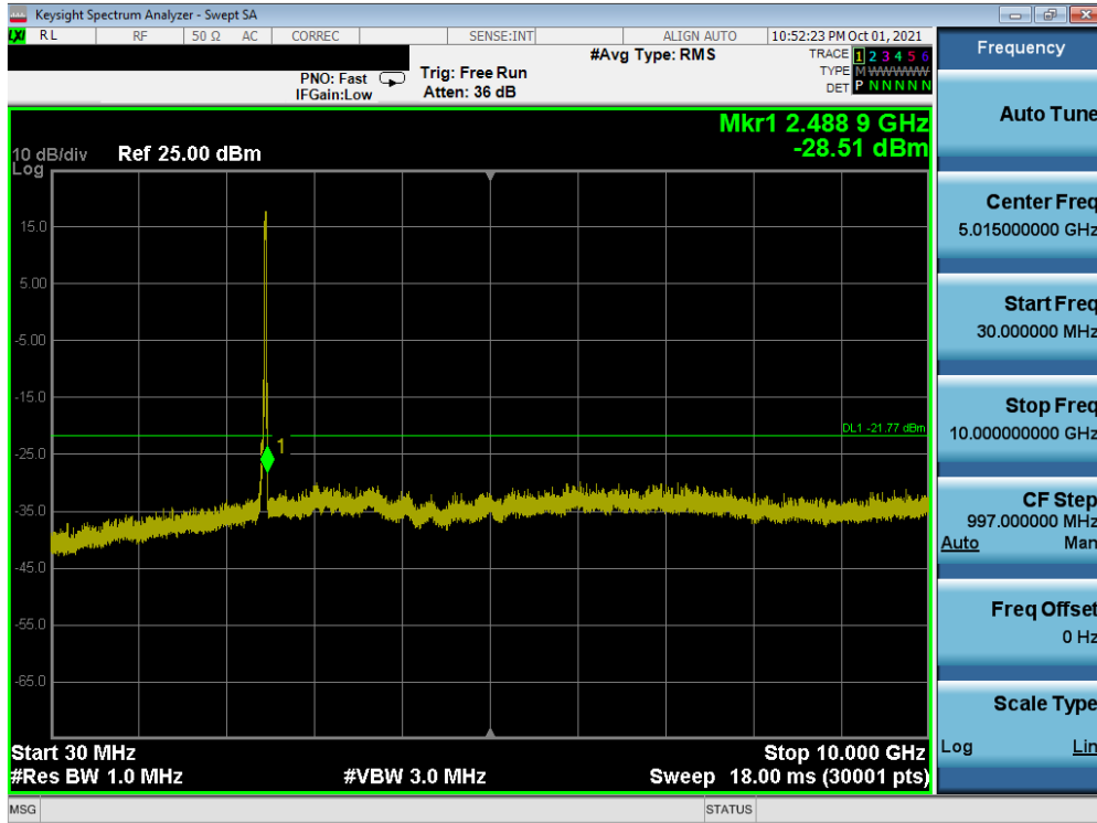
Plot 7-53. Conducted Spurious Plot SISO ANT1 (802.11ax OFDMA – 242 Tones – Ch. 11)
