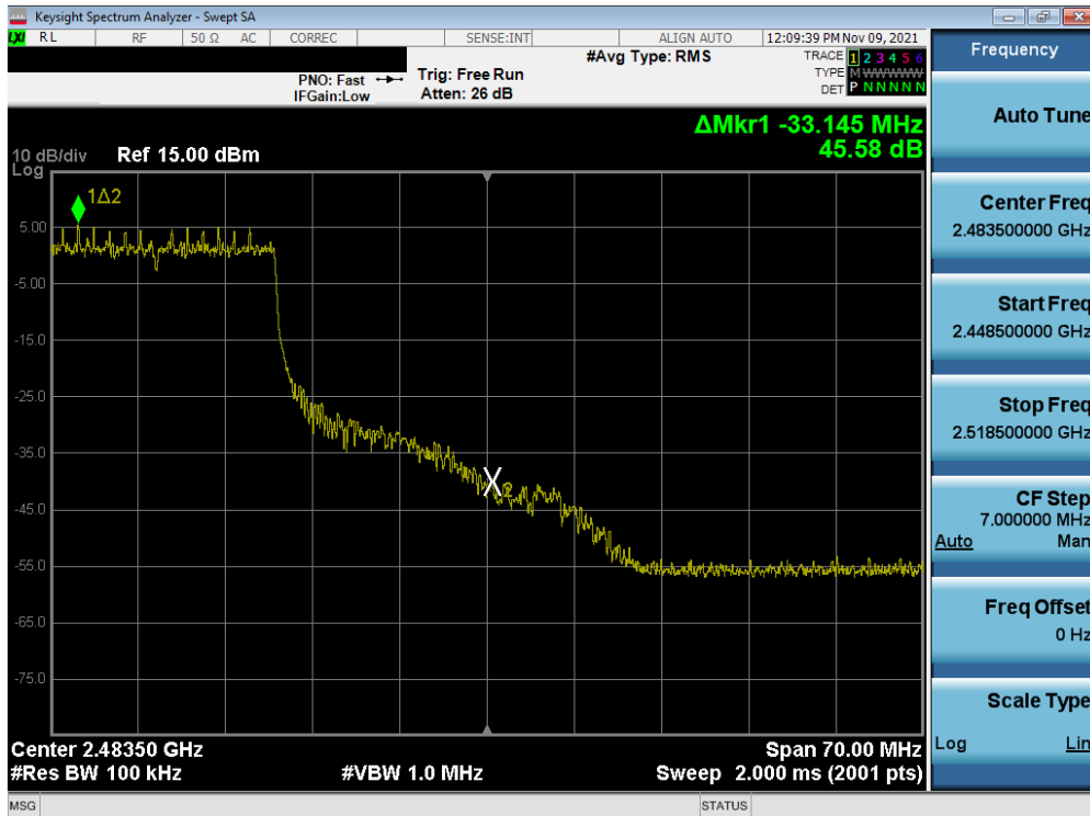
Plot 7-39. Band Edge Plot SISO ANT2 (802.11ax OFDMA – 242 Tones – Ch. 10)
