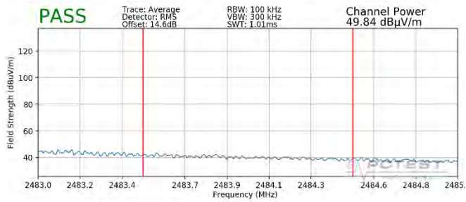
Plot 7-143. Radiated Restricted Upper Band Edge Measurement MIMO (Average – 242 Tones)
