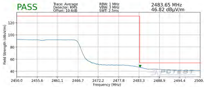
Plot 7-119. Radiated Restricted Upper Band Edge Measurement SISO ANT2 (Average – 242 Tones)
