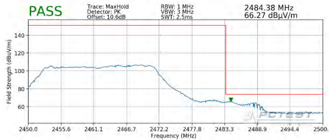
Plot 7-104. Radiated Restricted Upper Band Edge Measurement SISO ANT1 (Peak – 242 Tones)
