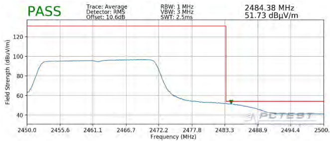
Plot 7-103. Radiated Restricted Upper Band Edge Measurement SISO ANT1 (Average – 242 Tones)
