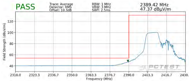
Plot 7-127. Radiated Restricted Lower Band Edge Measurement MIMO (Average – 106 Tones)
