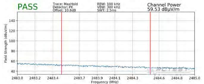
Plot 7-116. Radiated Restricted Upper Band Edge Measurement SISO ANT2 (Peak – 106 Tones)
