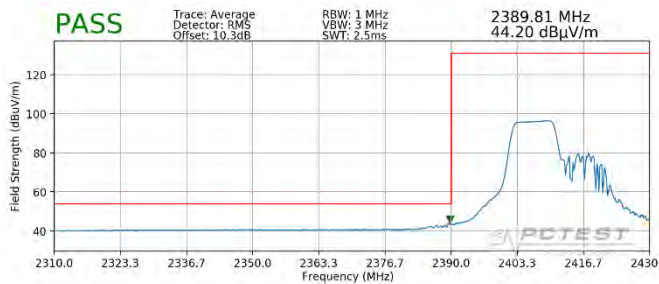
Plot 7-109. Radiated Restricted Lower Band Edge Measurement SISO ANT2 (Average – 106 Tones)
