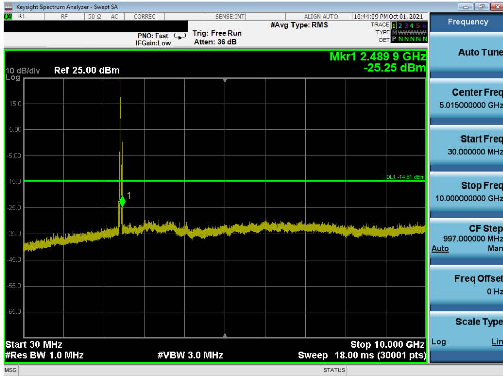
Plot 7-45. Conducted Spurious Plot SISO ANT1 (802.11ax OFDMA – 26 Tones – Ch. 6)
