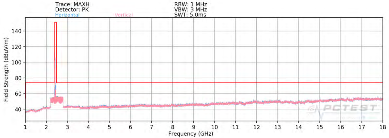
Plot 7-67. Radiated Spurious Plot above 1GHz SISO ANT1 (802.11ax OFDMA – 106 Tones – Ch. 1)
