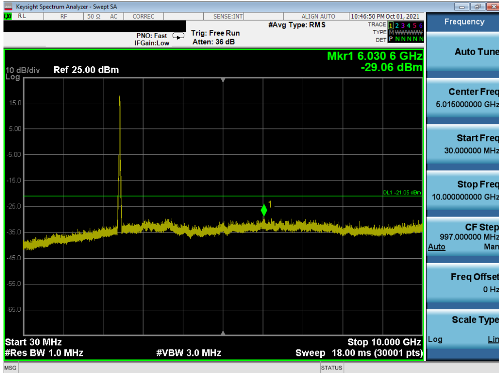
Plot 7-51. Conducted Spurious Plot SISO ANT1 (802.11ax OFDMA – 242 Tones – Ch. 6)
