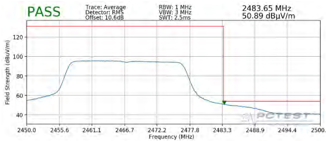
Plot 7-105. Radiated Restricted Upper Band Edge Measurement SISO ANT1 (Average – 242 Tones)
