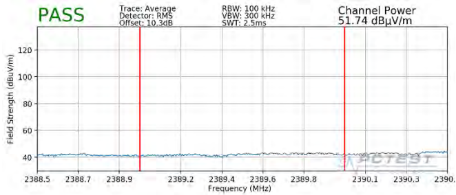
Plot 7-135. Radiated Restricted Lower Band Edge Measurement MIMO (Average – 242 Tones)
