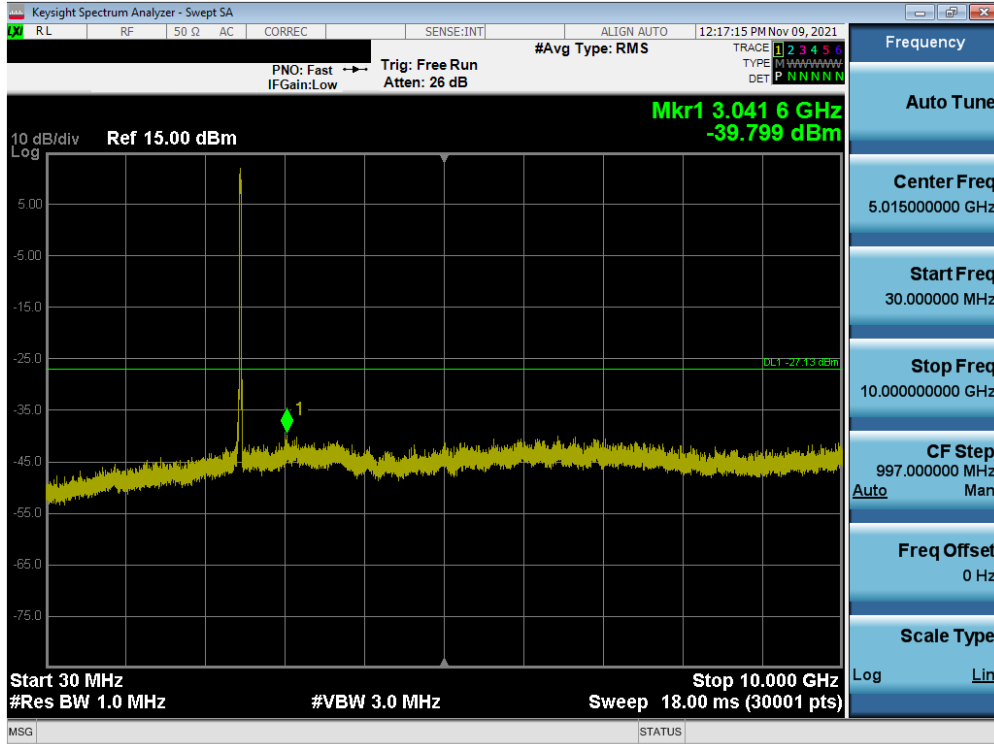
Plot 7-65. Conducted Spurious Plot SISO ANT2 (802.11ax OFDMA – 242 Tones – Ch. 11)
