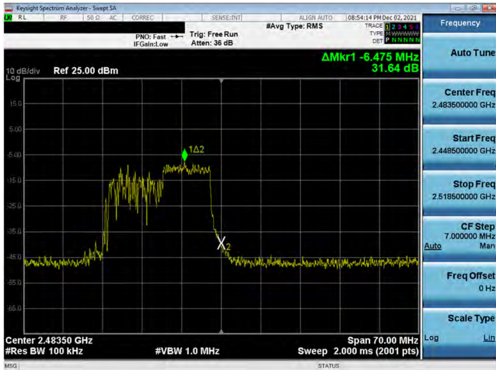
Plot 7-37. Band Edge Plot SISO ANT2 (802.11ax OFDMA – 106 Tones – Ch. 13)
