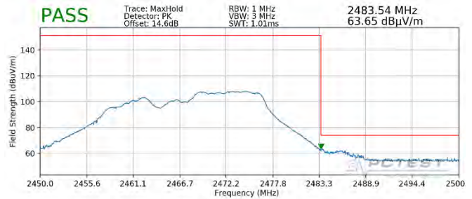
Plot 7-132. Radiated Restricted Upper Band Edge Measurement MIMO (Peak – 106 Tones)
