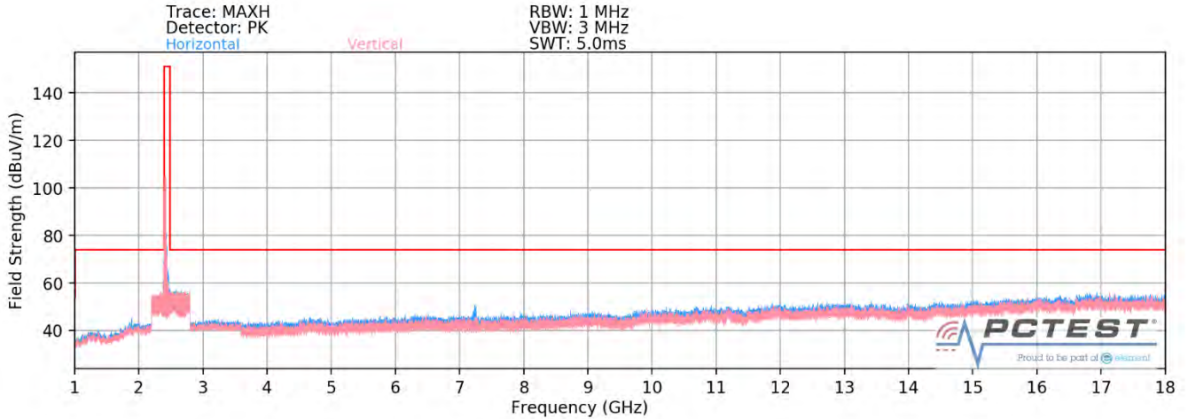
Plot 7-86. Radiated Spurious Plot above 1GHz MIMO (802.11ax OFDMA – 242 Tones – Ch. 1)
