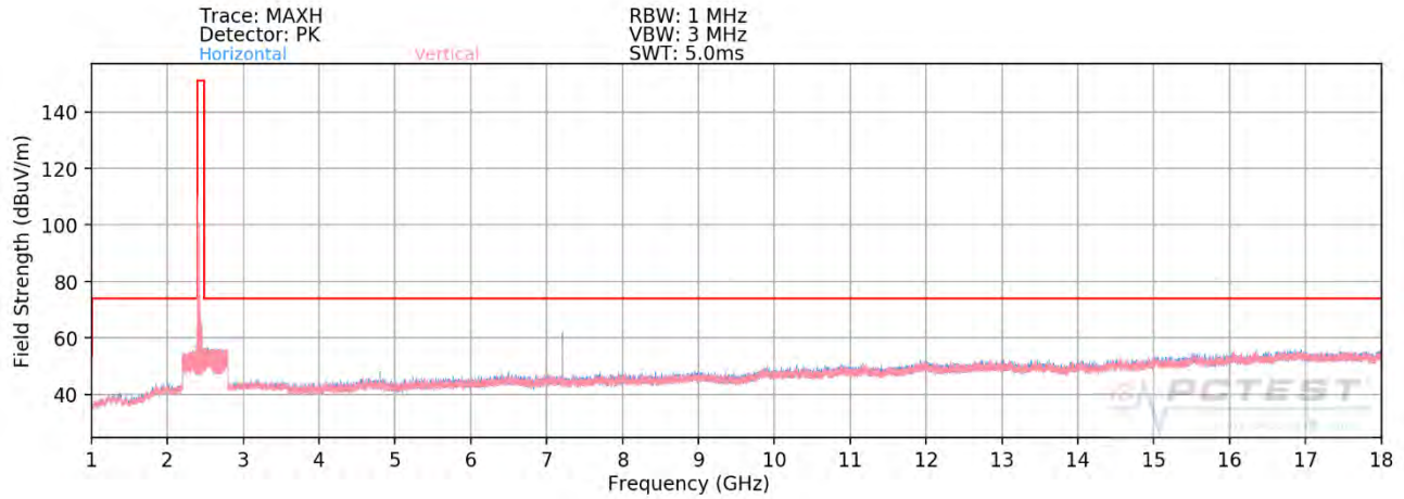
Plot 7-75. Radiated Spurious Plot above 1GHz SISO ANT2 (802.11ax OFDMA – 106 Tones – Ch. 1)
