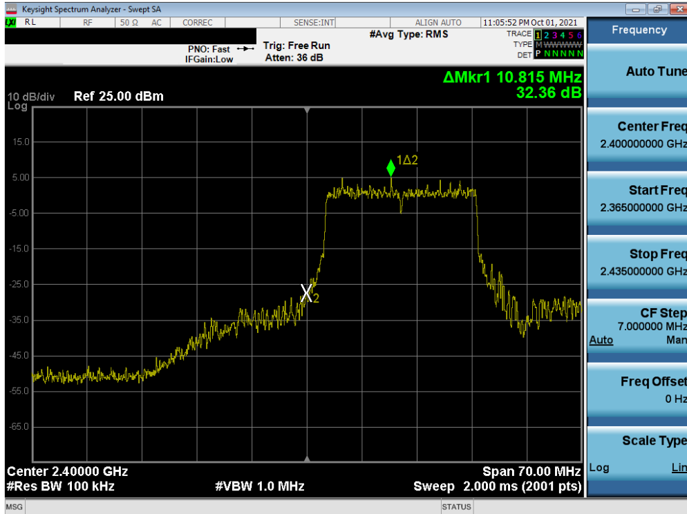
Plot 7-38. Band Edge Plot SISO ANT2 (802.11ax OFDMA – 242 Tones – Ch. 1)
