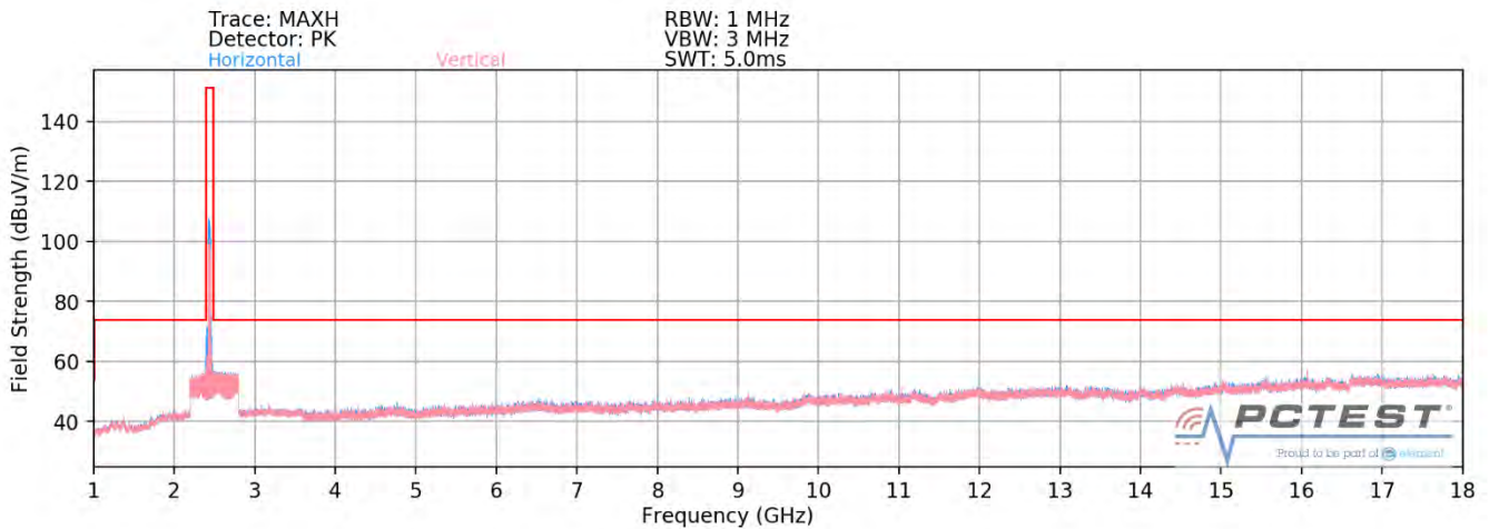
Plot 7-79. Radiated Spurious Plot above 1GHz SISO ANT2 (802.11ax OFDMA – 242 Tones – Ch. 6)
