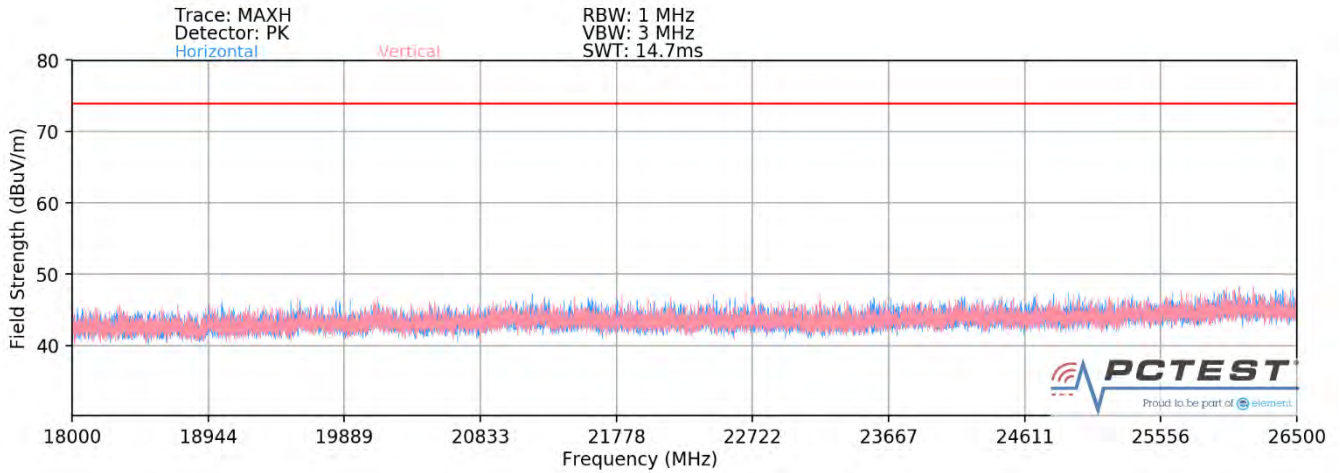
Plot 7-89. Radiated Spurious Plot above 18GHz MIMO (802.11ax OFDMA – 106 Tones)
