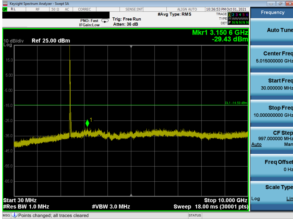
Plot 7-43. Conducted Spurious Plot SISO ANT1 (802.11ax OFDMA – 26 Tones – Ch. 1)
