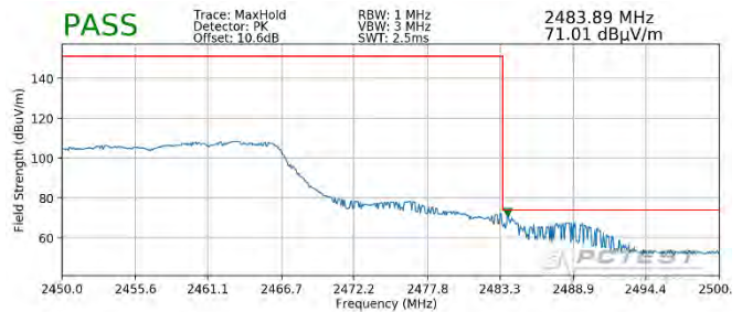
Plot 7-102. Radiated Restricted Upper Band Edge Measurement SISO ANT1 (Peak – 242 Tones)
