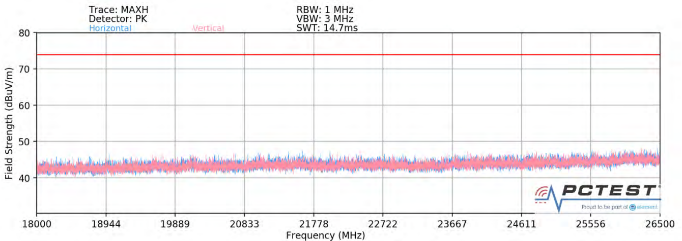
Plot 7-90. Radiated Spurious Plot above 18GHz MIMO (802.11ax OFDMA – 242 Tones)
