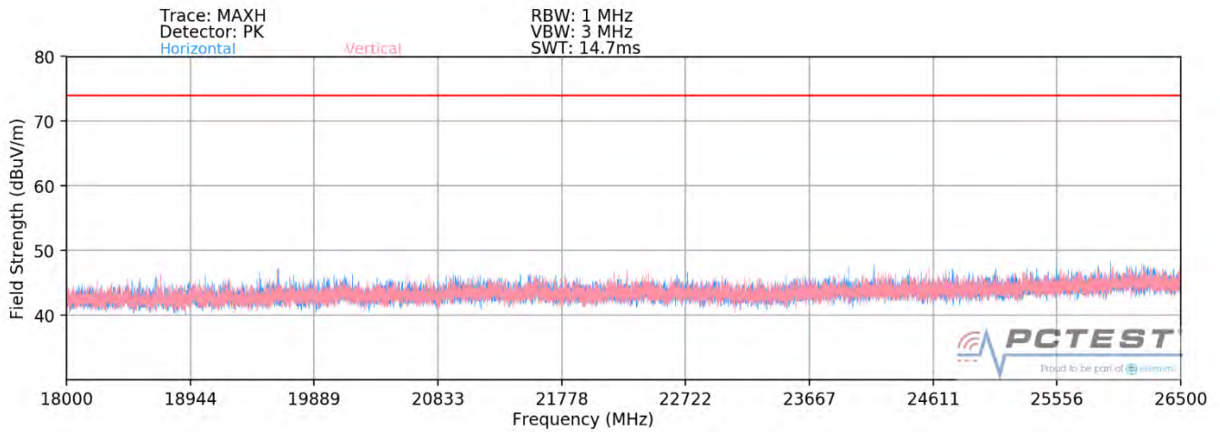
Plot 7-73. Radiated Spurious Plot above 18GHz SISO ANT1 (802.11ax OFDMA – 106 Tones)
