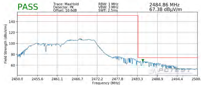
Plot 7-112. Radiated Restricted Upper Band Edge Measurement SISO ANT2 (Peak – 106 Tones)
