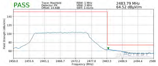
Plot 7-142. Radiated Restricted Upper Band Edge Measurement MIMO (Peak – 242 Tones)
