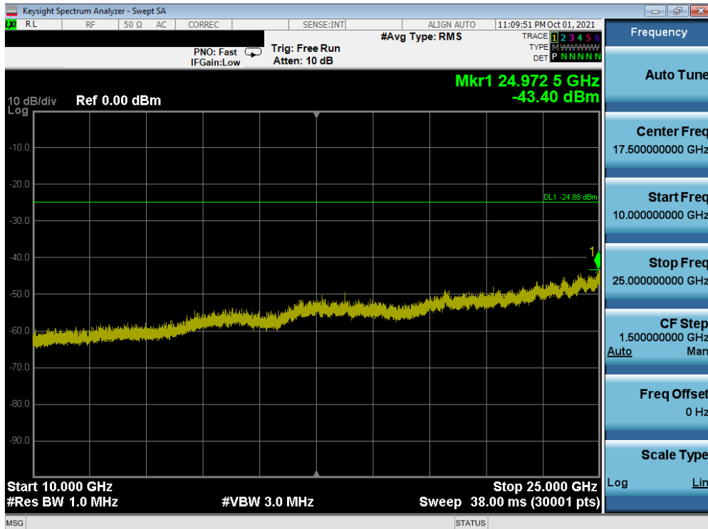
Plot 7-64. Conducted Spurious Plot SISO ANT2 (802.11ax OFDMA – 242 Tones – Ch. 6)
