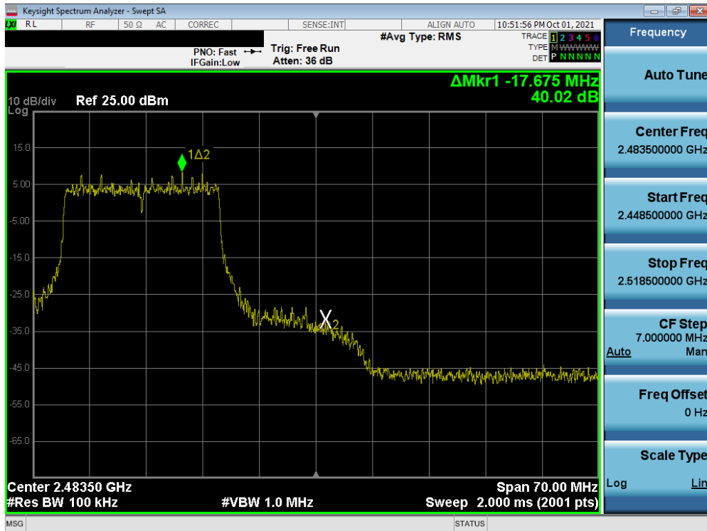
Plot 7-31. Band Edge Plot SISO ANT1 (802.11ax OFDMA – 242 Tones – Ch. 11)
