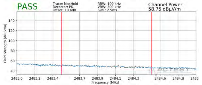
Plot 7-98. Radiated Restricted Upper Band Edge Measurement SISO ANT1 (Peak – 106 Tones)
