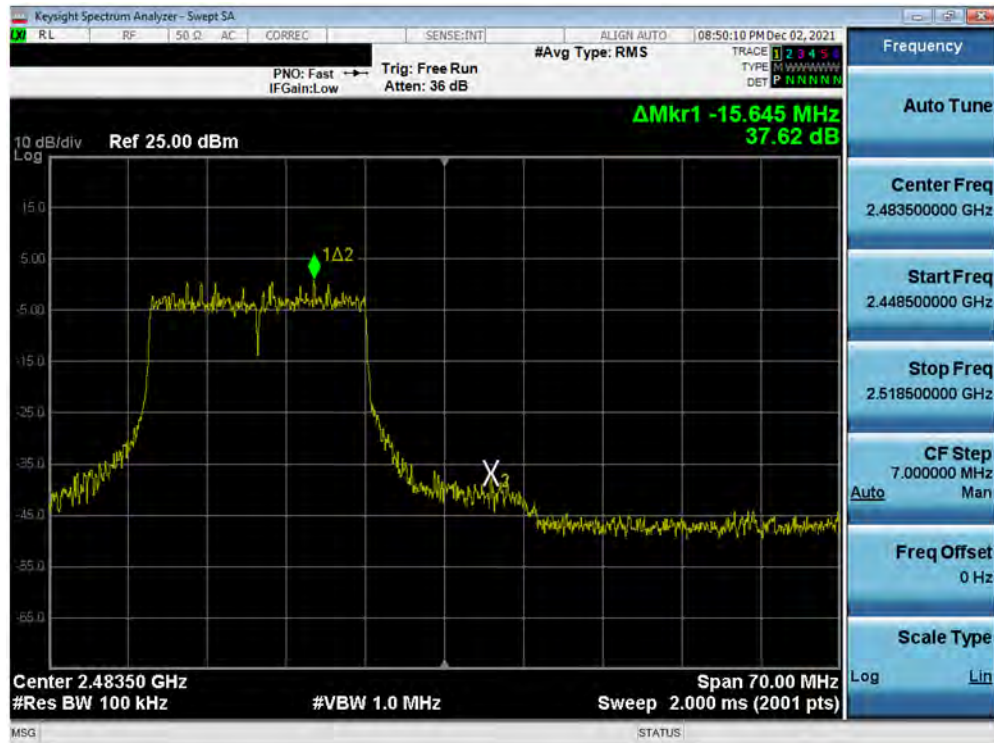
Plot 7-32. Band Edge Plot SISO ANT1 (802.11ax OFDMA – 242 Tones – Ch. 12)
