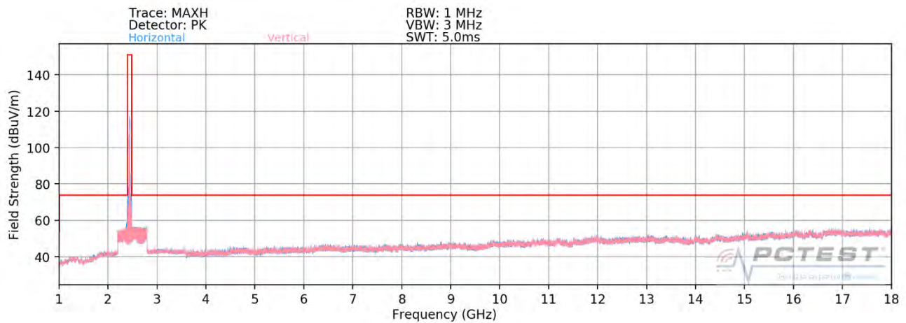
Plot 7-68. Radiated Spurious Plot above 1GHz SISO ANT1 (802.11ax OFDMA – 106 Tones – Ch. 6)
