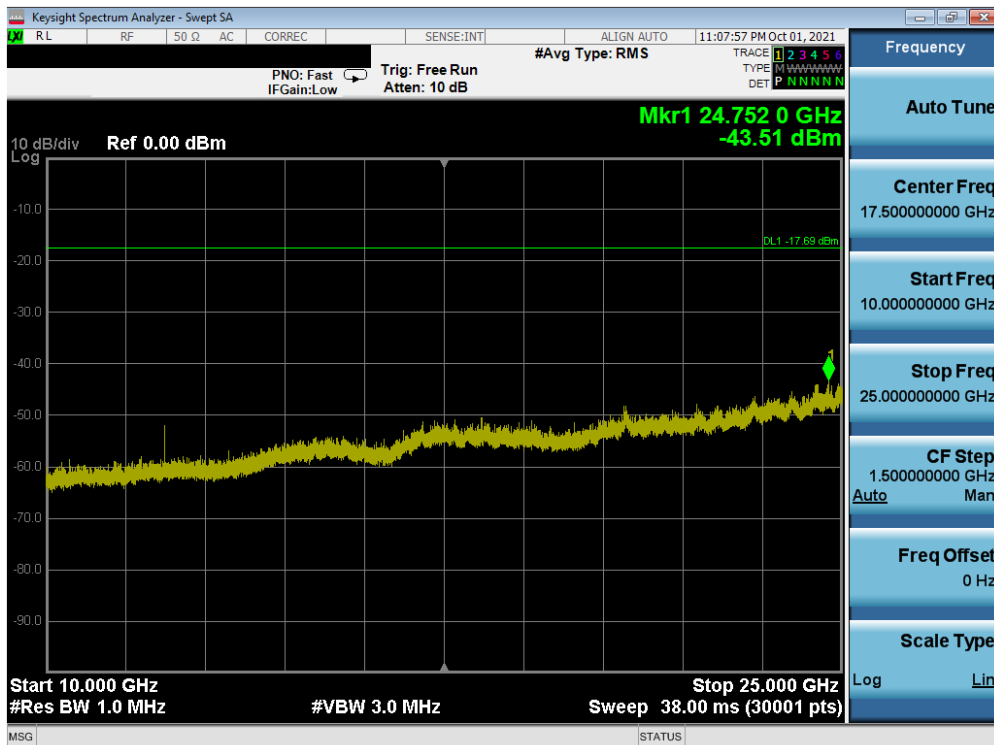
Plot 7-58. Conducted Spurious Plot SISO ANT2 (802.11ax OFDMA – 26 Tones – Ch. 6)
