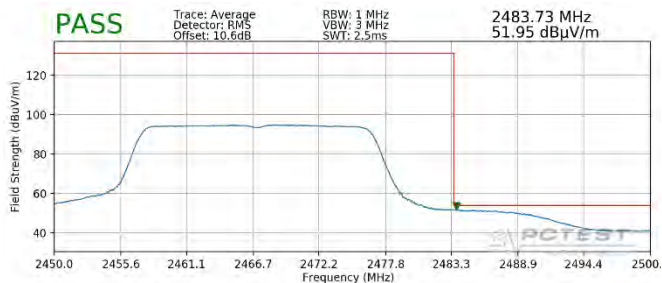
Plot 7-123. Radiated Restricted Upper Band Edge Measurement SISO ANT2 (Average – 242 Tones)
