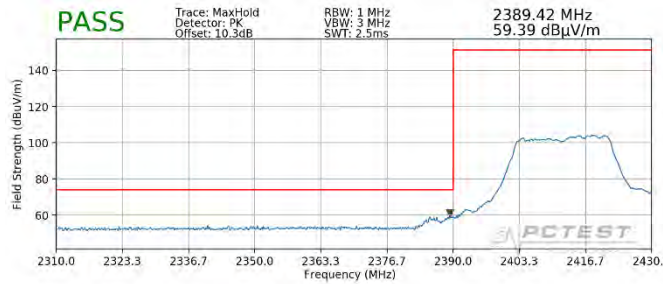
Plot 7-118. Radiated Restricted Lower Band Edge Measurement SISO ANT2 (Peak – 242 Tones)
