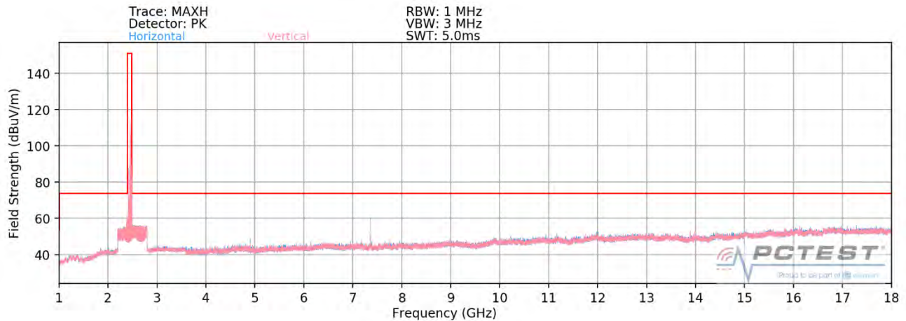
Plot 7-85. Radiated Spurious Plot above 1GHz MIMO (802.11ax OFDMA – 106 Tones – Ch. 11)
