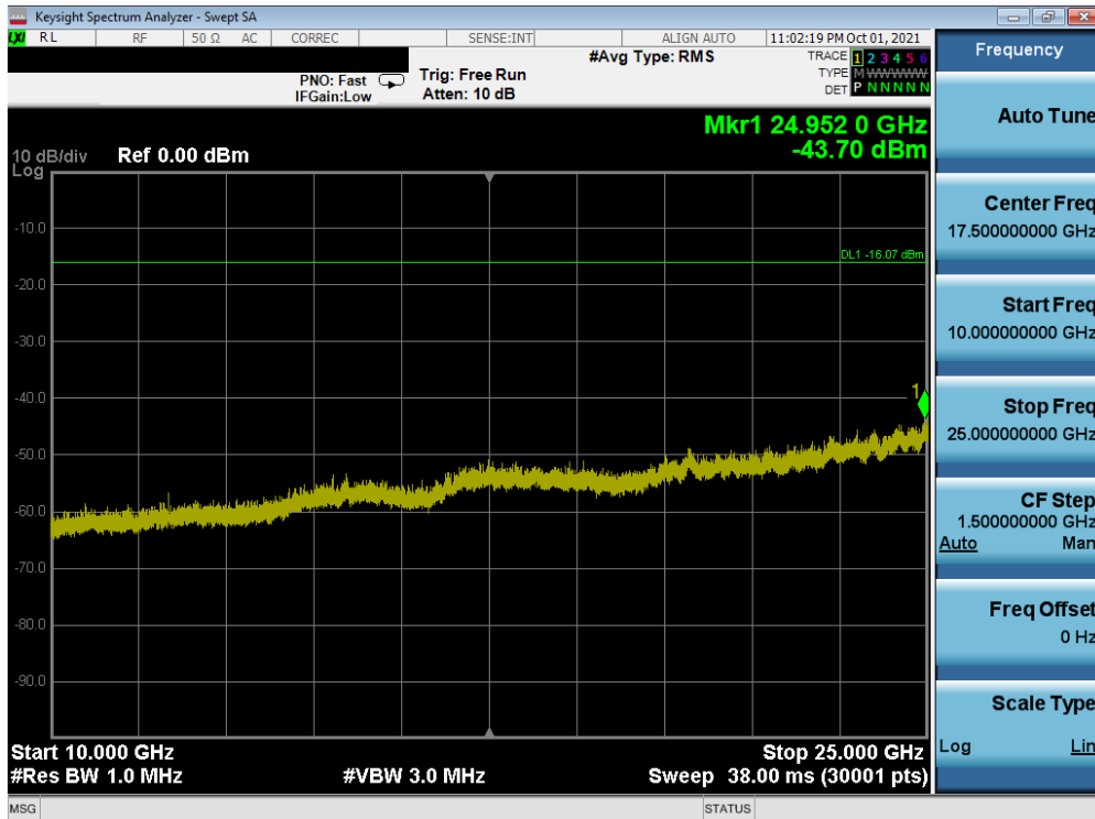
Plot 7-56. Conducted Spurious Plot SISO ANT2 (802.11ax OFDMA – 26 Tones – Ch. 1)
