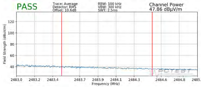
Plot 7-125. Radiated Restricted Upper Band Edge Measurement SISO ANT2 (Average – 242 Tones)
