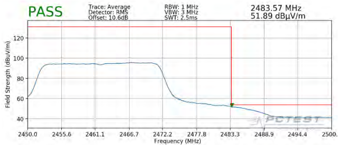
Plot 7-139. Radiated Restricted Upper Band Edge Measurement MIMO (Average – 242 Tones)
