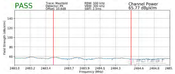
Plot 7-96. Radiated Restricted Upper Band Edge Measurement SISO ANT1 (Peak – 106 Tones)
