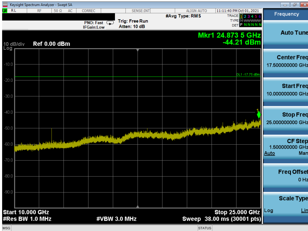
Plot 7-60. Conducted Spurious Plot SISO ANT2 (802.11ax OFDMA – 26 Tones – Ch. 11)
