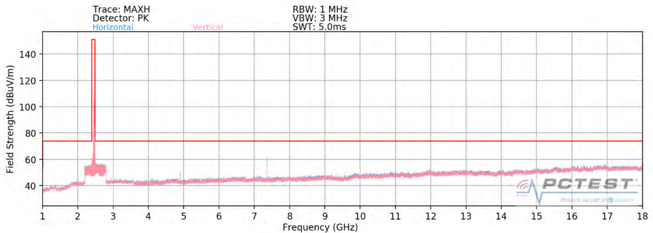
Plot 7-77. Radiated Spurious Plot above 1GHz SISO ANT2 (802.11ax OFDMA – 106 Tones – Ch. 11)
