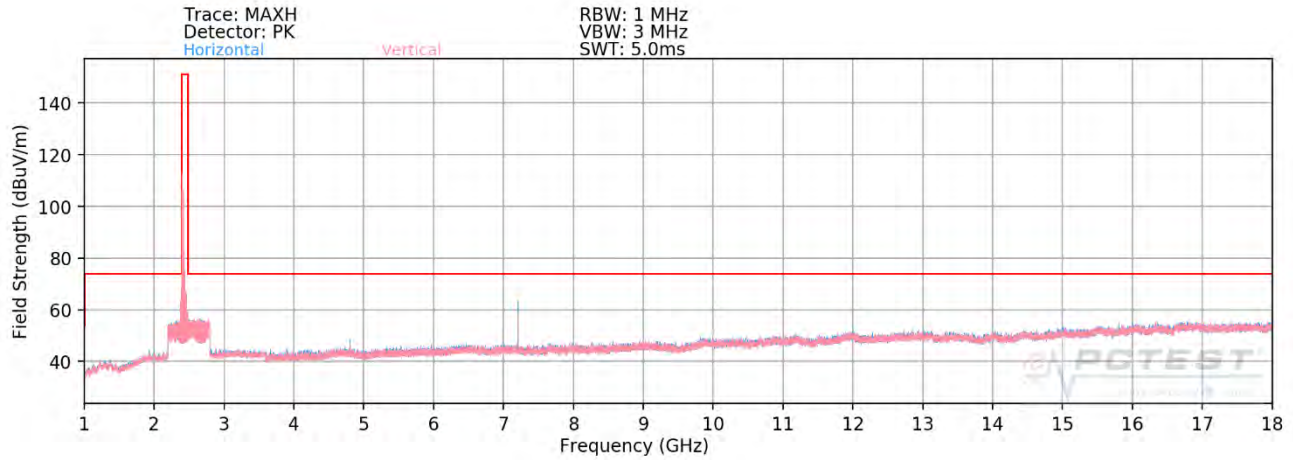
Plot 7-83. Radiated Spurious Plot above 1GHz MIMO (802.11ax OFDMA – 106 Tones – Ch. 1)
