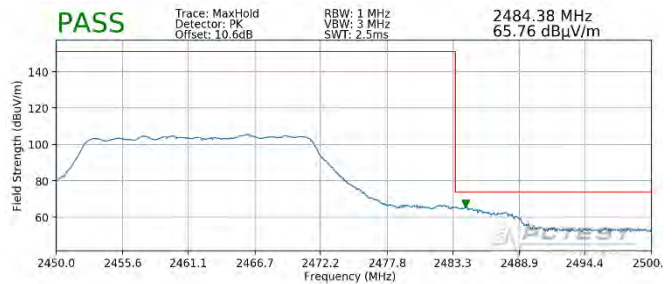
Plot 7-140. Radiated Restricted Upper Band Edge Measurement MIMO (Peak – 242 Tones)
