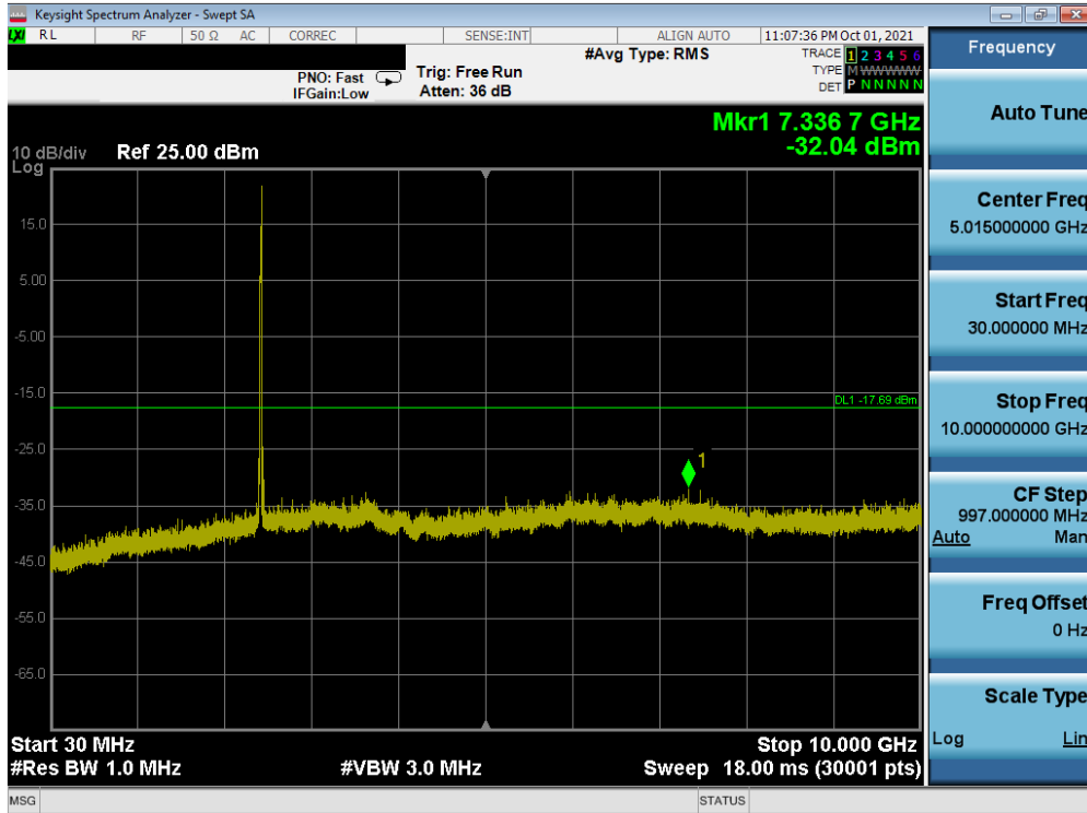
Plot 7-57. Conducted Spurious Plot SISO ANT2 (802.11ax OFDMA – 26 Tones – Ch. 6)
