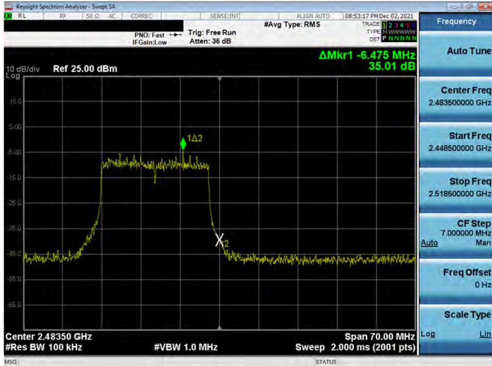
Plot 7-42. Band Edge Plot SISO ANT2 (802.11ax OFDMA – 242 Tones – Ch. 13)
