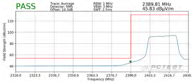
Plot 7-117. Radiated Restricted Lower Band Edge Measurement SISO ANT2 (Average – 242 Tones)
