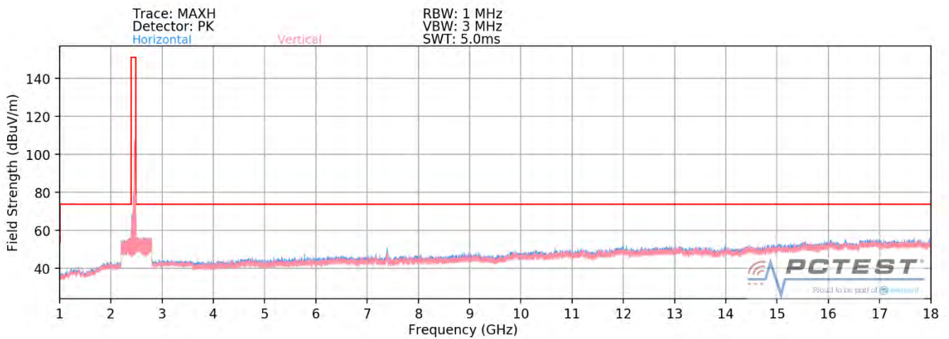
Plot 7-88. Radiated Spurious Plot above 1GHz MIMO (802.11ax OFDMA – 242 Tones – Ch. 11)
