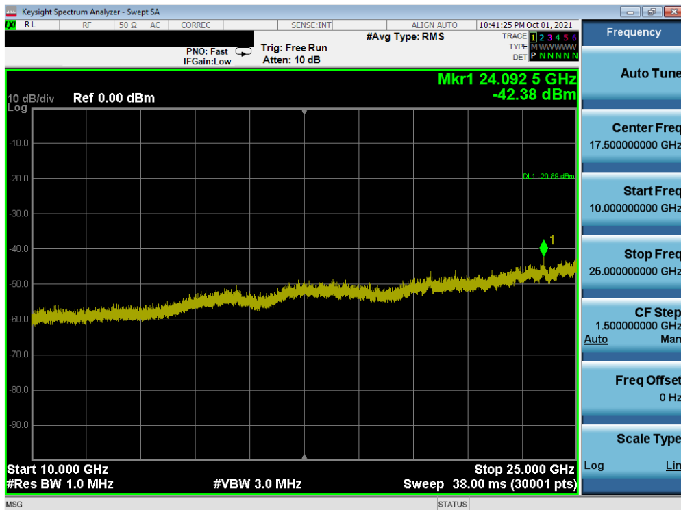
Plot 7-50. Conducted Spurious Plot SISO ANT1 (802.11ax OFDMA – 242 Tones – Ch. 1)
