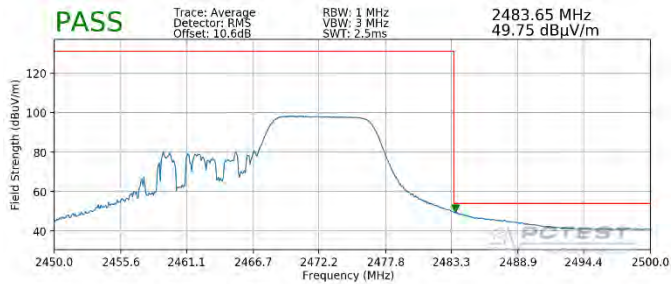
Plot 7-113. Radiated Restricted Upper Band Edge Measurement SISO ANT2 (Average – 106 Tones)
