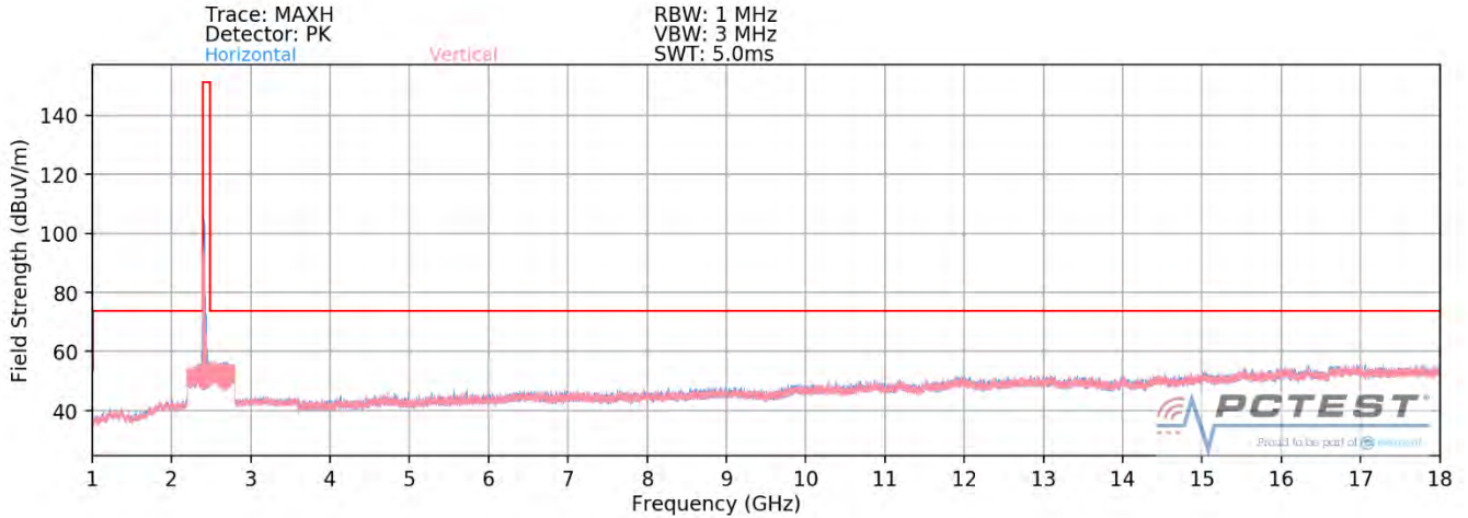
Plot 7-70. Radiated Spurious Plot above 1GHz SISO ANT1 (802.11ax OFDMA – 242 Tones – Ch. 1)
