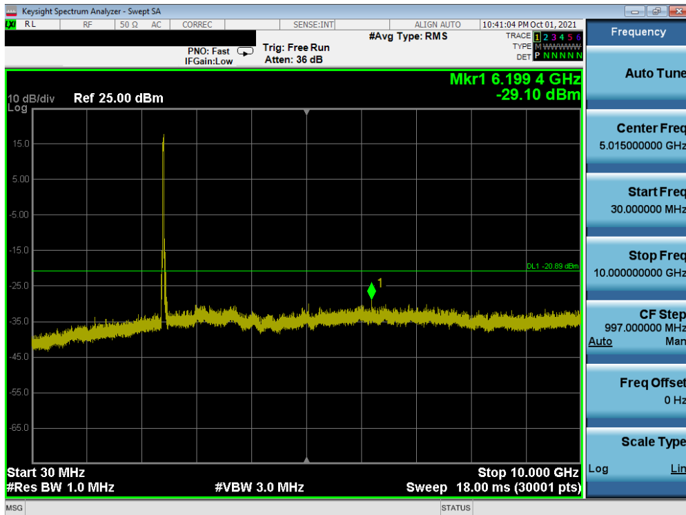
Plot 7-49. Conducted Spurious Plot SISO ANT1 (802.11ax OFDMA – 242 Tones – Ch. 1)
