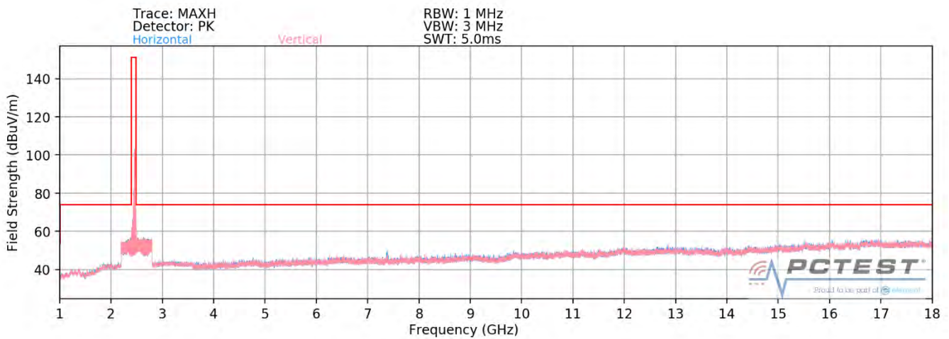
Plot 7-80. Radiated Spurious Plot above 1GHz SISO ANT2 (802.11ax OFDMA – 242 Tones – Ch. 11)
