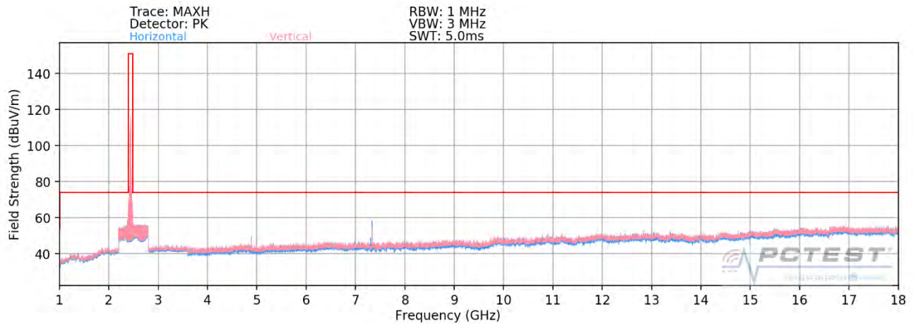
Plot 7-84. Radiated Spurious Plot above 1GHz MIMO (802.11ax OFDMA – 106 Tones – Ch. 6)
