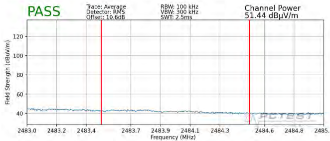
Plot 7-101. Radiated Restricted Upper Band Edge Measurement SISO ANT1 (Average – 242 Tones)
