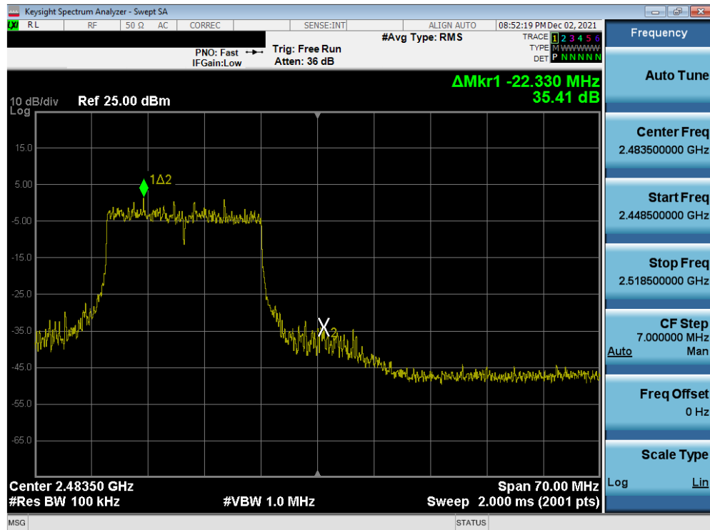
Plot 7-41. Band Edge Plot SISO ANT2 (802.11ax OFDMA – 242 Tones – Ch. 12)
