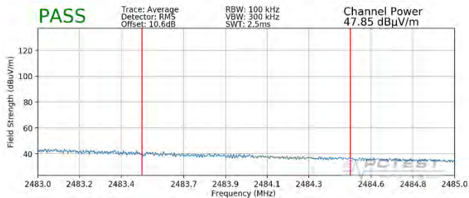
Plot 7-115. Radiated Restricted Upper Band Edge Measurement SISO ANT2 (Average – 106 Tones)
