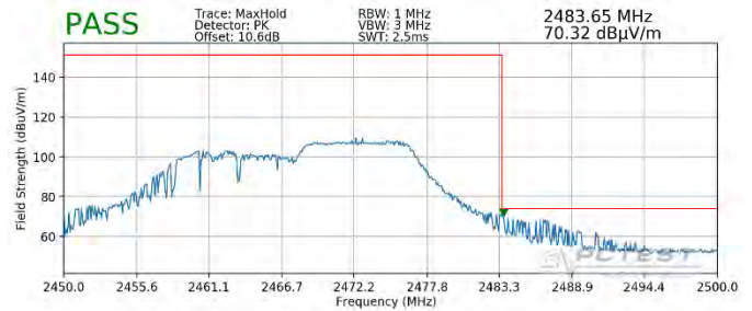
Plot 7-114. Radiated Restricted Upper Band Edge Measurement SISO ANT2 (Peak – 106 Tones)
