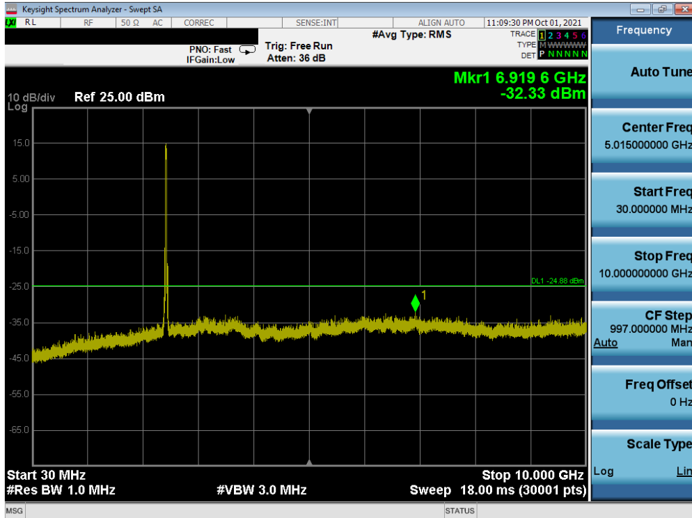
Plot 7-63. Conducted Spurious Plot SISO ANT2 (802.11ax OFDMA – 242 Tones – Ch. 6)
