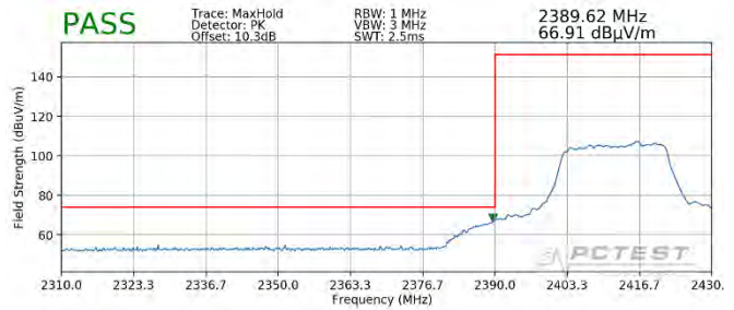
Plot 7-136. Radiated Restricted Lower Band Edge Measurement MIMO (Peak – 242 Tones)
