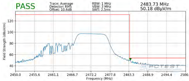
Plot 7-95. Radiated Restricted Upper Band Edge Measurement SISO ANT1 (Average – 106 Tones)
