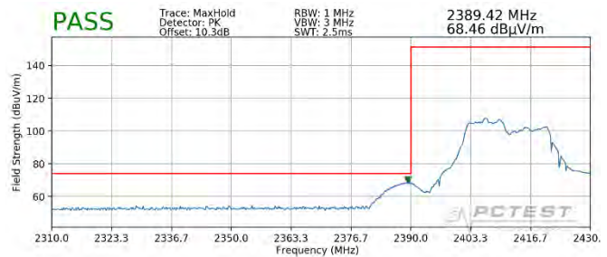
Plot 7-110. Radiated Restricted Lower Band Edge Measurement SISO ANT2 (Peak – 106 Tones)
