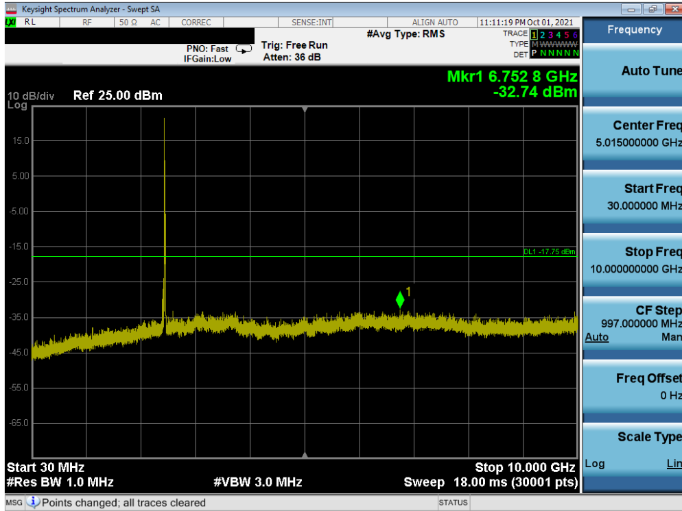
Plot 7-59. Conducted Spurious Plot SISO ANT2 (802.11ax OFDMA – 26 Tones – Ch. 11)
