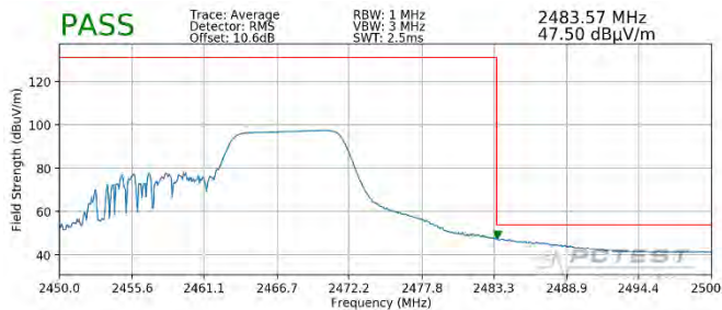
Plot 7-111. Radiated Restricted Upper Band Edge Measurement SISO ANT2 (Average – 106 Tones)
