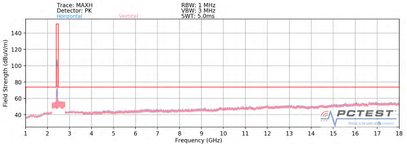
Plot 7-71. Radiated Spurious Plot above 1GHz SISO ANT1 (802.11ax OFDMA – 242 Tones – Ch. 6)
