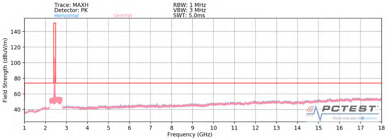
Plot 7-87. Radiated Spurious Plot above 1GHz MIMO (802.11ax OFDMA – 242 Tones – Ch. 6)
