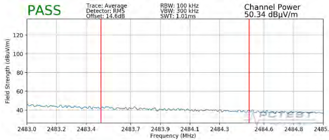
Plot 7-133. Radiated Restricted Upper Band Edge Measurement MIMO (Average – 106 Tones)
