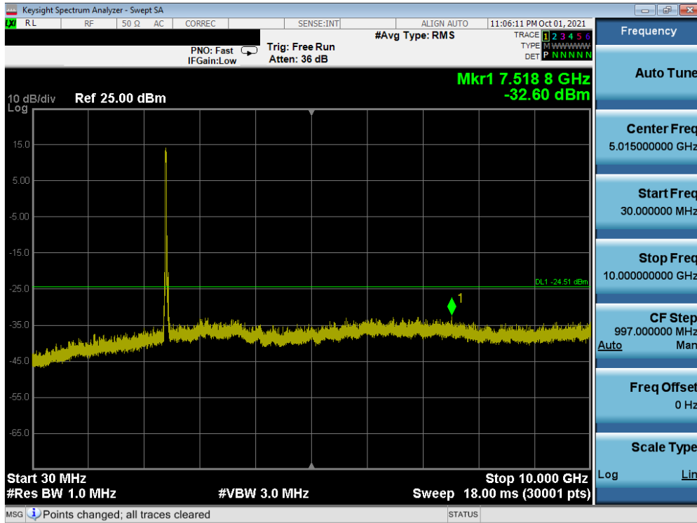
Plot 7-61. Conducted Spurious Plot SISO ANT2 (802.11ax OFDMA – 242 Tones – Ch. 1)
