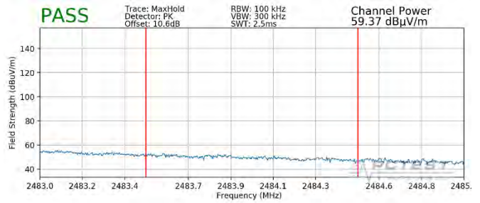
Plot 7-126. Radiated Restricted Upper Band Edge Measurement SISO ANT2 (Peak – 242 Tones)
