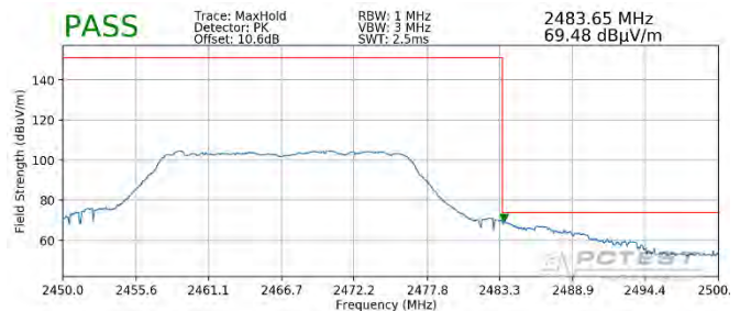
Plot 7-124. Radiated Restricted Upper Band Edge Measurement SISO ANT2 (Peak – 242 Tones)
