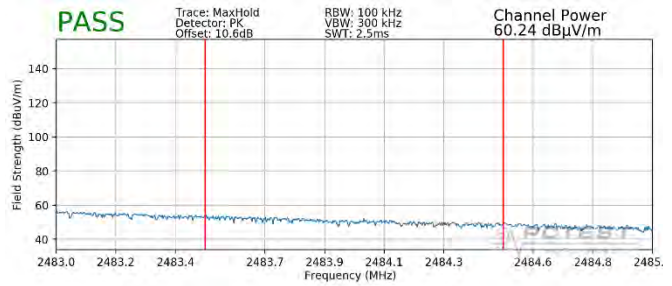
Plot 7-108. Radiated Restricted Upper Band Edge Measurement SISO ANT1 (Peak – 242 Tones)
