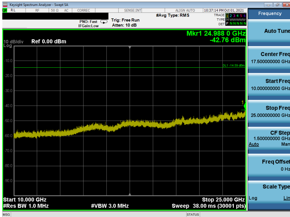
Plot 7-44. Conducted Spurious Plot SISO ANT1 (802.11ax OFDMA – 26 Tones – Ch. 1)
