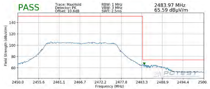
Plot 7-106. Radiated Restricted Upper Band Edge Measurement SISO ANT1 (Peak – 242 Tones)
