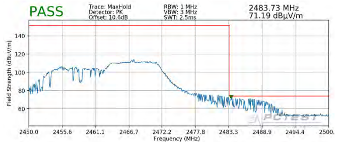
Plot 7-94. Radiated Restricted Upper Band Edge Measurement SISO ANT1 (Peak – 106 Tones)
