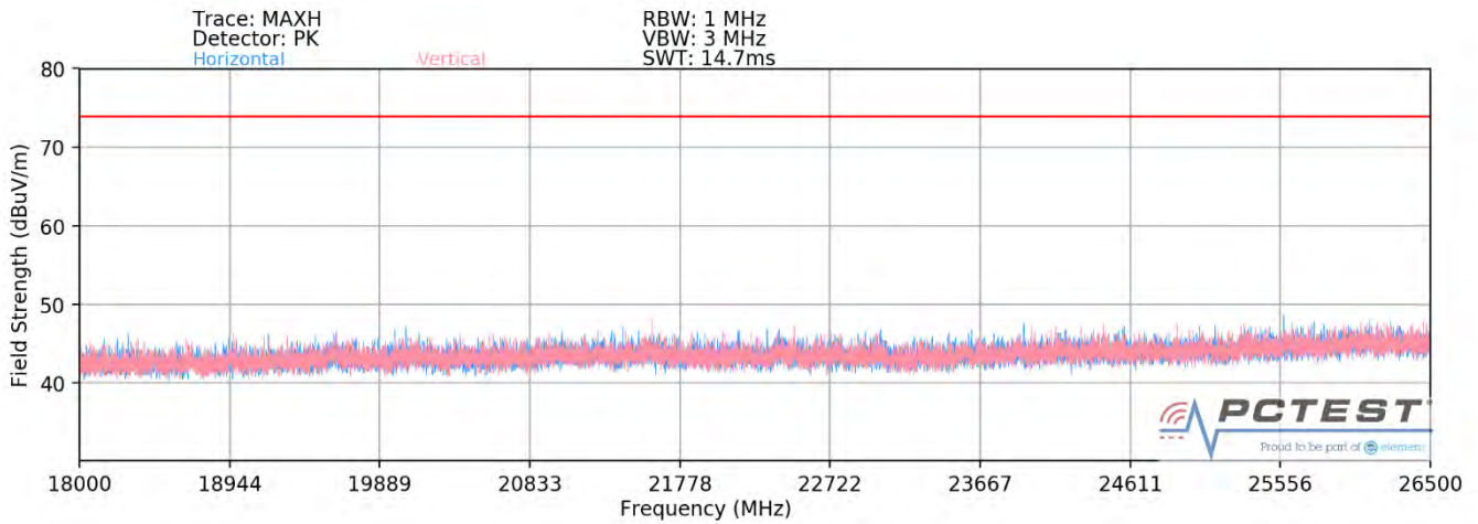
Plot 7-81. Radiated Spurious Plot above 18GHz SISO ANT2 (802.11ax OFDMA – 106 Tones)
