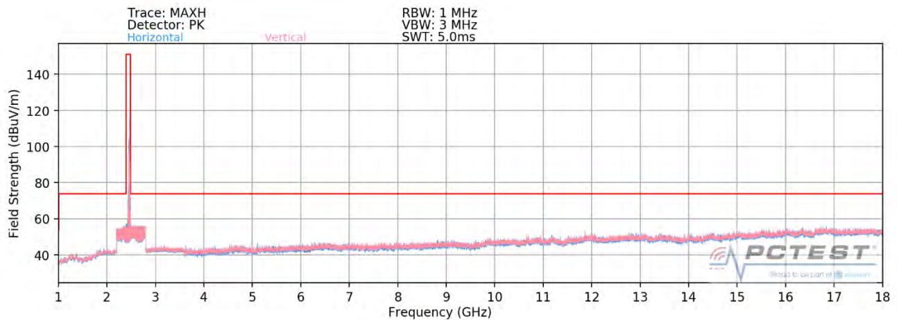
Plot 7-69. Radiated Spurious Plot above 1GHz SISO ANT1 (802.11ax OFDMA – 106 Tones – Ch. 11)
