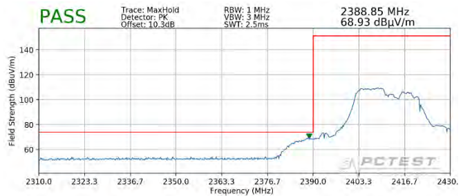
Plot 7-128. Radiated Restricted Lower Band Edge Measurement MIMO (Peak – 106 Tones)
