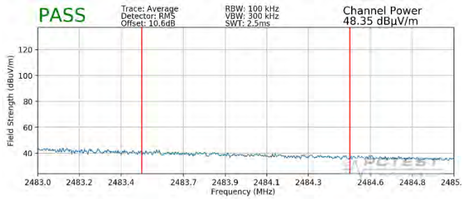
Plot 7-107. Radiated Restricted Upper Band Edge Measurement SISO ANT1 (Average – 242 Tones)
