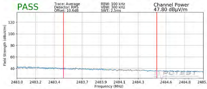
Plot 7-97. Radiated Restricted Upper Band Edge Measurement SISO ANT1 (Average – 106 Tones)
