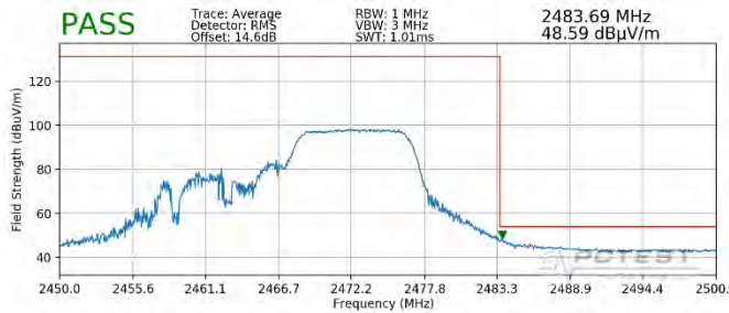
Plot 7-131. Radiated Restricted Upper Band Edge Measurement MIMO (Average – 106 Tones)
