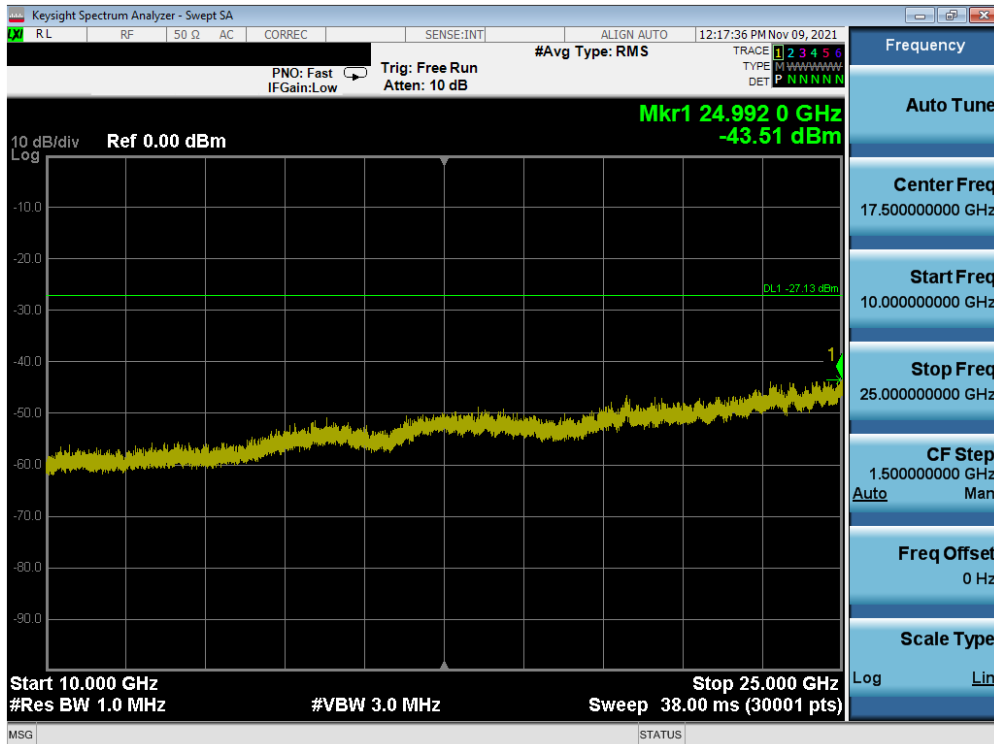
Plot 7-66. Conducted Spurious Plot SISO ANT2 (802.11ax OFDMA – 242 Tones – Ch. 11)
