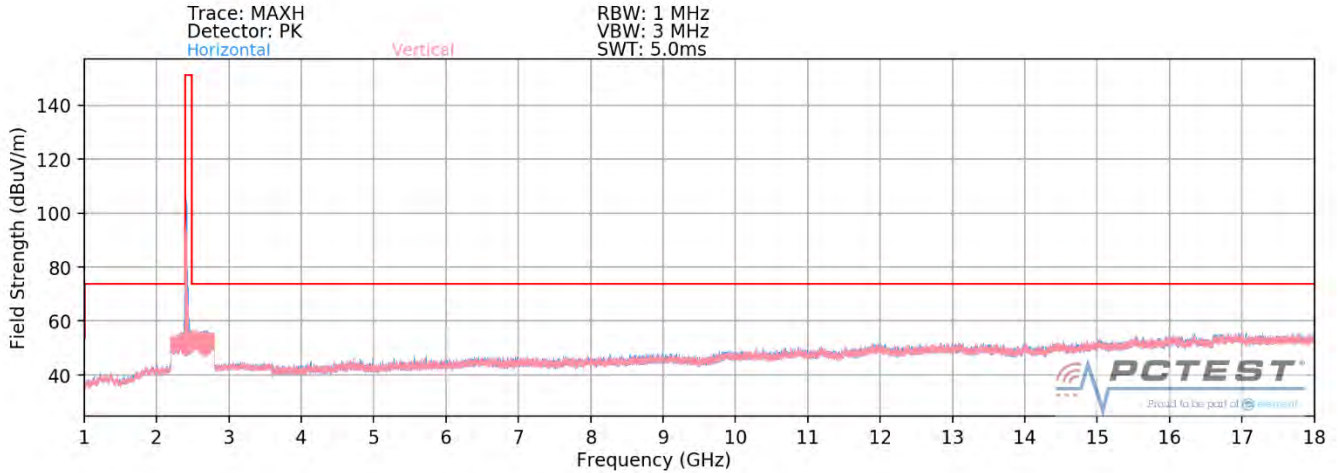
Plot 7-78. Radiated Spurious Plot above 1GHz SISO ANT2 (802.11ax OFDMA – 242 Tones – Ch. 1)
