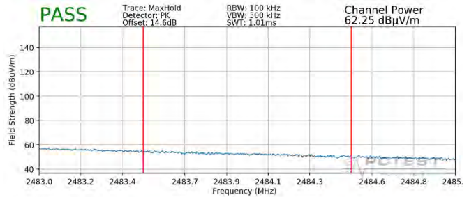
Plot 7-134. Radiated Restricted Upper Band Edge Measurement MIMO (Peak – 106 Tones)
