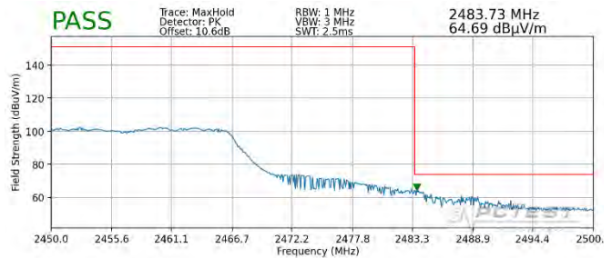
Plot 7-120. Radiated Restricted Upper Band Edge Measurement SISO ANT2 (Peak – 242 Tones)
