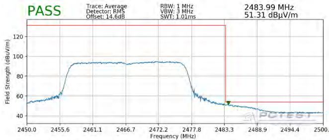
Plot 7-141. Radiated Restricted Upper Band Edge Measurement MIMO (Average – 242 Tones)
