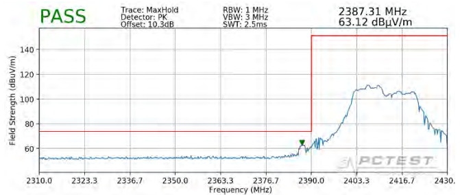
Plot 7-92. Radiated Restricted Lower Band Edge Measurement SISO ANT1 (Peak – 106 Tones)
