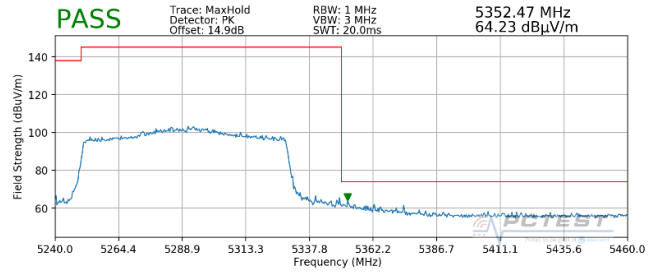
Plot 7-437. Radiated Upper Band Edge Plot MIMO WCP (Peak – UNII Band 2A)
