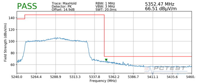
Plot 7-430. Radiated Upper Band Edge Plot MIMO (Peak – UNII Band 2A)
