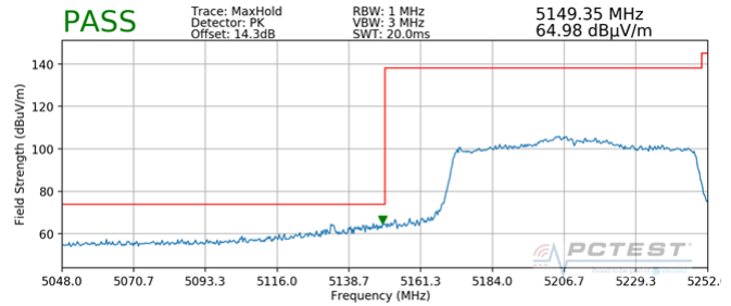
Plot 7-428. Radiated Lower Band Edge Plot MIMO (Peak – UNII Band 1)
