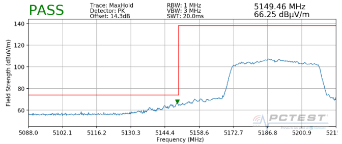
Plot 7-426. Radiated Lower Band Edge Plot MIMO WCP (Peak – UNII Band 1)
