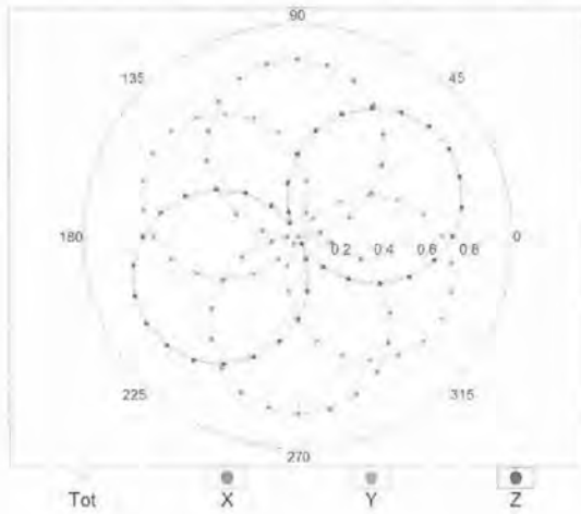
f=600 MHz,TEM
