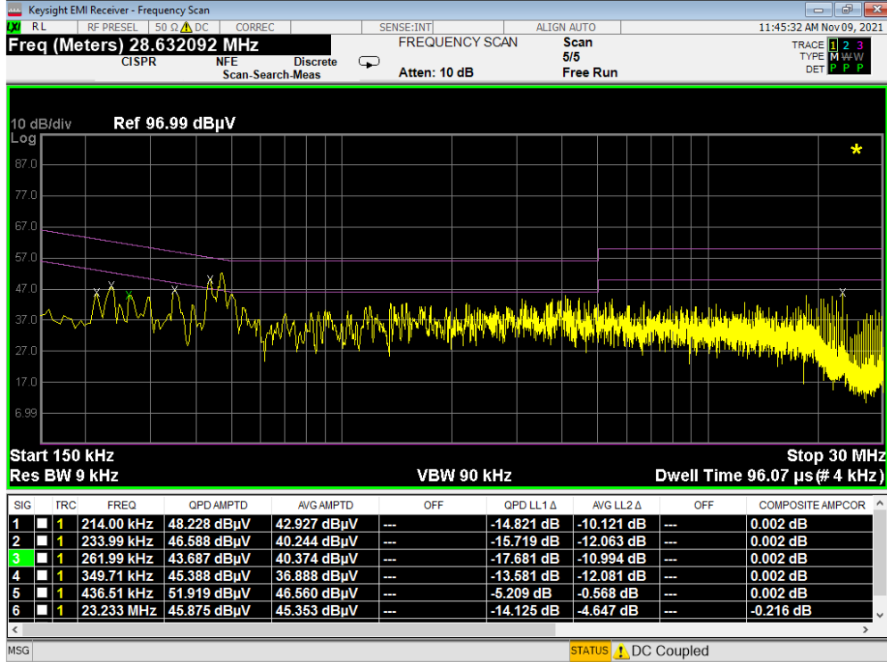
Plot 7-10. Line-Conducted Test Plot (L1) - Device to Device WPT – Config 1
