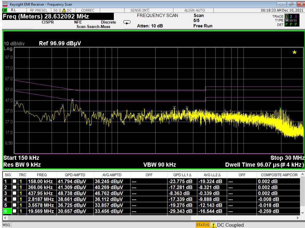
Plot 7-15. Line-Conducted Test Plot (N) - Device to Device WPT – Config 3
