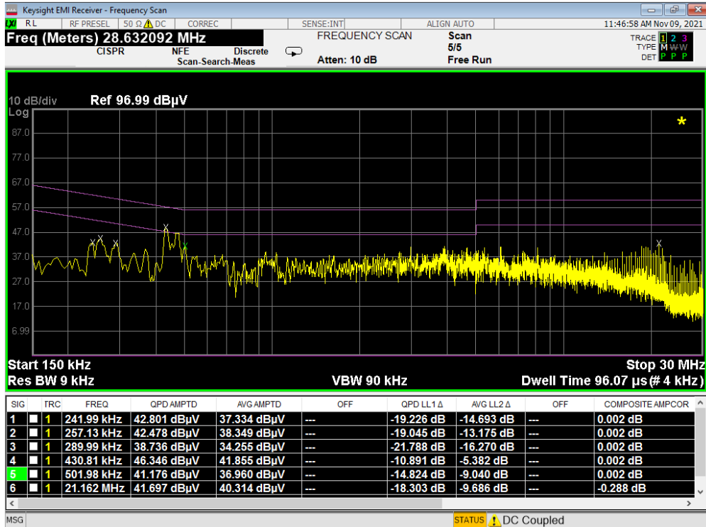
Plot 7-11. Line-Conducted Test Plot (N) - Device to Device WPT – Config 1
