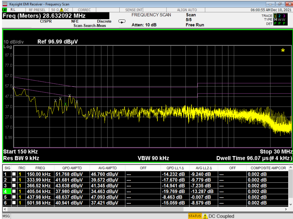
Plot 7-13. Line-Conducted Test Plot (N) - Device to Device WPT – Config 2
