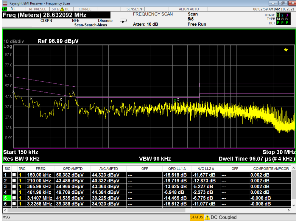
Plot 7-12. Line-Conducted Test Plot (L1) - Device to Device WPT – Config 2
