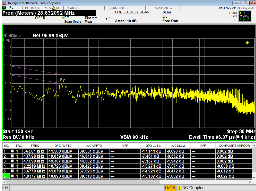
Plot 7-14. Line-Conducted Test Plot (L1) - Device to Device WPT – Config 3
