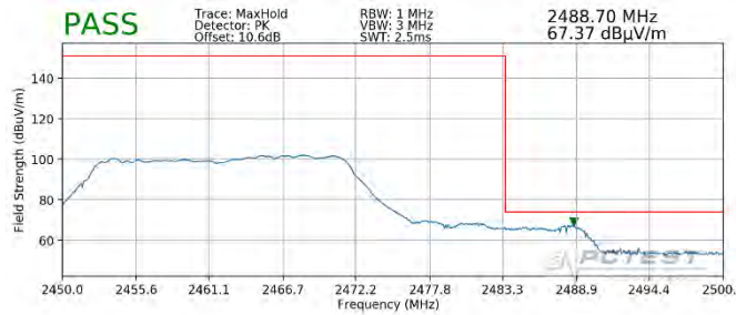
Plot 7-122. Radiated Restricted Upper Band Edge Measurement SISO ANT2 (Peak – 242 Tones)
