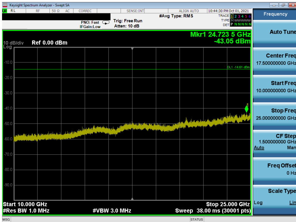
Plot 7-46. Conducted Spurious Plot SISO ANT1 (802.11ax OFDMA – 26 Tones – Ch. 6)
