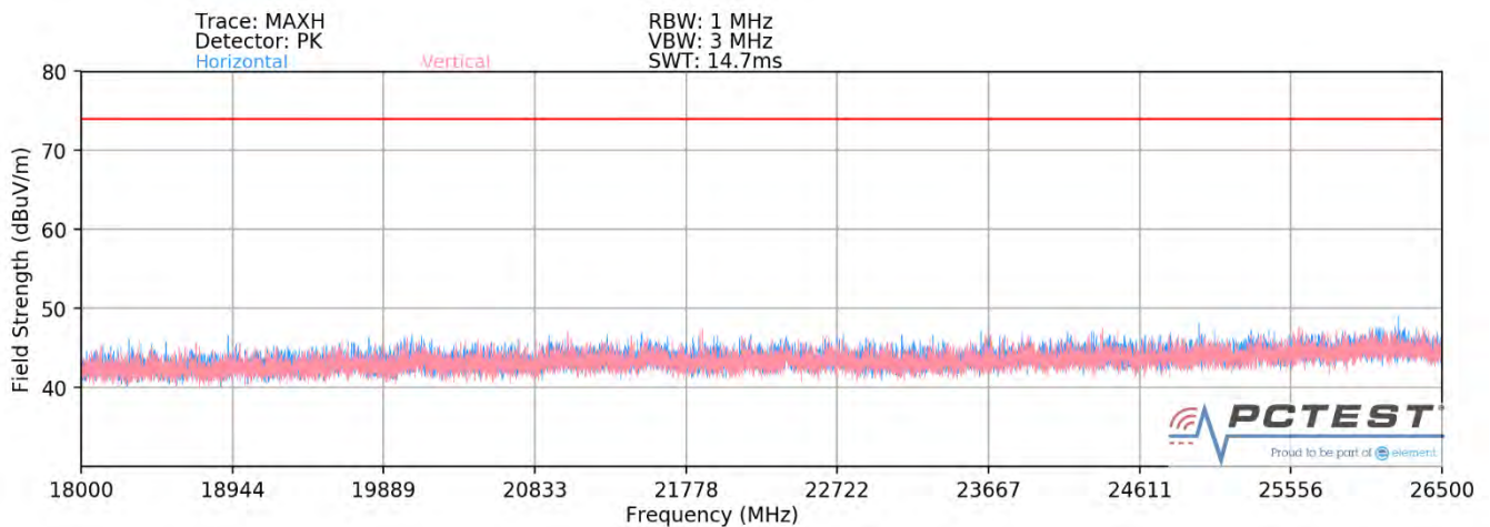
Plot 7-82. Radiated Spurious Plot above 18GHz SISO ANT2 (802.11ax OFDMA – 242 Tones)
