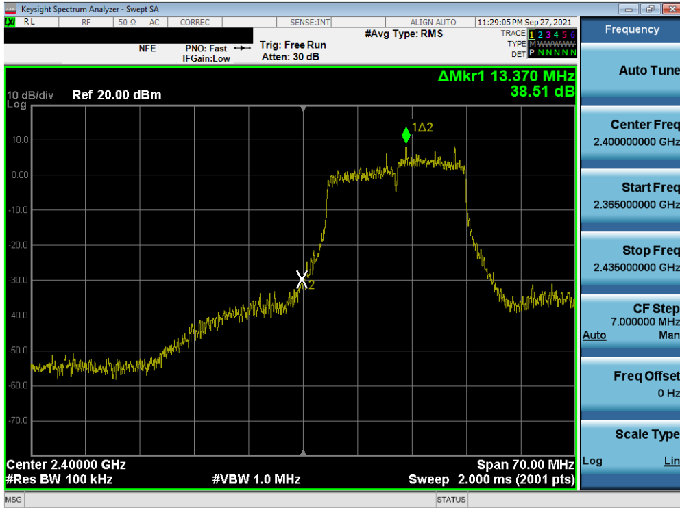
Plot 7-99. Band Edge Plot SISO ANT2 (802.11n (2.4GHz) – Ch. 1)
