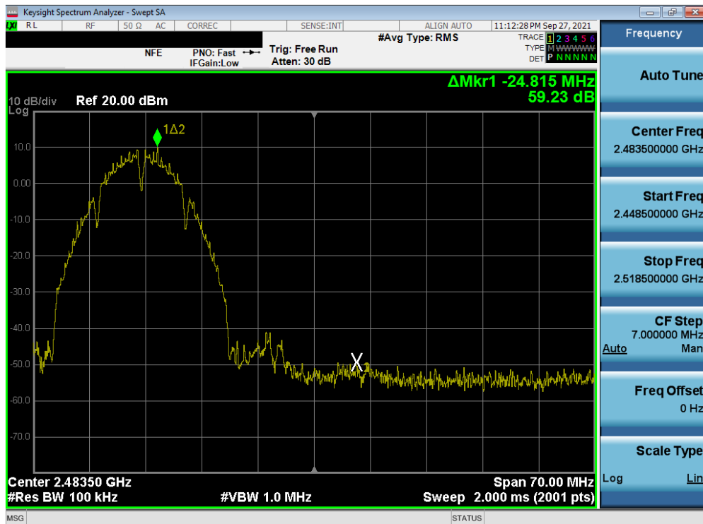
Plot 7-92. Band Edge Plot SISO ANT2 (802.11b – Ch. 11)
