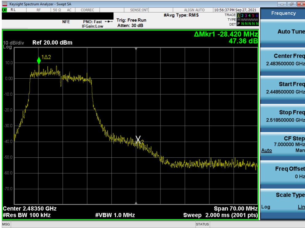
Plot 7-83. Band Edge Plot SISO ANT1 (802.11n (2.4GHz) – Ch. 11)
