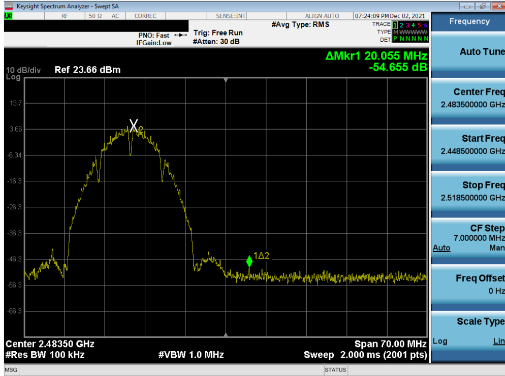
Plot 7-75. Band Edge Plot SISO ANT1 (802.11b – Ch. 12)
