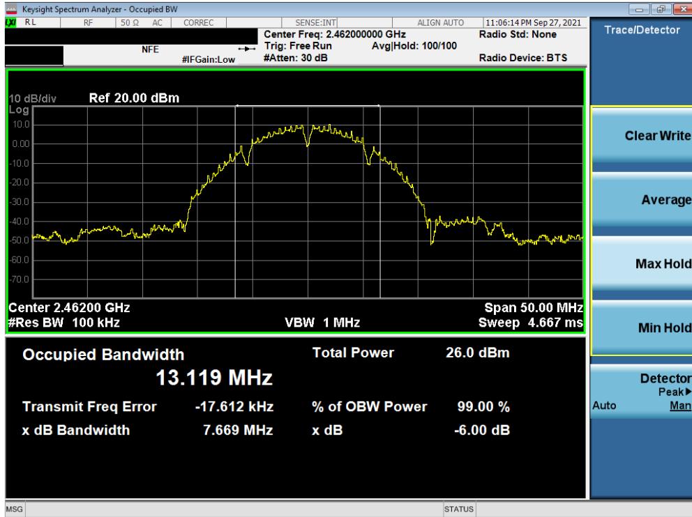
Plot 7-3. 6dB Bandwidth Plot SISO ANT1(802.11b – Ch. 11)
