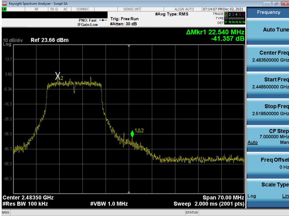
Plot 7-79. Band Edge Plot SISO ANT1 (802.11g – Ch. 12)
