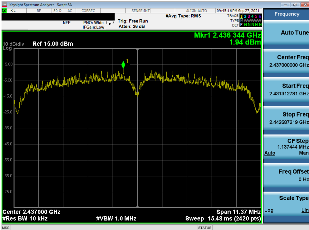
Plot 7-62. Power Spectral Density Plot MIMO ANT2 (802.11b (2.4GHz) – Ch. 6)
