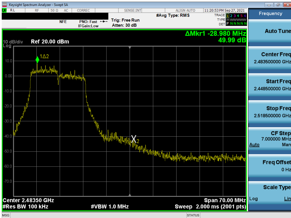
Plot 7-96. Band Edge Plot SISO ANT2 (802.11g - Ch. 11)
