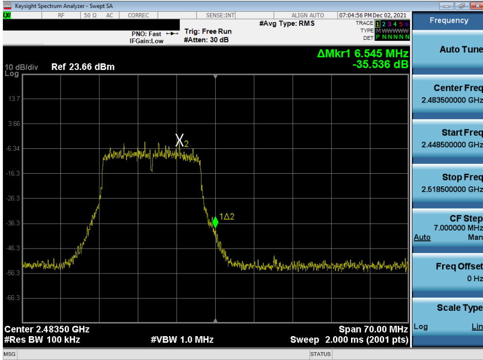
Plot 7-103. Band Edge Plot SISO ANT2 (802.11n (2.4GHz) – Ch. 13)
