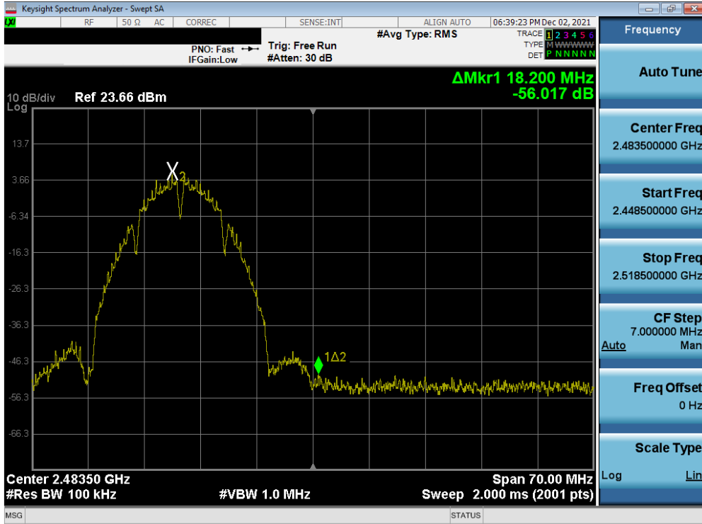
Plot 7-93. Band Edge Plot SISO ANT2 (802.11b – Ch. 12)
