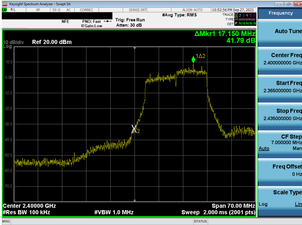
Plot 7-81. Band Edge Plot SISO ANT1 (802.11n (2.4GHz) – Ch. 1)
