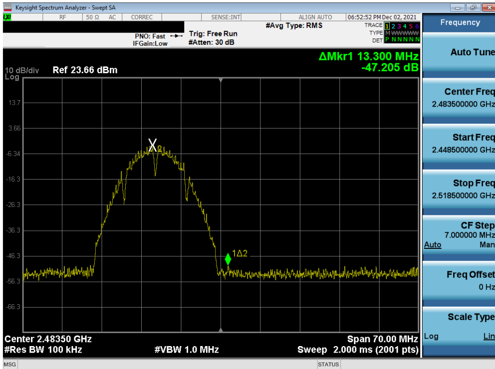
Plot 7-94. Band Edge Plot SISO ANT2 (802.11b – Ch. 13)
