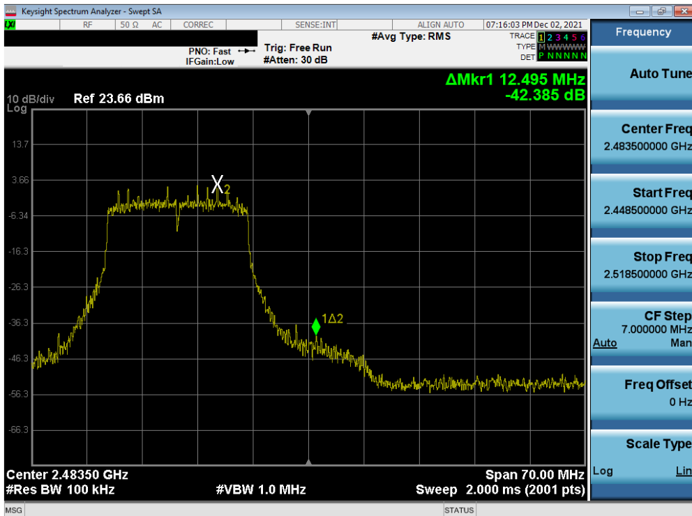
Plot 7-84. Band Edge Plot SISO ANT1 (802.11n (2.4GHz) – Ch. 12)
