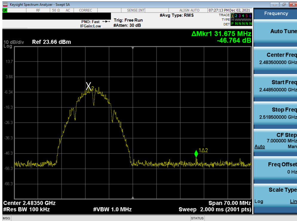
Plot 7-76. Band Edge Plot SISO ANT1 (802.11b – Ch. 13)
