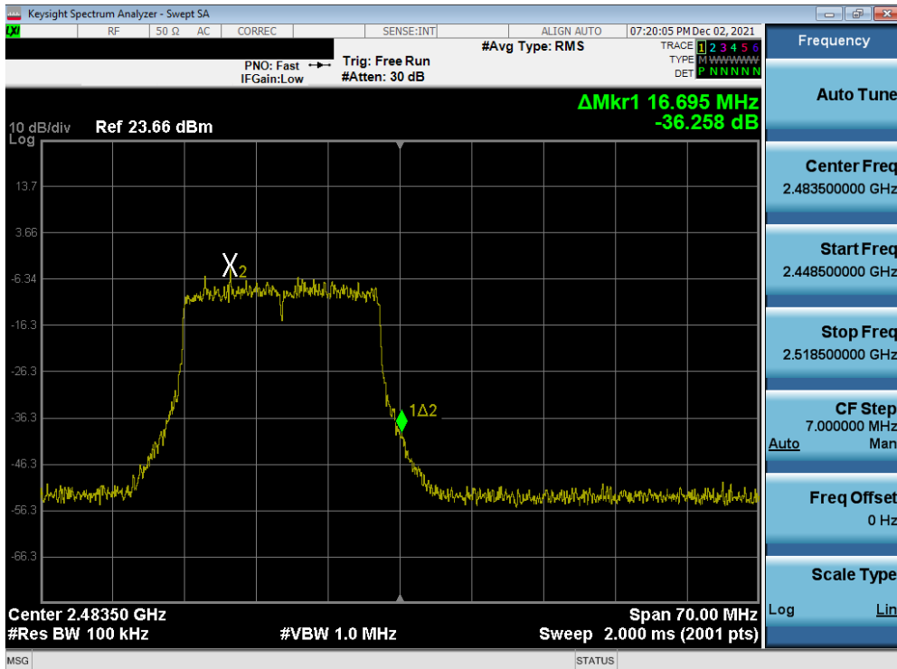
Plot 7-90. Band Edge Plot SISO ANT1 (802.11ax (2.4GHz) – Ch. 13)
