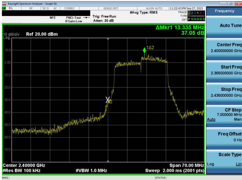
Plot 7-104. Band Edge Plot SISO ANT2 (802.11ax (2.4GHz) – Ch. 1)
