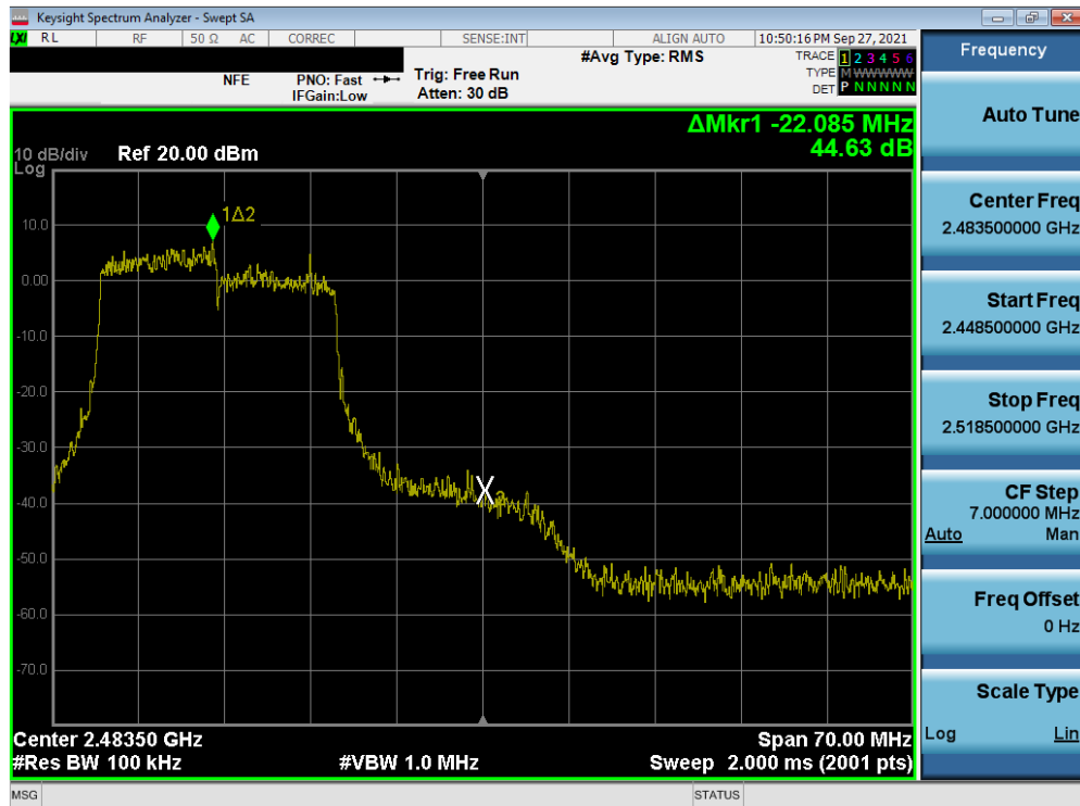
Plot 7-88. Band Edge Plot SISO ANT1 (802.11ax (2.4GHz) – Ch. 11)
