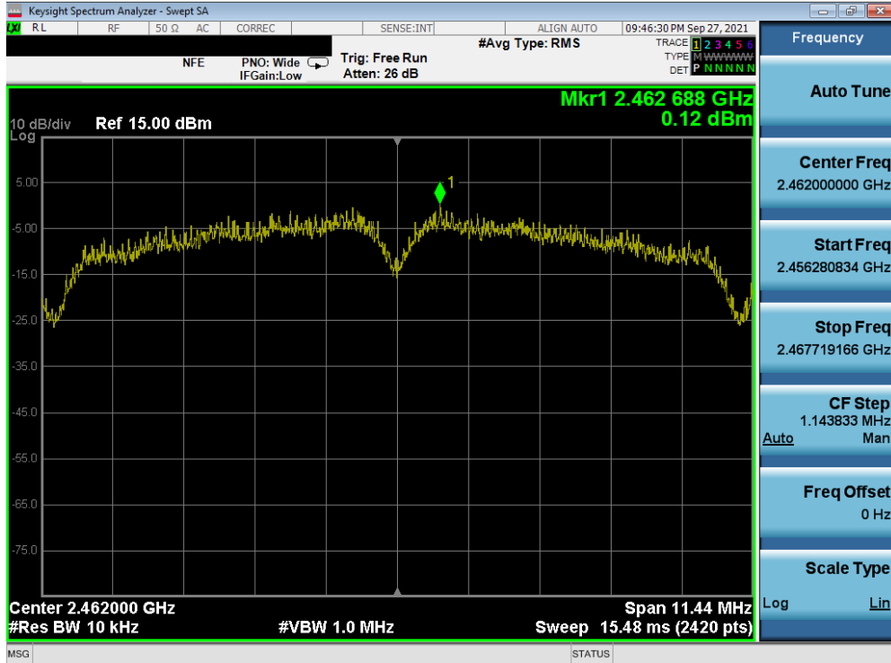
Plot 7-63. Power Spectral Density Plot MIMO ANT2 (802.11b (2.4GHz) – Ch. 11)
