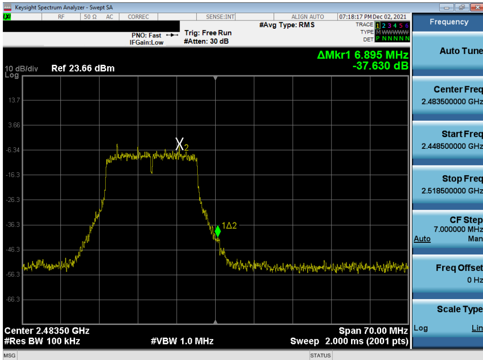
Plot 7-80. Band Edge Plot SISO ANT1 (802.11g – Ch. 13)
