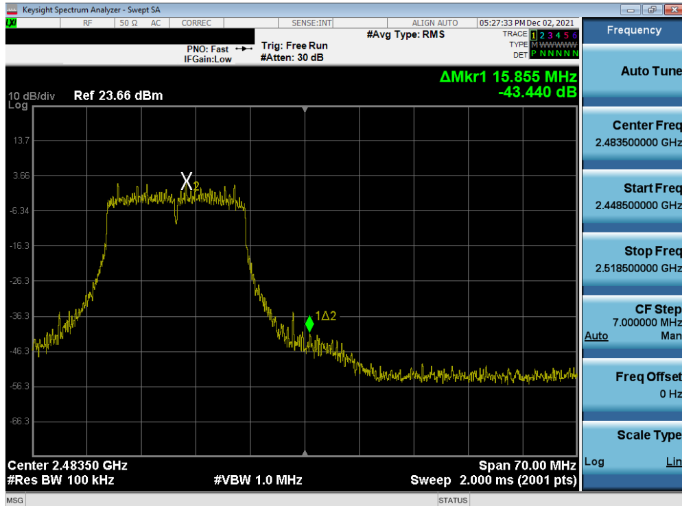
Plot 7-102. Band Edge Plot SISO ANT2 (802.11n (2.4GHz) – Ch. 12)
