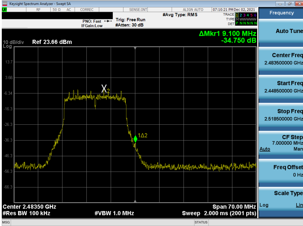
Plot 7-85. Band Edge Plot SISO ANT1 (802.11n (2.4GHz) – Ch. 13)
