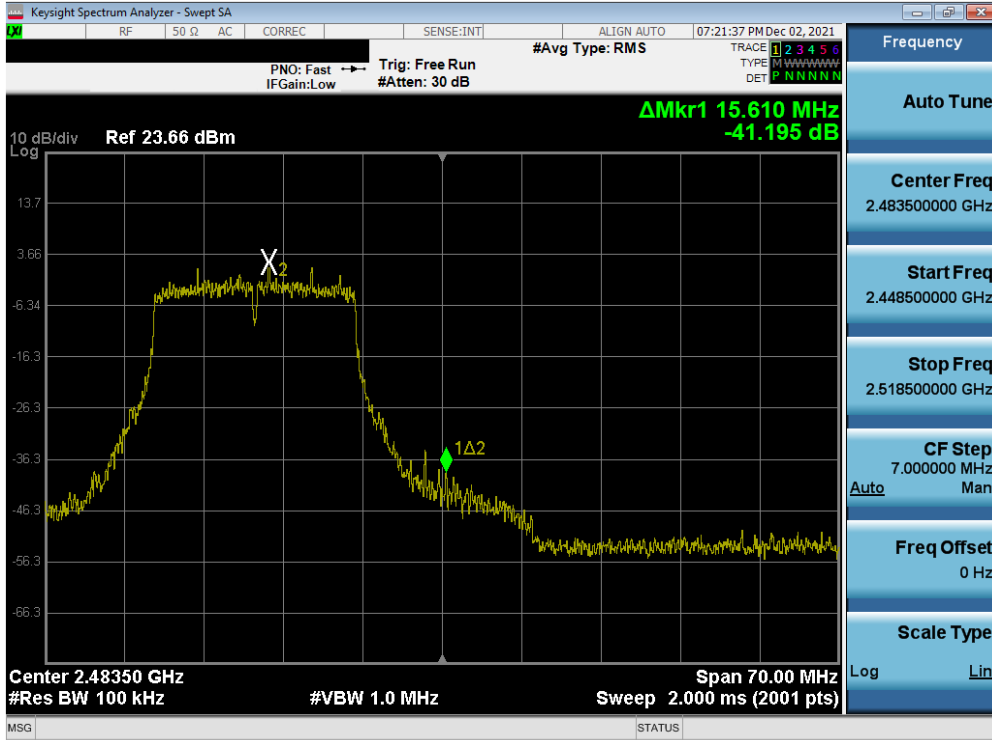
Plot 7-89. Band Edge Plot SISO ANT1 (802.11ax (2.4GHz) – Ch. 12)
