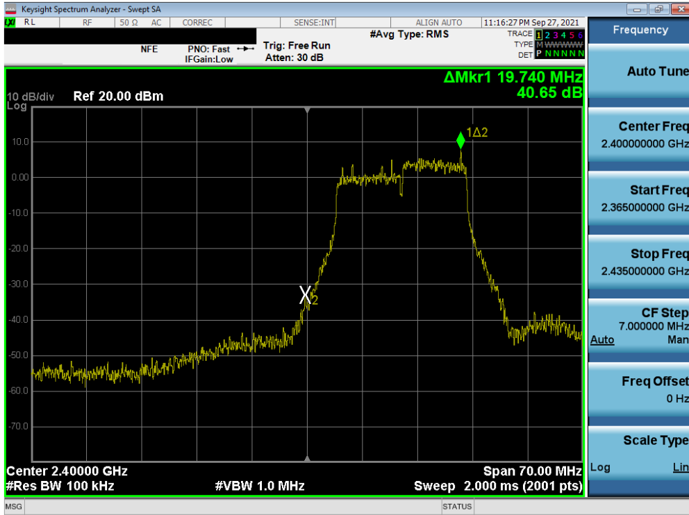
Plot 7-95. Band Edge Plot SISO ANT2 (802.11g- Ch. 1)
