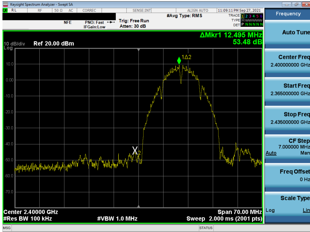
Plot 7-91. Band Edge Plot SISO ANT2 (802.11b – Ch. 1)
