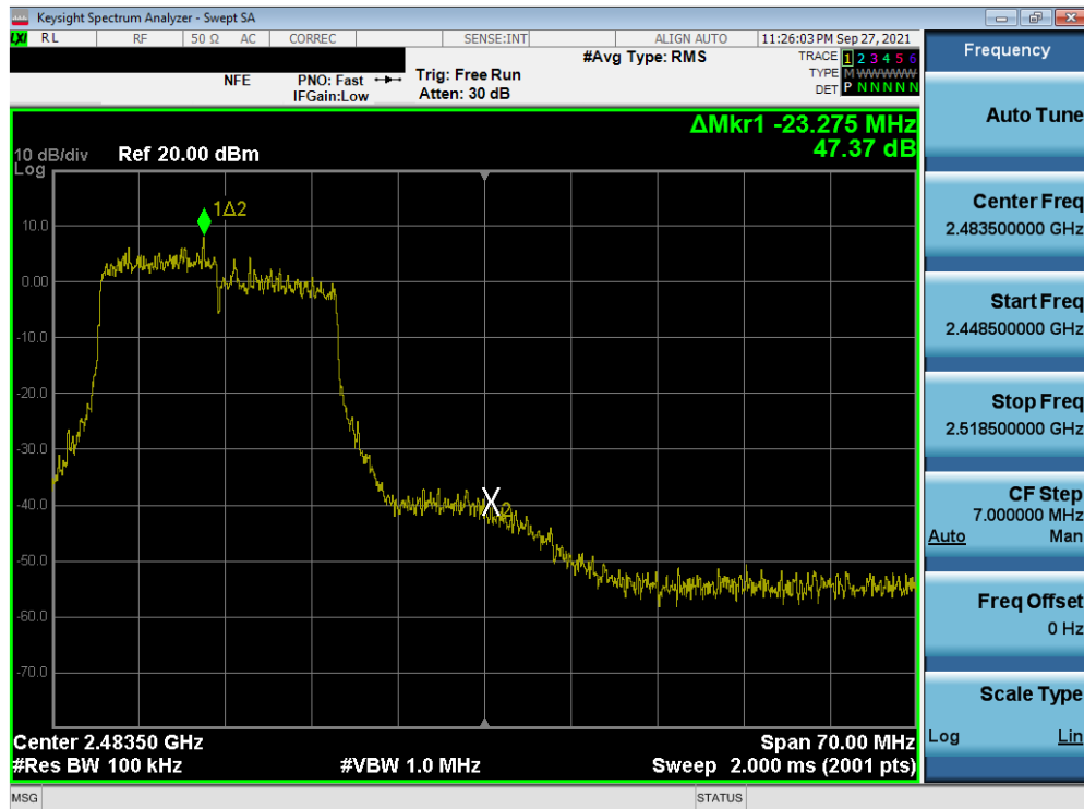
Plot 7-106. Band Edge Plot SISO ANT2 (802.11ax (2.4GHz) – Ch. 11)
