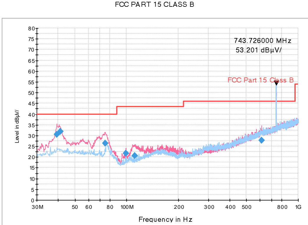
Figure 2: Radiated Emission (30 MHz to 1 GHz), [EUT+TA] LTE B12+B13+B17 Middle ch Idle
