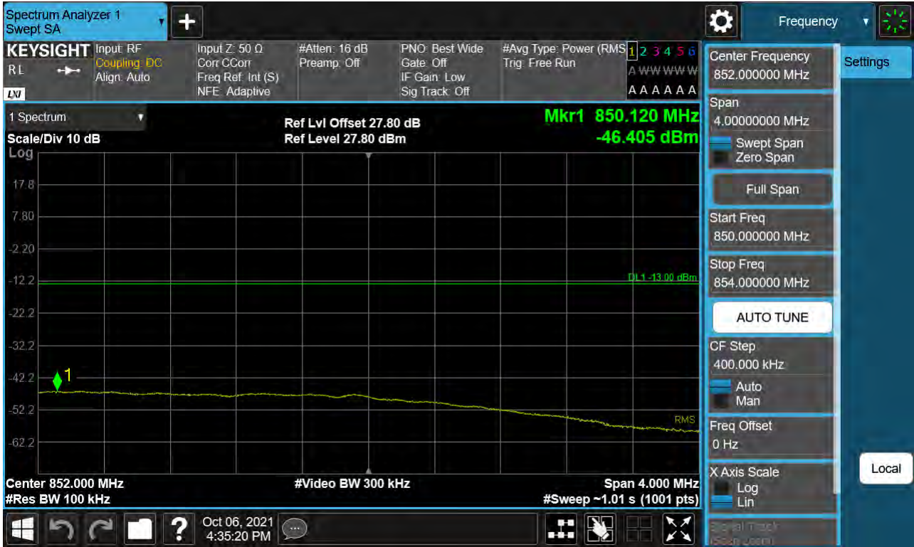
Sub6 n5. Upper Extended Band Edge Plot (20 M BW Ch.167800 BPSK_RB100_0)
