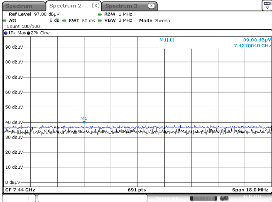
Radiated Spurious Emissions plot – Peak & Average Result ( \pi/4 DQPSK, Ch.78 3rd Harmonic, Z-H)
