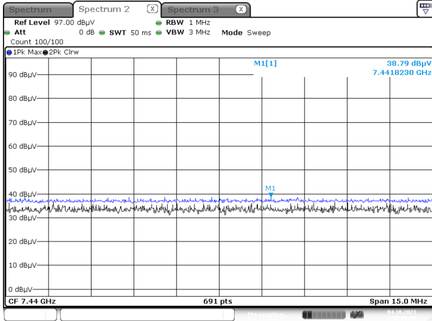
Radiated Spurious Emissions plot – Peak & Average Result (GFSK, Ch.78 3rd Harmonic, Z-H)
