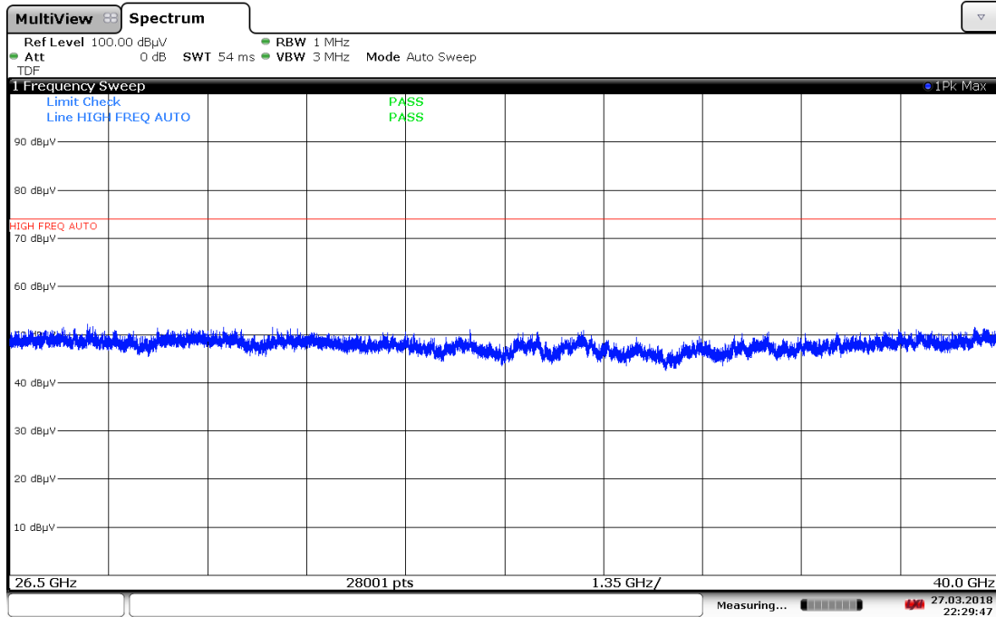
Plot 7-86. Radiated Spurious Plot 26.5GHz - 40GHz (802.11a) – Vertical
