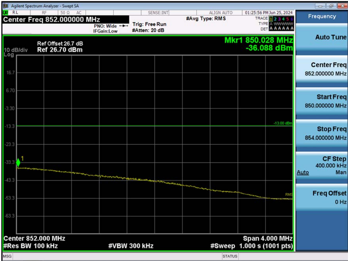
BAND26. Upper Extended Band Edge Plot (3 M BW Ch.27025 QPSK_RB15_0)
