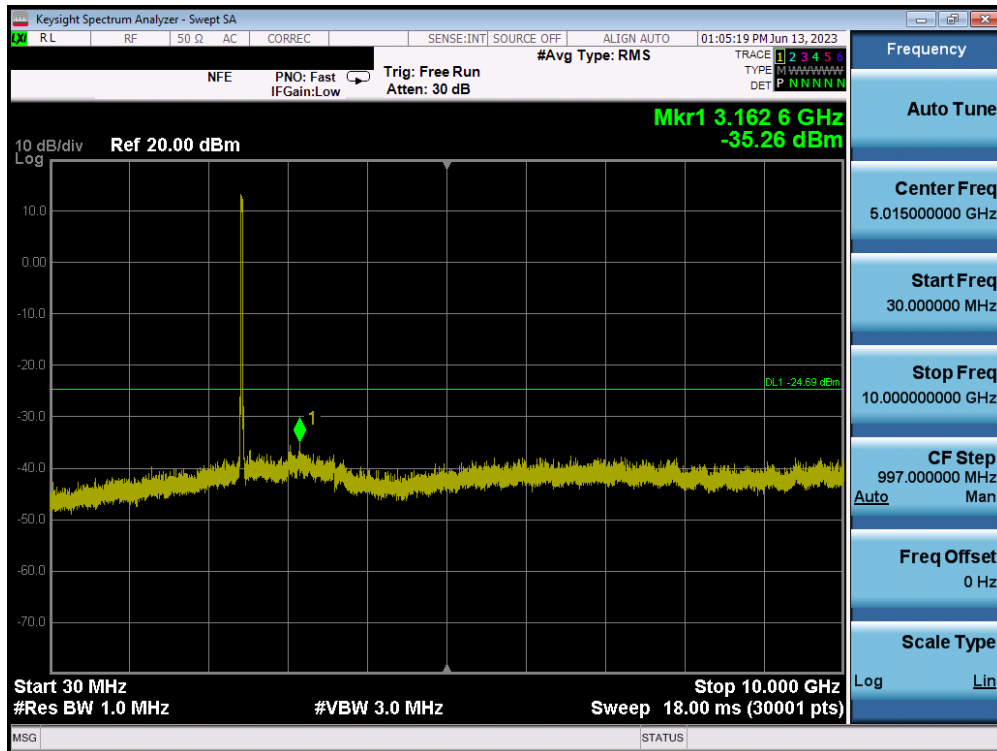
Plot 7-69. Conducted Spurious Plot MIMO ANT1 (802.11ax OFDMA – 242 Tones – Ch. 6) – ANT 1
