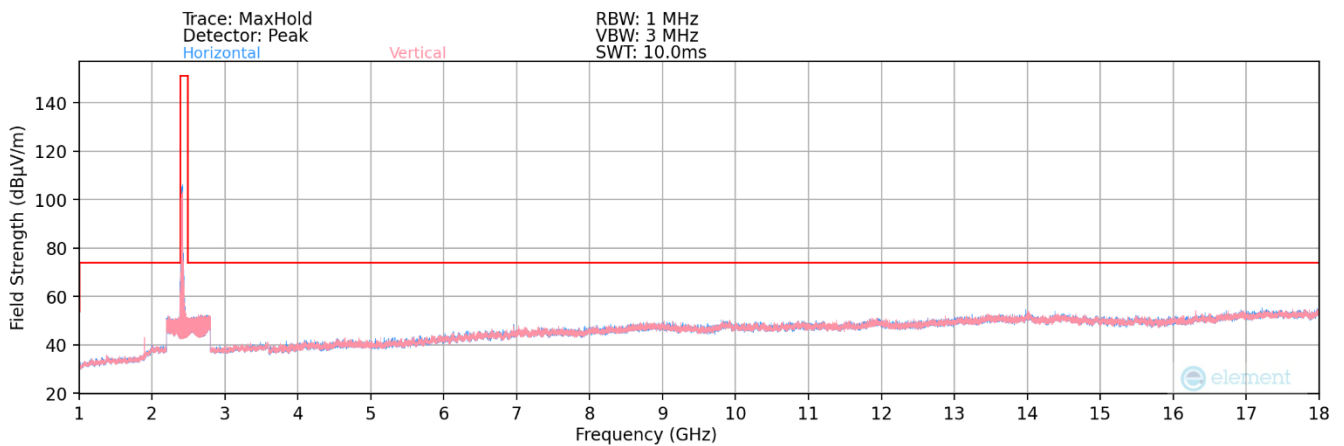
Plot 7-89. Radiated Spurious Plot above 1GHz SISO ANT2 (802.11ax OFDMA – 242 Tones – Ch. 1)
