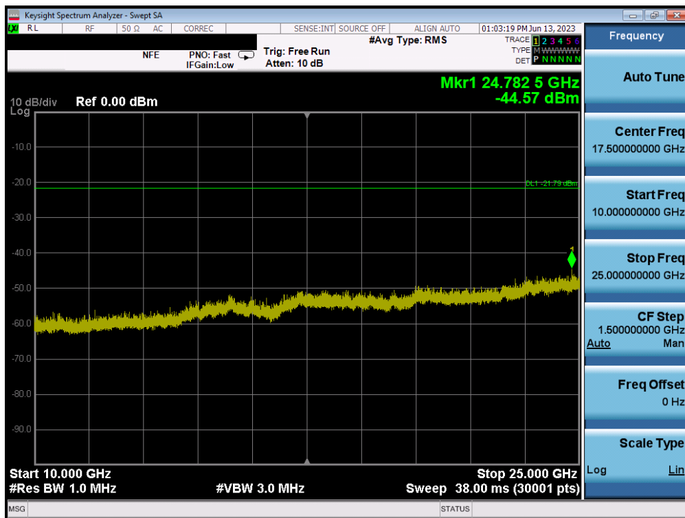
Plot 7-64. Conducted Spurious Plot MIMO ANT1 (802.11ax OFDMA – 26 Tones – Ch. 6) – ANT 1
