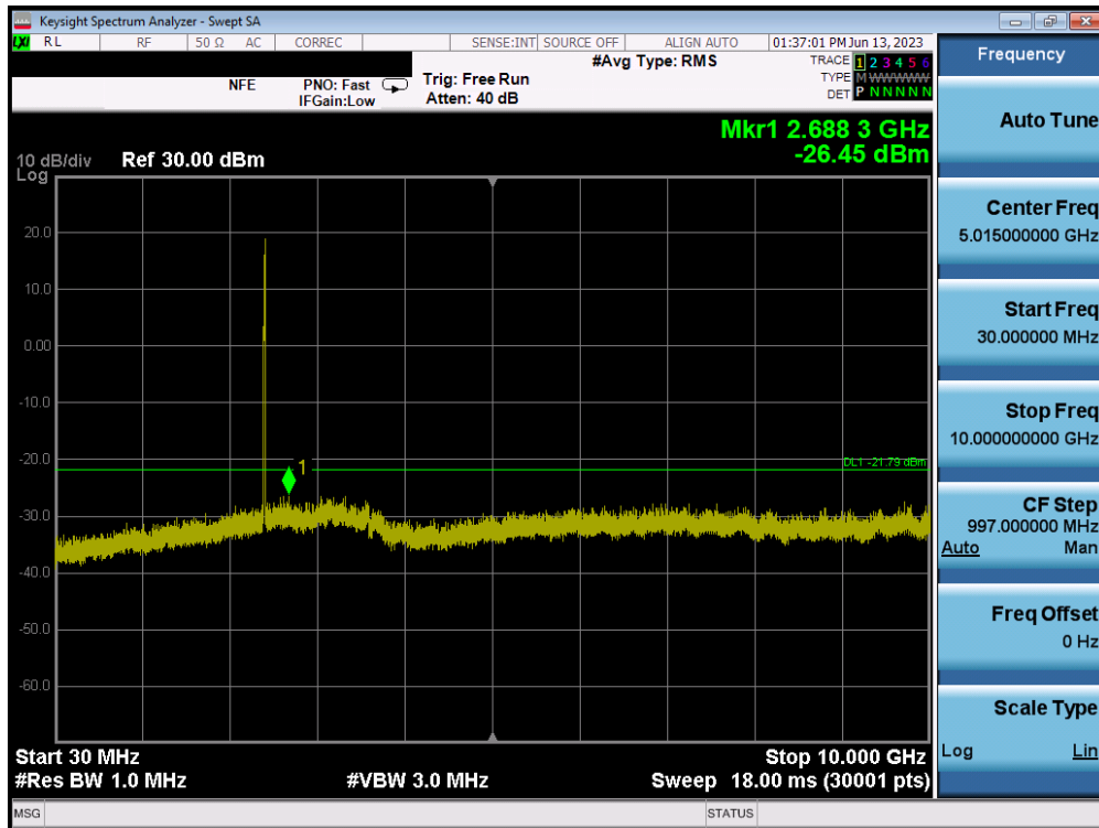
Plot 7-73. Conducted Spurious Plot MIMO ANT1 (802.11ax OFDMA – 26 Tones – Ch. 1) – ANT 2
