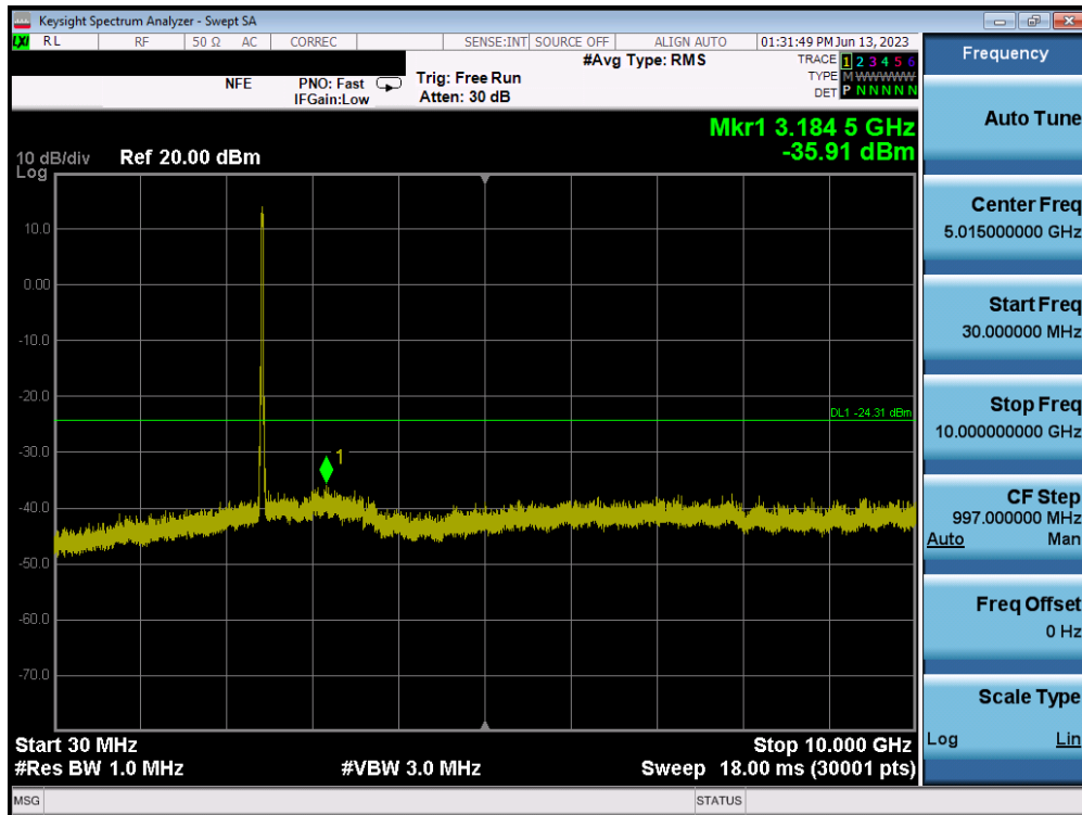
Plot 7-81. Conducted Spurious Plot MIMO ANT2 (802.11ax OFDMA – 242 Tones – Ch. 6) – ANT 2
