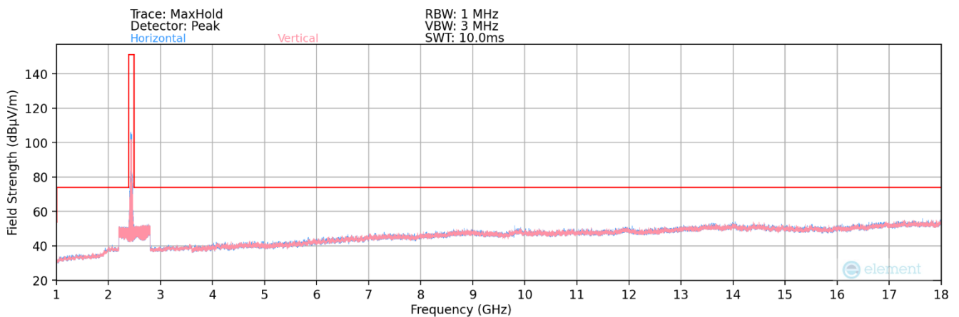
Plot 7-90. Radiated Spurious Plot above 1GHz SISO ANT2 (802.11ax OFDMA – 242 Tones – Ch. 6)
