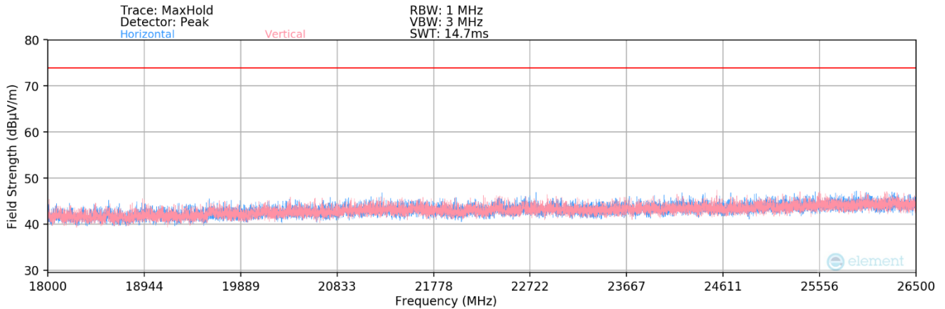
Plot 7-88. Radiated Spurious Plot above 18GHz SISO ANT2 (802.11ax OFDMA – 26 Tones)
