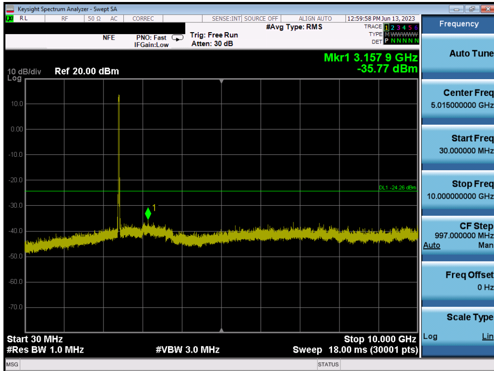
Plot 7-67. Conducted Spurious Plot MIMO ANT1 (802.11ax OFDMA – 242 Tones – Ch. 1) – ANT 1
