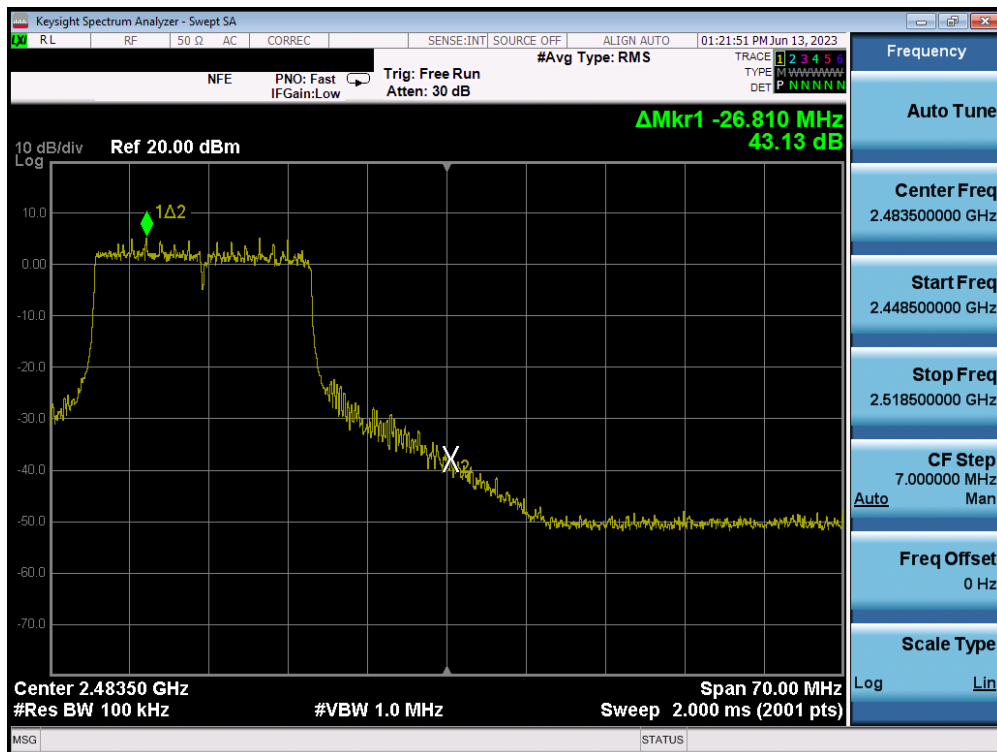
Plot 7-48. Band Edge Plot MIMO ANT2 (802.11ax OFDMA – 242 Tones – Ch. 11) – ANT 2
