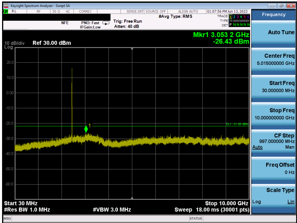
Plot 7-65. Conducted Spurious Plot MIMO ANT1 (802.11ax OFDMA – 26 Tones – Ch. 11) – ANT 1
