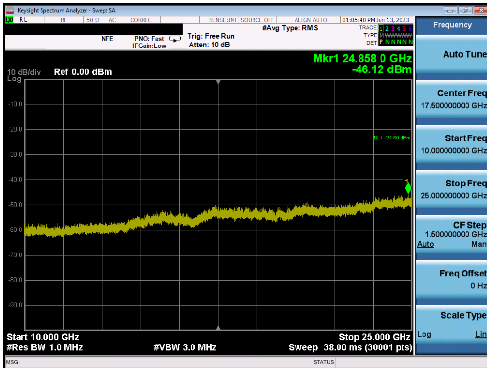
Plot 7-70. Conducted Spurious Plot MIMO ANT1 (802.11ax OFDMA – 242 Tones – Ch. 6) – ANT 1
