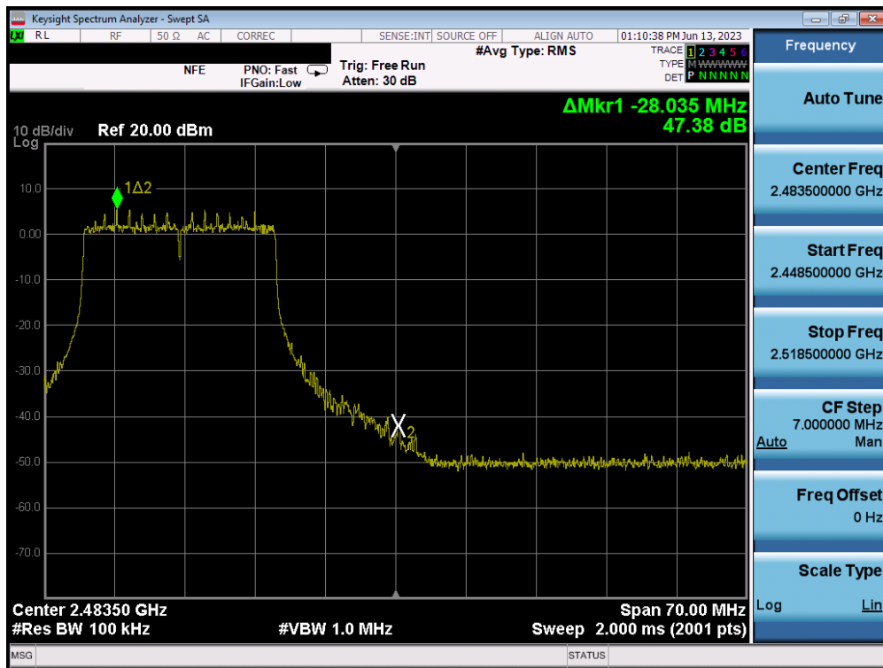
Plot 7-44. Band Edge Plot MIMO ANT1 (802.11ax OFDMA – 242 Tones – Ch. 11) – ANT 1
