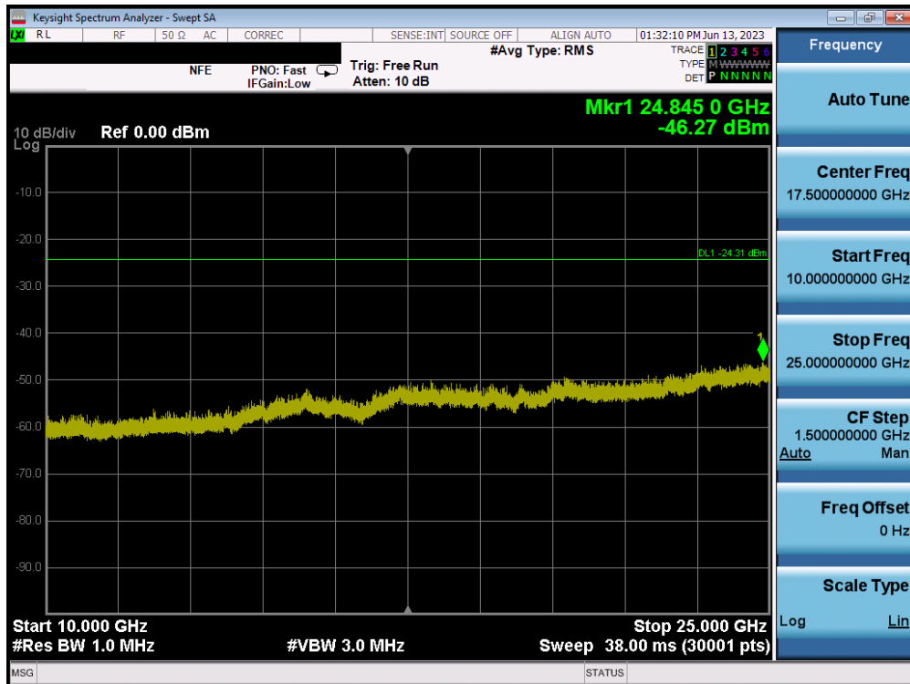
Plot 7-82. Conducted Spurious Plot MIMO ANT2 (802.11ax OFDMA – 242 Tones – Ch. 6) – ANT 2
