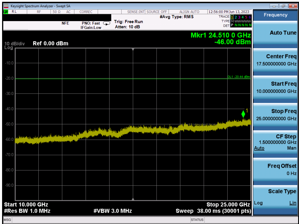
Plot 7-62. Conducted Spurious Plot MIMO ANT1 (802.11ax OFDMA – 26 Tones – Ch. 1) – ANT 1
