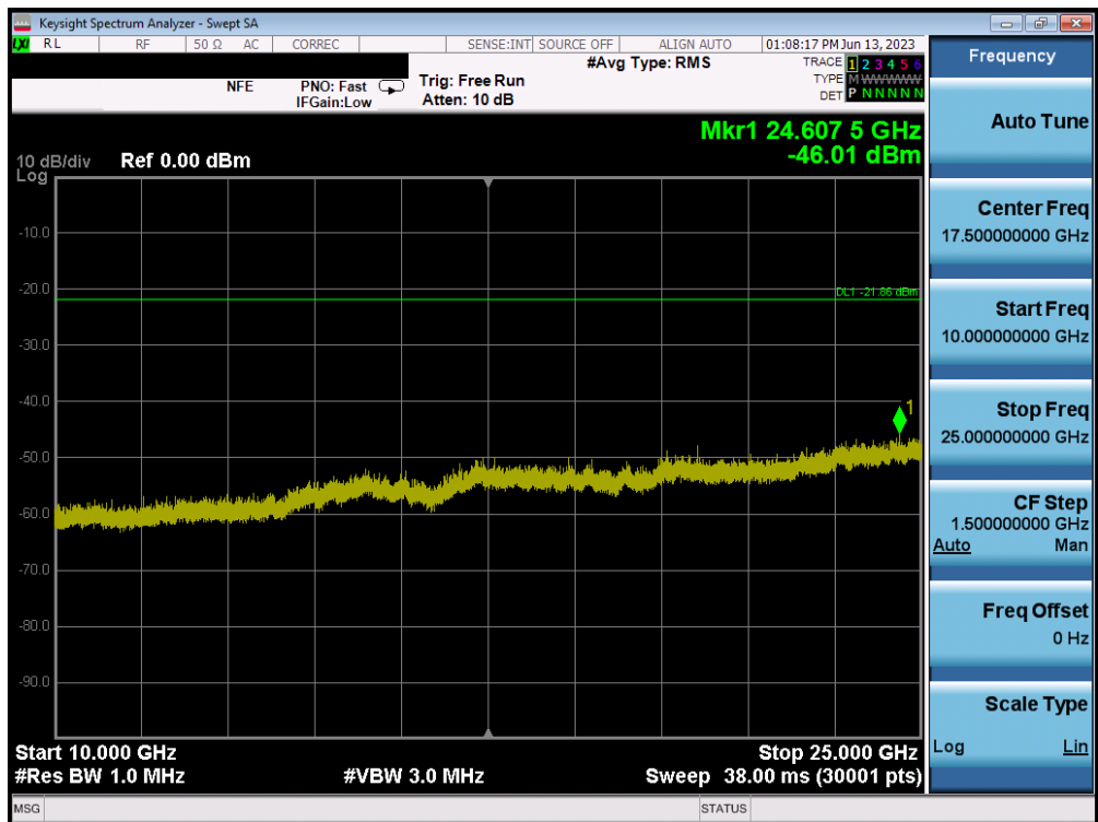
Plot 7-66. Conducted Spurious Plot MIMO ANT1 (802.11ax OFDMA – 26 Tones – Ch. 11) – ANT 1
