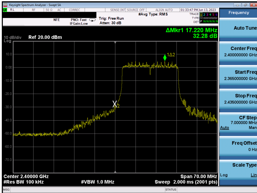
Plot 7-47. Band Edge Plot MIMO ANT2 (802.11ax OFDMA – 242 Tones – Ch. 1) – ANT 2
