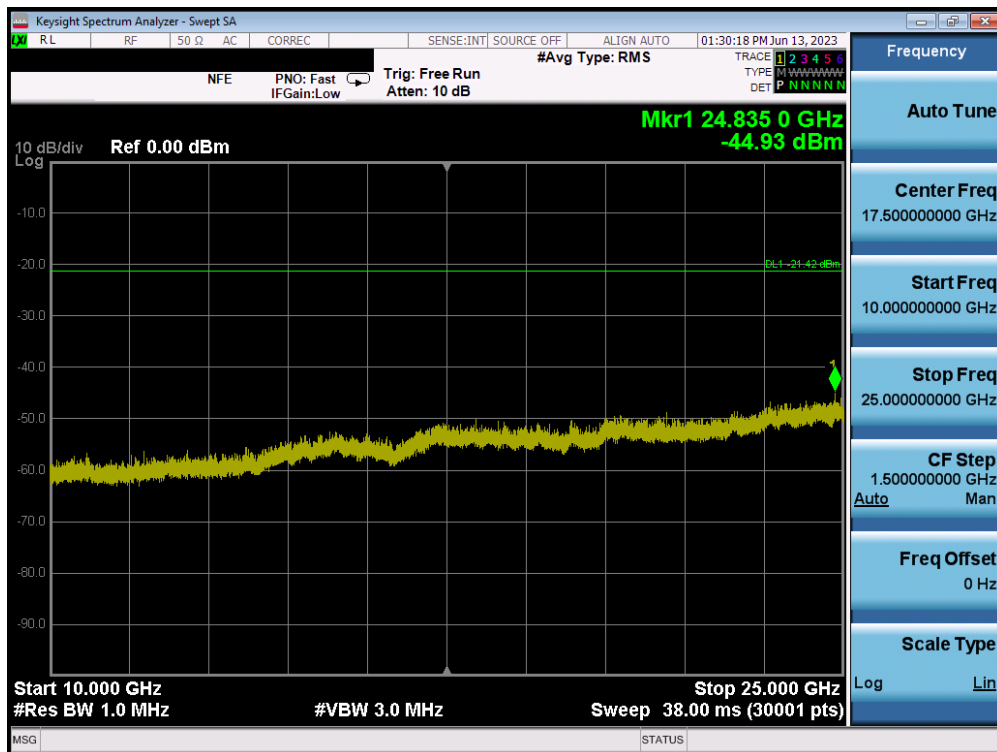
Plot 7-76. Conducted Spurious Plot MIMO ANT2 (802.11ax OFDMA – 26 Tones – Ch. 6) – ANT 2
