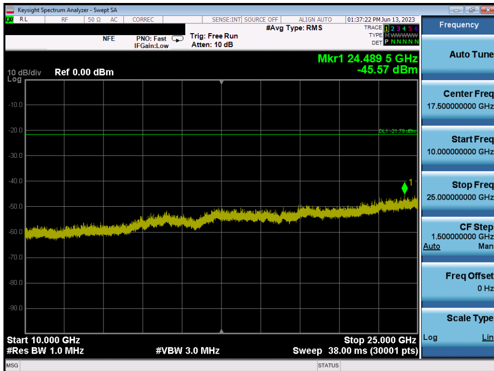
Plot 7-74. Conducted Spurious Plot MIMO ANT2 (802.11ax OFDMA – 26 Tones – Ch. 1) – ANT 2
