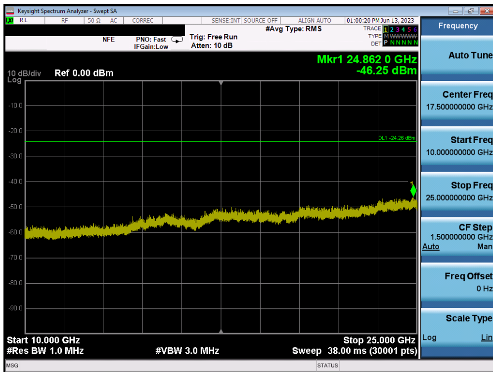
Plot 7-68. Conducted Spurious Plot MIMO ANT1 (802.11ax OFDMA – 242 Tones – Ch. 1) – ANT 1
