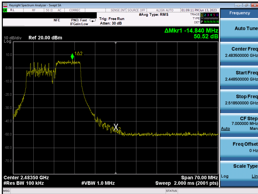
Plot 7-42. Band Edge Plot MIMO ANT1 (802.11ax OFDMA – 106 Tones – Ch. 11) – ANT 1
