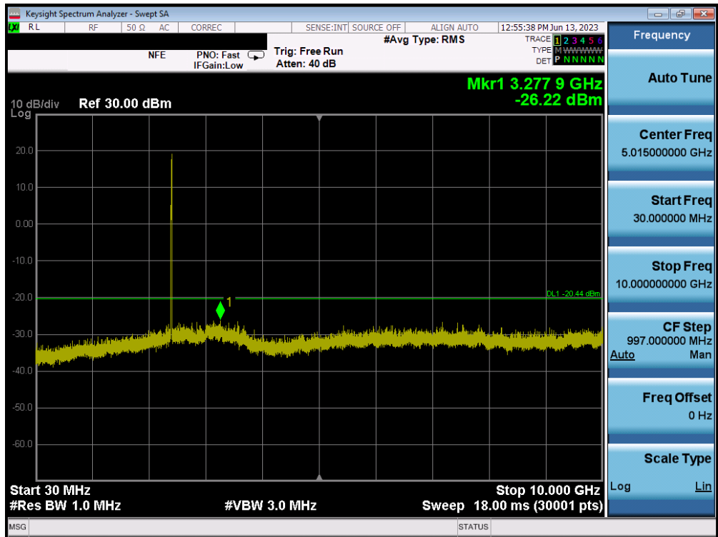
Plot 7-61. Conducted Spurious Plot MIMO ANT1 (802.11ax OFDMA – 26 Tones – Ch. 1) – ANT 1
