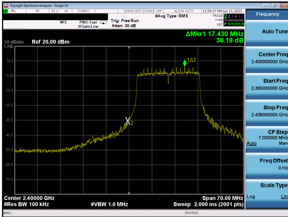
Plot 7-43. Band Edge Plot MIMO ANT1 (802.11ax OFDMA – 242 Tones – Ch. 1) – ANT 1
