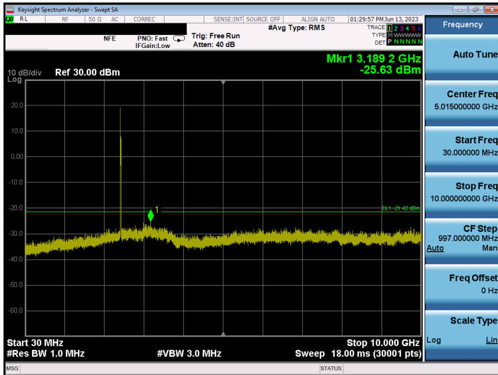
Plot 7-75. Conducted Spurious Plot MIMO ANT2 (802.11ax OFDMA – 26 Tones – Ch. 6) – ANT 2
