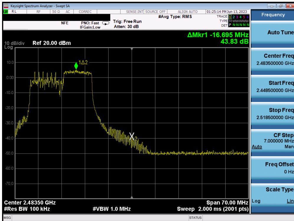
Plot 7-46. Band Edge Plot MIMO ANT2 (802.11ax OFDMA – 106 Tones – Ch. 11) – ANT 2
