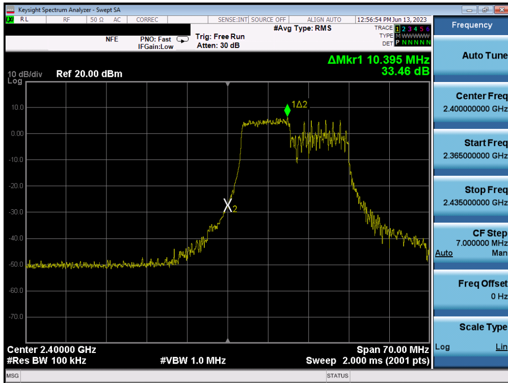
Plot 7-41. Band Edge Plot MIMO ANT1 (802.11ax OFDMA – 106 Tones – Ch. 1) – ANT 1
