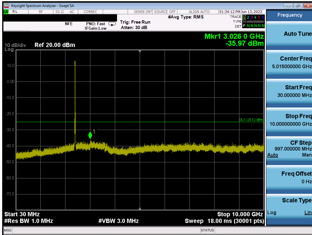
Plot 7-79. Conducted Spurious Plot MIMO ANT2 (802.11ax OFDMA – 242 Tones – Ch. 1) – ANT 2
