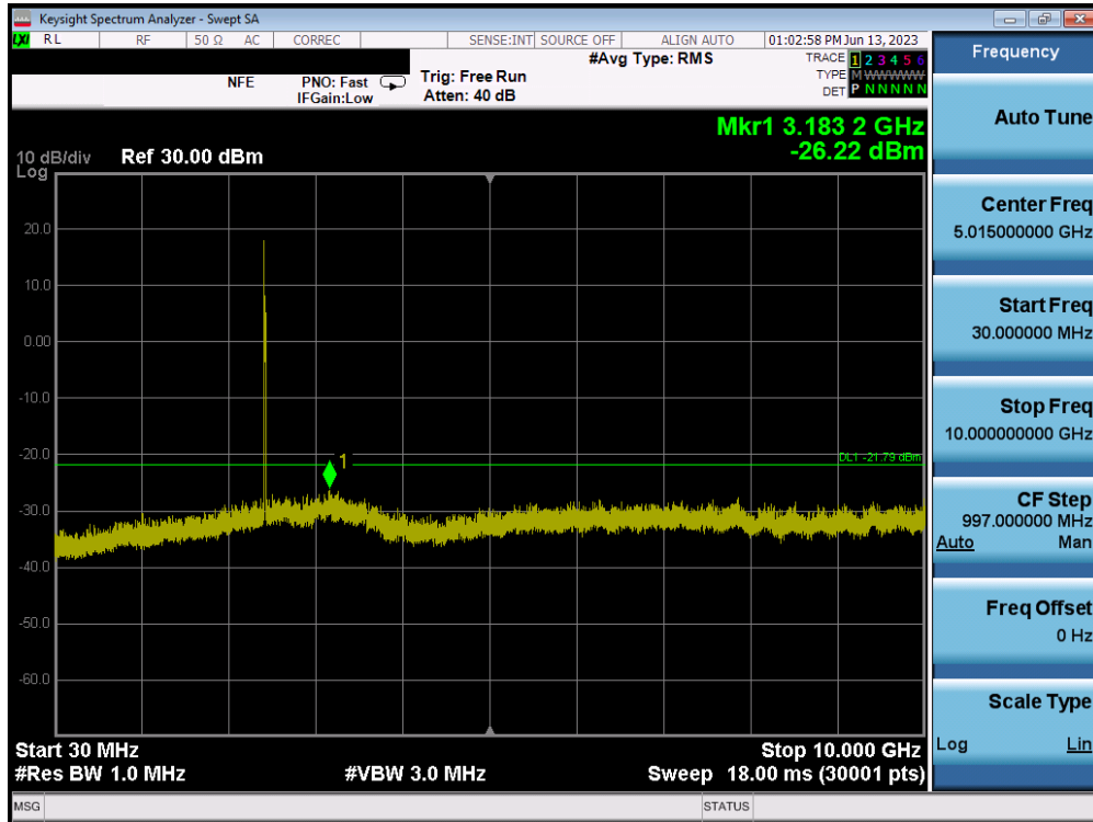
Plot 7-63. Conducted Spurious Plot MIMO ANT1 (802.11ax OFDMA – 26 Tones – Ch. 6) – ANT 1
