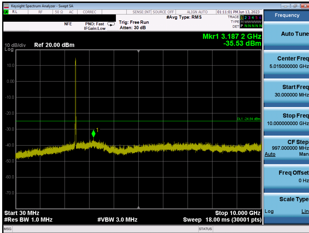
Plot 7-71. Conducted Spurious Plot MIMO ANT1 (802.11ax OFDMA – 242 Tones – Ch. 11) – ANT 1
