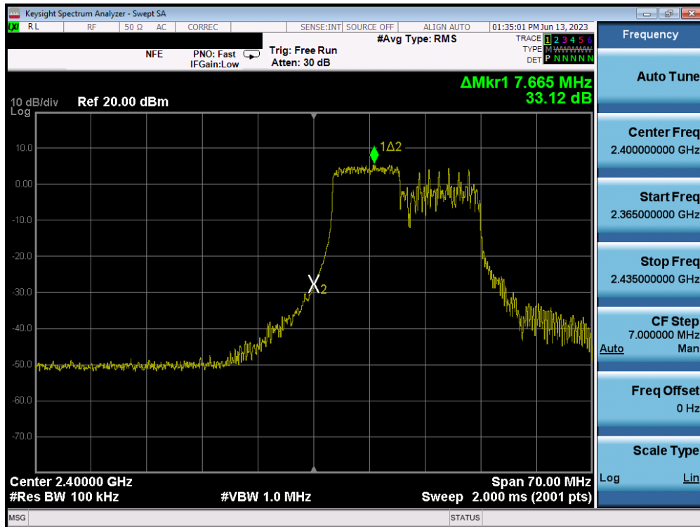
Plot 7-45. Band Edge Plot MIMO ANT2 (802.11ax OFDMA – 106 Tones – Ch. 1) – ANT 2
