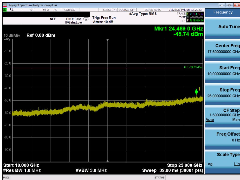
Plot 7-84. Conducted Spurious Plot MIMO ANT2 (802.11ax OFDMA – 242 Tones – Ch. 11) – ANT 2
