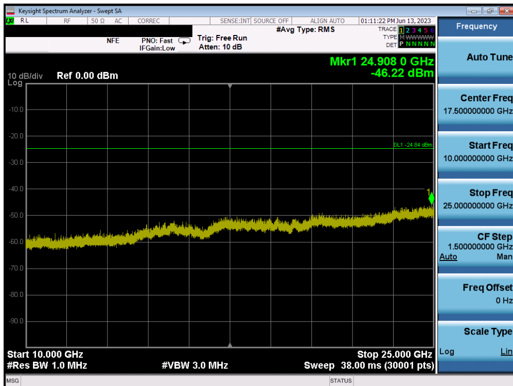
Plot 7-72. Conducted Spurious Plot MIMO ANT1 (802.11ax OFDMA – 242 Tones – Ch. 11) – ANT 1
