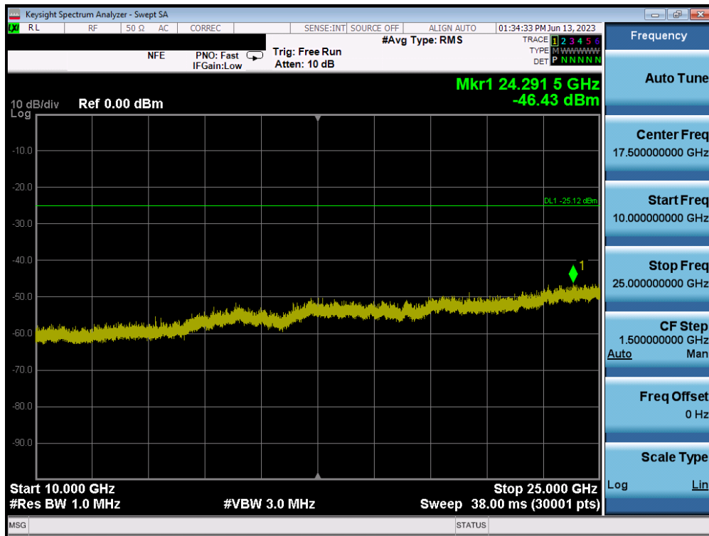
Plot 7-80. Conducted Spurious Plot MIMO ANT2 (802.11ax OFDMA – 242 Tones – Ch. 1) – ANT 2
