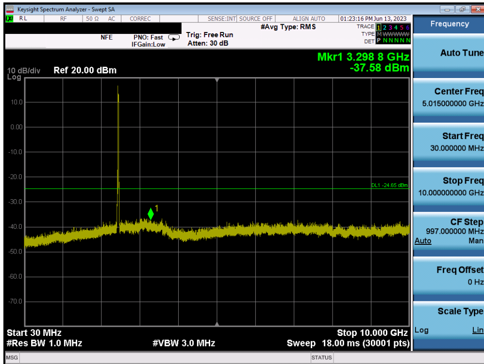
Plot 7-83. Conducted Spurious Plot MIMO ANT2 (802.11ax OFDMA – 242 Tones – Ch. 11) – ANT 2
