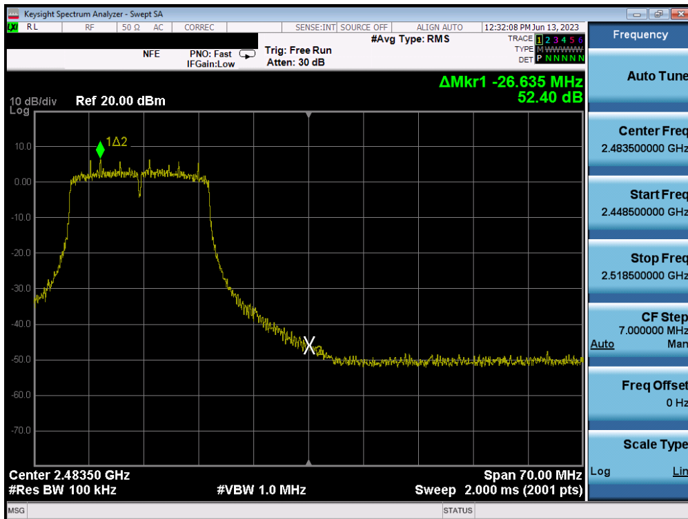
Plot 7-86. Band Edge Plot MIMO ANT1 (802.11n (2.4GHz) – Ch. 11)
