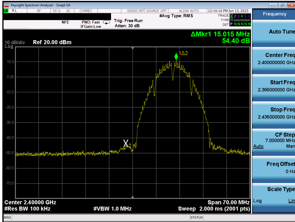
Plot 7-81. Band Edge Plot MIMO ANT1 (802.11b – Ch. 1)
