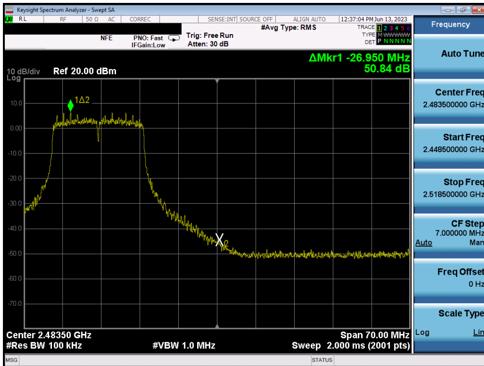
Plot 7-84. Band Edge Plot MIMO ANT1 (802.11g - Ch. 11)
