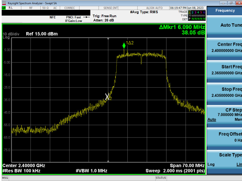
Plot 7-77. Band Edge Plot SISO ANT2 (802.11n (2.4GHz) – Ch. 1)
