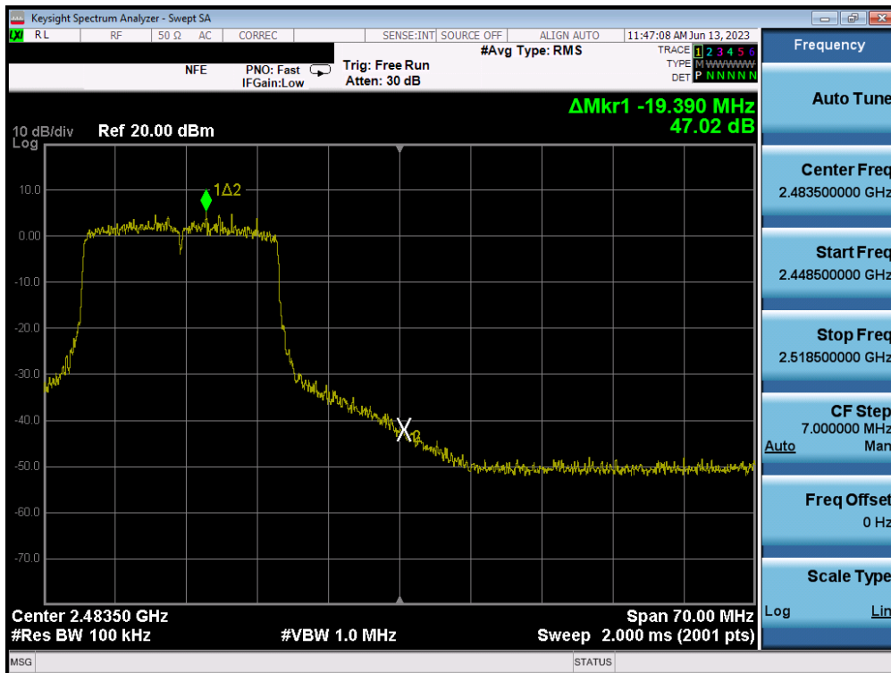
Plot 7-96. Band Edge Plot MIMO ANT2 (802.11ax (2.4GHz) – Ch. 11)
