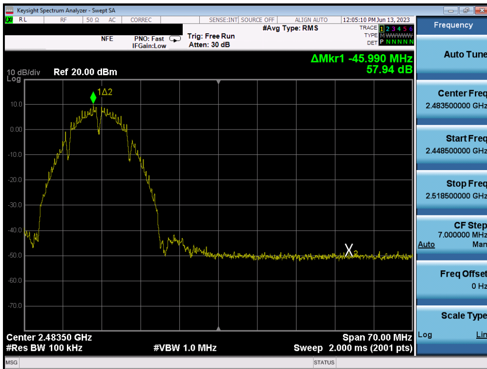
Plot 7-90. Band Edge Plot MIMO ANT2 (802.11b – Ch. 11)
