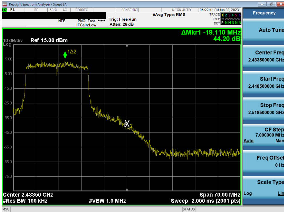
Plot 7-78. Band Edge Plot SISO ANT2 (802.11n (2.4GHz) – Ch. 11)
