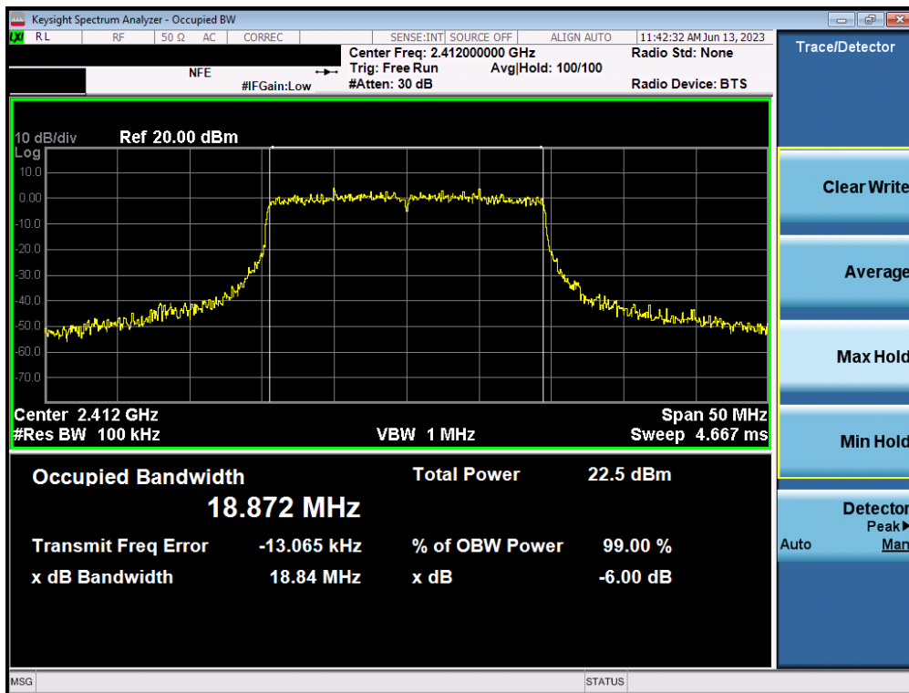
Plot 7-34. 6dB Bandwidth Plot MIMO ANT2 (802.11ax (2.4GHz) – Ch. 1)
