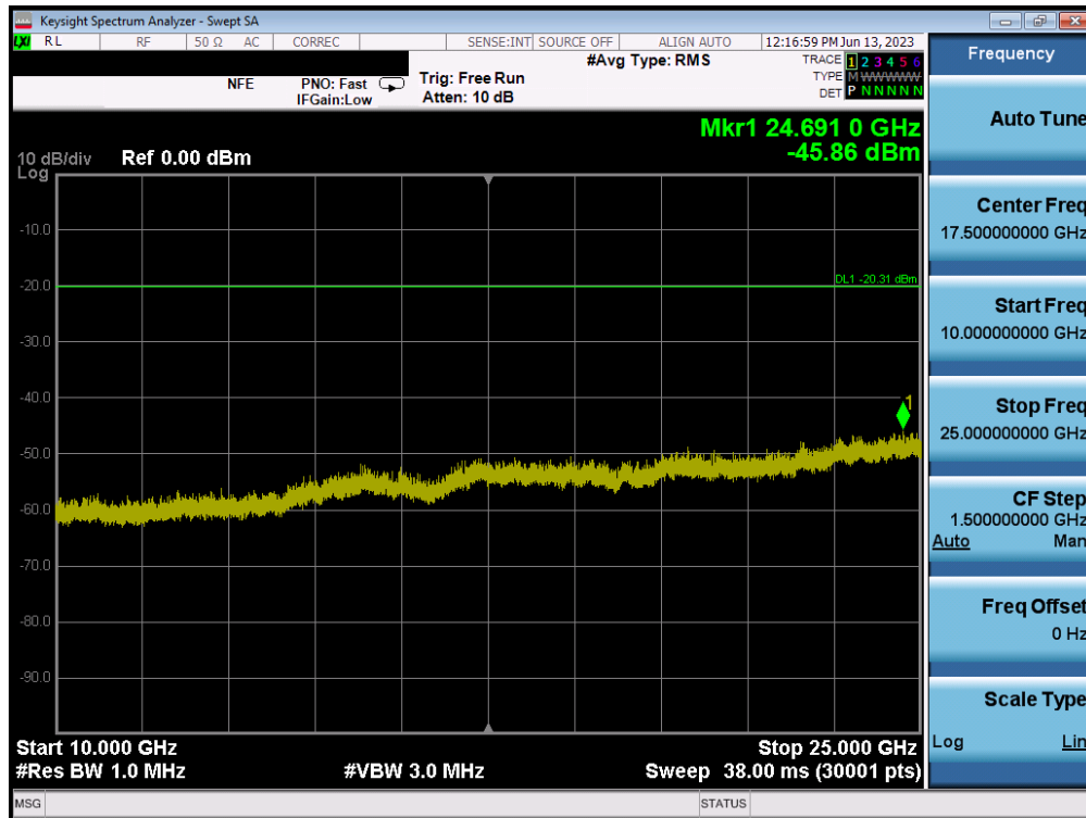
Plot 7-104. Conducted Spurious Plot MIMO ANT1 (802.11b – Ch. 1)
