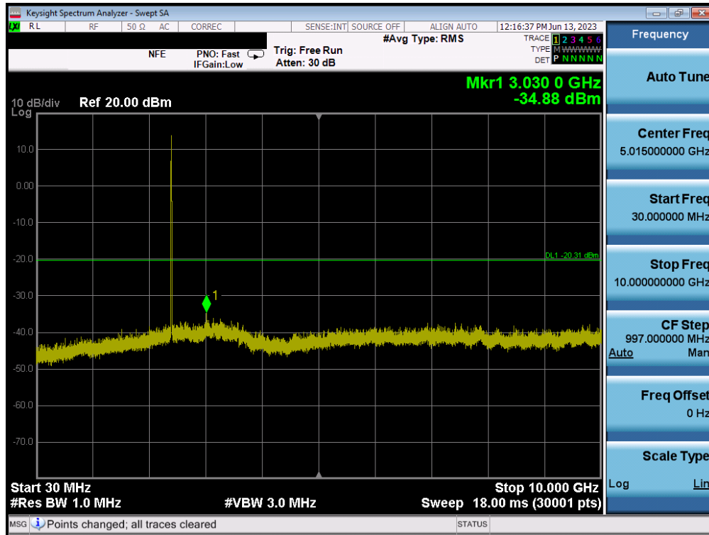
Plot 7-103. Conducted Spurious Plot MIMO ANT1 (802.11b – Ch. 1)
