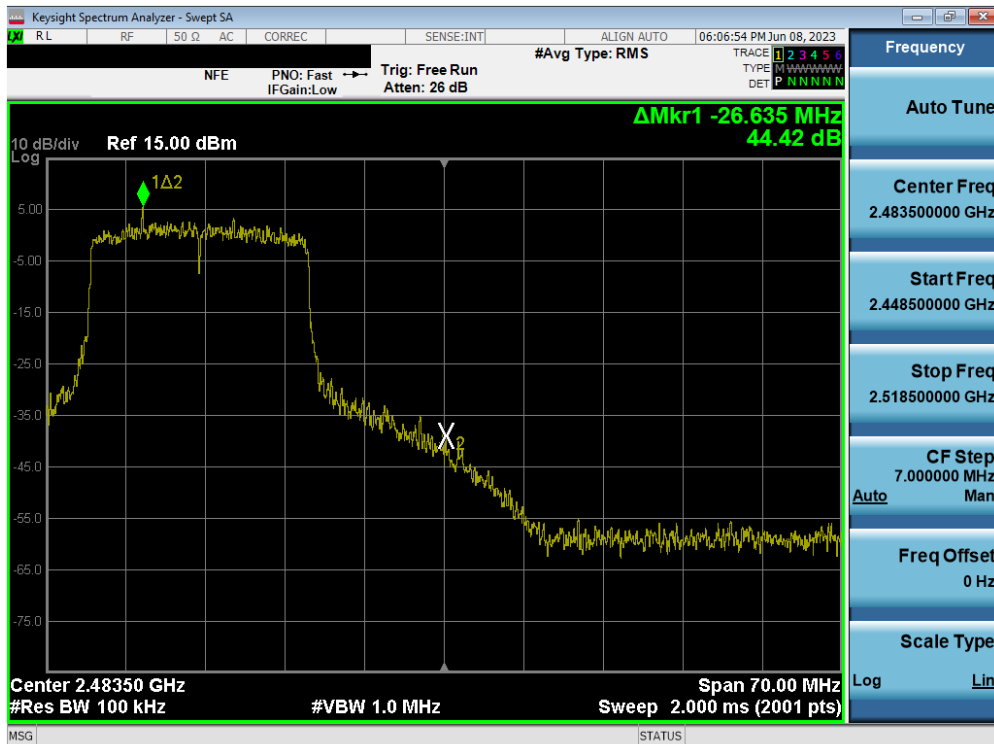
Plot 7-80. Band Edge Plot SISO ANT2 (802.11ax (2.4GHz) – Ch. 11)
