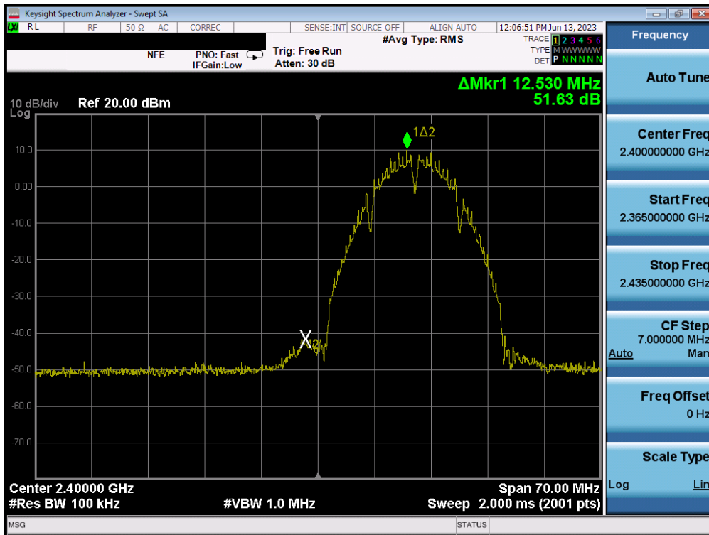
Plot 7-89. Band Edge Plot MIMO ANT2 (802.11b – Ch. 1)
