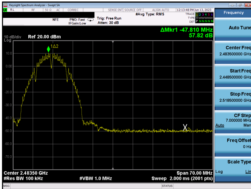
Plot 7-82. Band Edge Plot MIMO ANT1 (802.11b – Ch. 11)
