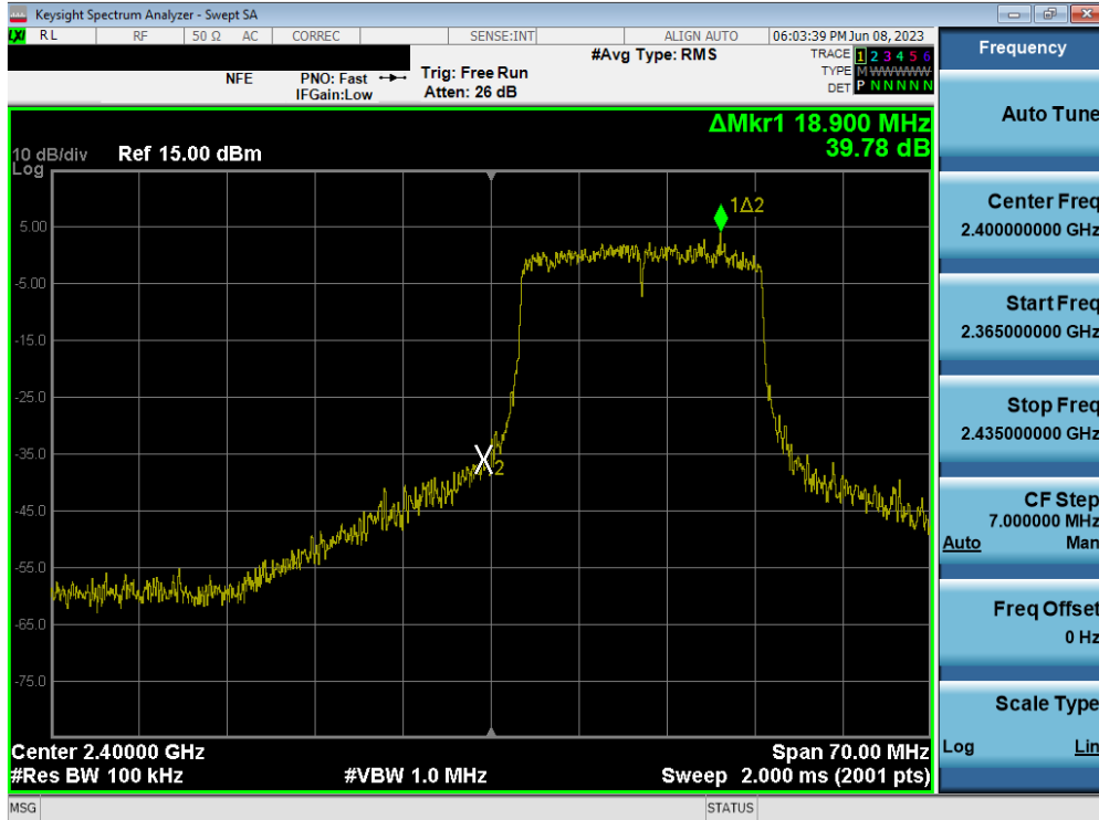
Plot 7-79. Band Edge Plot SISO ANT2 (802.11ax (2.4GHz) – Ch. 1)
