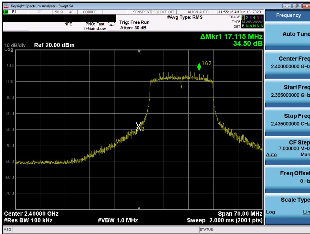
Plot 7-93. Band Edge Plot MIMO ANT2 (802.11n (2.4GHz) – Ch. 1)
