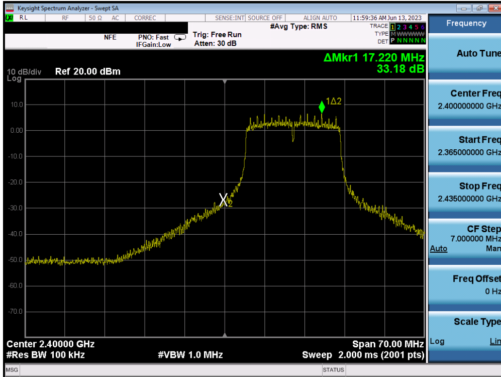
Plot 7-91. Band Edge Plot MIMO ANT2 (802.11g- Ch. 1)
