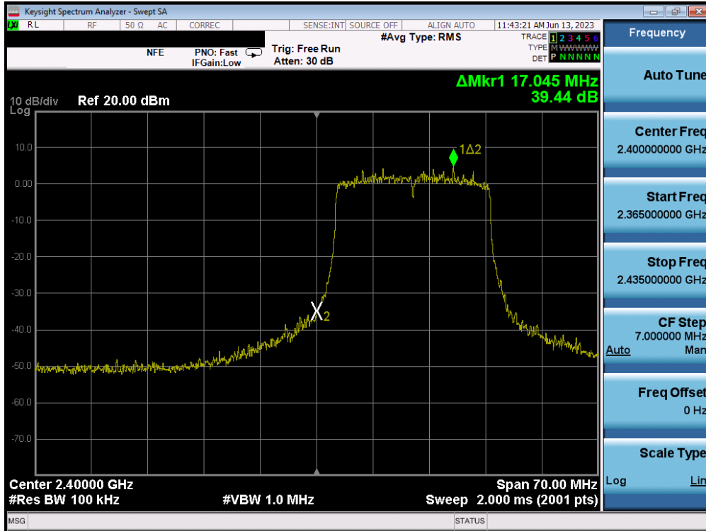
Plot 7-95. Band Edge Plot MIMO ANT2 (802.11ax (2.4GHz) – Ch. 1)
