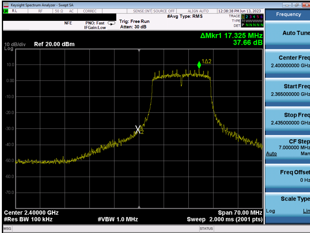
Plot 7-83. Band Edge Plot MIMO ANT1 (802.11g- Ch. 1)
