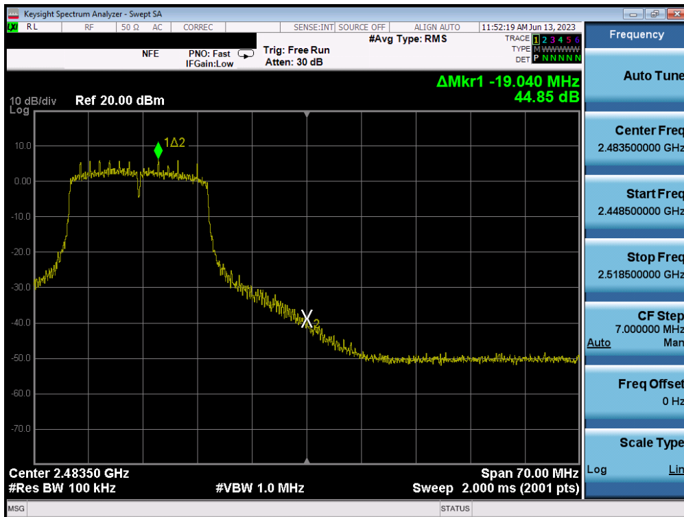
Plot 7-94. Band Edge Plot MIMO ANT2 (802.11n (2.4GHz) – Ch. 11)
