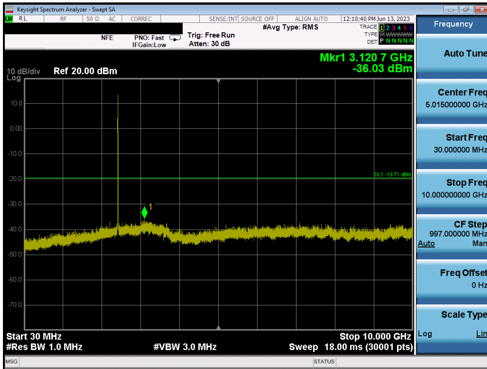
Plot 7-105. Conducted Spurious Plot MIMO ANT1 (802.11b – Ch. 6)
