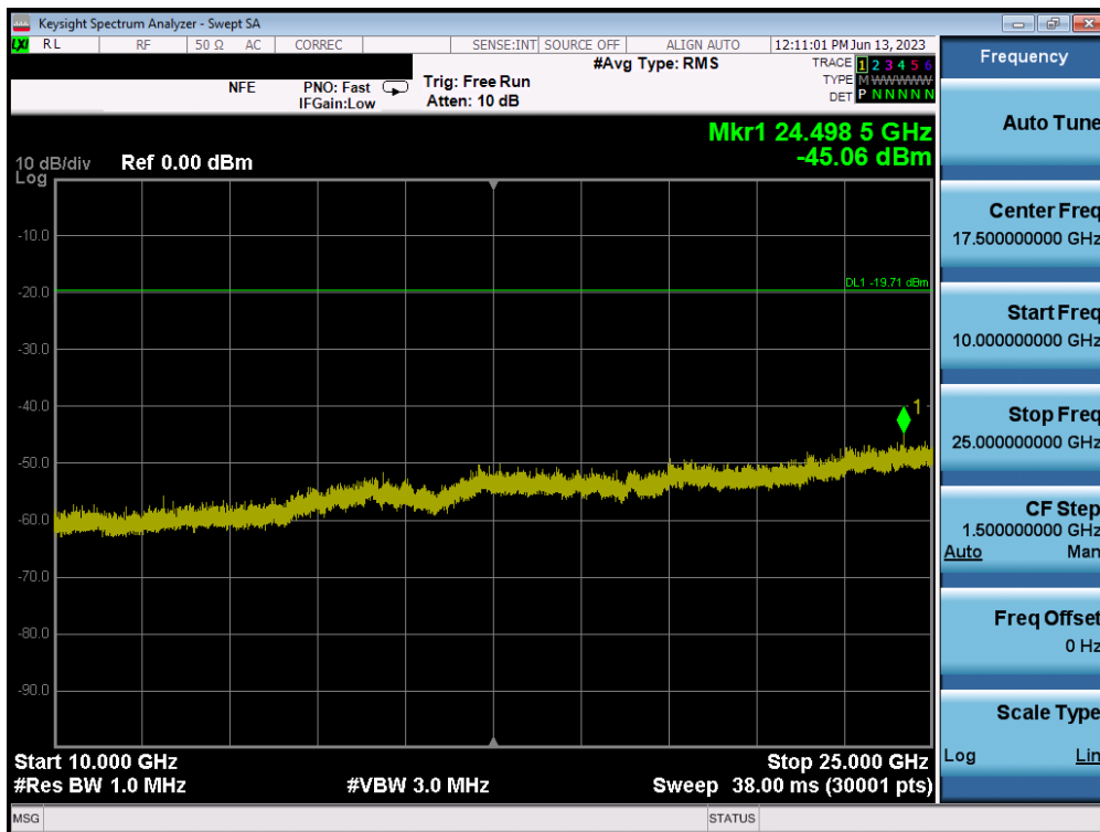
Plot 7-106. Conducted Spurious Plot MIMO ANT1 (802.11b – Ch. 6)
