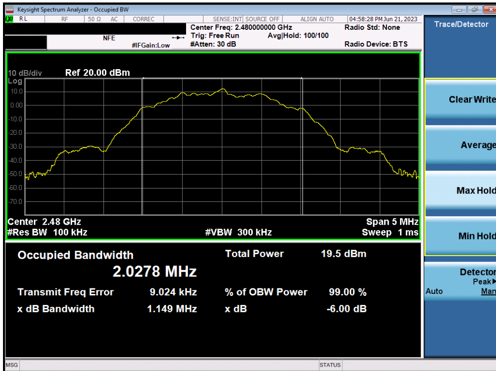
Plot 7-18. 6dB Bandwidth Plot (Bluetooth (LE), 2Mbps – Ch. 39) – ANT 2
