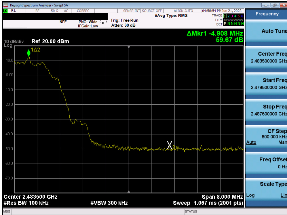
Plot 7-66. Band Edge Plot (Bluetooth (LE), 2Mbps – Ch. 39) – ANT 2
