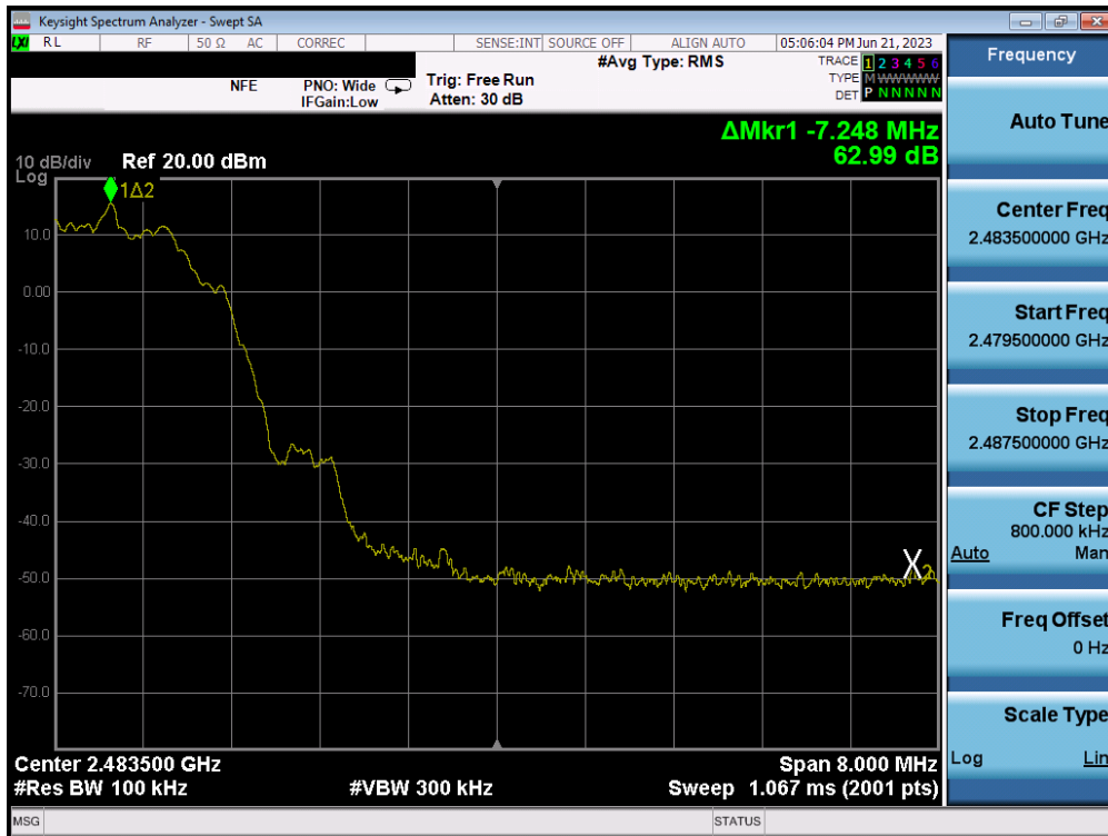
Plot 7-62. Band Edge Plot (Bluetooth (LE), 2Mbps – Ch. 39) – ANT 1
