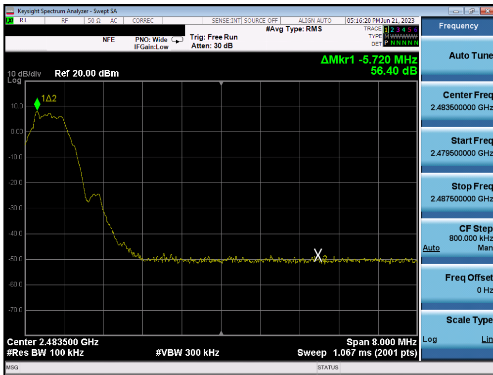
Plot 7-58. Band Edge Plot (Bluetooth (LE), 500kbps – Ch. 39) – ANT 1
