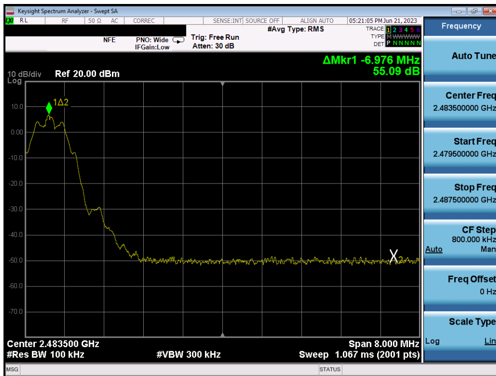
Plot 7-56. Band Edge Plot (Bluetooth (LE), 125kbps – Ch. 39) – ANT 1
